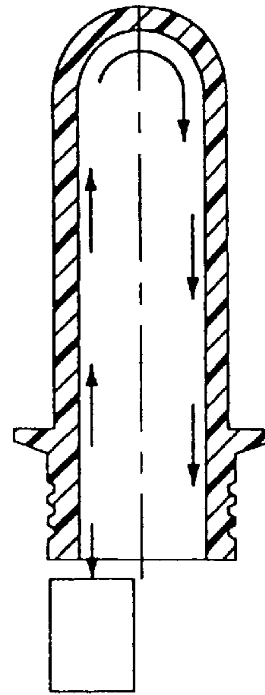
FIG. 20 (PRIOR ART)
