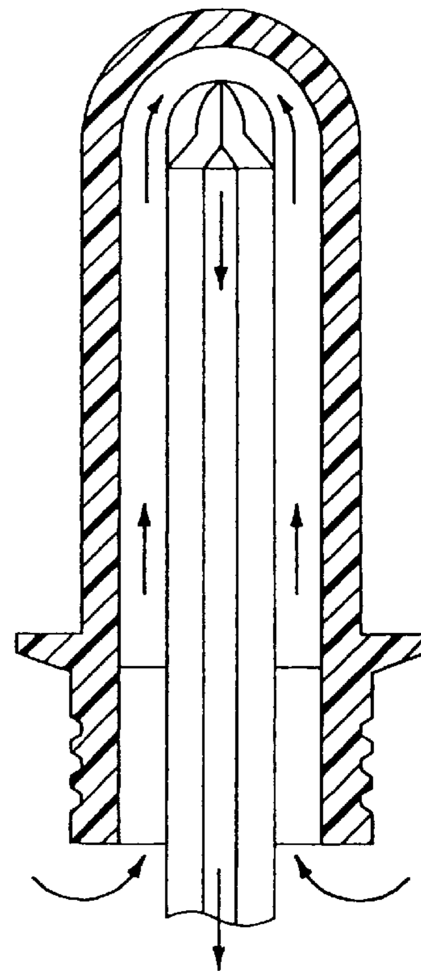
FIG. 22 (PRIOR ART)
