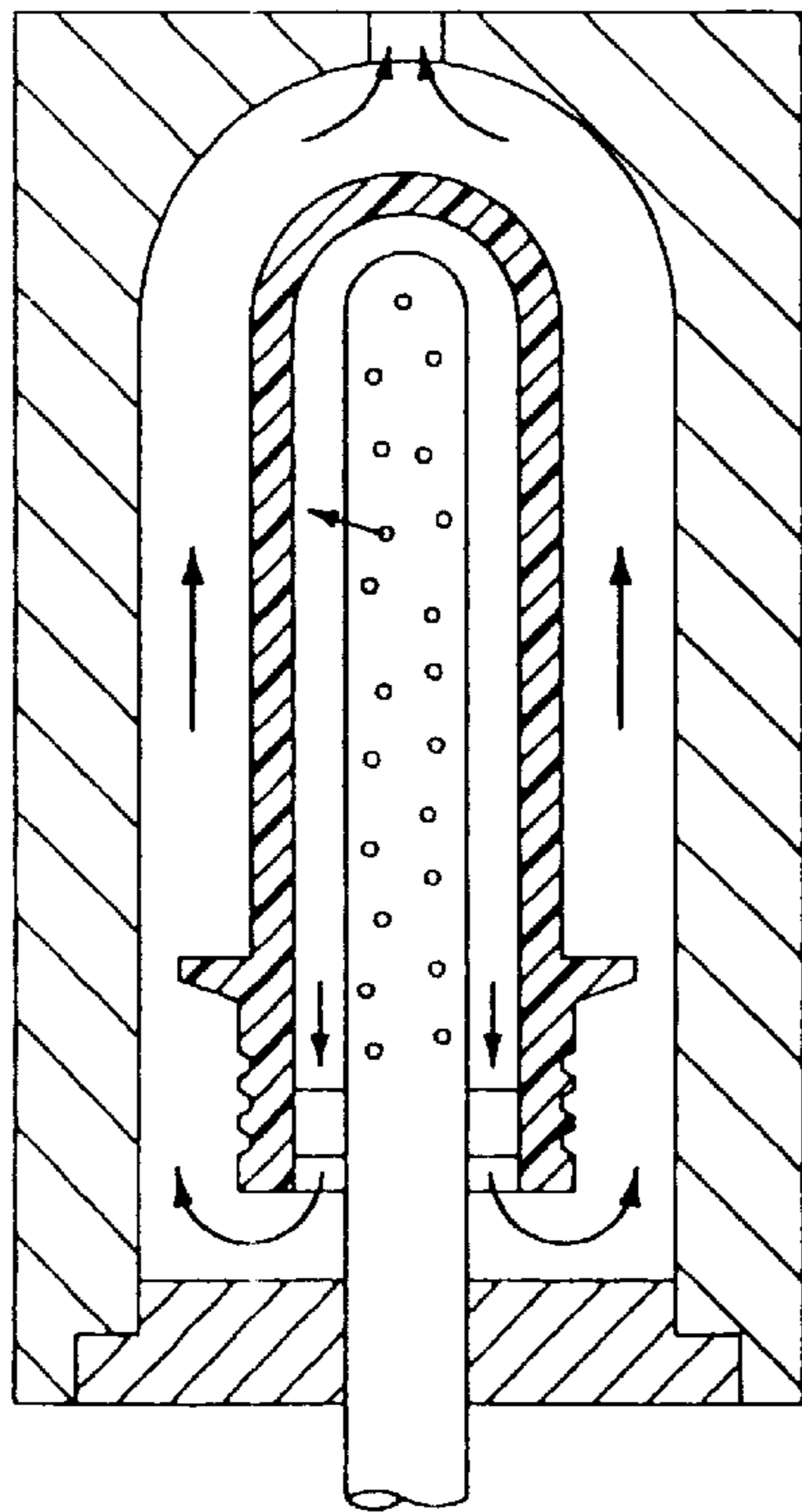
FIG. 21 (PRIOR ART)
