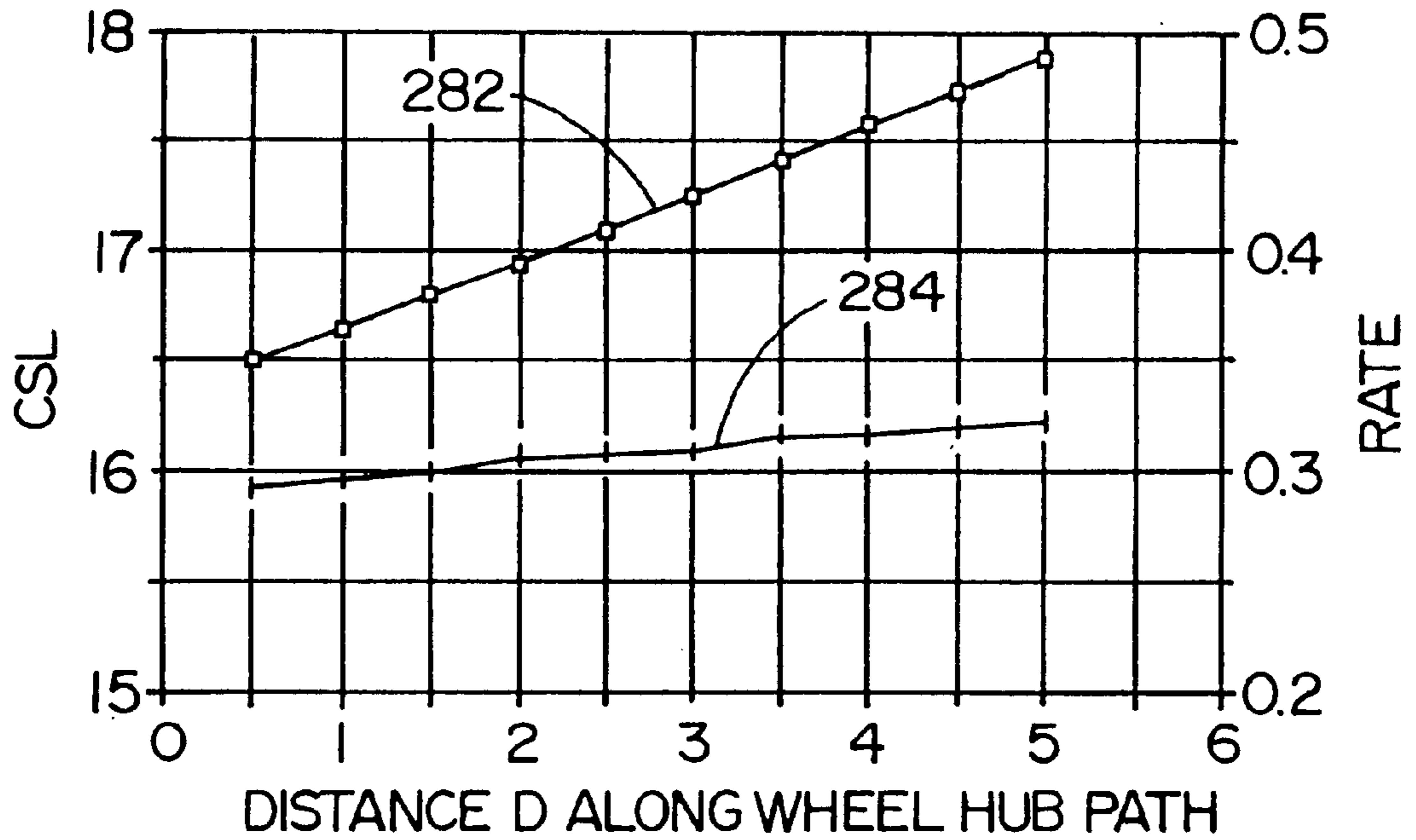
FIG. 17 PRIOR ART
