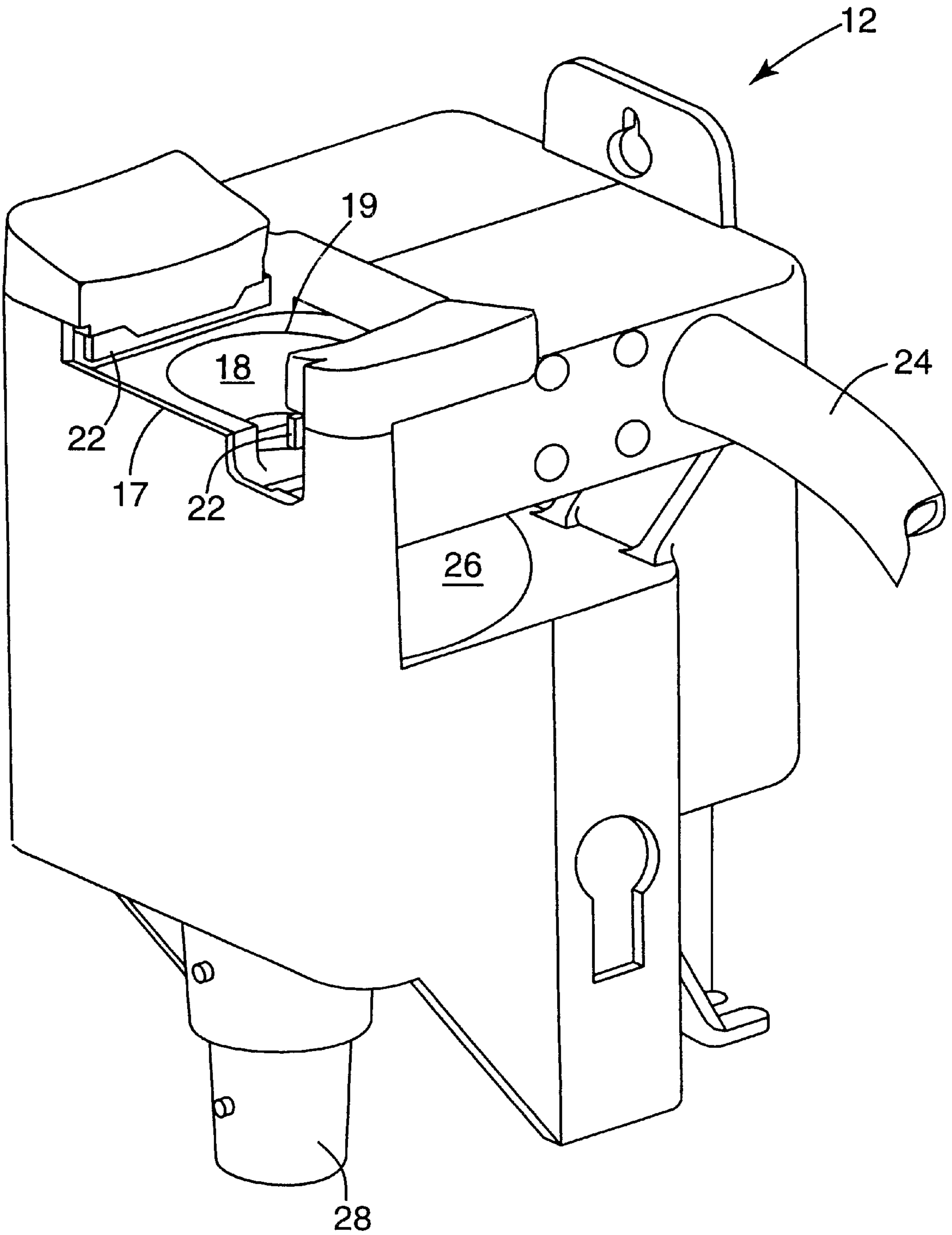
FIG. 1 PRIOR ART
