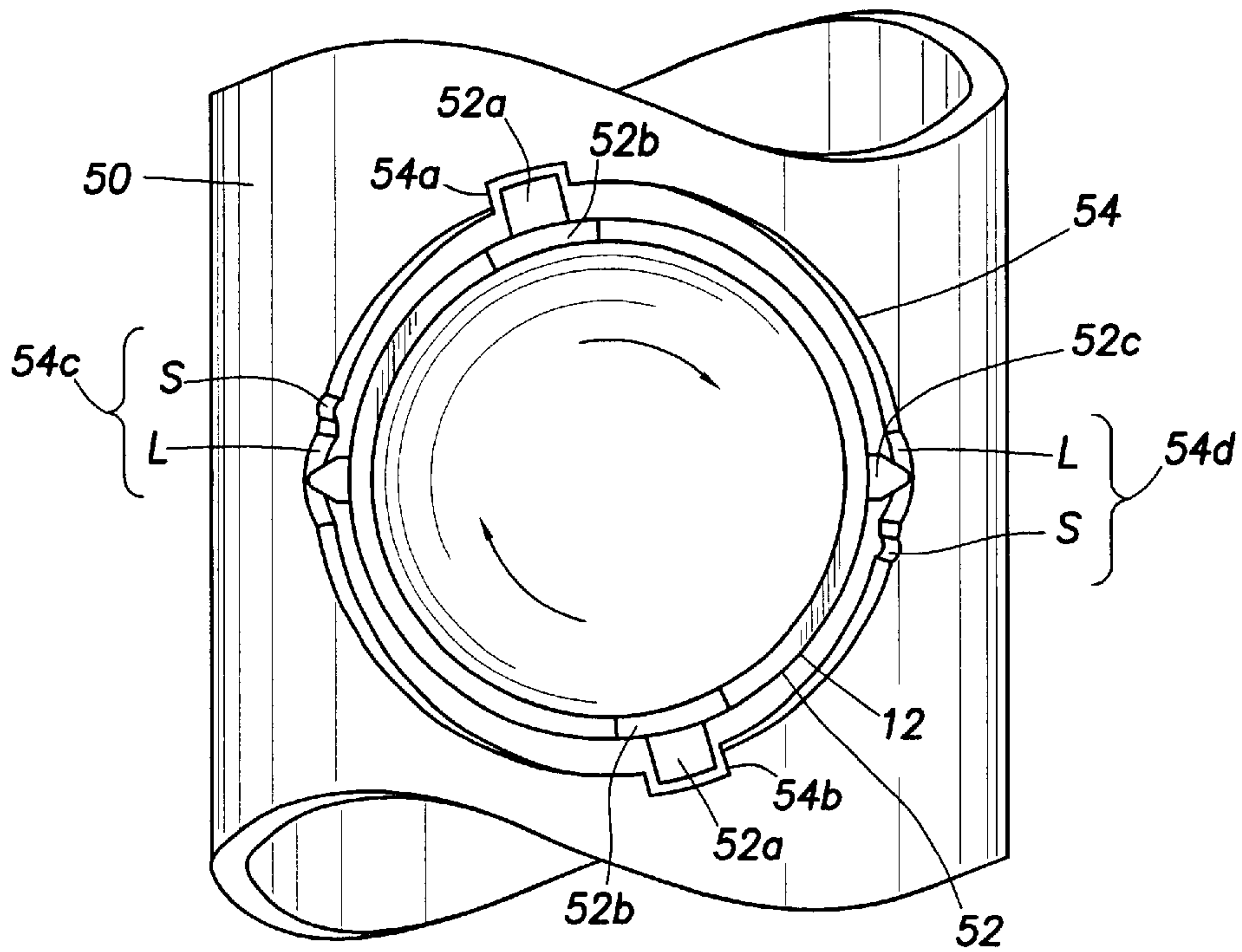
FIG. 6 (PRIOR ART)
