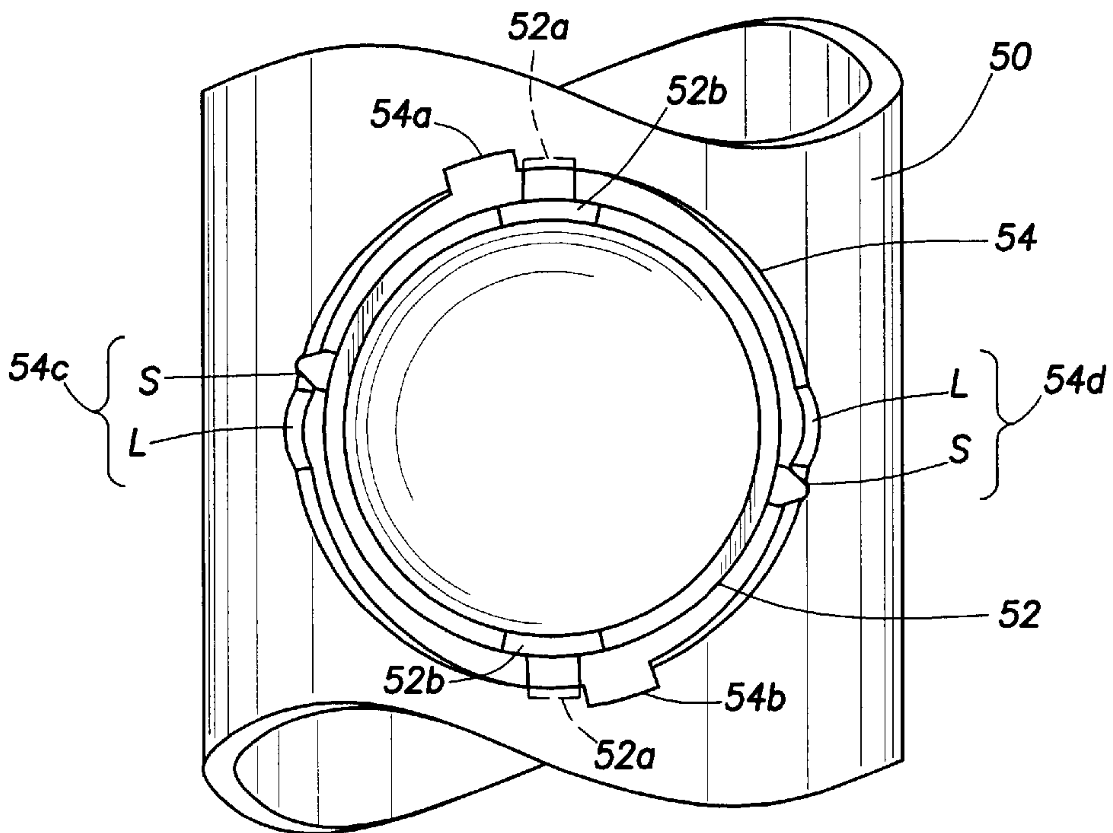
FIG. 7 (PRIOR ART)
