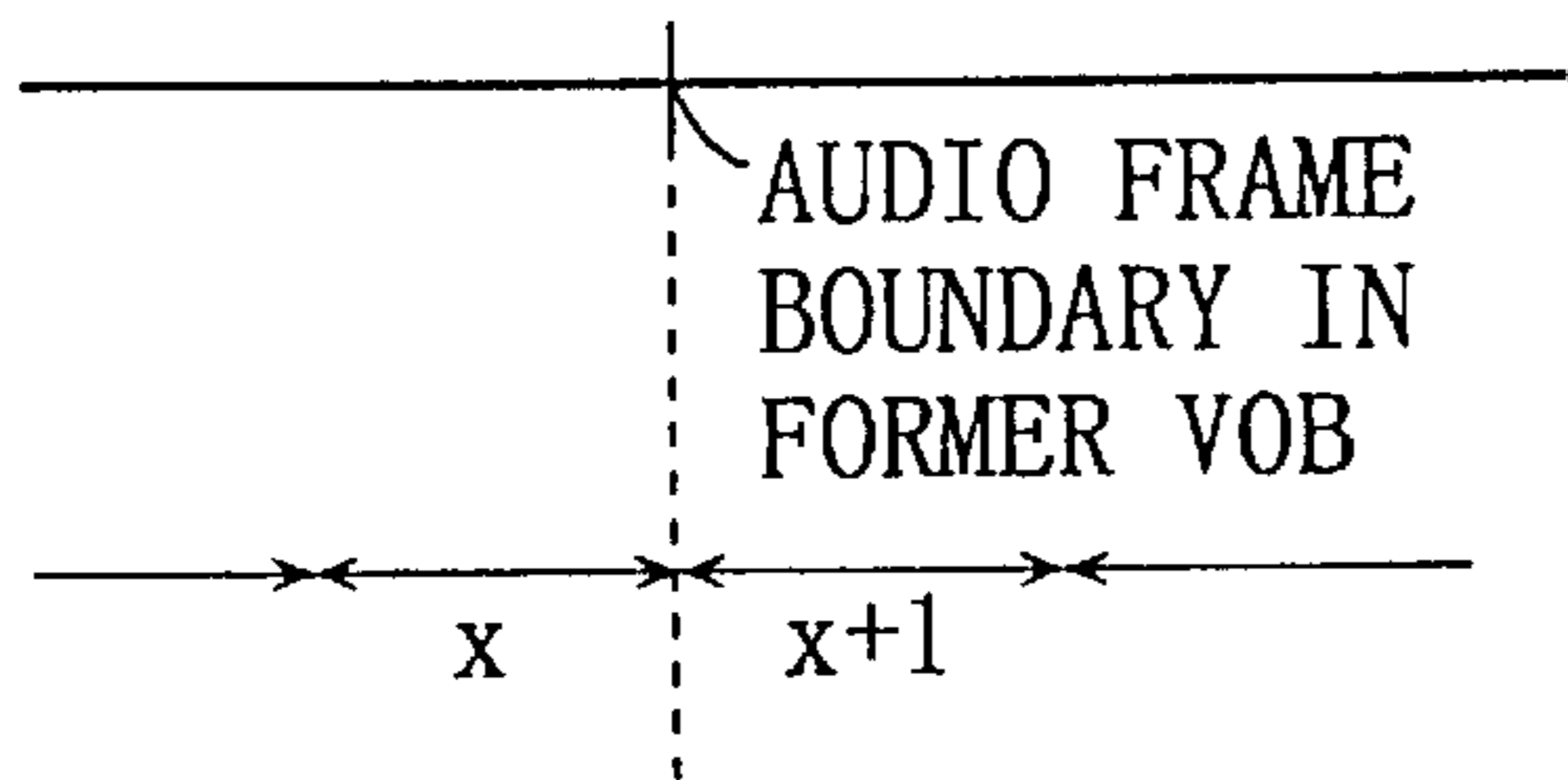
FIG. 24B FIRST_SCR+STC_offset
