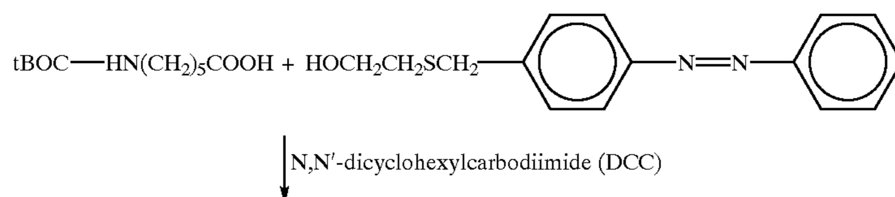
Reaction Scheme 2
