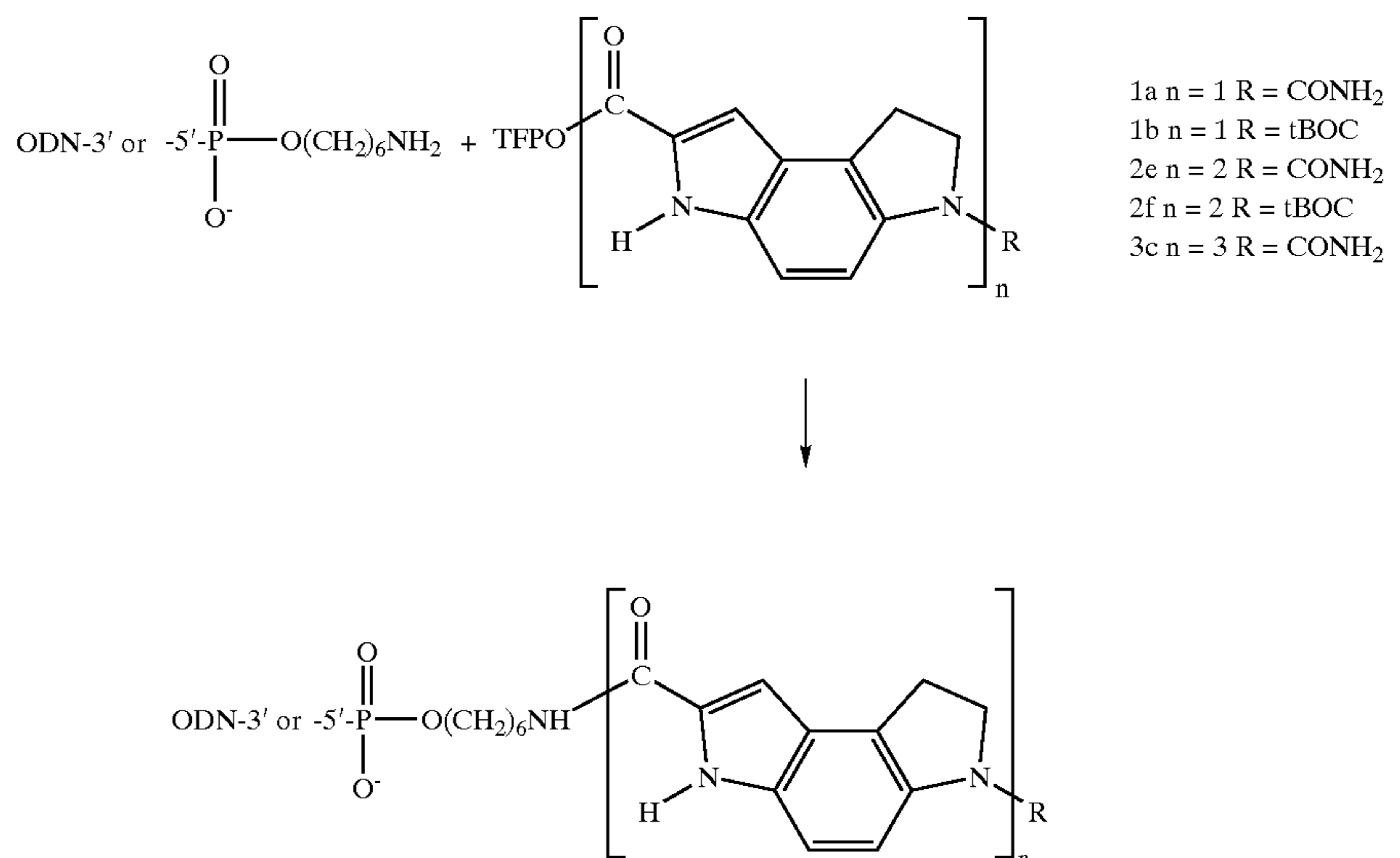
Reaction Scheme 3
