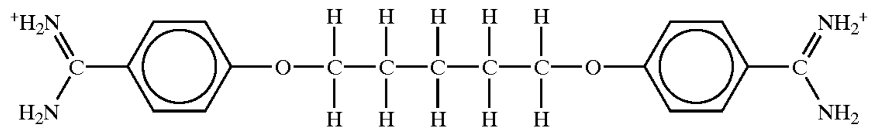
Pentamidine
