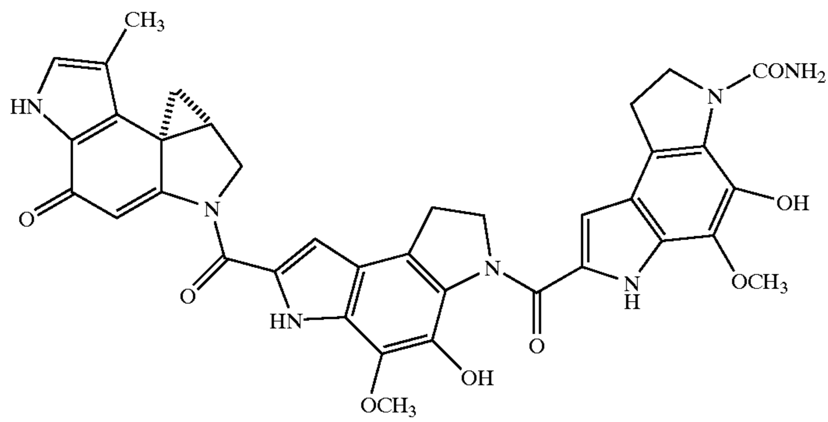
CC-1065
