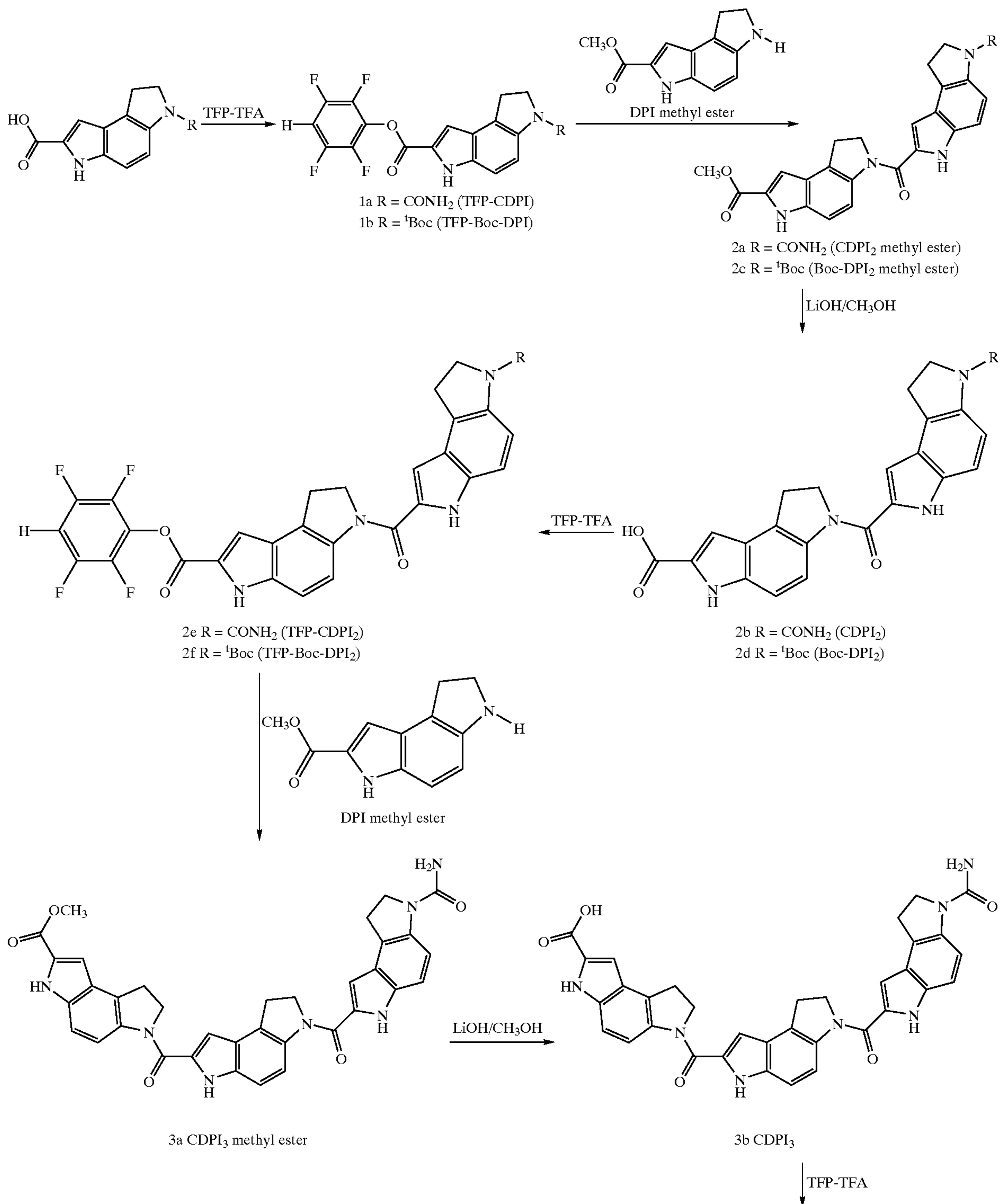
Reaction Scheme 1
