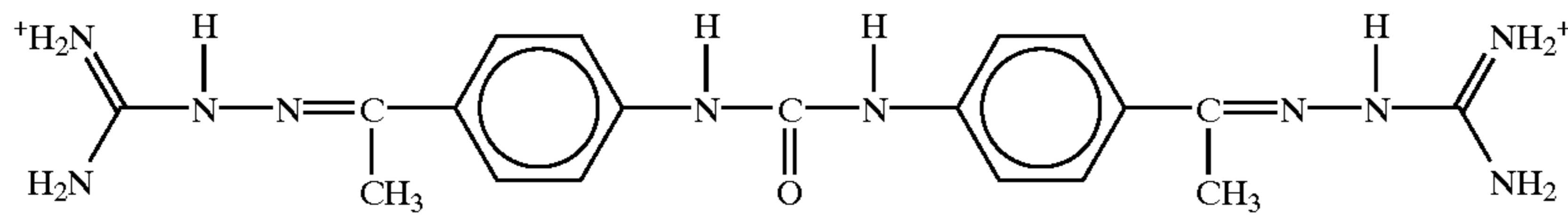
DDUG
