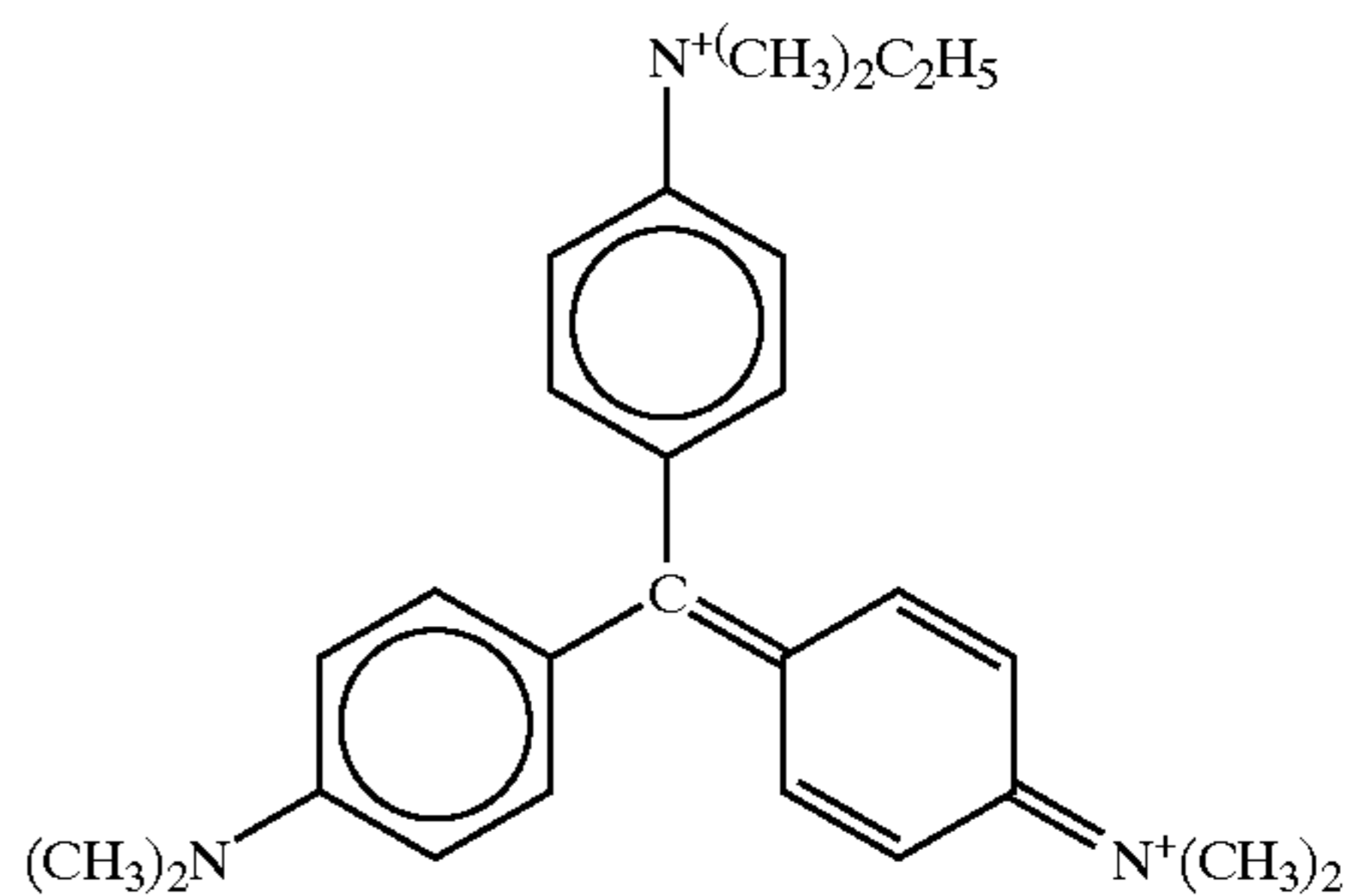
Methyl Green
