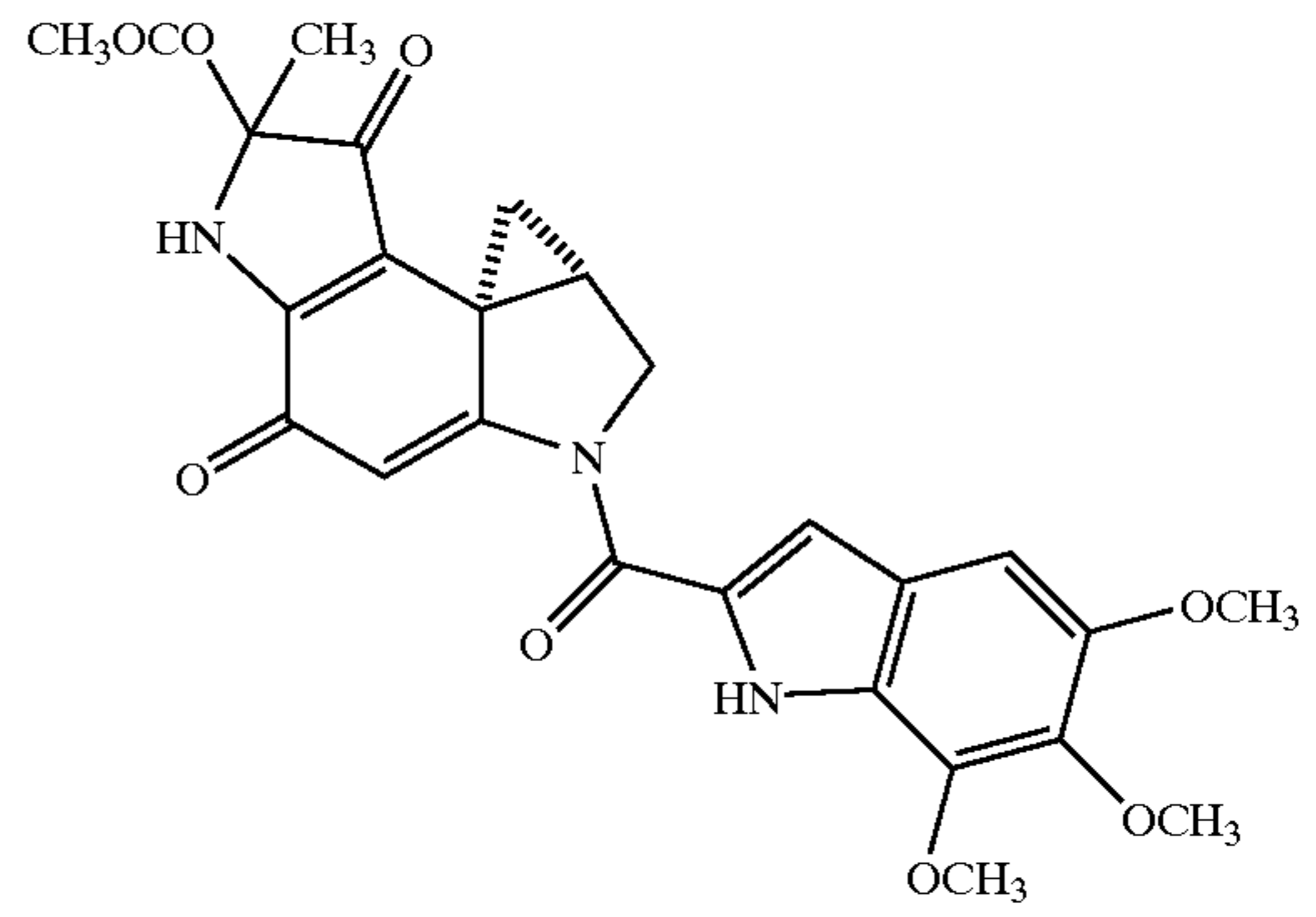
Duocarmycin A
