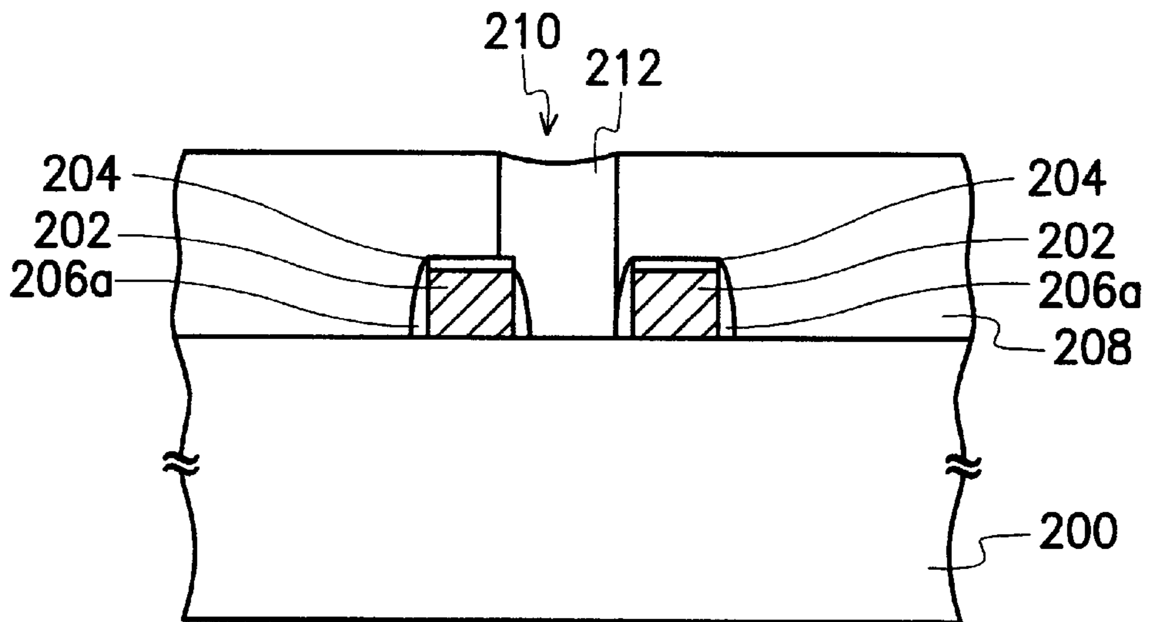
FIG. 2C (PRIOR ART)
