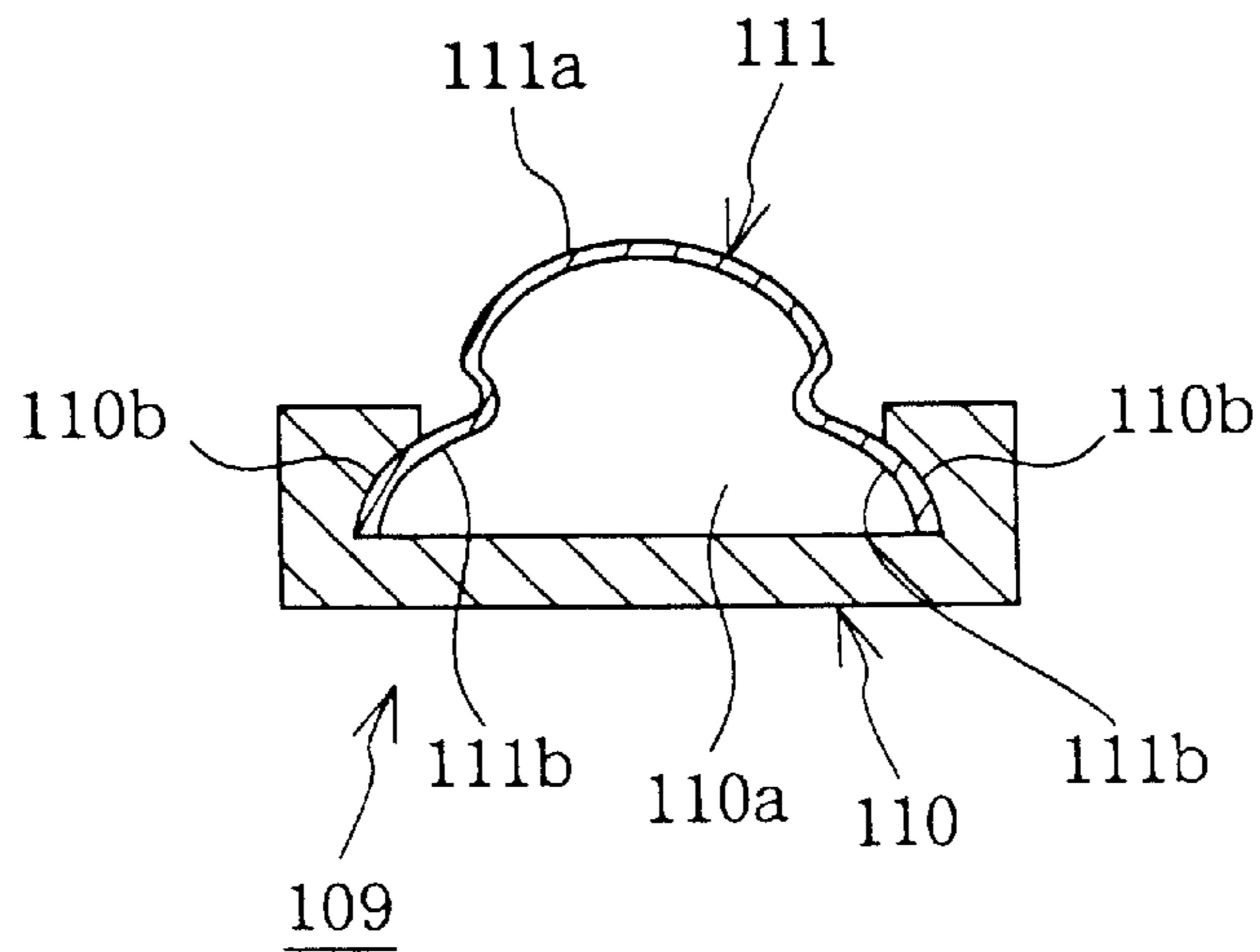
FIG.23 (PRIOR ART)
