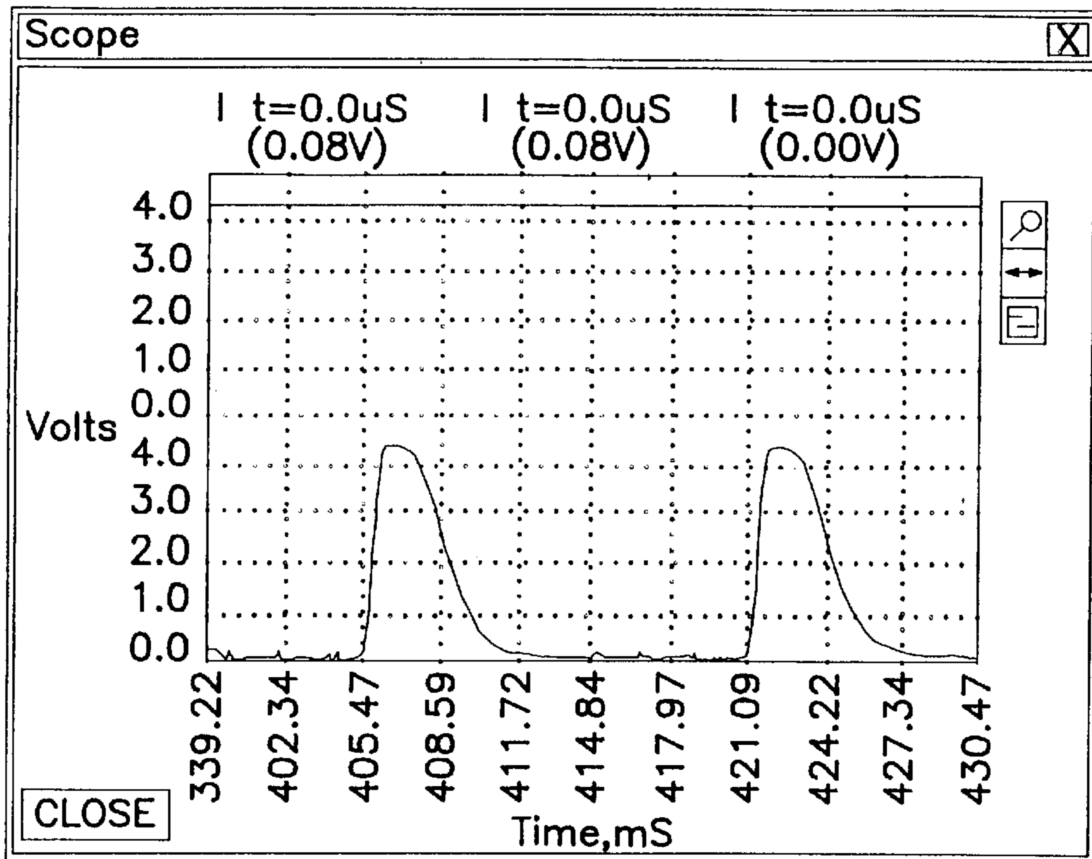
CRT photoresponse
