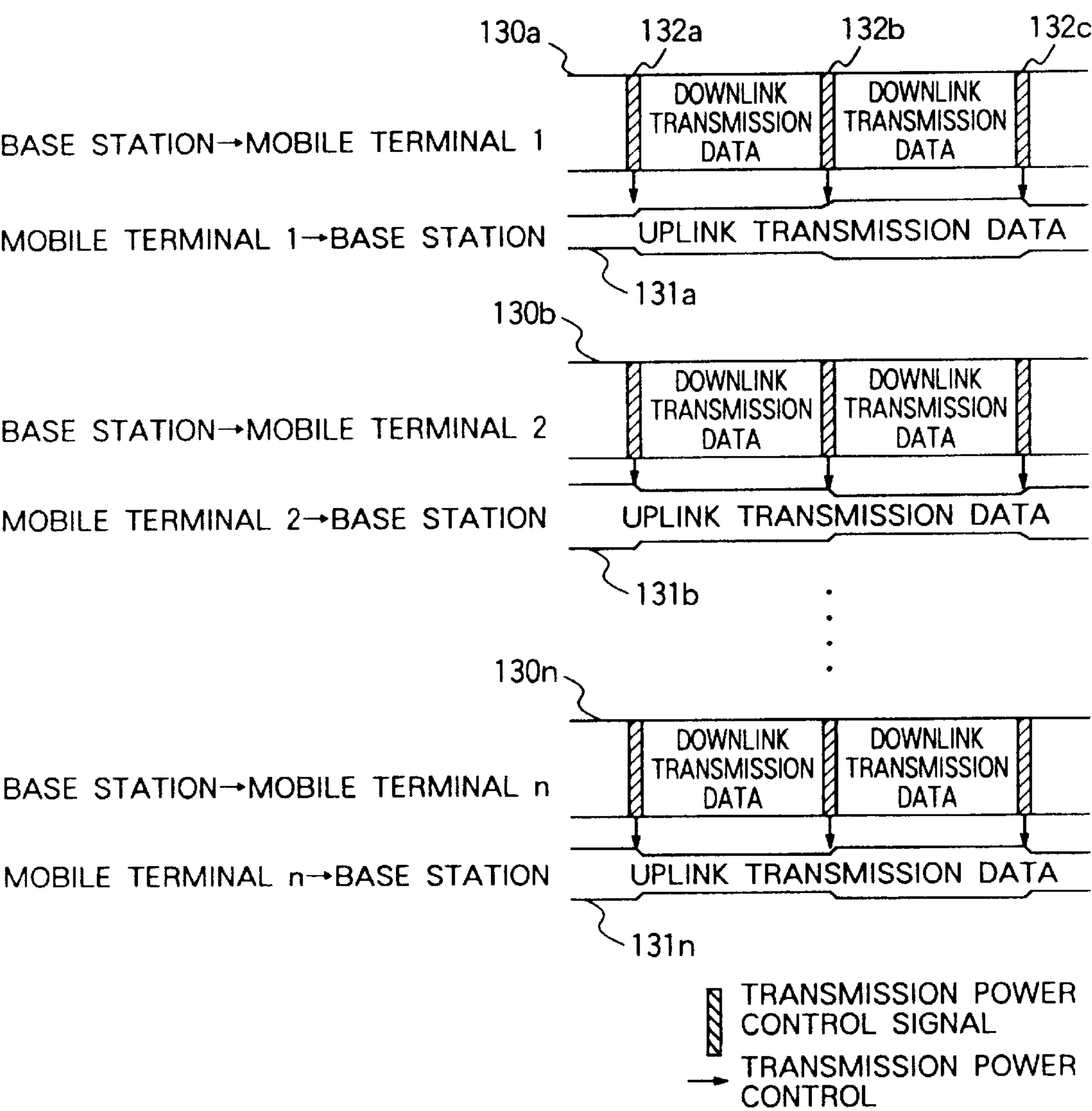
FIG. 12 PRIOR ART
