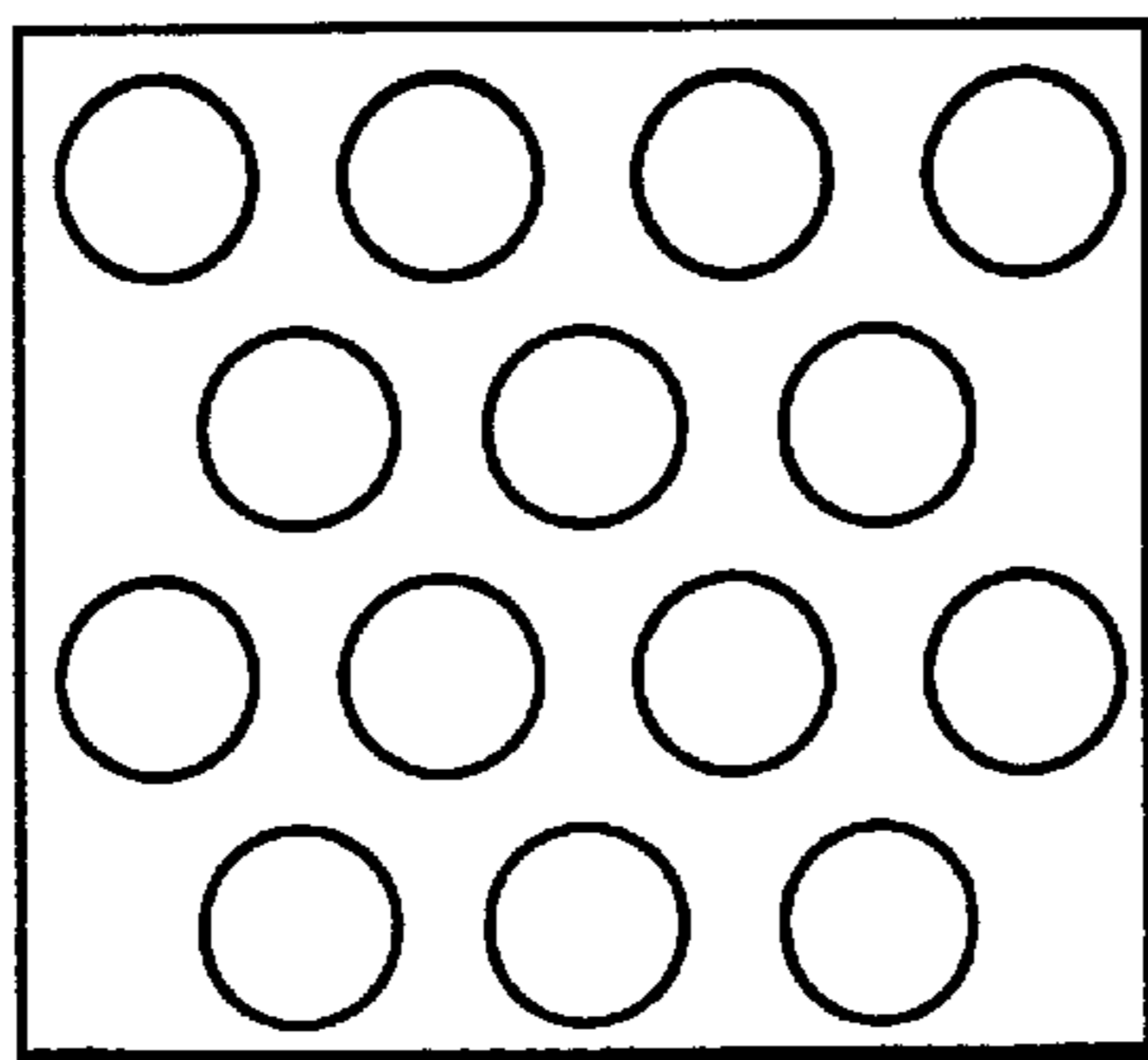
TRIANGULAR LATTICE
