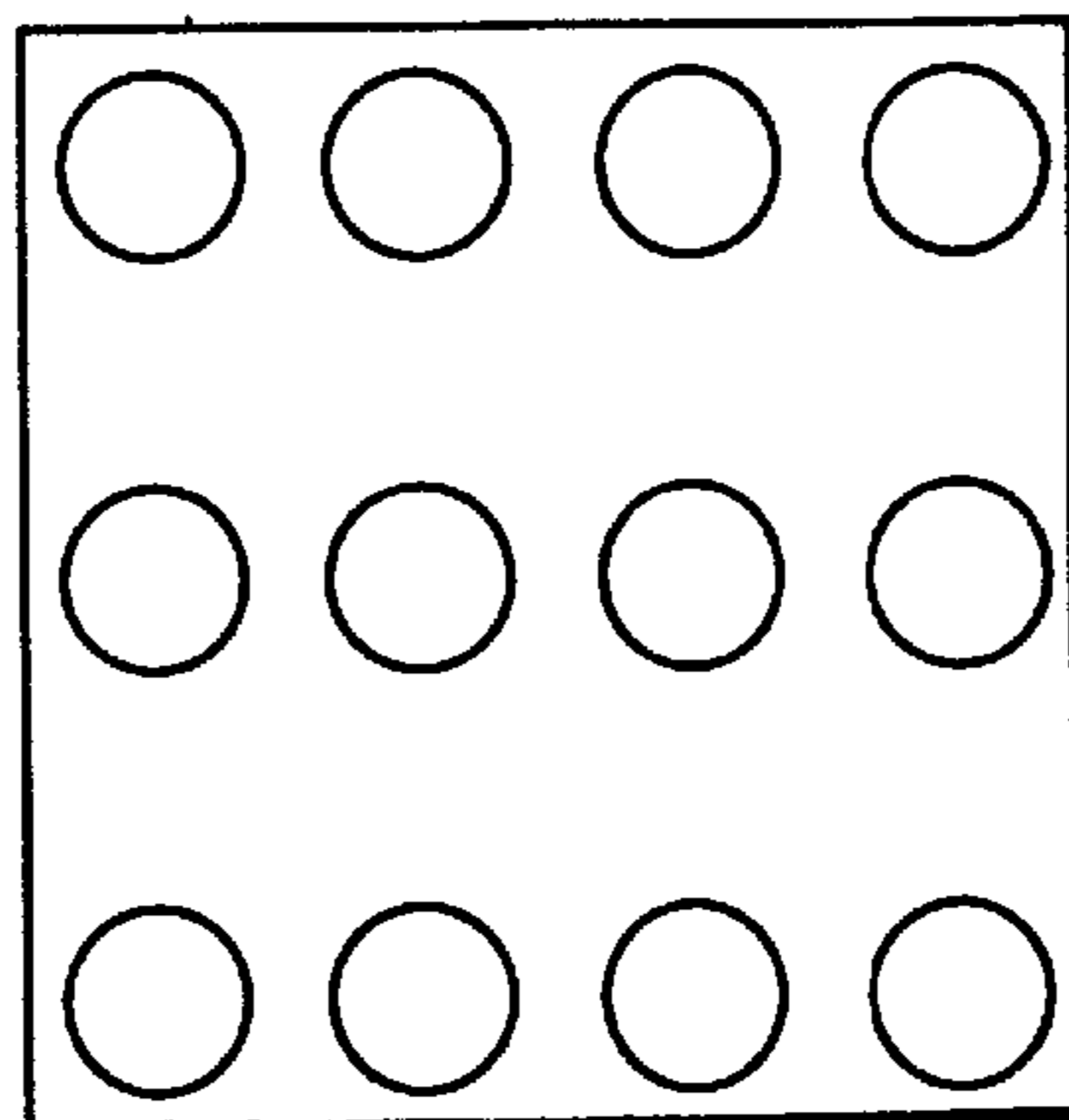
RECTANGULAR LATTICE
