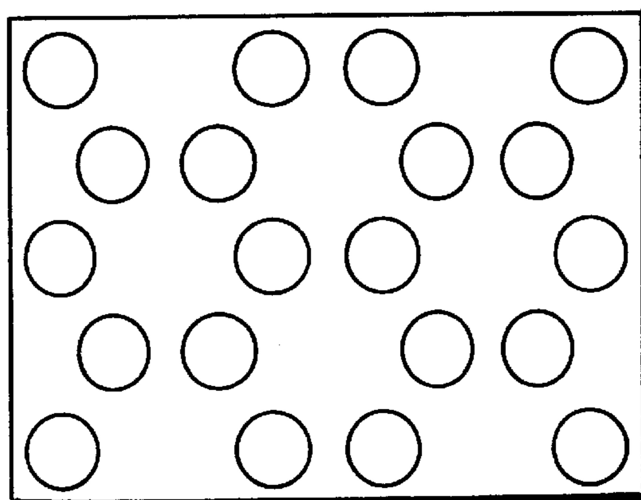
GRAPHITE LATTICE
