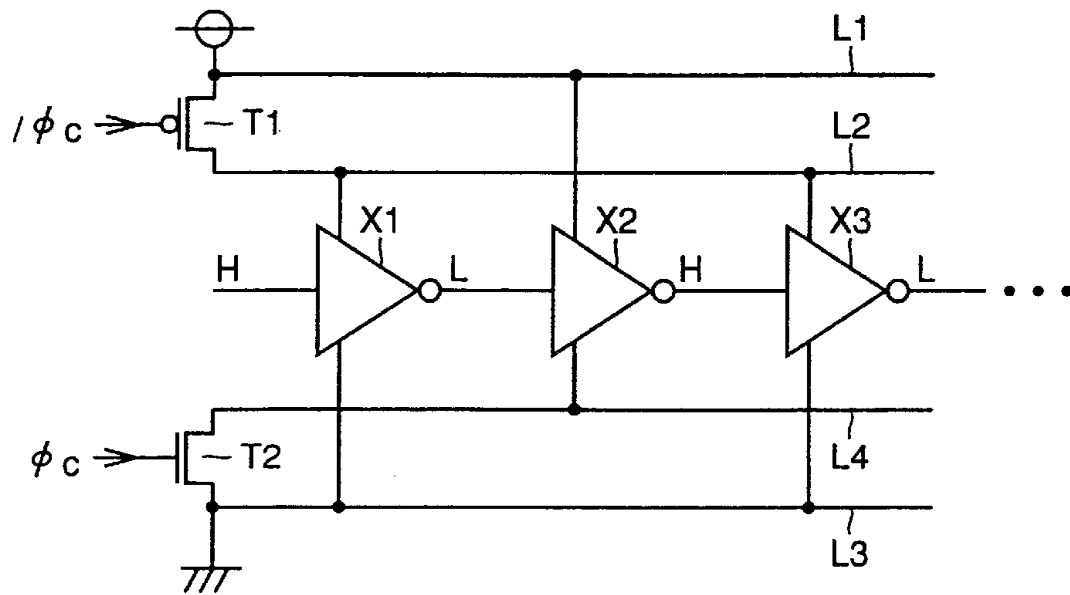
FIG.67 PRIOR ART
