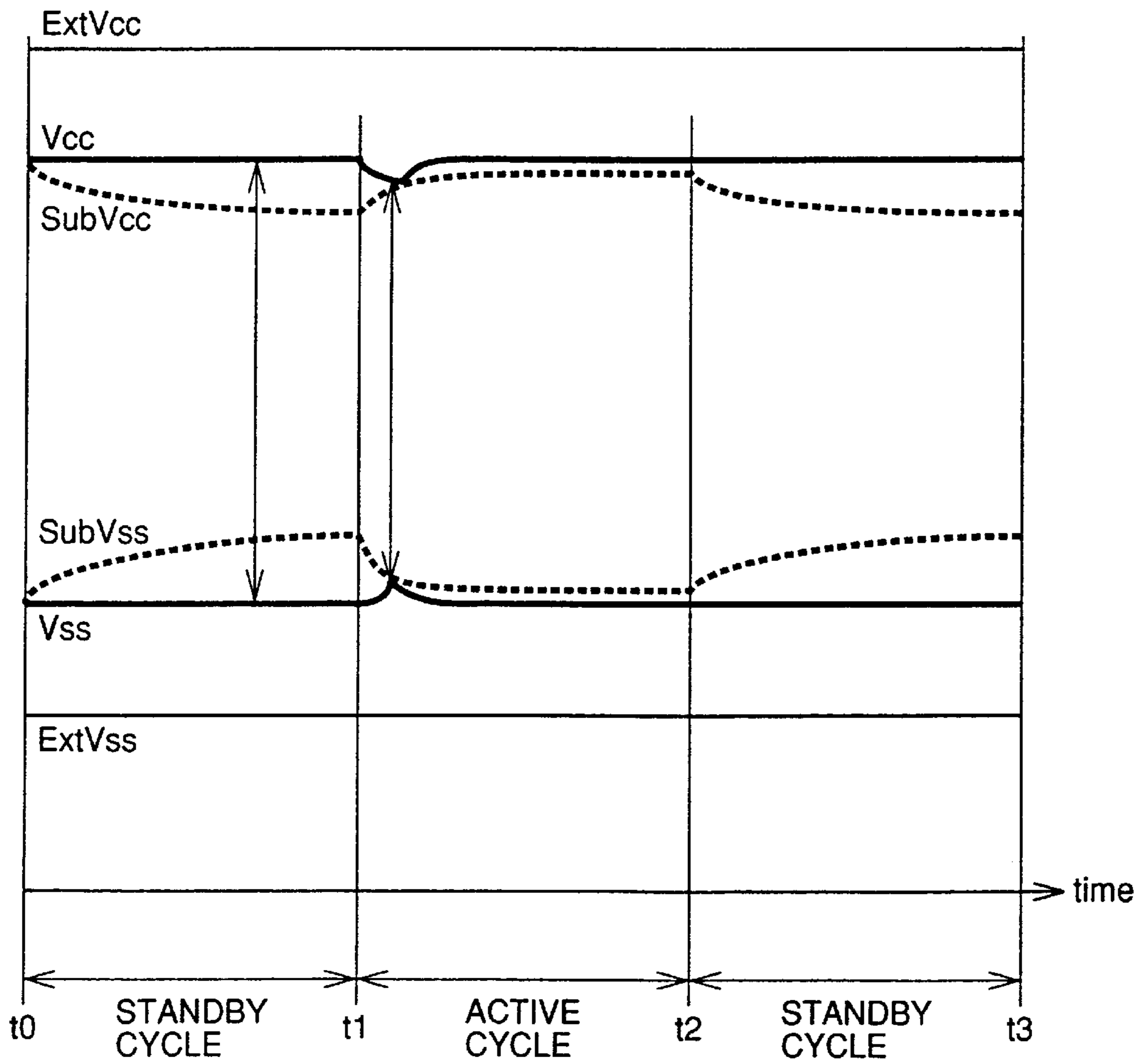
FIG.68 PRIOR ART
