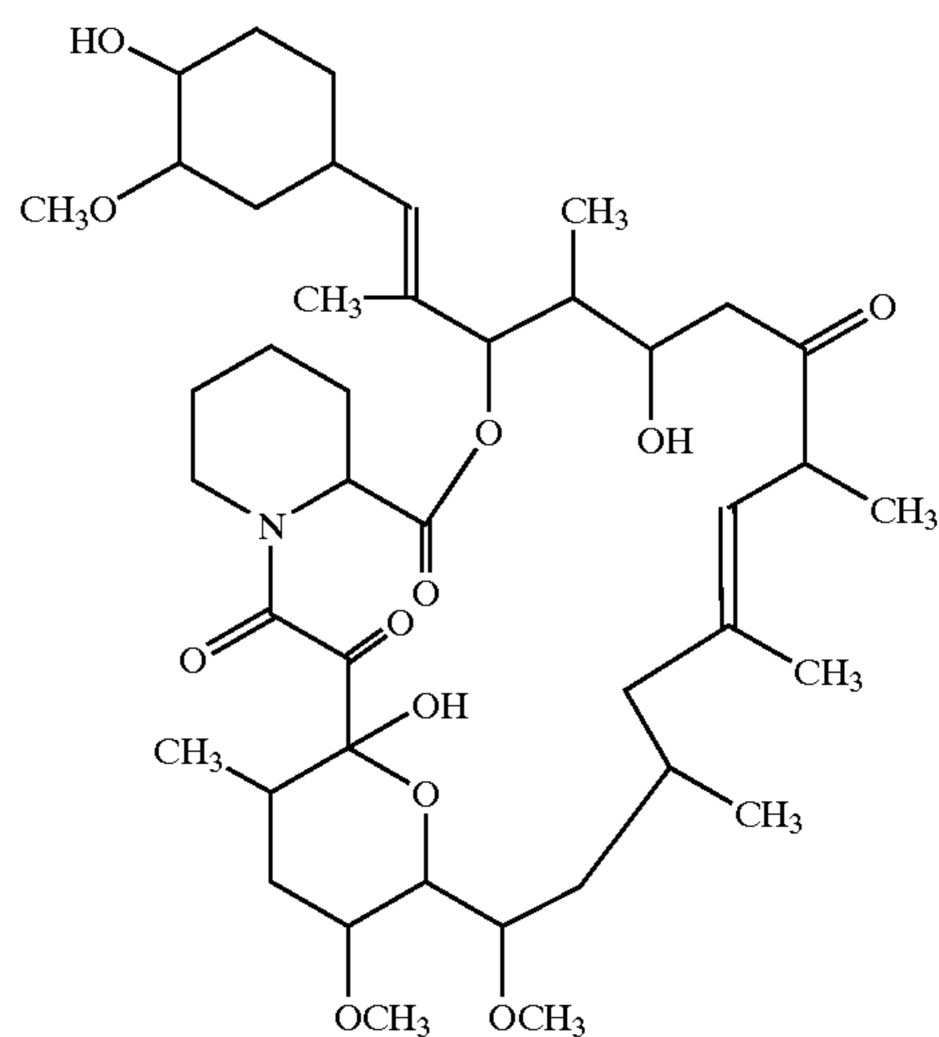
1,14-Dihydroxy-12-[2-(4-hydroxy-3-methoxycyclohexyl)-1-methylvinyl]-23,25-dimethoxy-13,19,17,21,27-pentamethyl-11,28-dioxo-4-azatricyclo[22.3.1.0 4,9 ]-octacos-18-ene-2,3,10,16-tetraone
