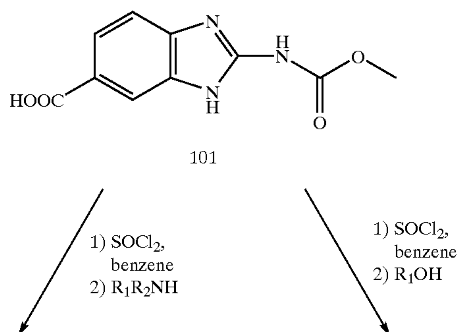
Reaction Scheme 1
