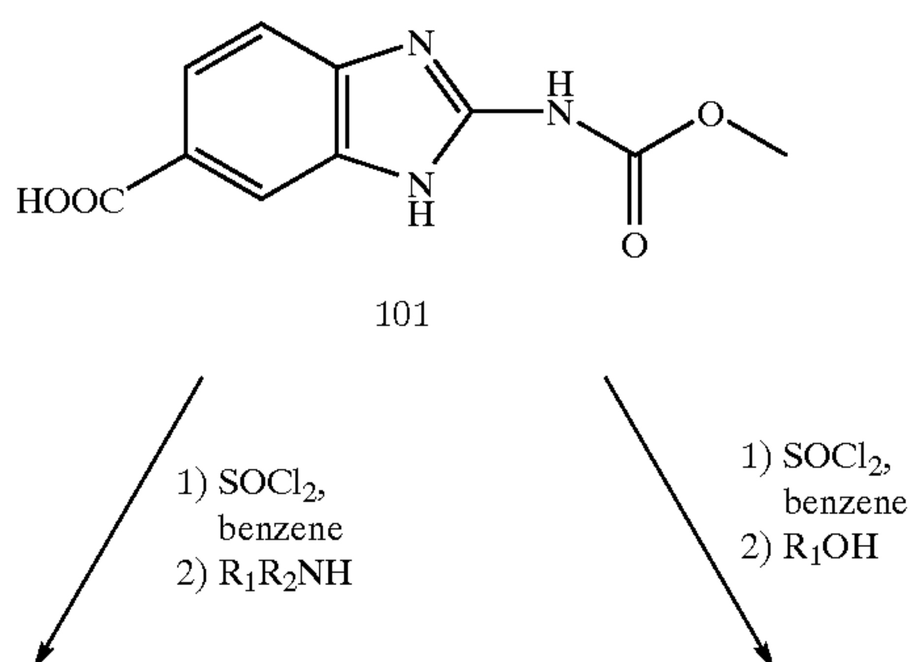
Reaction Scheme 1
