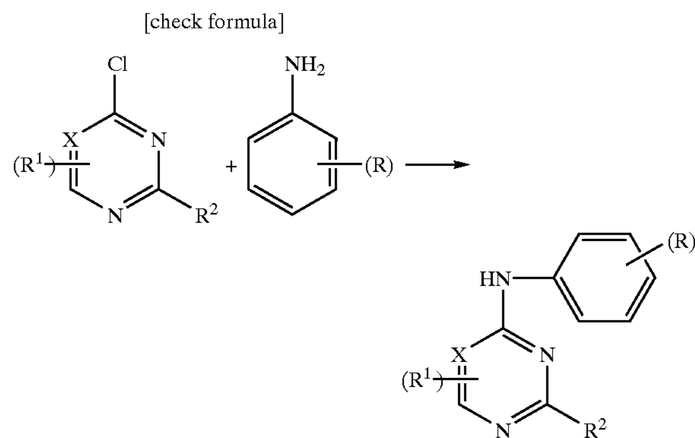
Scheme 1
