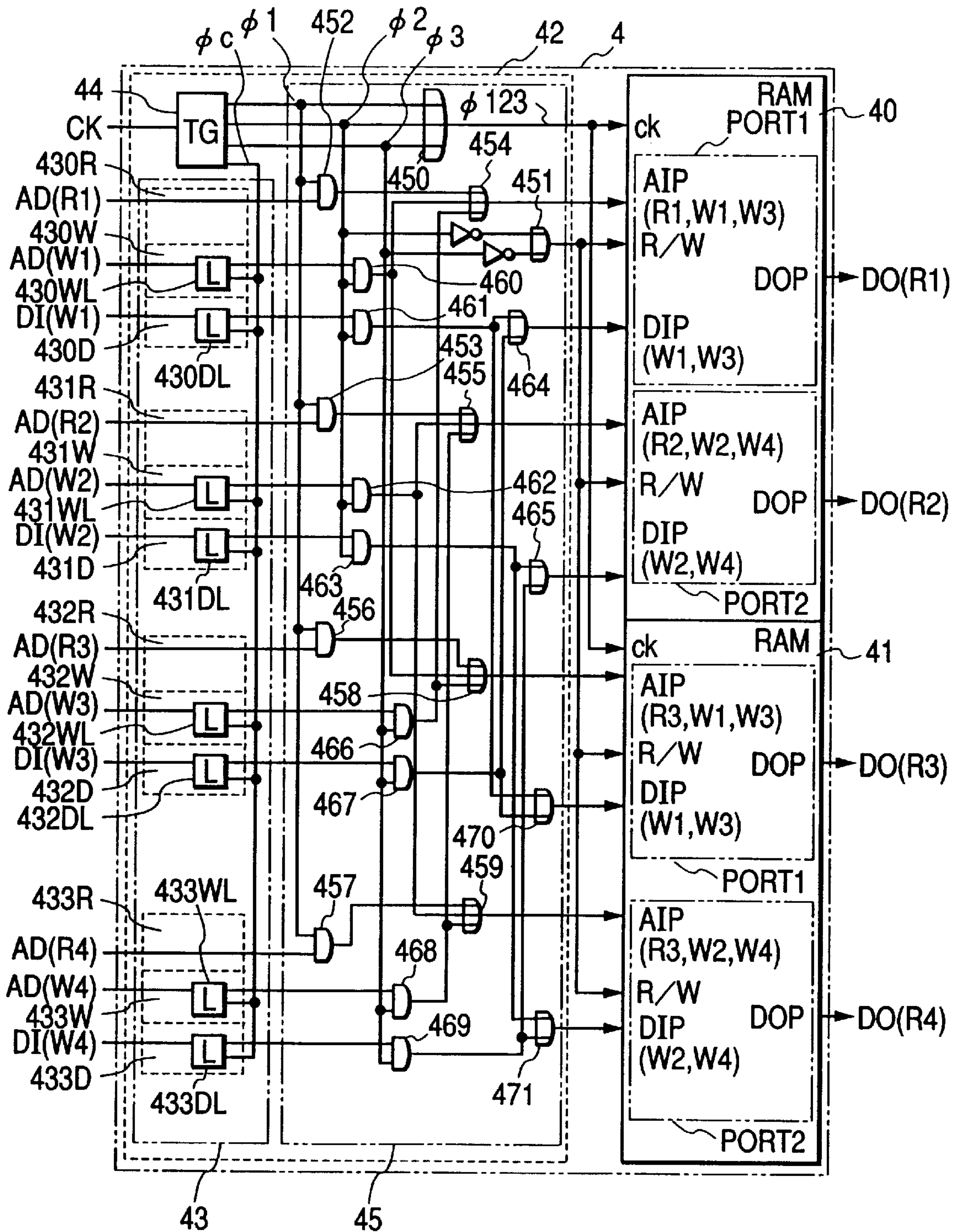
8 PORT RAM (USING TWO 2-PORT RAMS)
