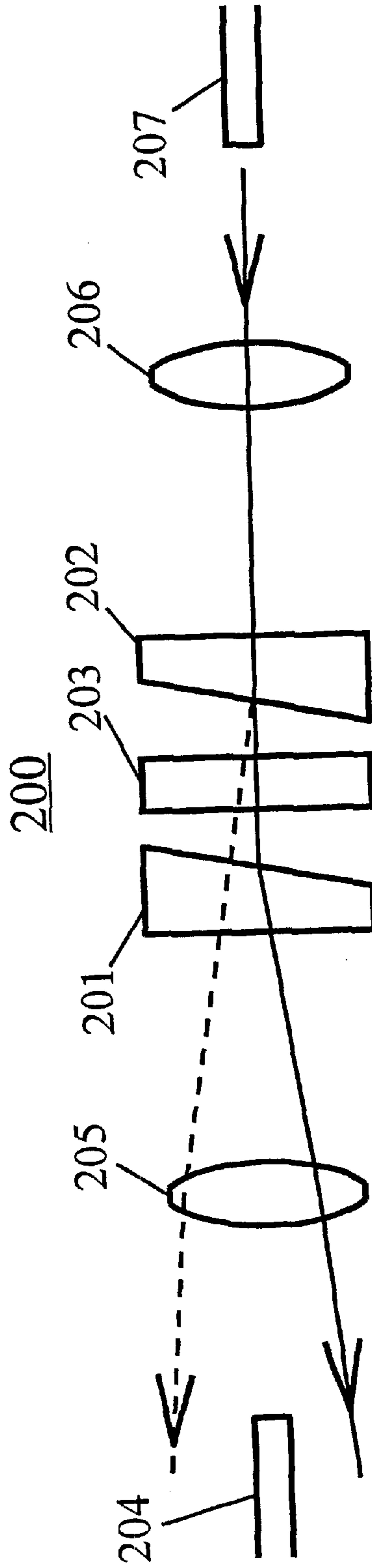
Figure 2B PRIOR ART
