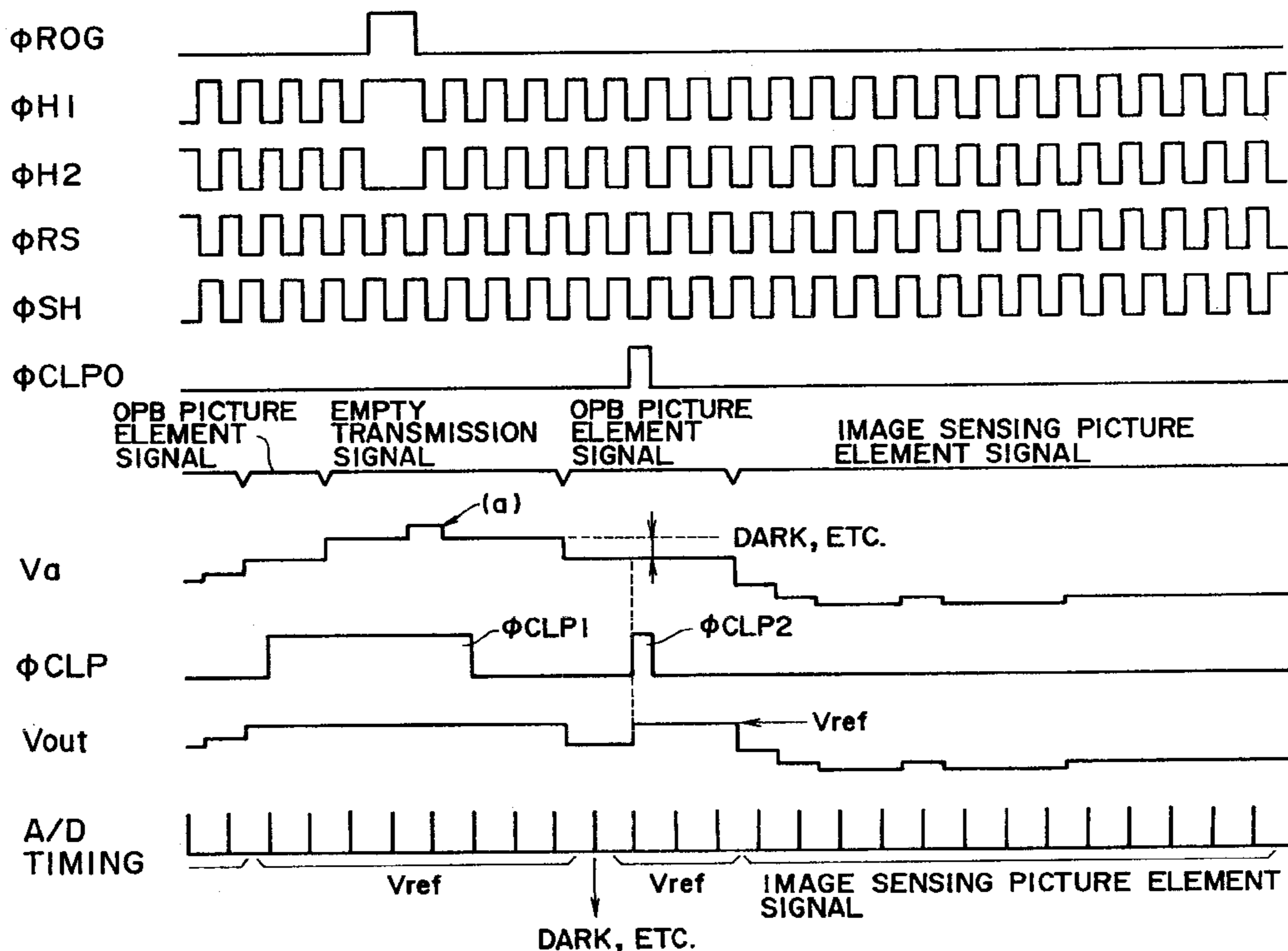
TIMING CHARTS FOR EXPLAINING THE OPERATIONS OF A SECOND EMBODIMENT
