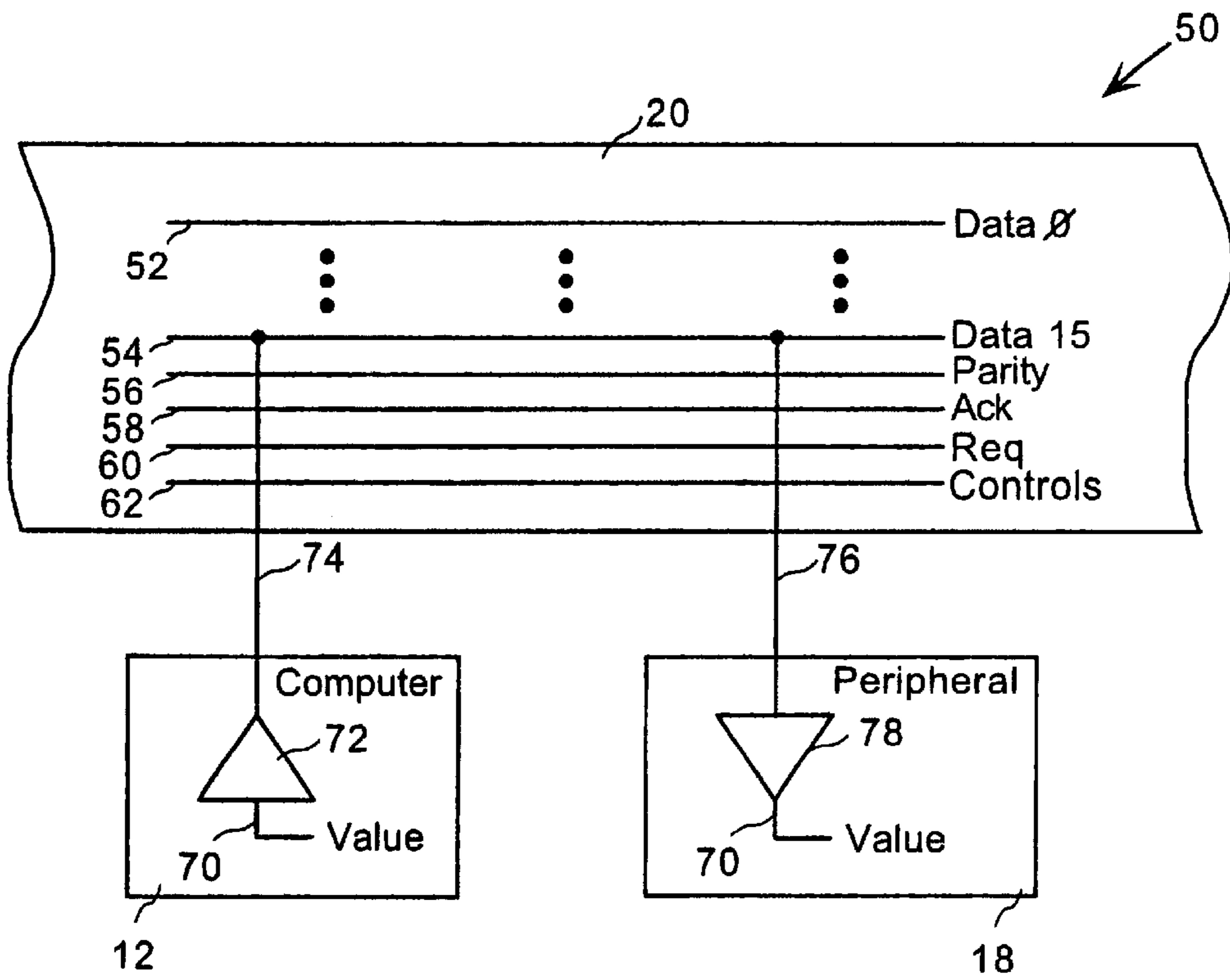
FIG. 2 (prior art)
