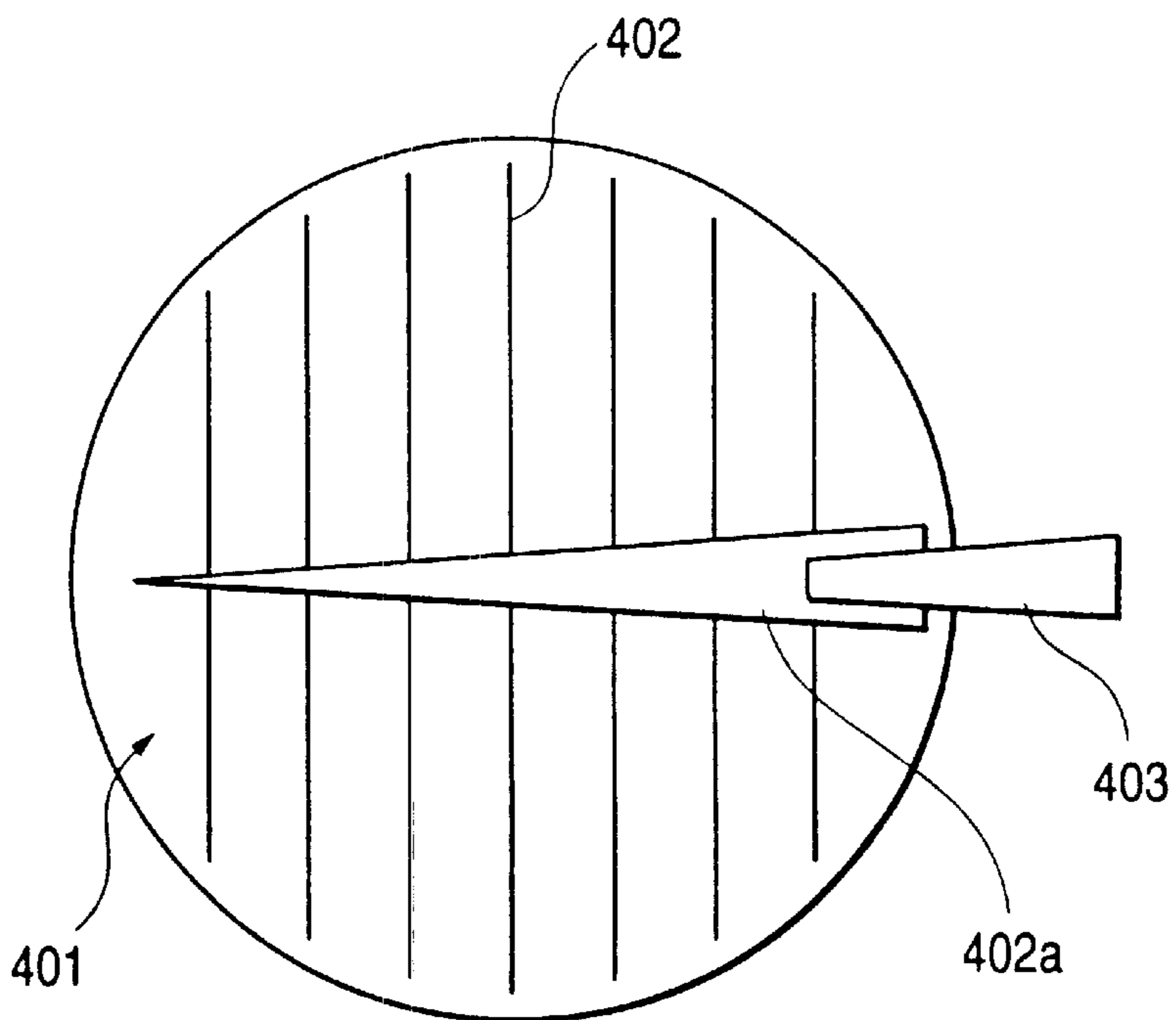
FIG. 3 PRIOR ART
