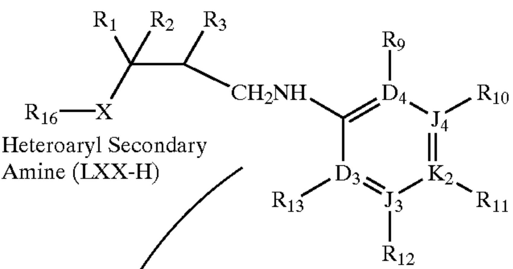
Scheme 54
