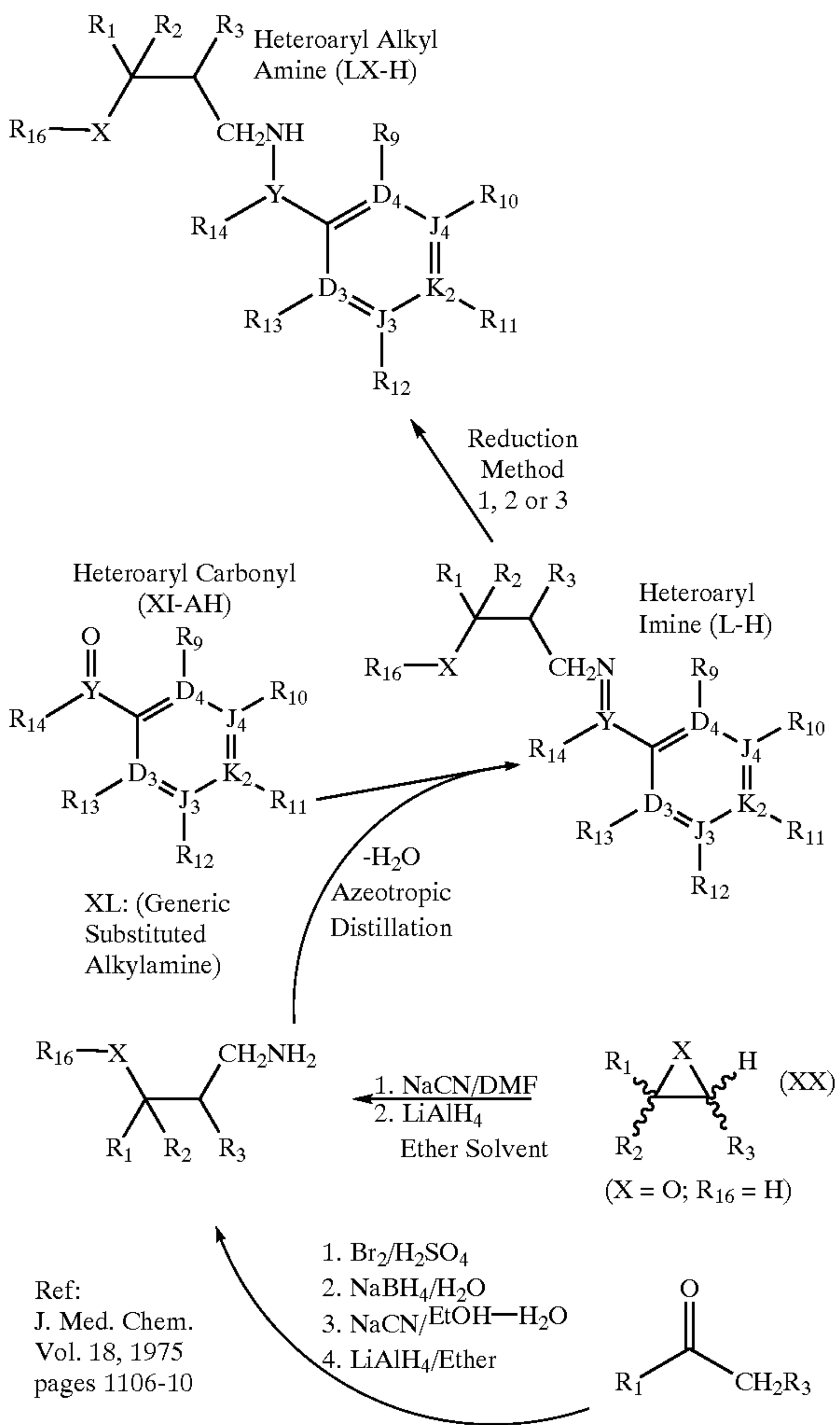
Scheme 30
