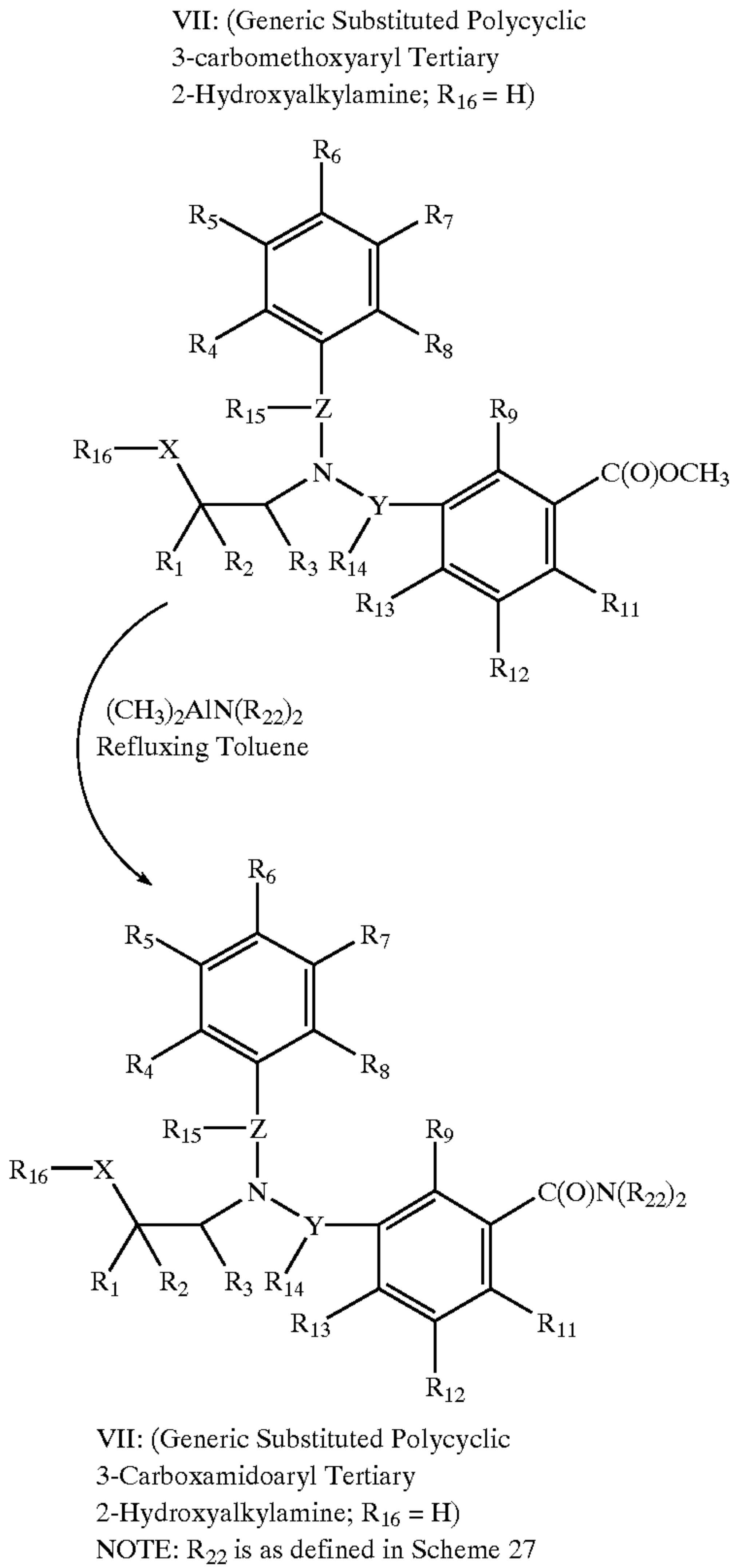
Scheme 36
