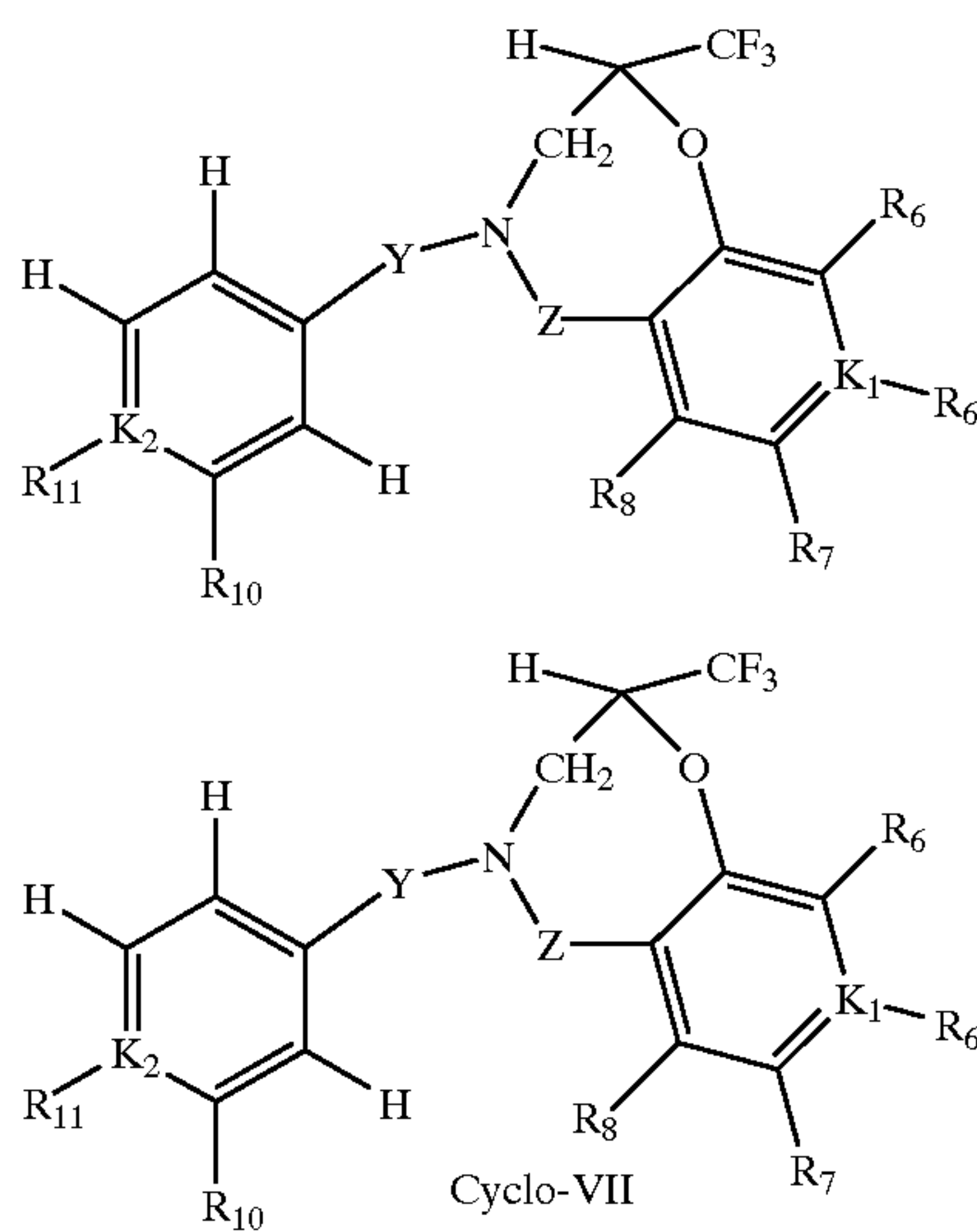
Structure of Substituted Tricyclictertiary-2-oxyalkylamines
