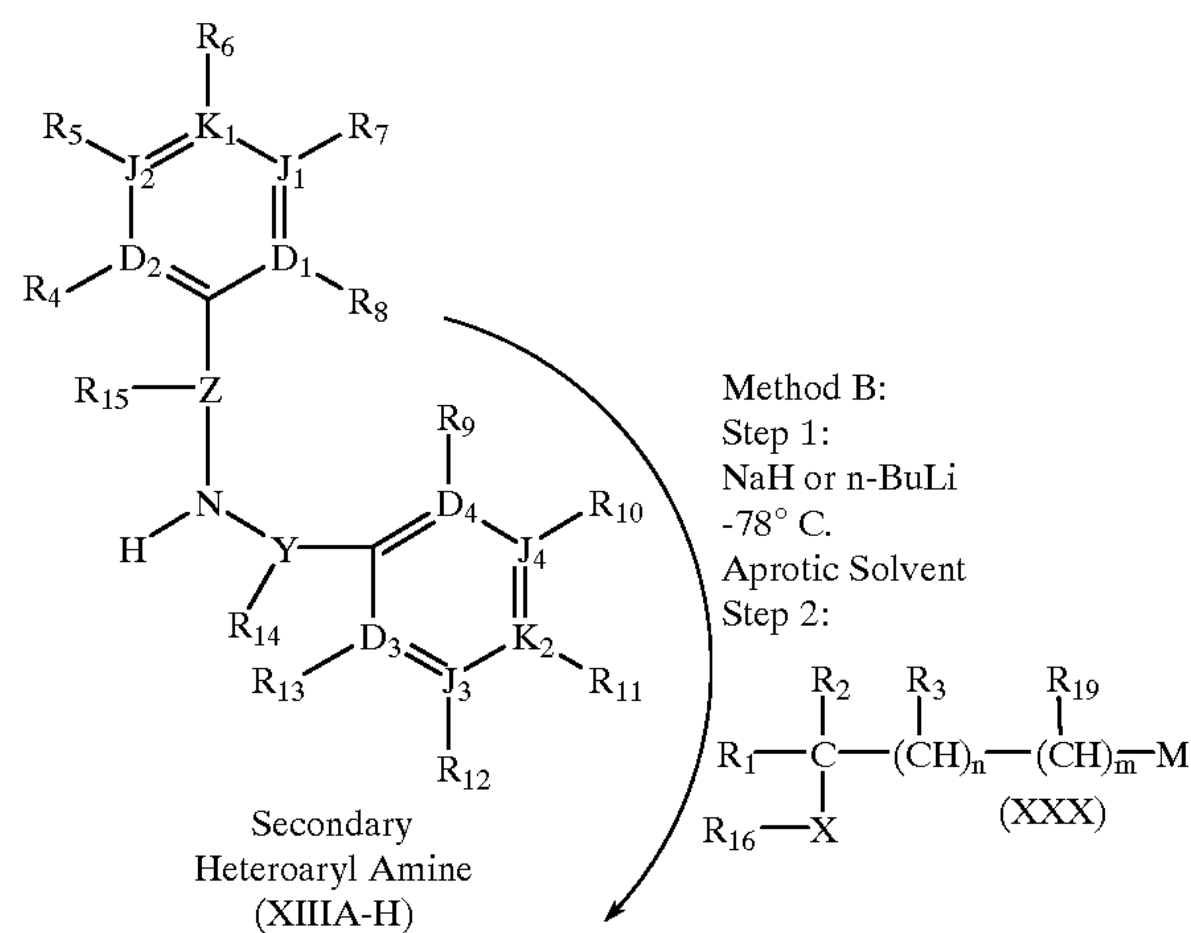
Scheme 6
