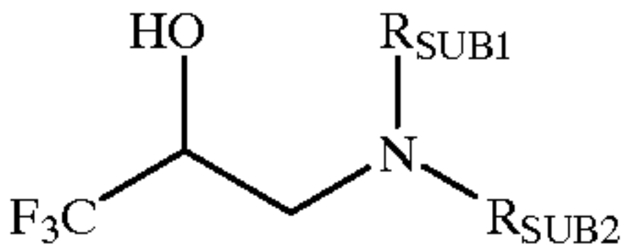
Example Table 47. 3-[N-(aryl)-[(aryl)methyl]amino]-1,1,1-trifluoro-2-propanols.
