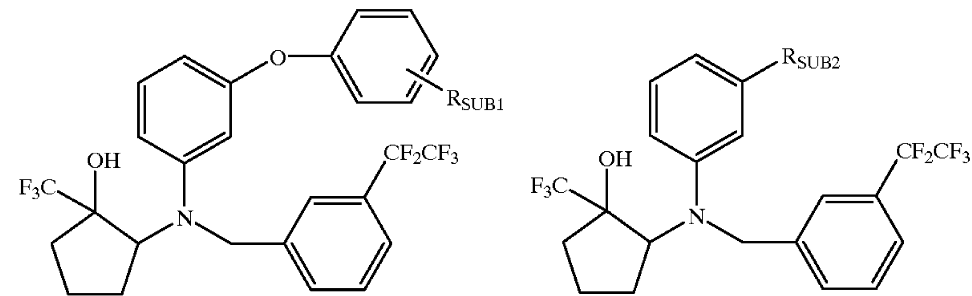
Example Table 54. Substituted 2-[N-(aryl)-[(aryl)methyl]amino]-1-trifluoromethylcyclopentanols.
