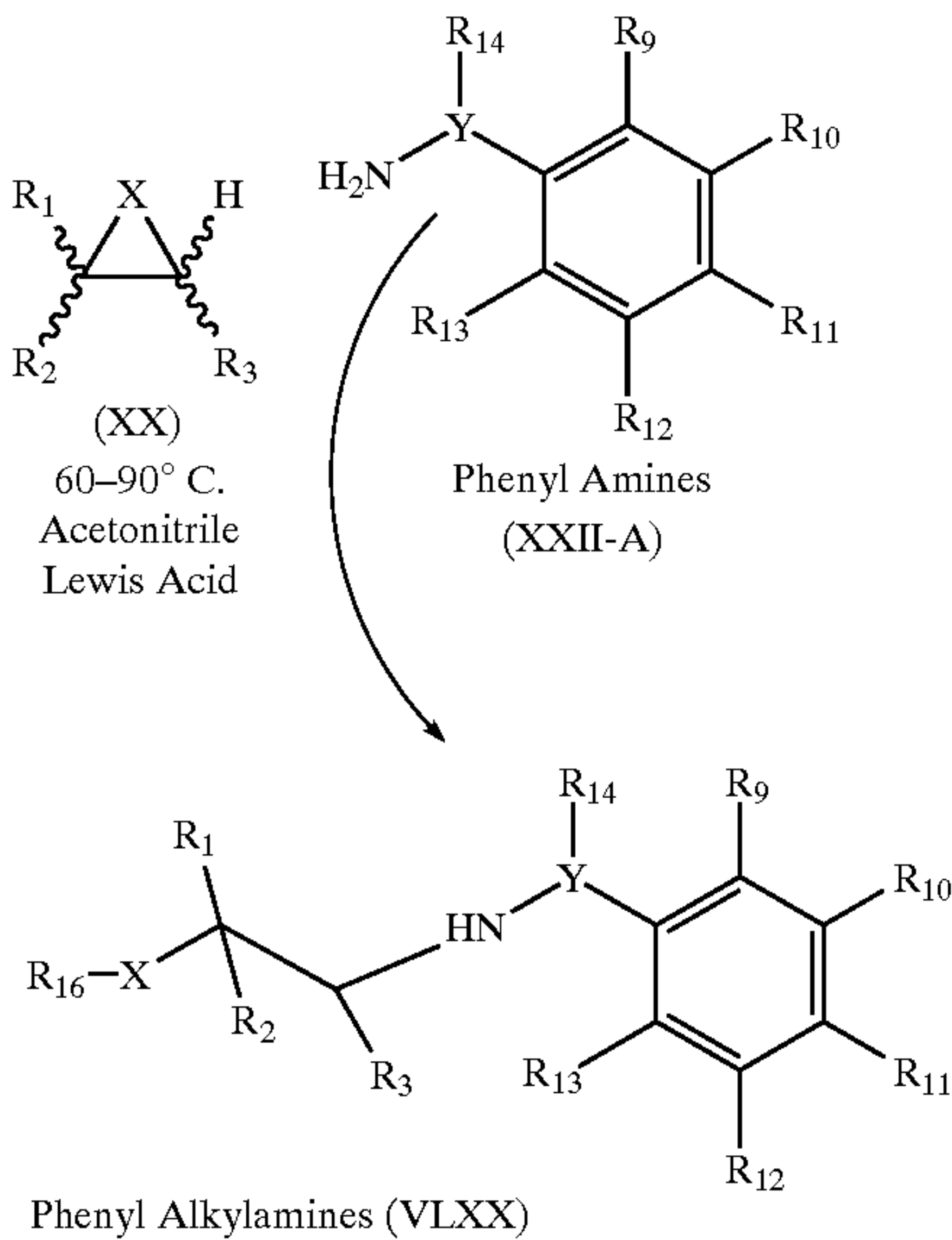
Scheme 58
