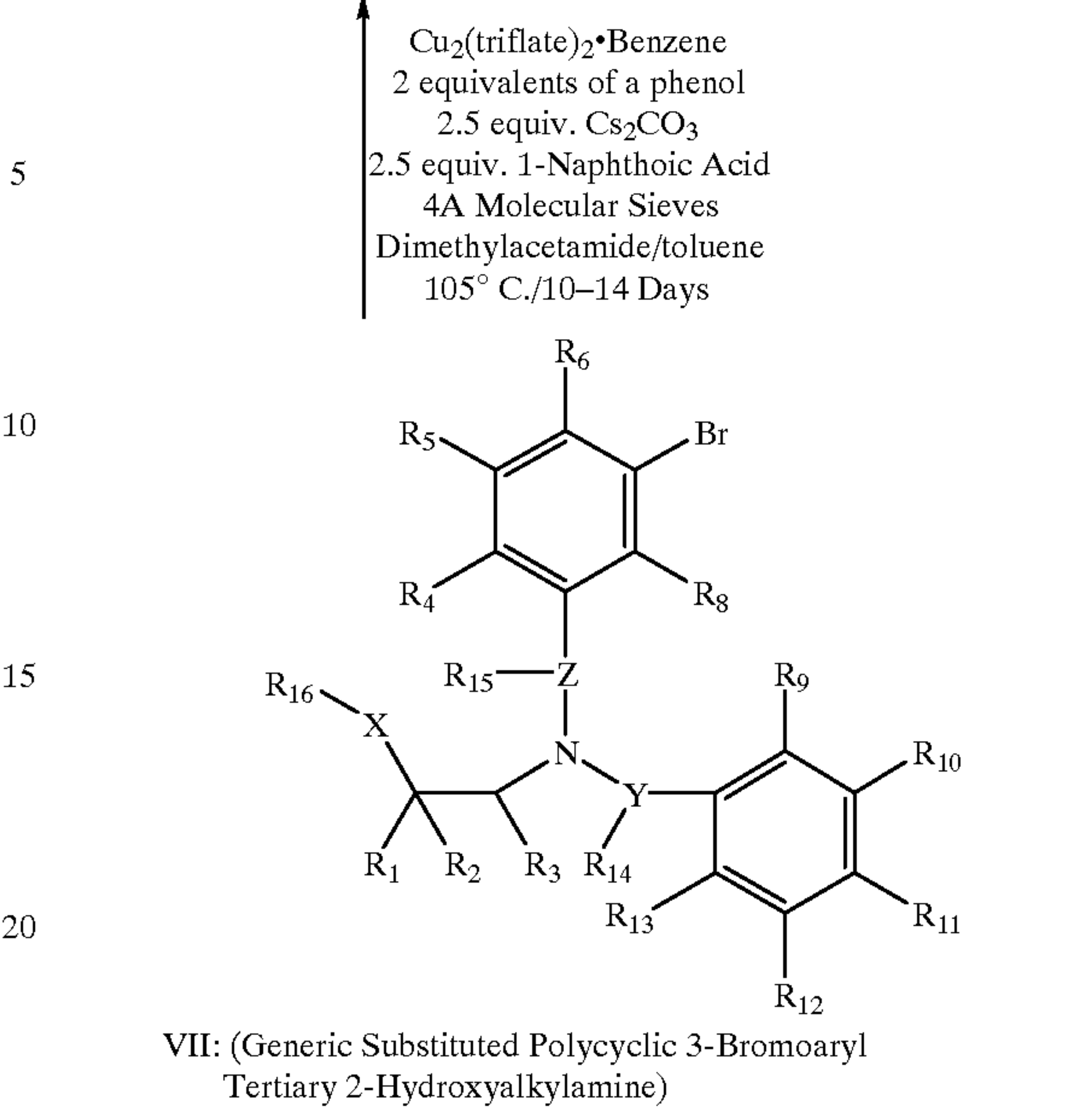
Scheme 9
