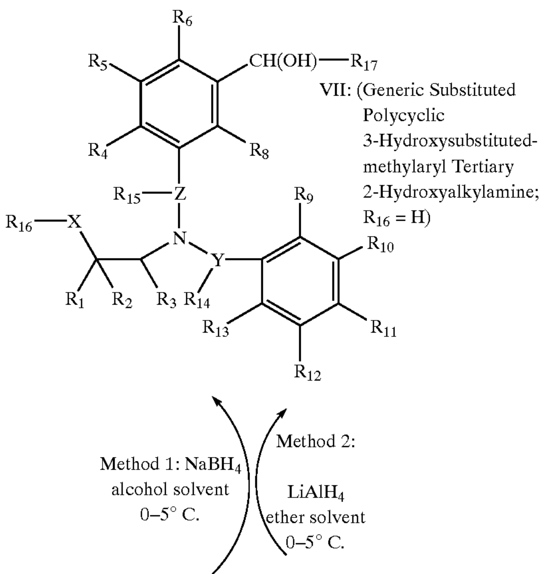
Scheme 29
