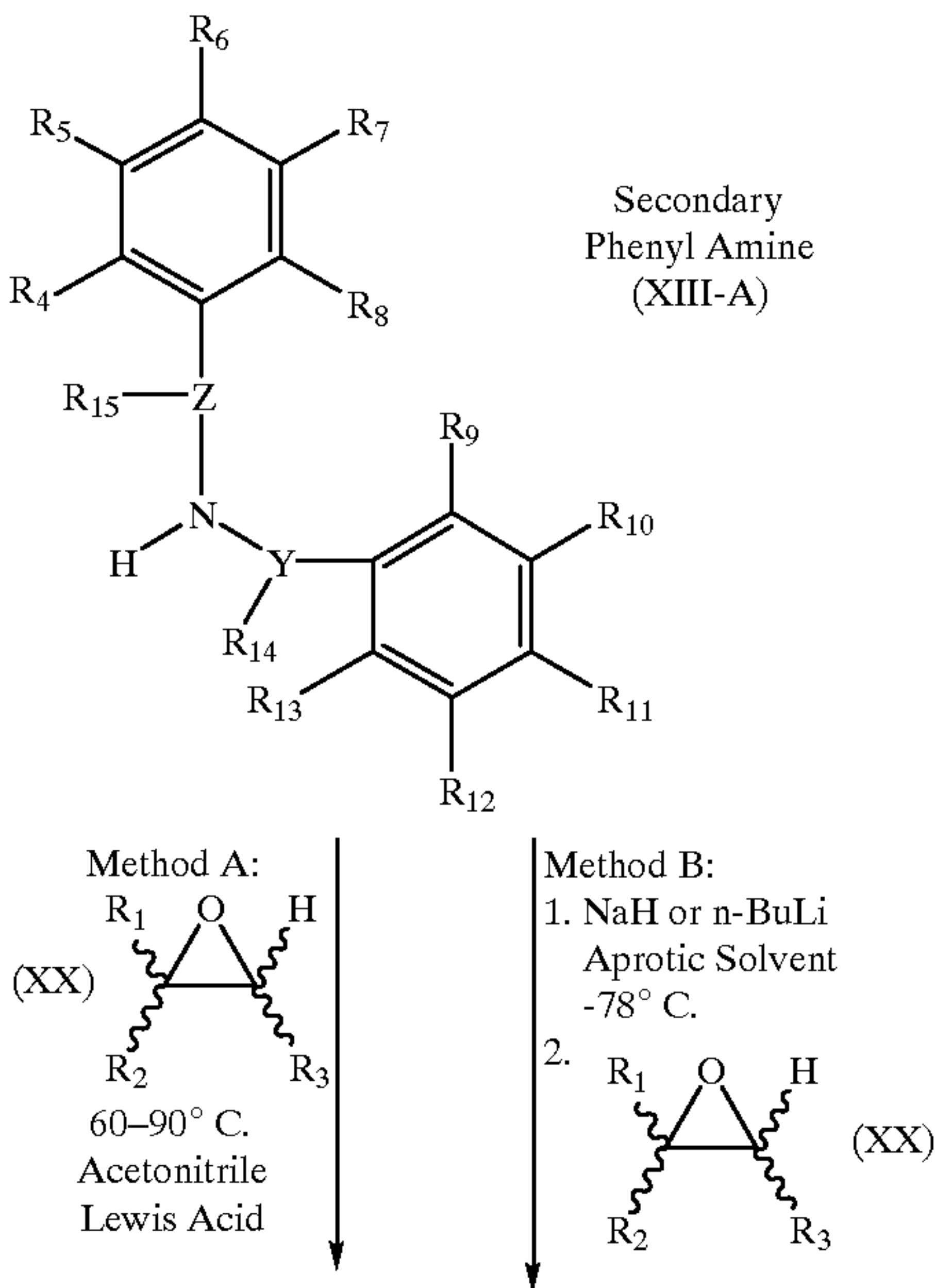
Scheme 11
