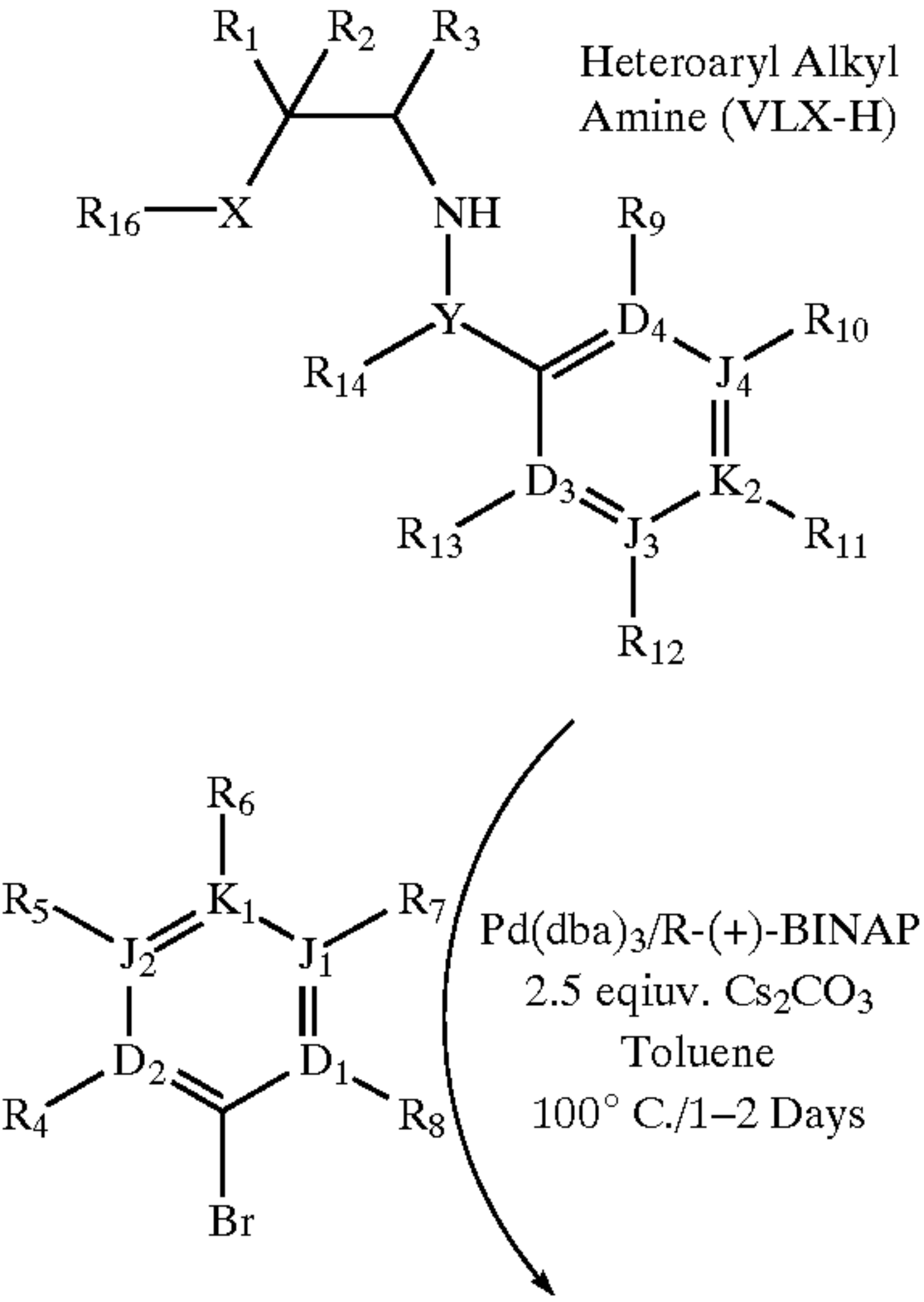
Scheme 47
