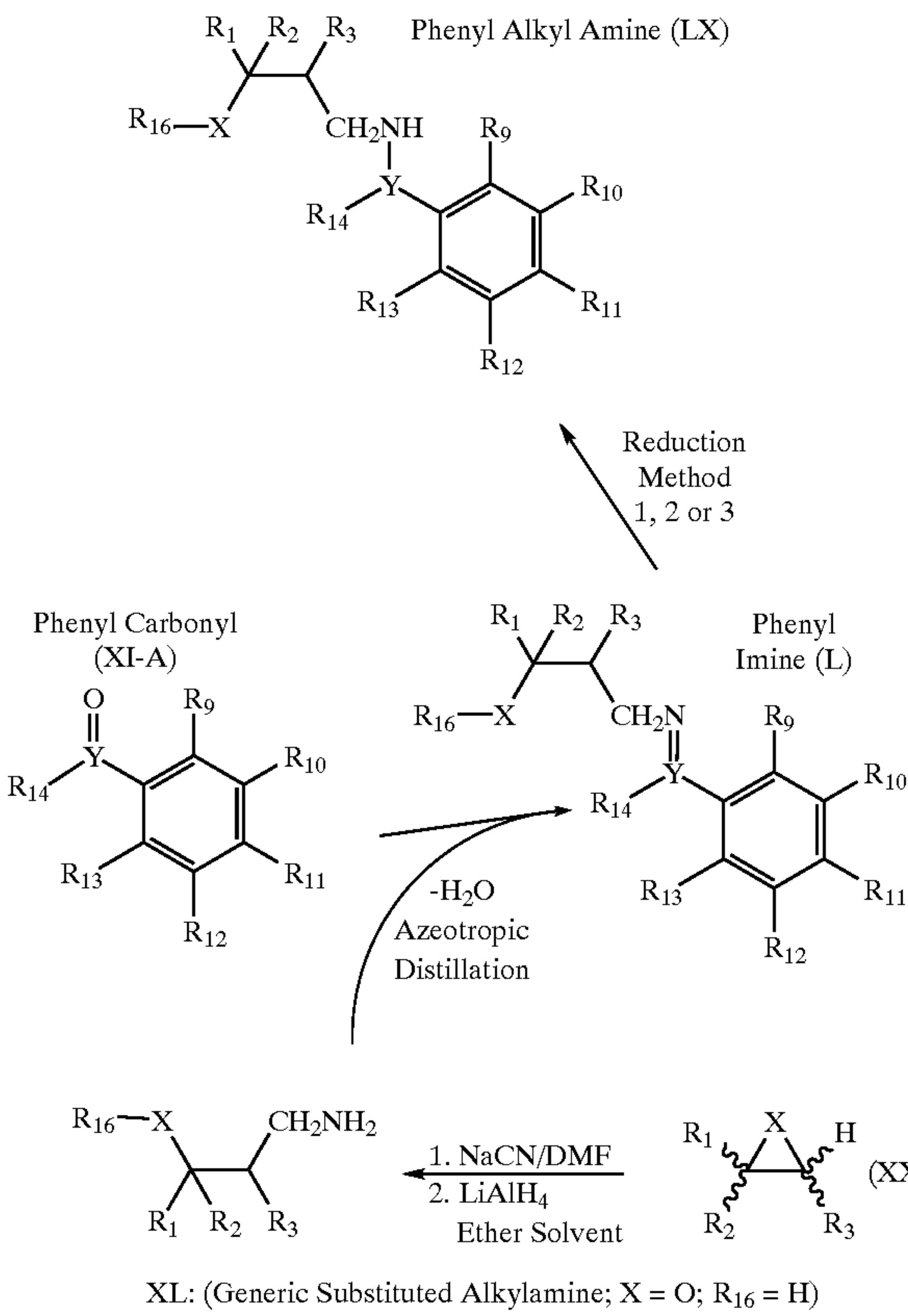
Scheme 33
