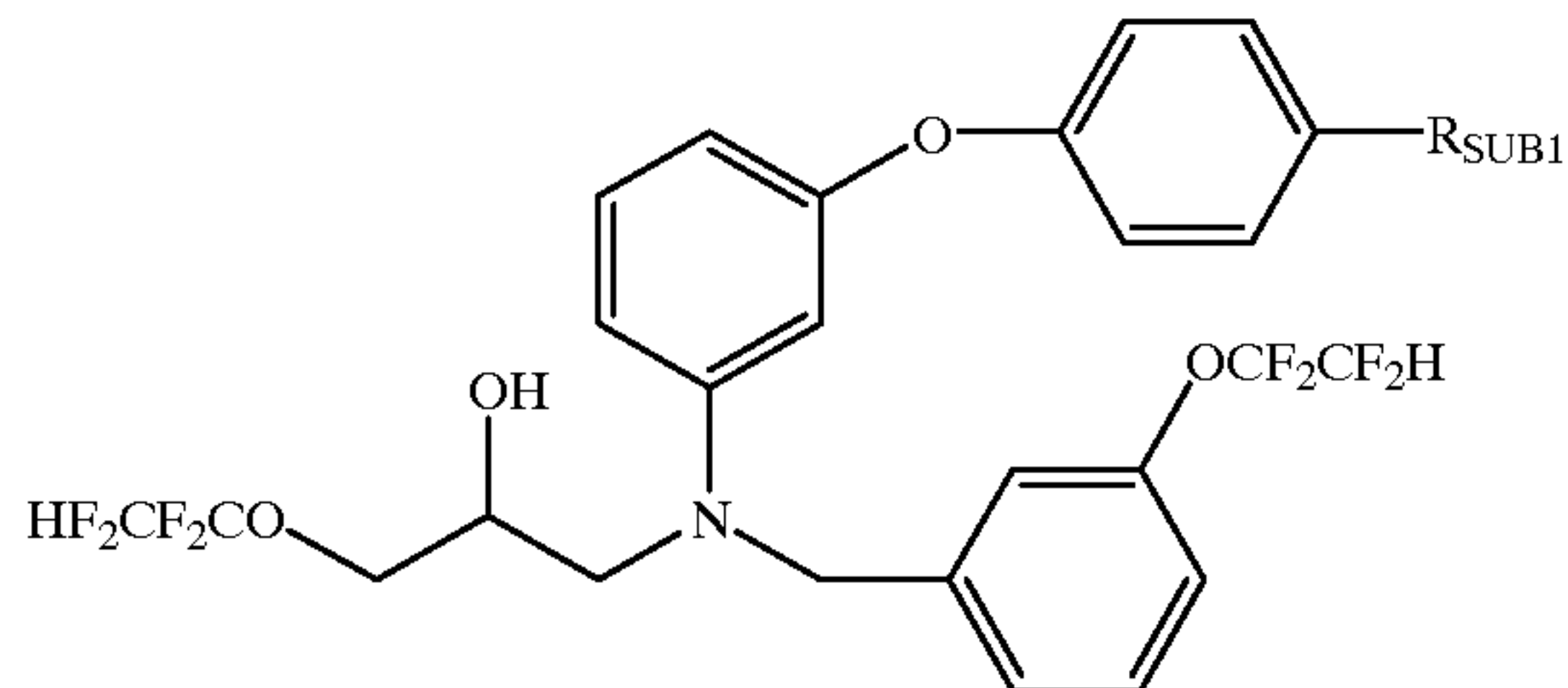
Example Table 48. 3-[N-(aryl)-N-(aralkyl)amino]- 1-haloalkoxy-2-propanols.
