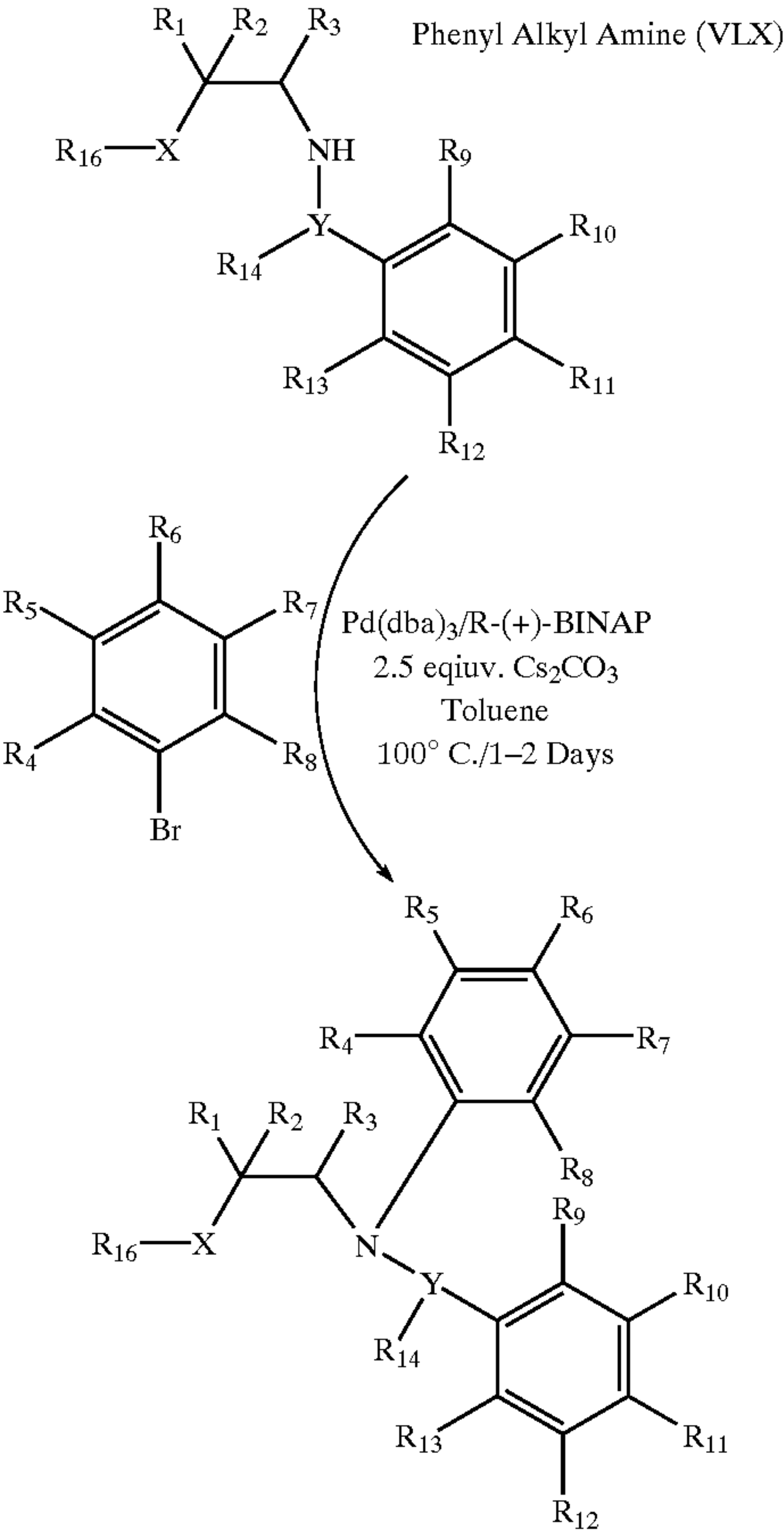
VII: (Generic Substituted Polycyclic Phenyl Tertiary 2-hydroxyalkylamine)
