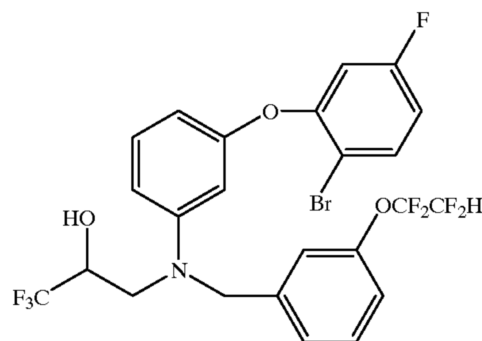
3-[[3-(2-bromo-5-fluorophenoxy)phenyl][[3-(1,1,2,2-tetrafluoroethoxy)phenyl]methyl]amino]-1,1,1-trifluoro-2-propanol
