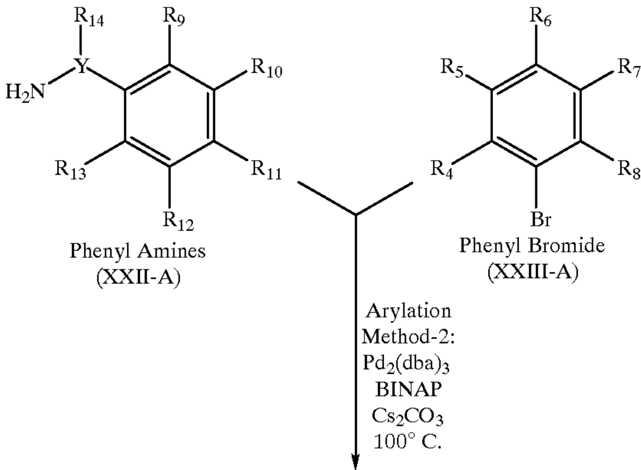
Scheme 10
