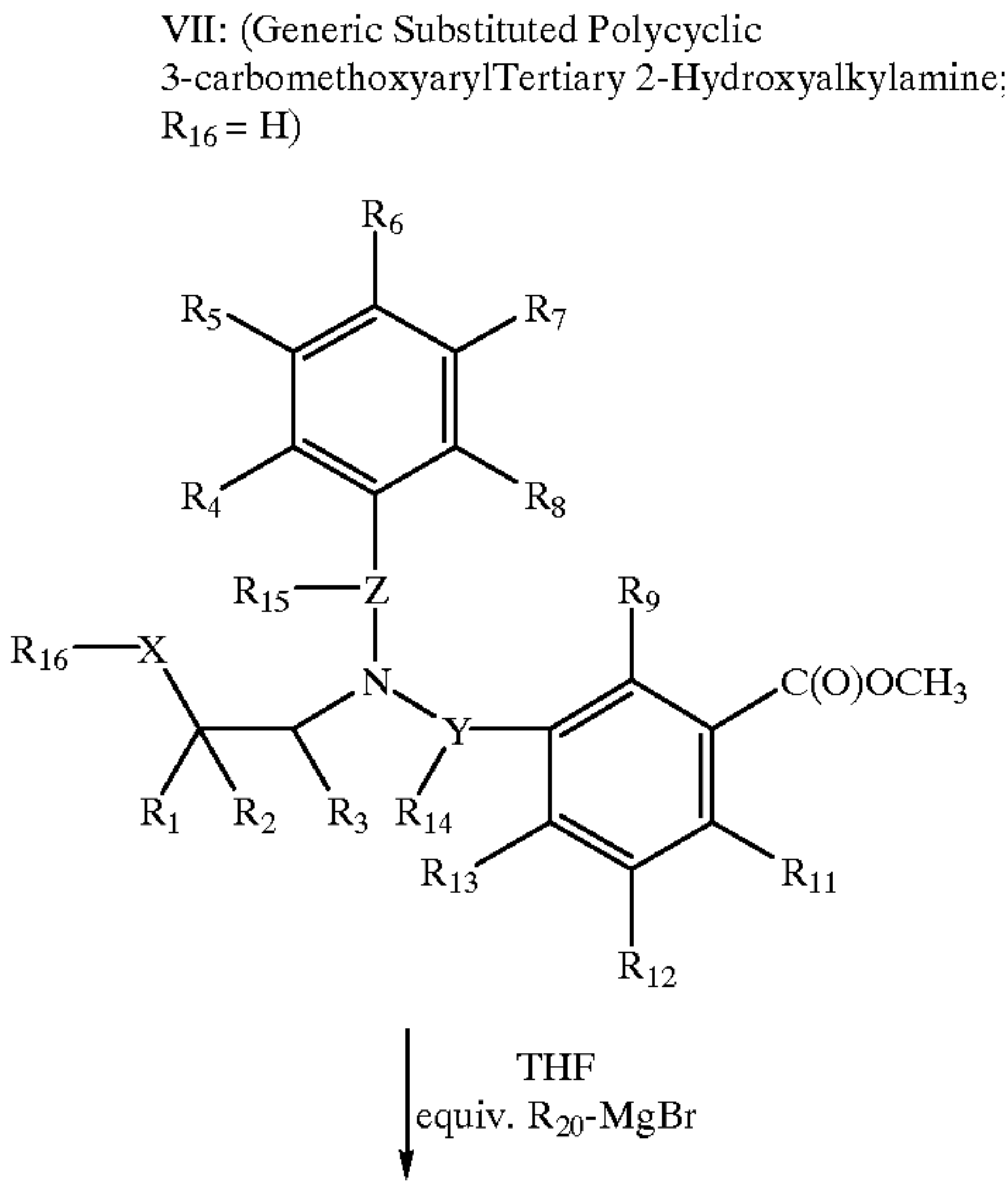
Scheme 37
