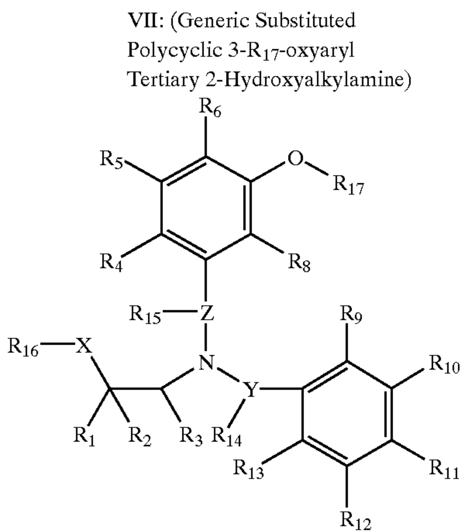
Scheme 20
