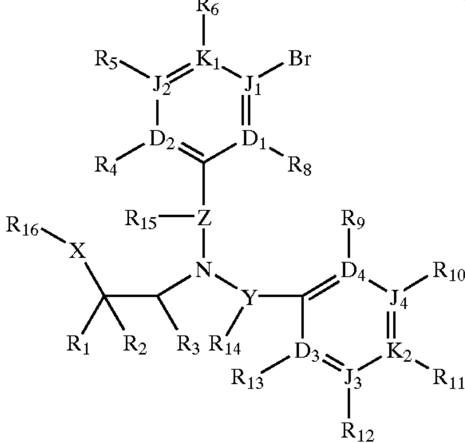
VII-H: (Generic Substituted Polycyclic 3-Bromoheteroaryl Tertiary 2-Hydroxyalkylamine)
