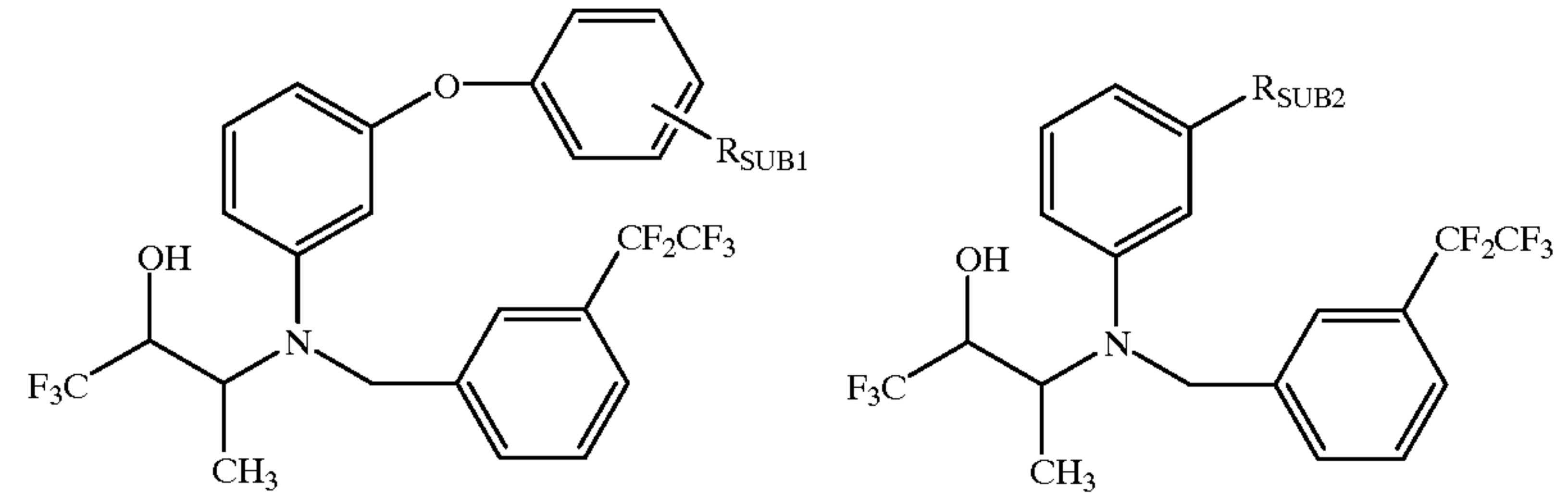
Example Table 52. Substituted 3-[N-(aryl)-[(aryl)methyl]amino]-1,1,1-trifluoro-2-butanols.
