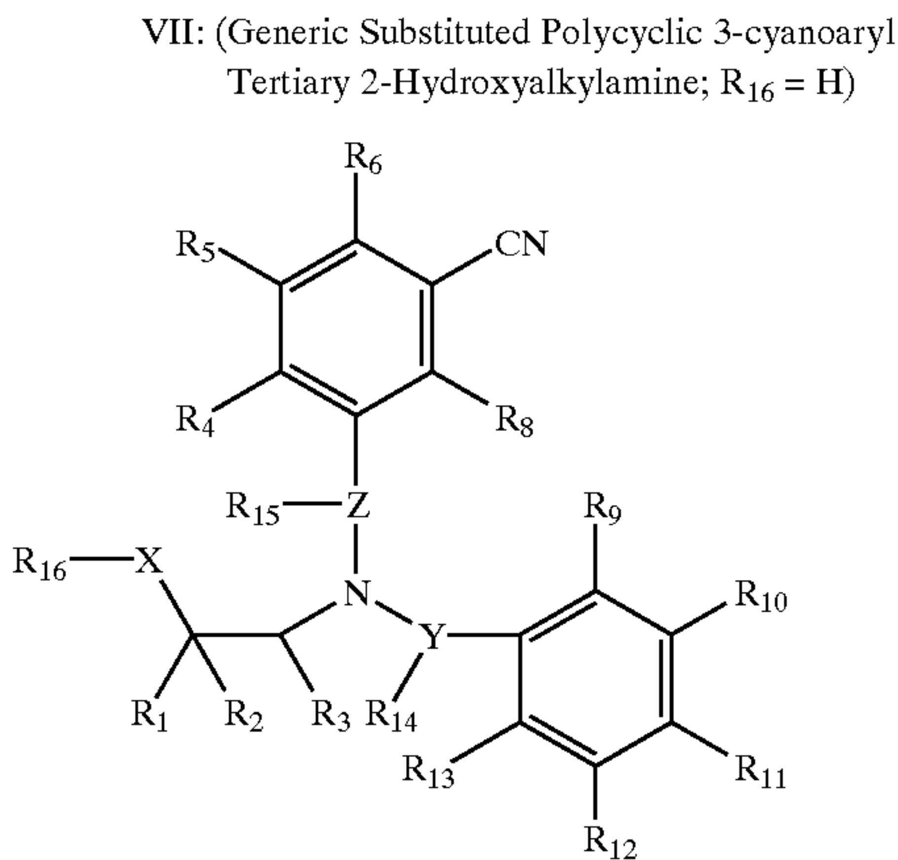
Scheme 28
