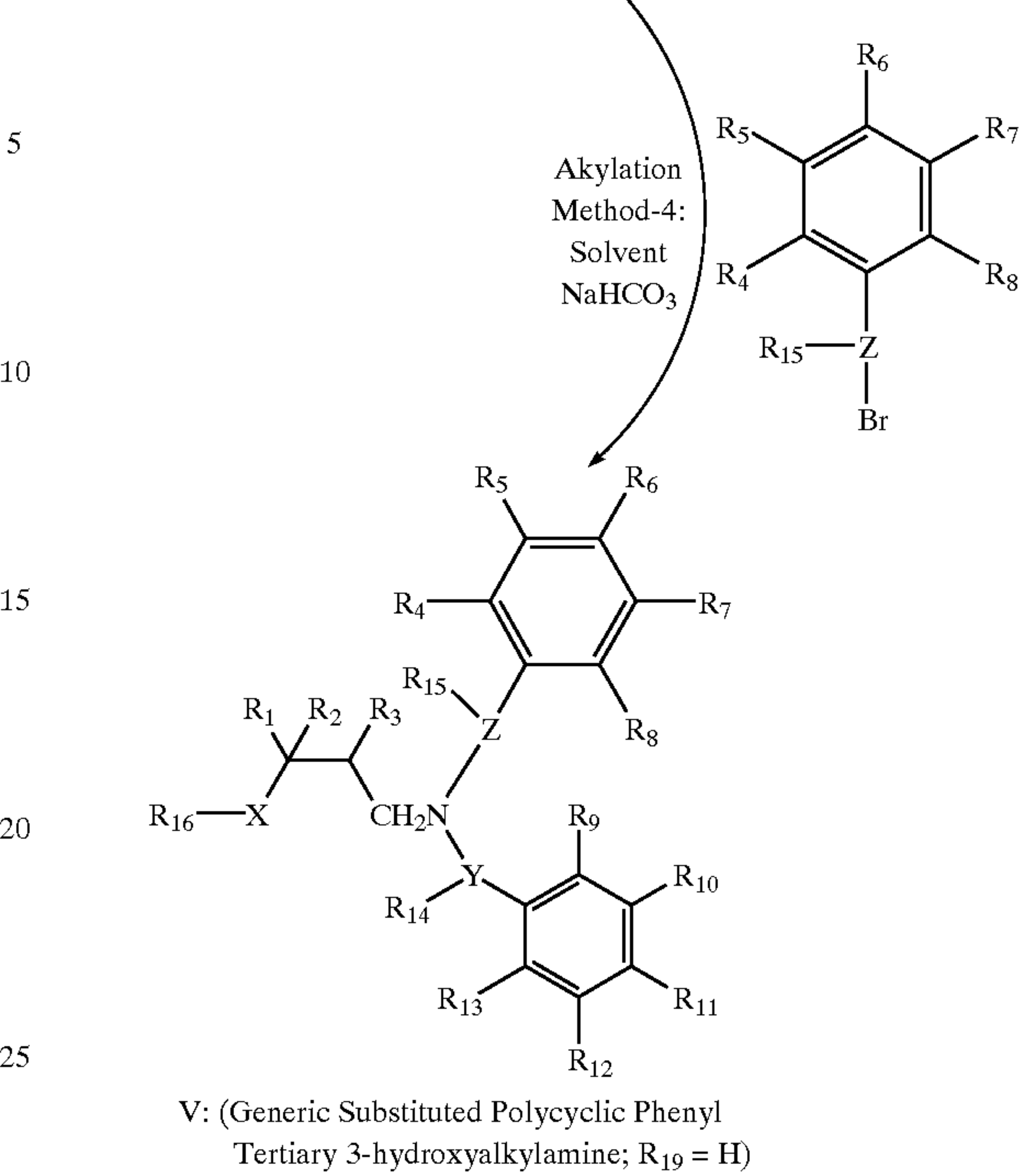
Scheme 35
