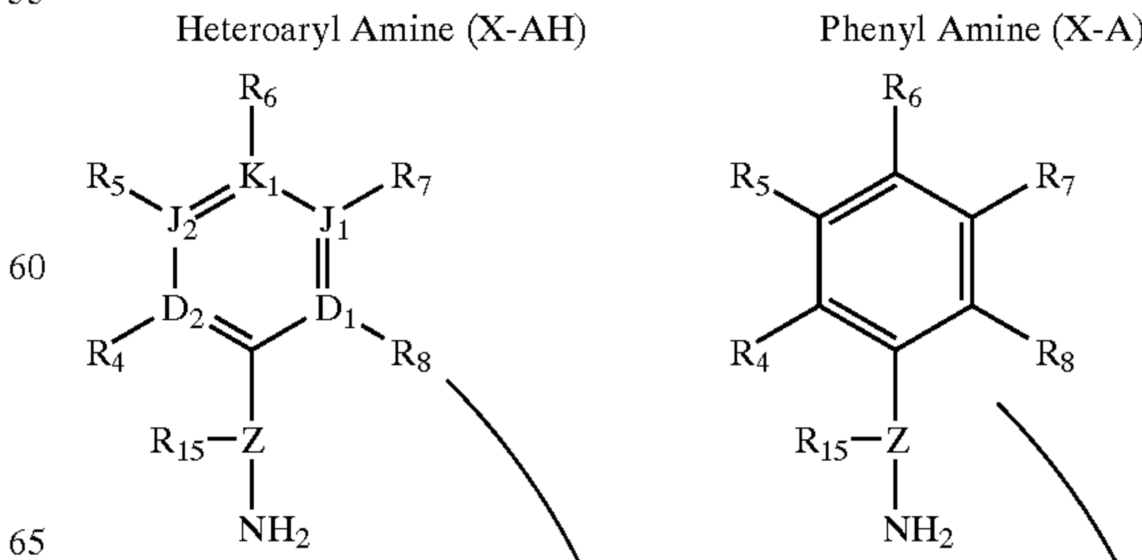
Scheme 4
