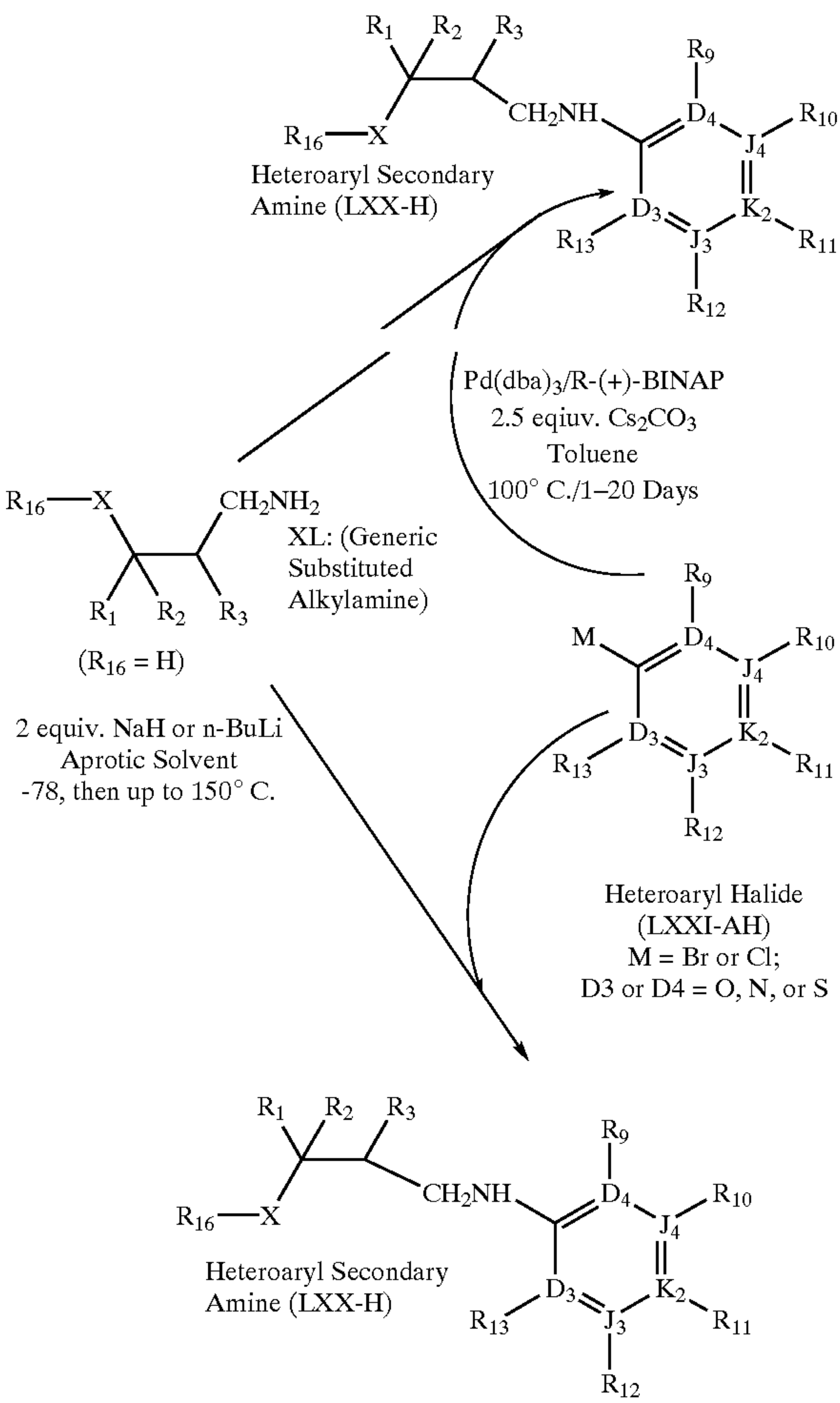
Scheme 54
