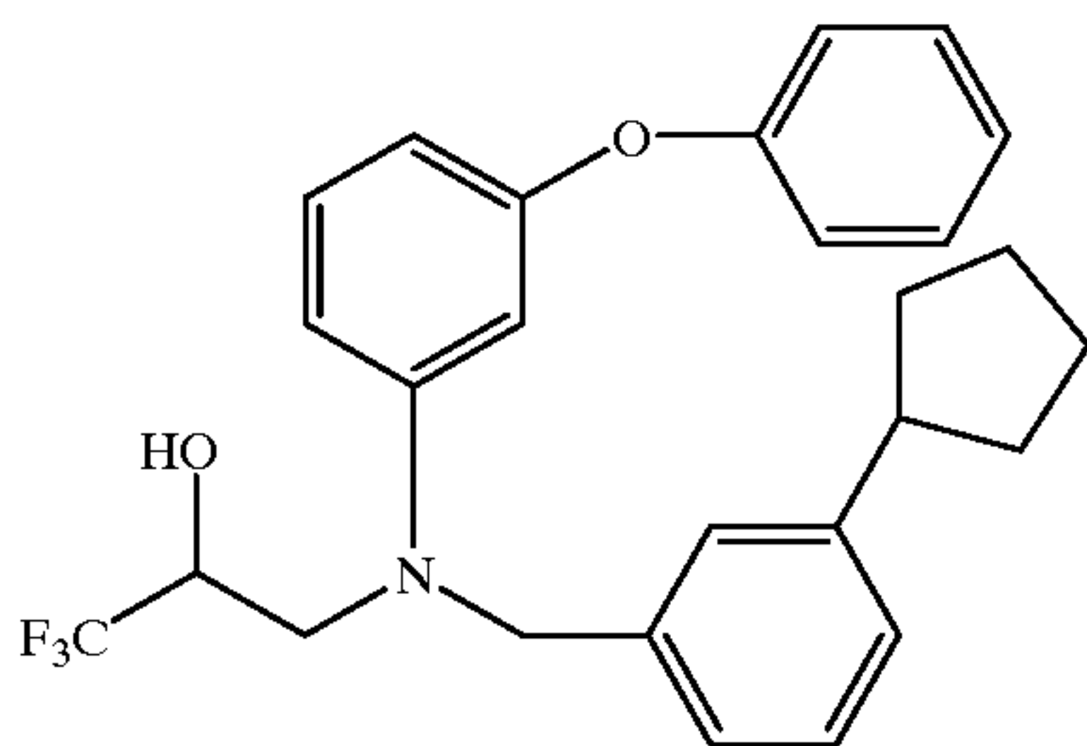
3-[(3-phenoxyphenyl)-[(3-cyclopentylphenyl)methyl]amino]-1,1,1-trifluoro-2-propanol
