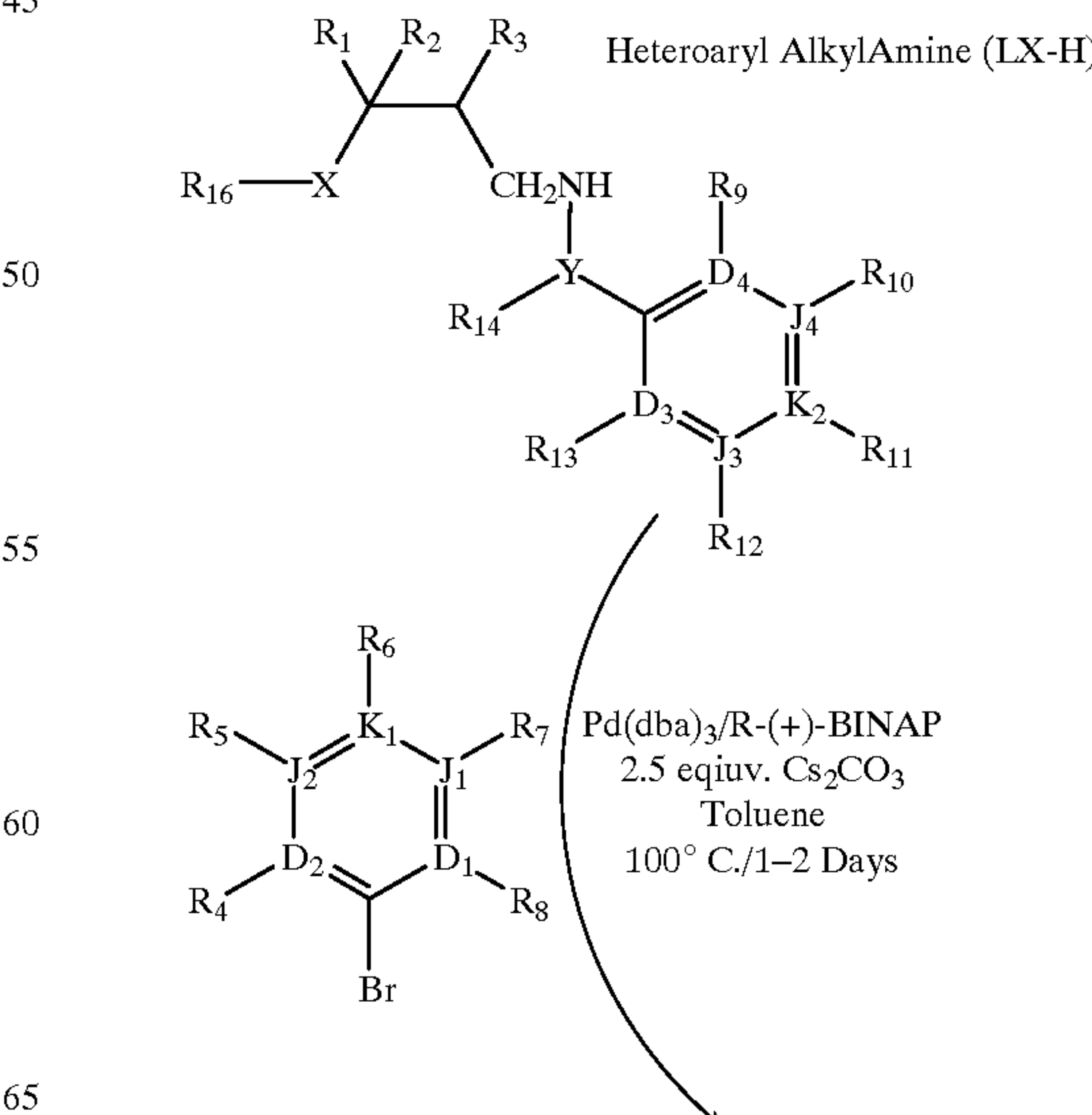
Scheme 32
