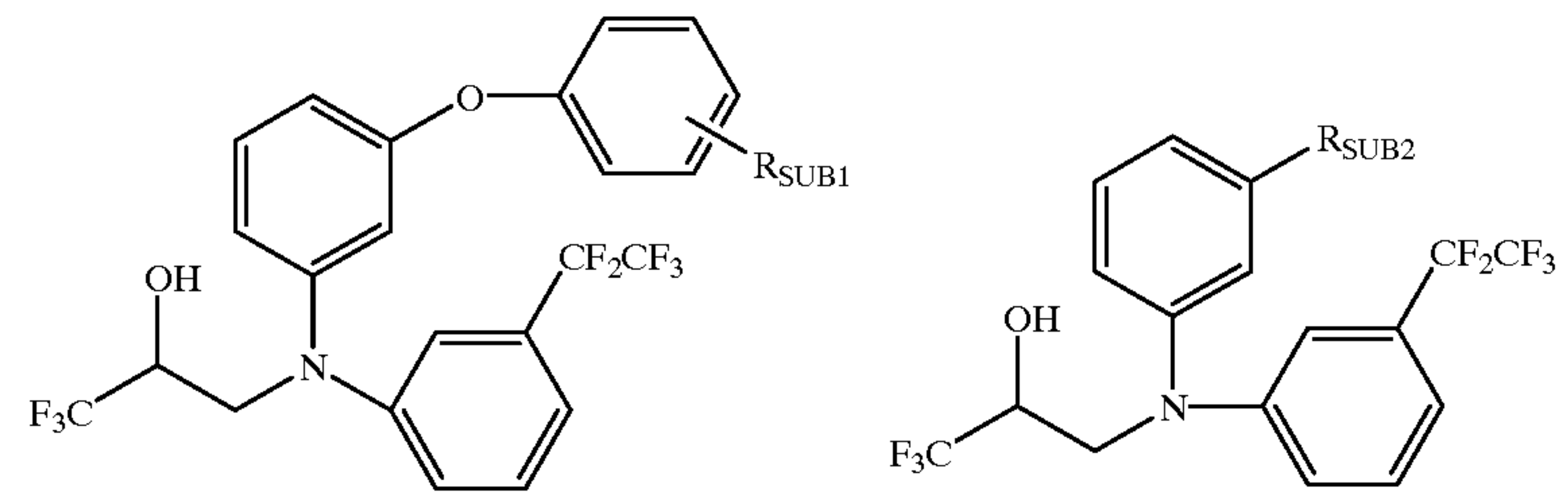
Example Table 53. Substituted 3-[N,N'-(diaryl)amino]-1,1,1,2,2-pentafluoro-2-propanols.
