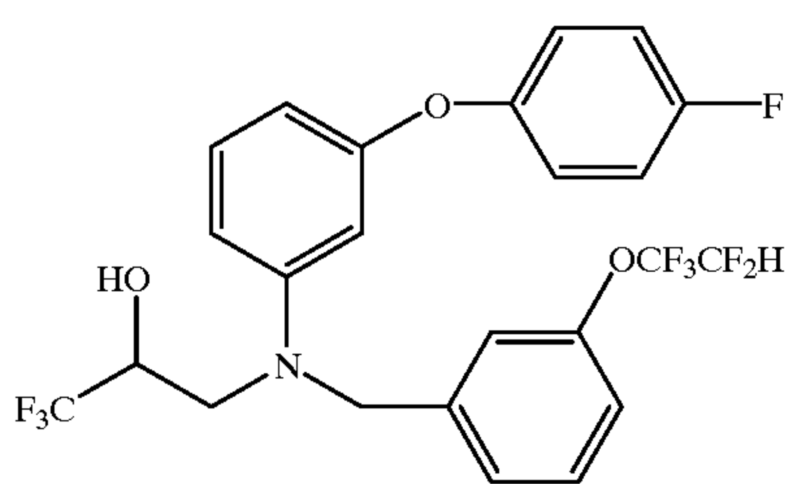
3-[[3-(4-fluorophenoxy)phenyl][[3-(1,1,2,2-tetrafluoroethoxy)phenyl]methyl]amino]-1,1,1-trifluoro-2-propanol
