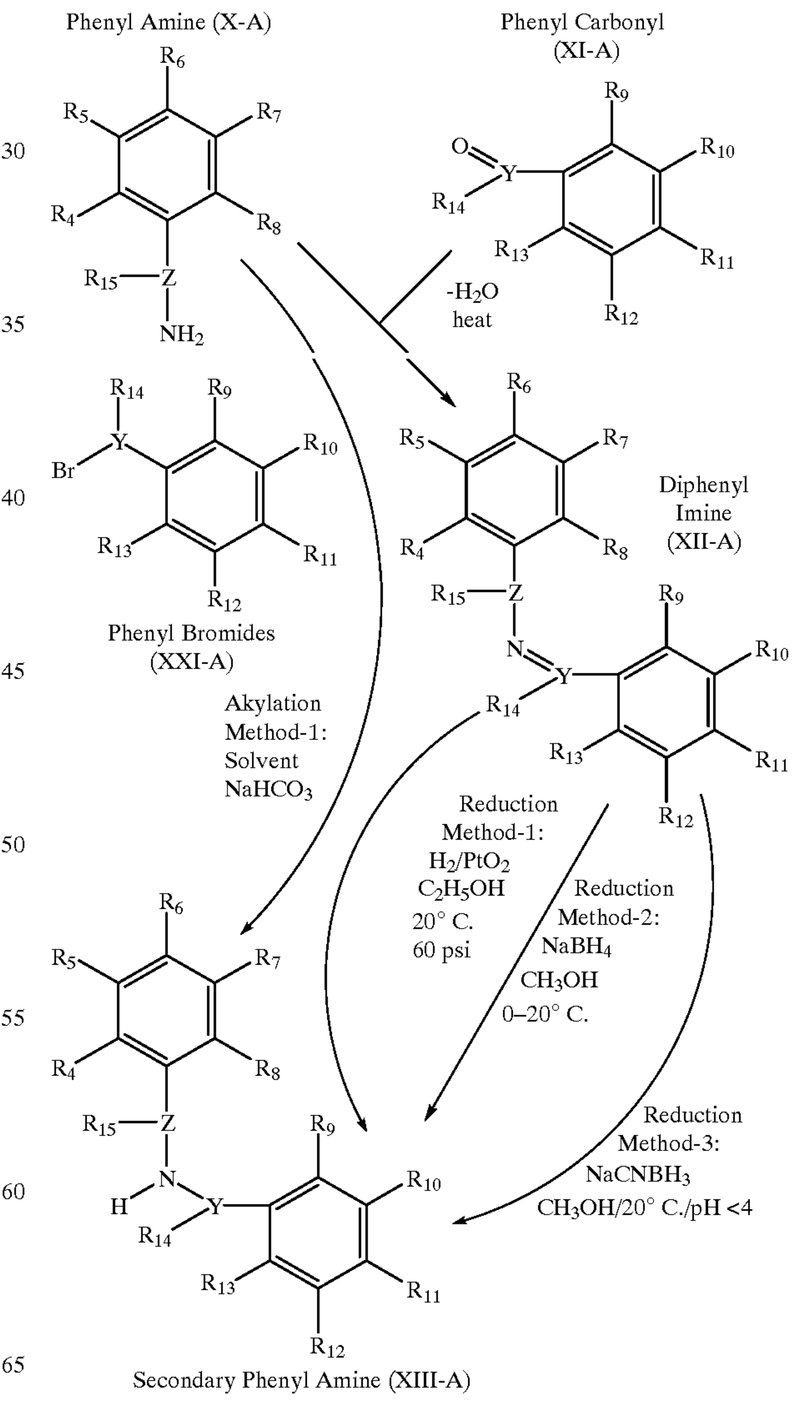
Scheme 9
