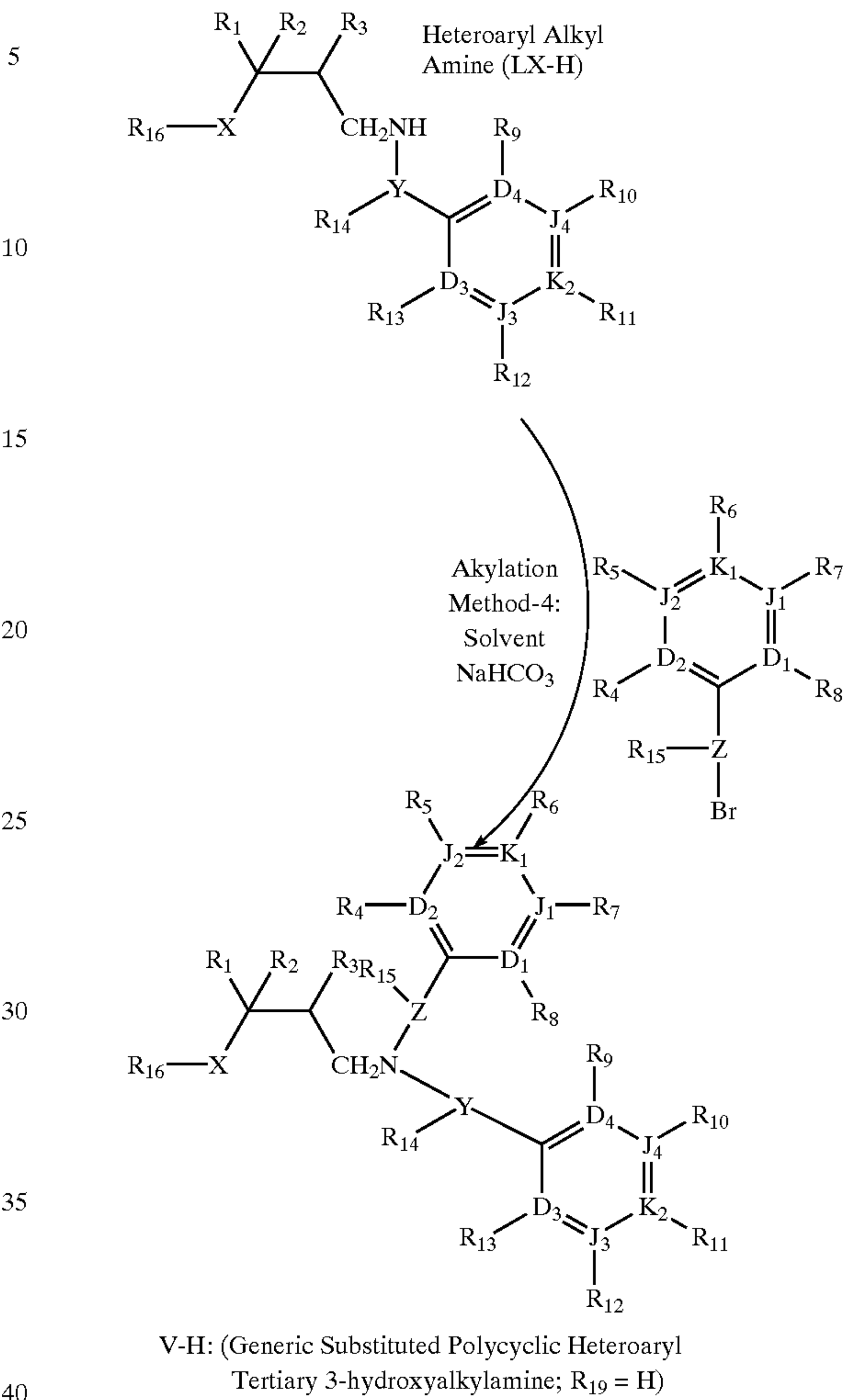
Scheme 31
