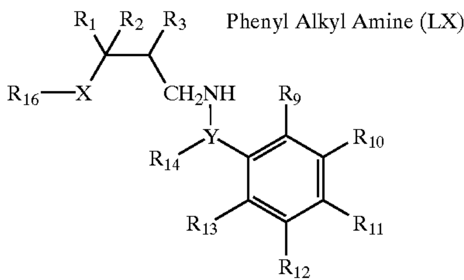
Scheme 34
