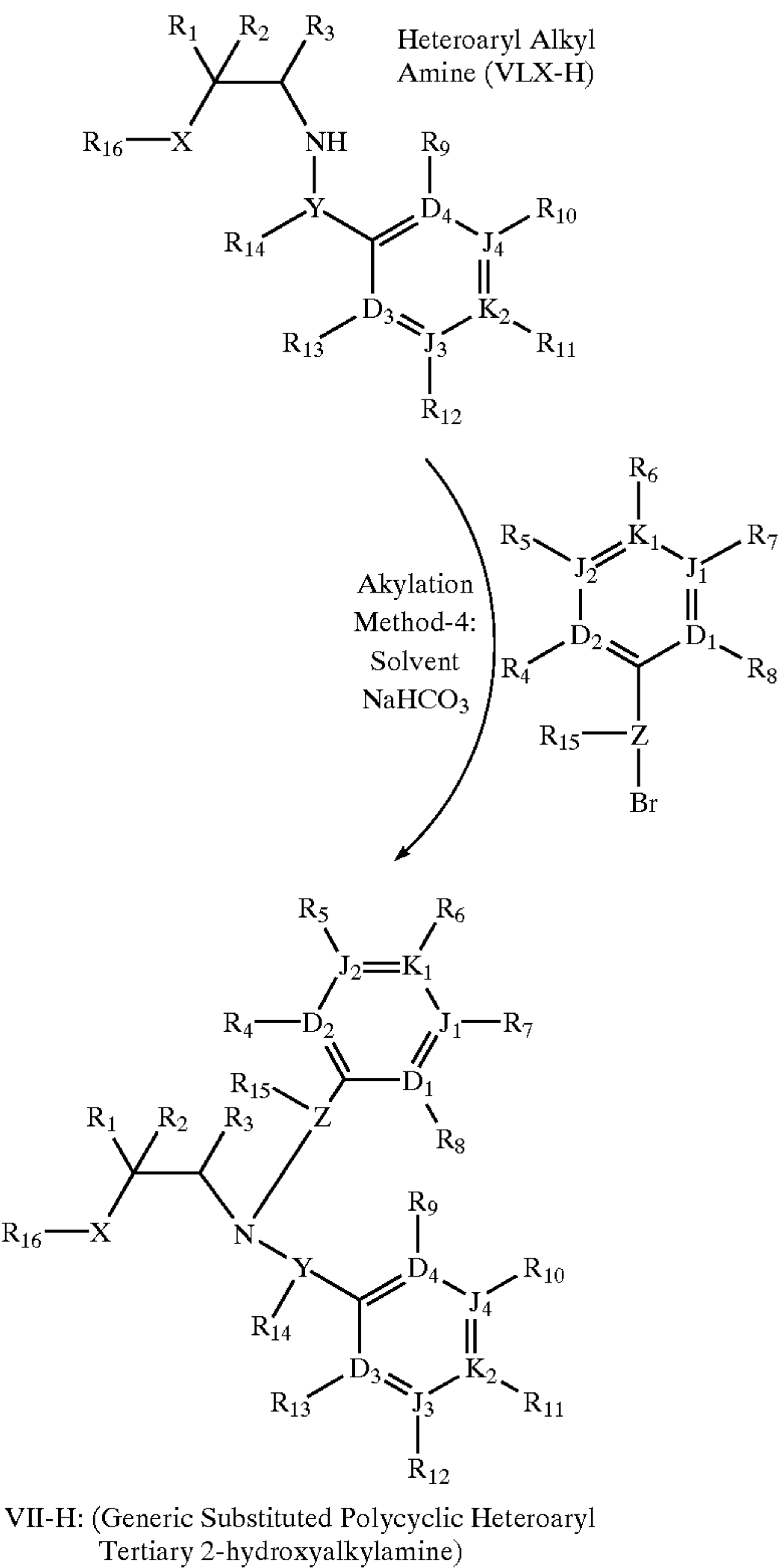
Scheme 46
