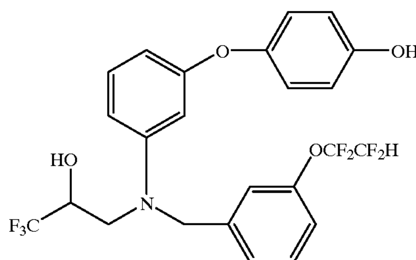
4-[3-[[3-(1,1,2,2-tetrafluoroethoxy)phenyl]methyl]amino]phenol (3,3,3-trifluoro-2-hydroxypropyl)aminophenoxy]phenol
