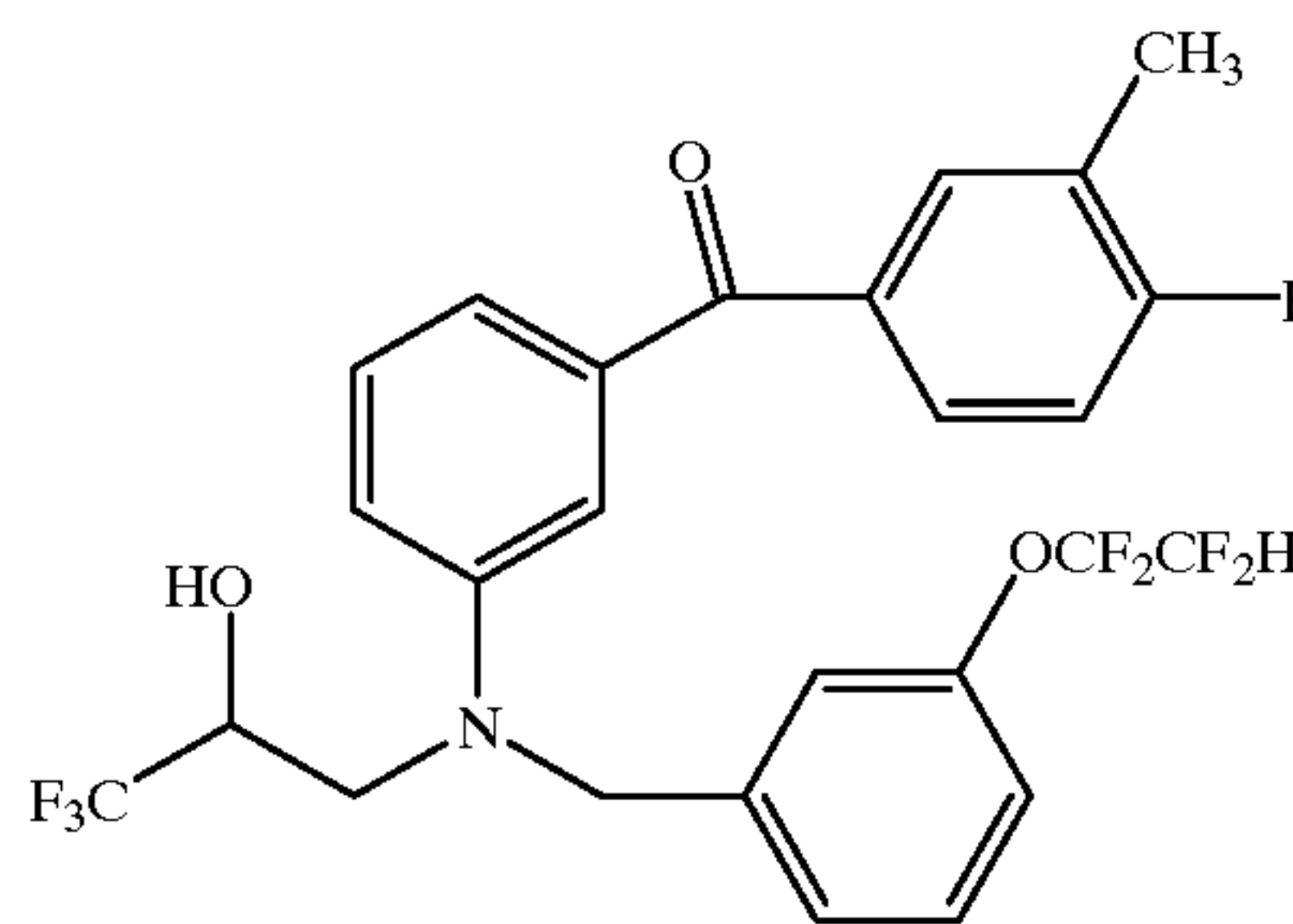
(4-Fluoro-3-methylphenyl)[3-[[[(1,1,2,2-tetrafluoroethoxy) phenyl]methyl](3,3,3-trifluoro-2-hydroxypropyl)amino]phenyl]methanone
