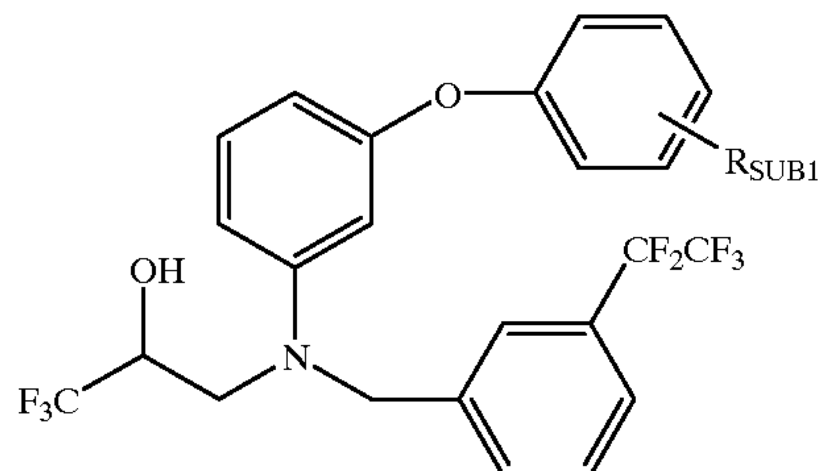
Substituted 3-[N-(aryl)-[(aryl)methyl]amino]- 1,1,1-trifluoro-2-propanols
