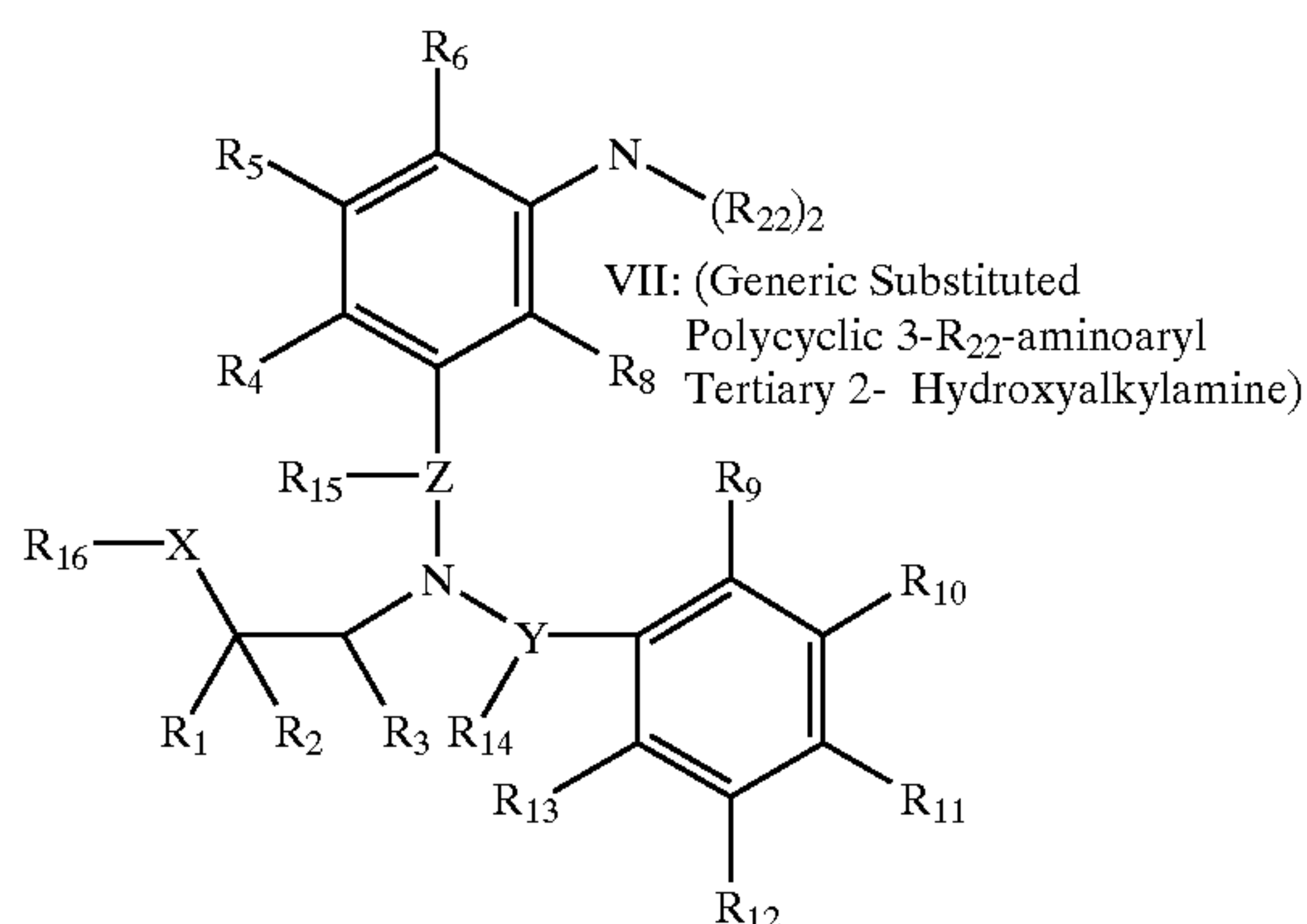
Scheme 23
