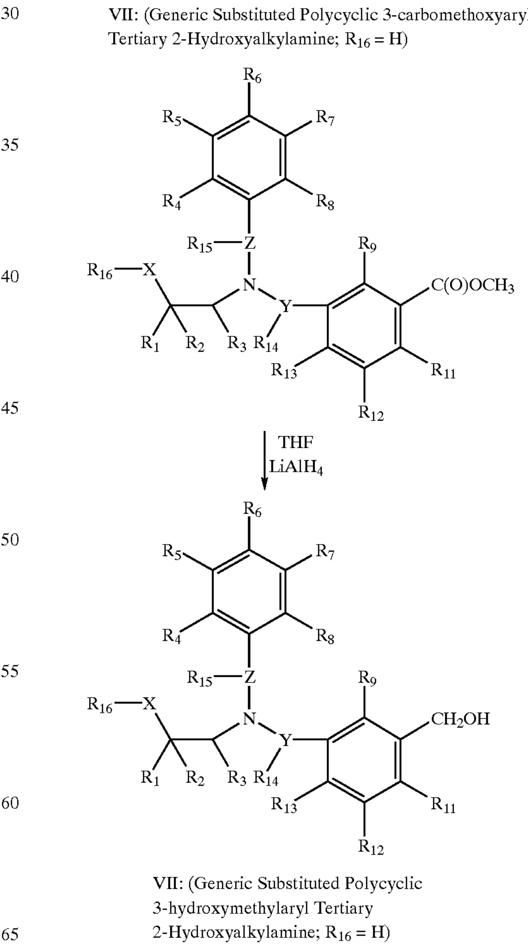
Scheme 38
