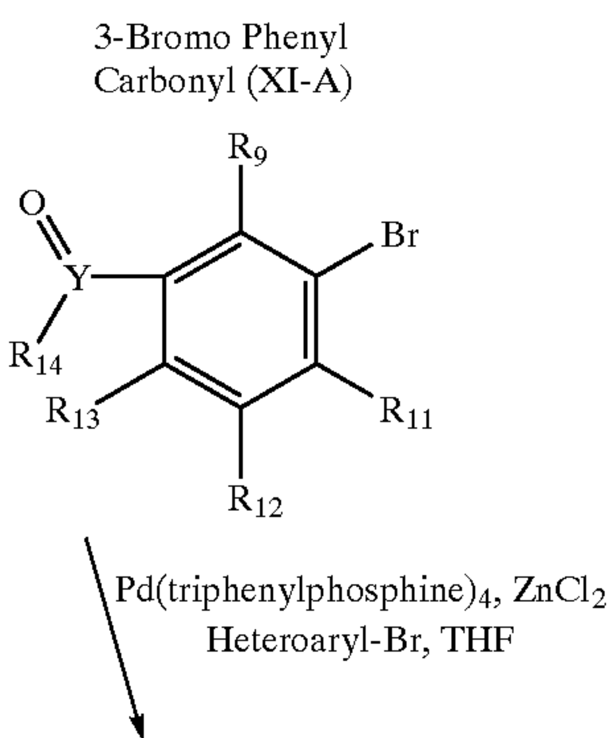
Scheme 43
