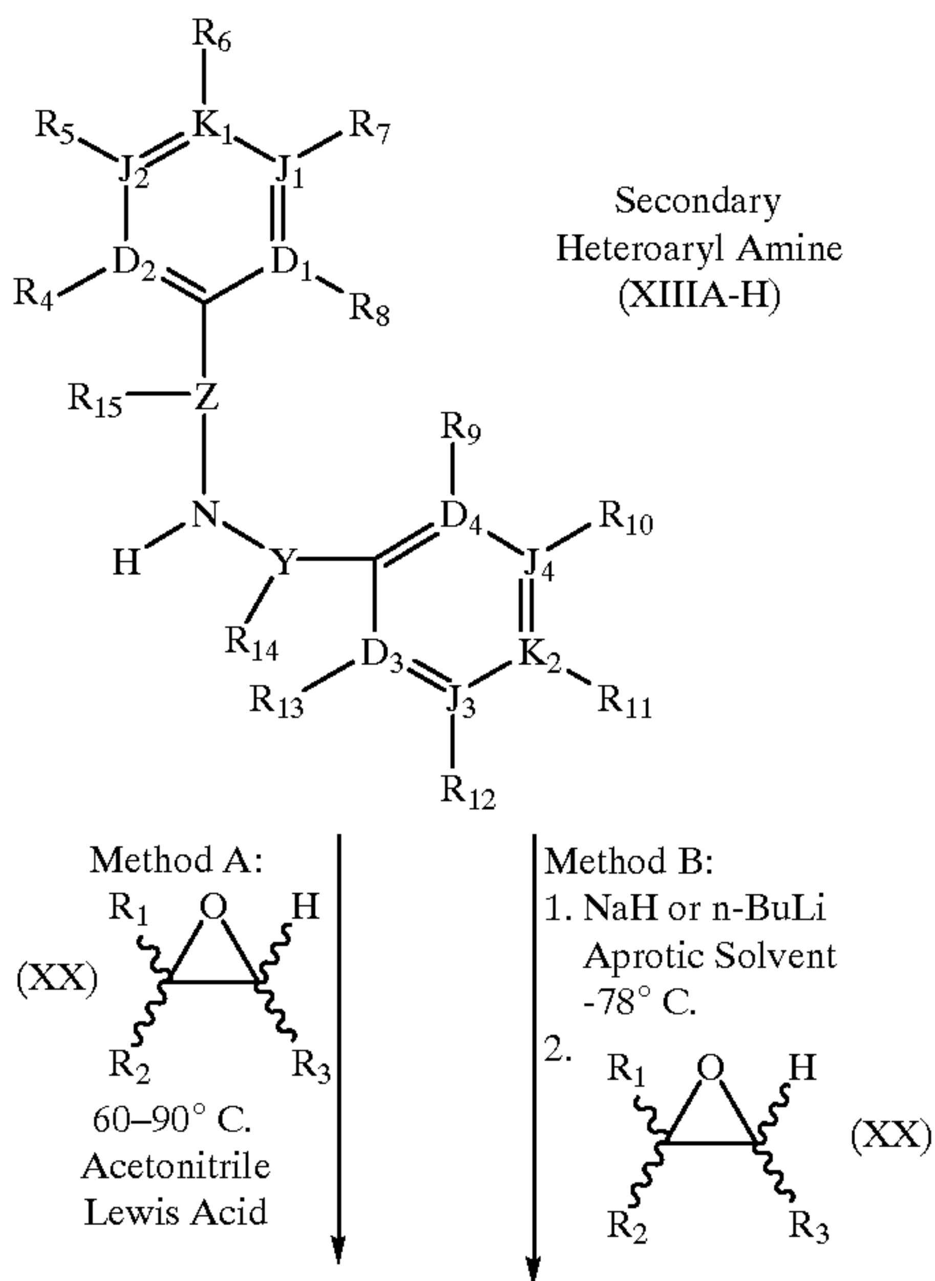
Scheme 7
