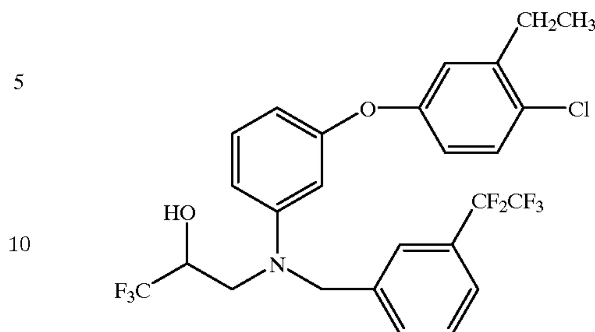
3-[(4-chloro-3-ethylphenoxy)phenyl][[3-(pentafluoroethyl)phenyl]methyl]-amino]-1,1,1-trifluoro-2-propanol.
