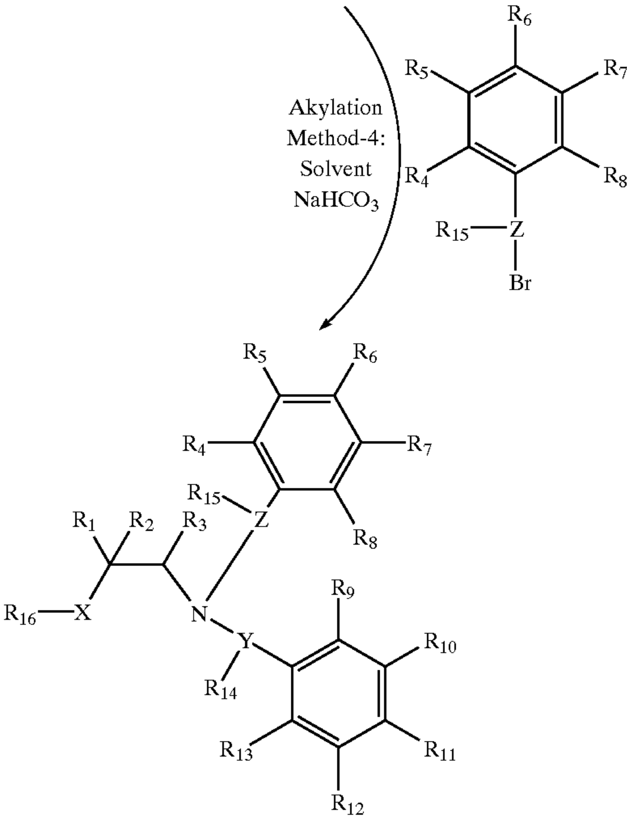
VII: (Generic Substituted Polycyclic Phenyl Tertiary 2-hydroxyalkylamine)
