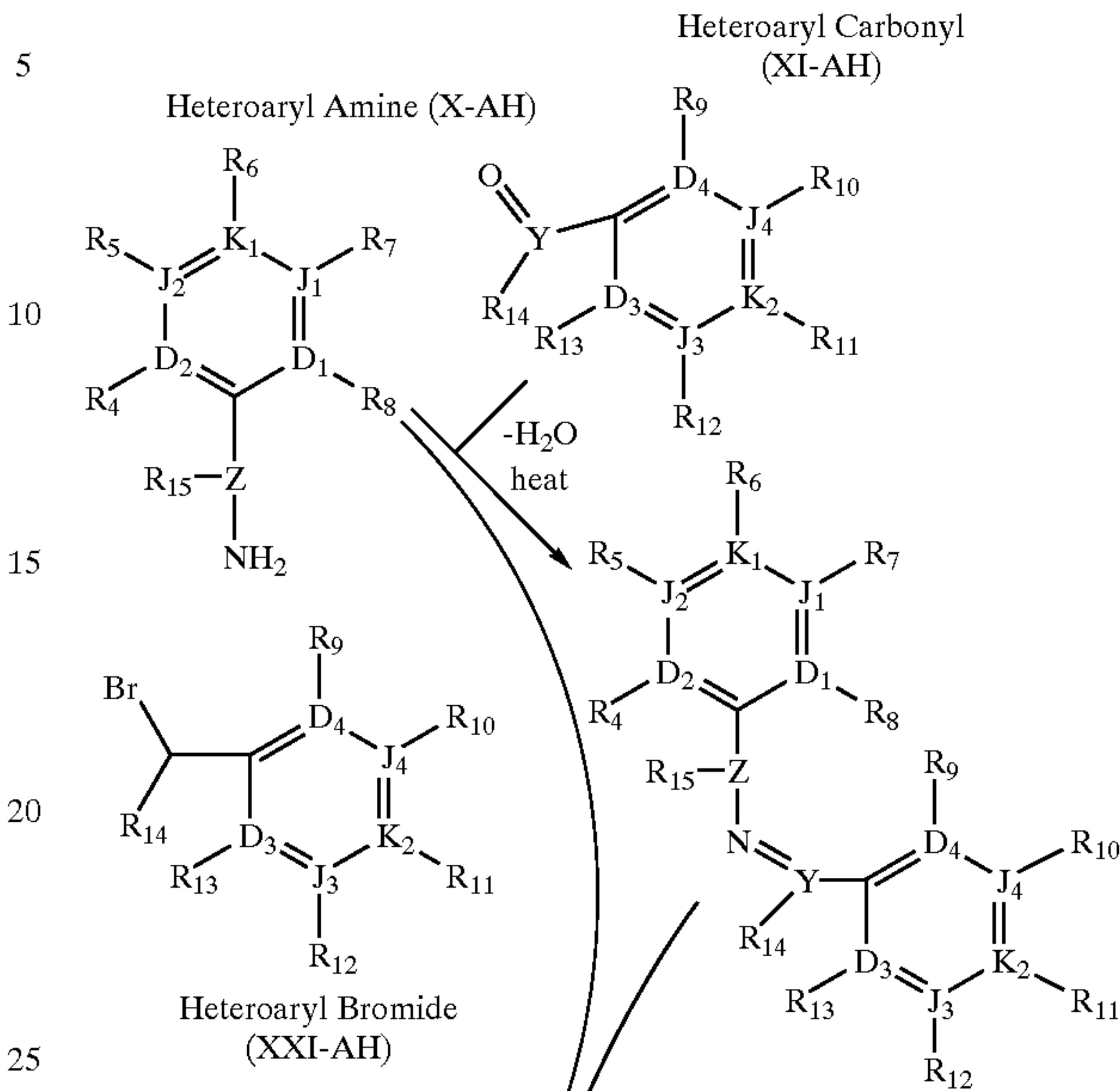
Scheme 3
