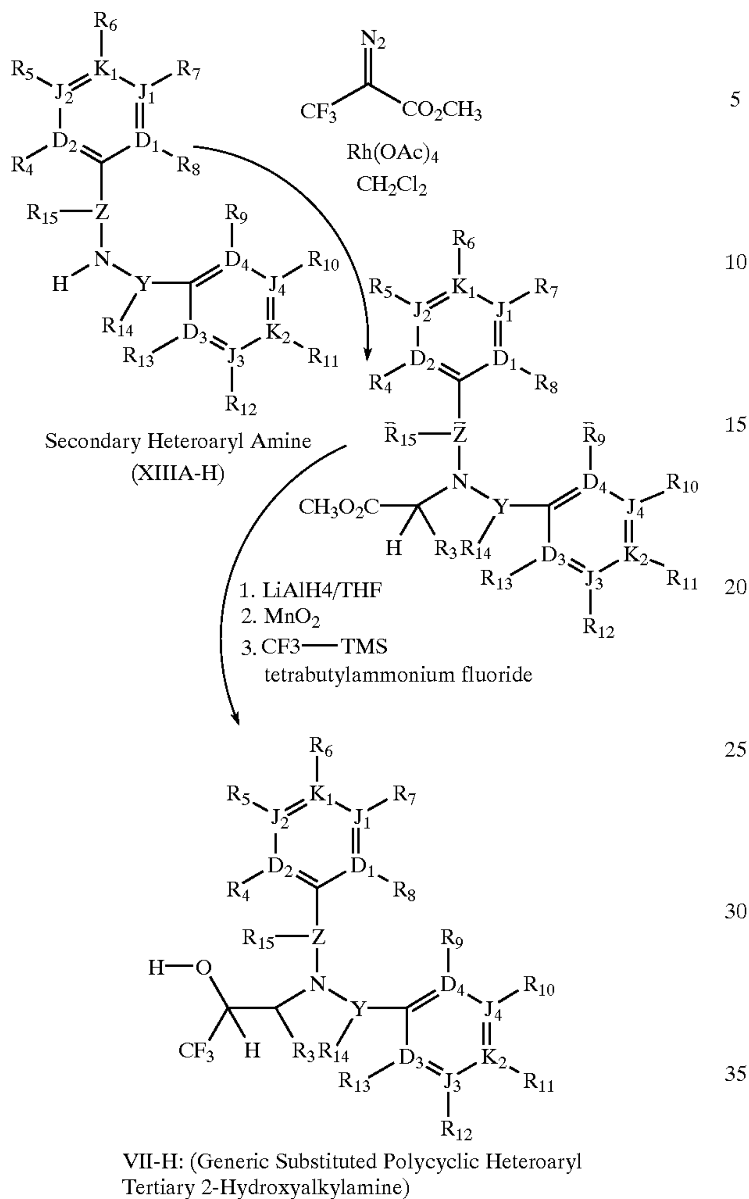
Scheme 57
