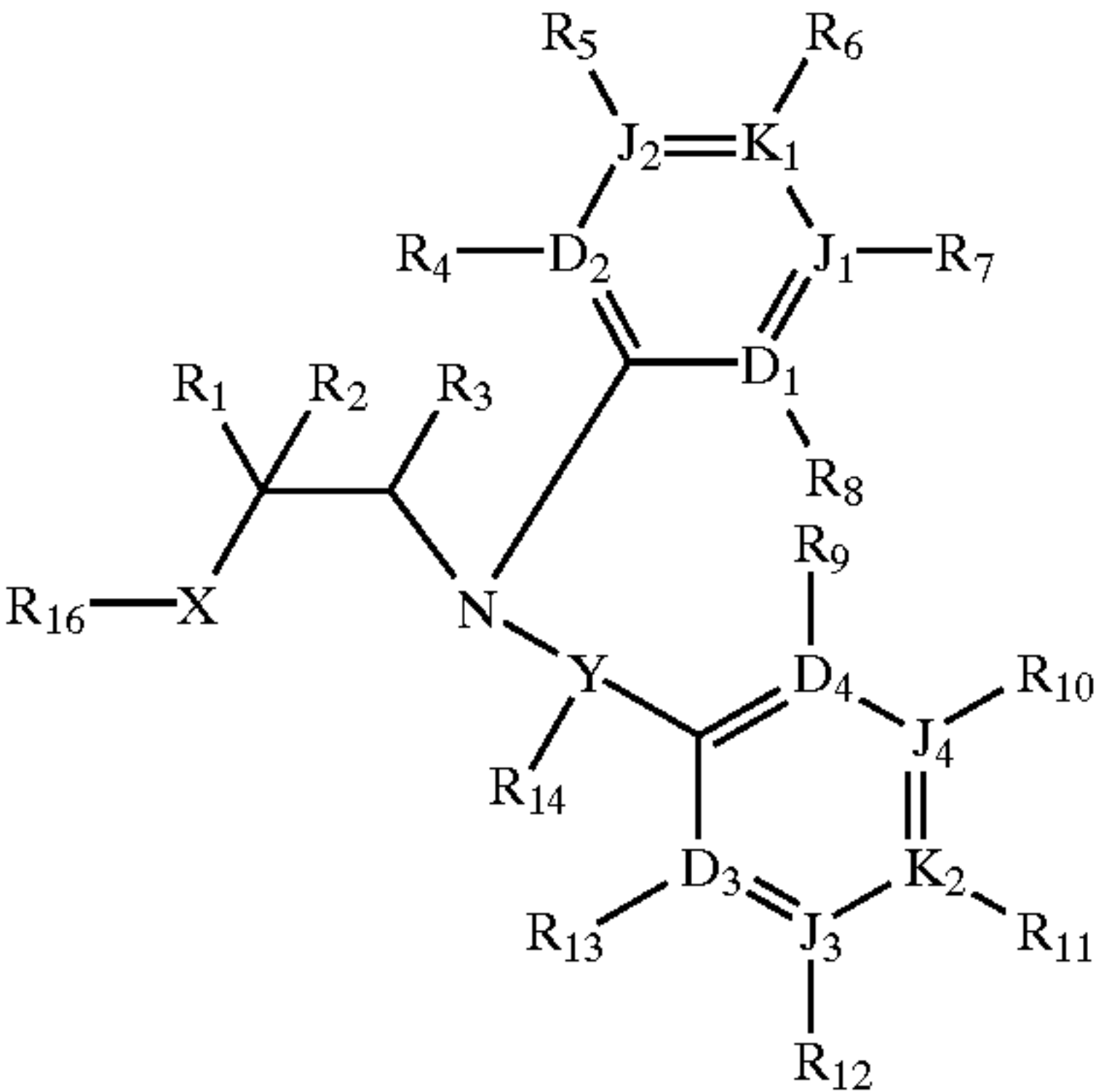
VII-H: (Generic Substituted Polycyclic Heteroaryl Tertiary 2-hydroxyalkylamine)
