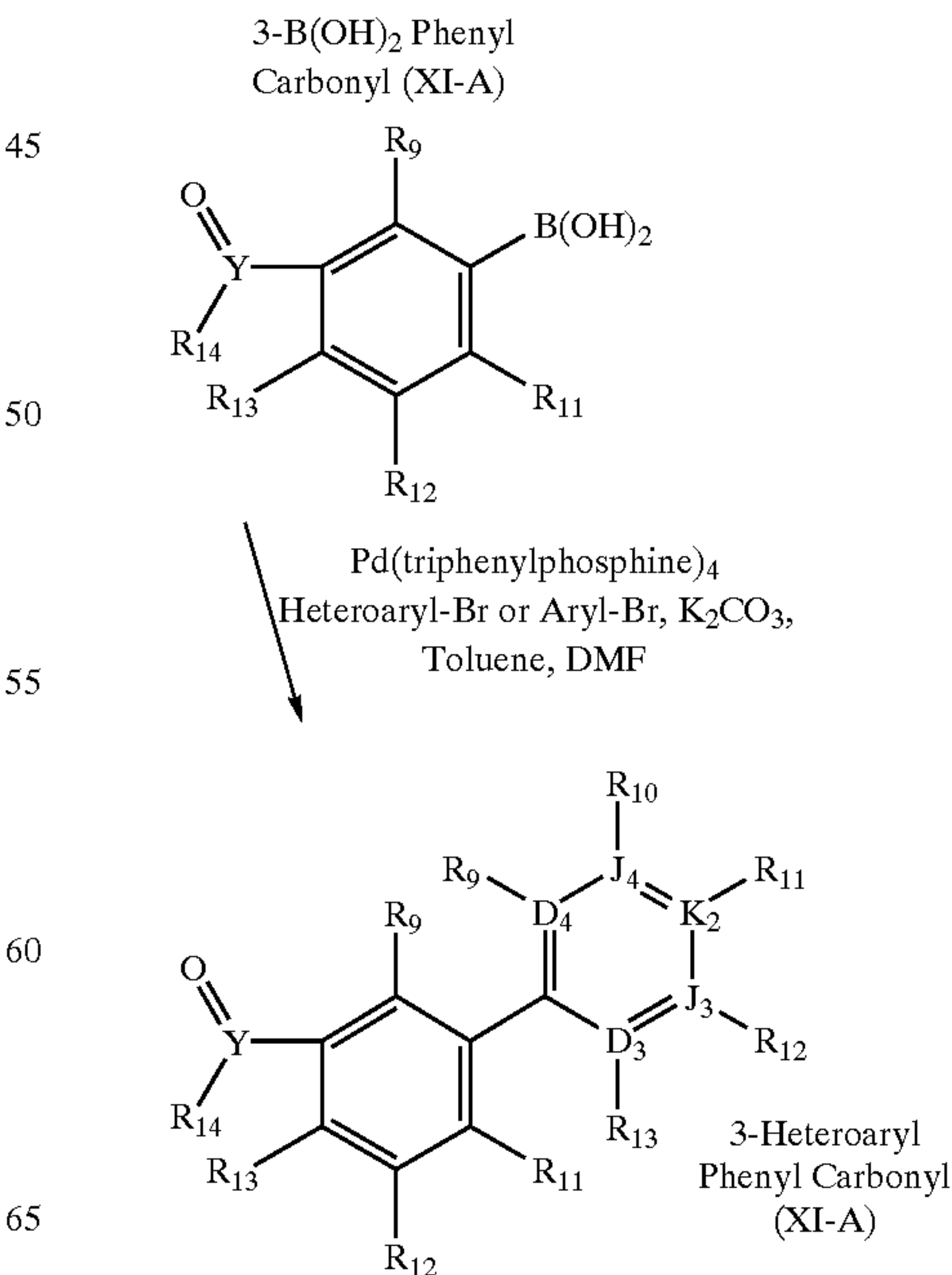
Scheme 44
