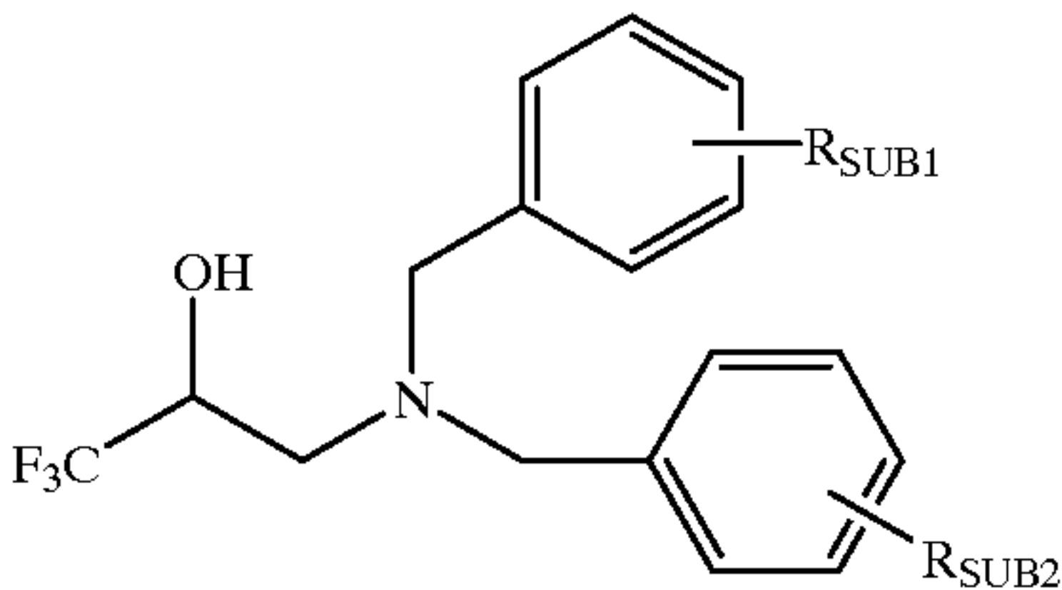
Example Table 44. 3-[N-[(aryl)methyl]-[(aryl)methyl]amino]-1,1,1-trifluoro-2-propanols.
