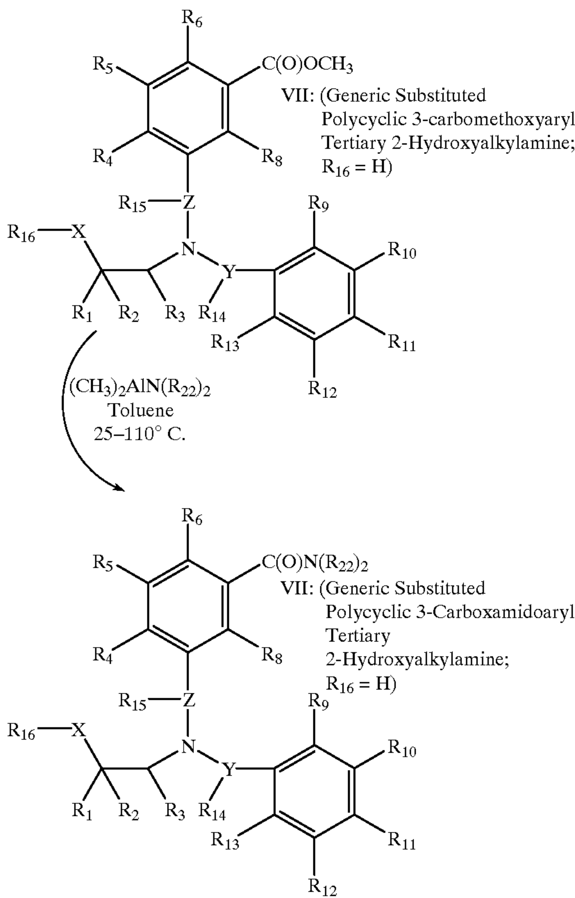
Scheme 27
