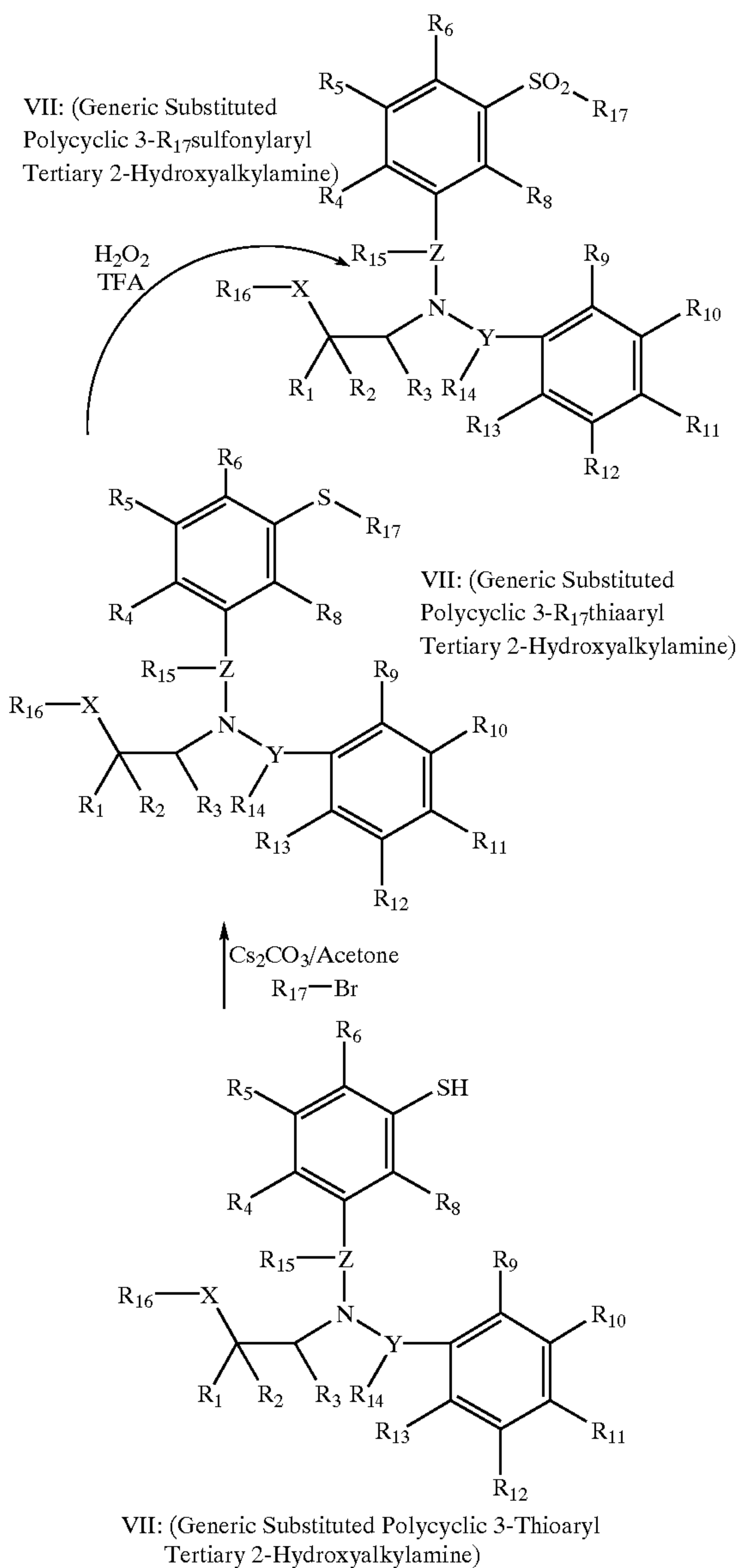
Scheme 19
