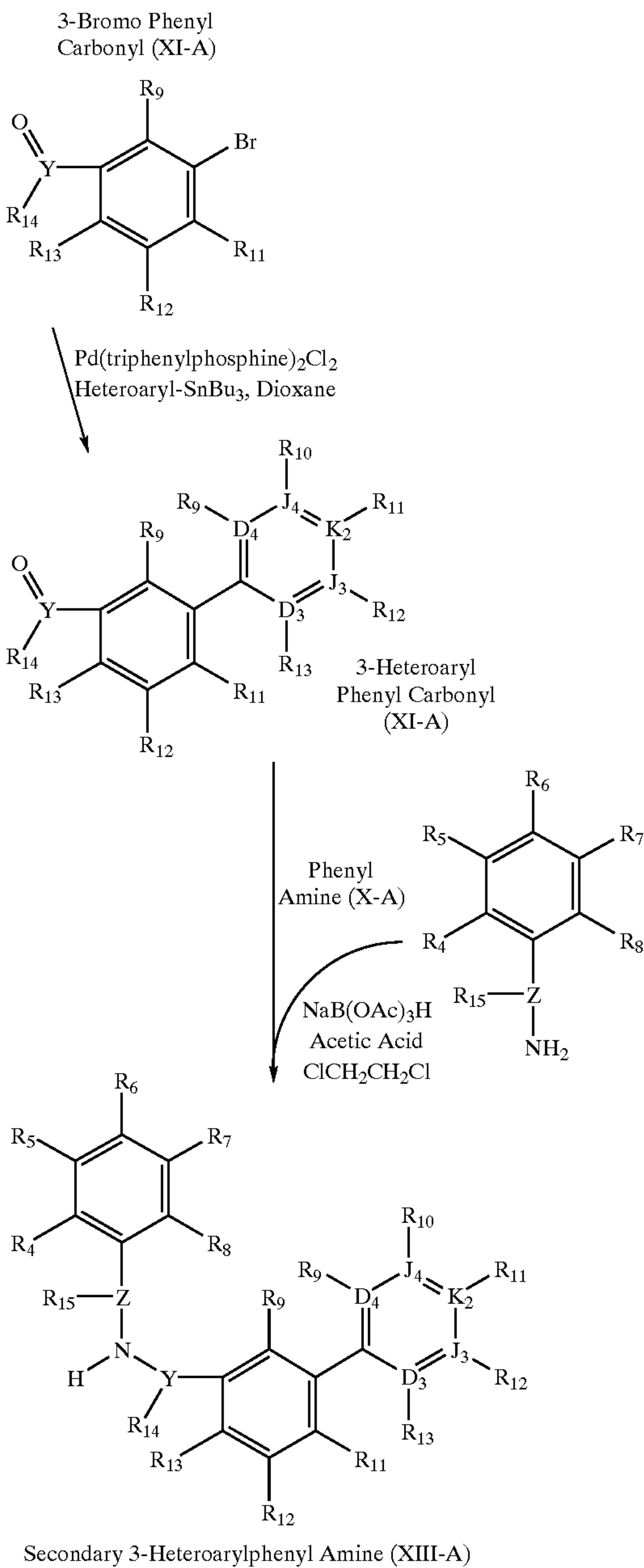
Scheme 42
