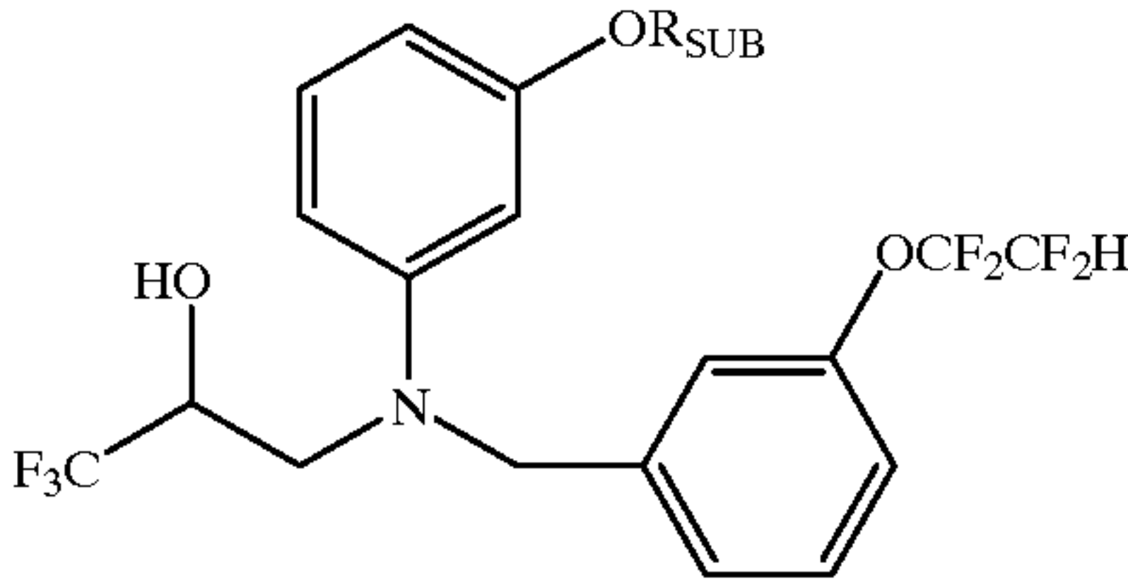
Example Table 19. 3-[[[3-aryloxyphenyl]methyl]amino]-1,1,1-trifluoro-2-propanols.
