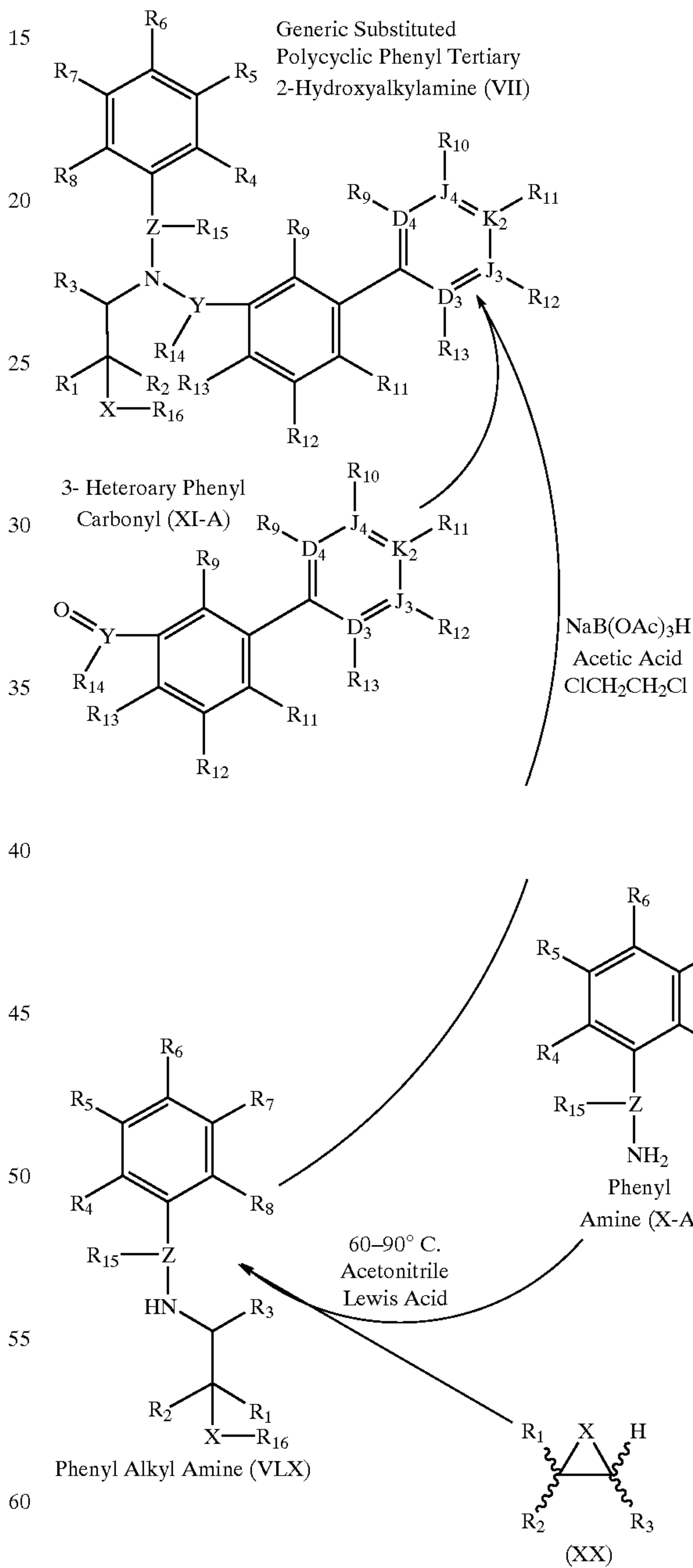
Scheme 56
