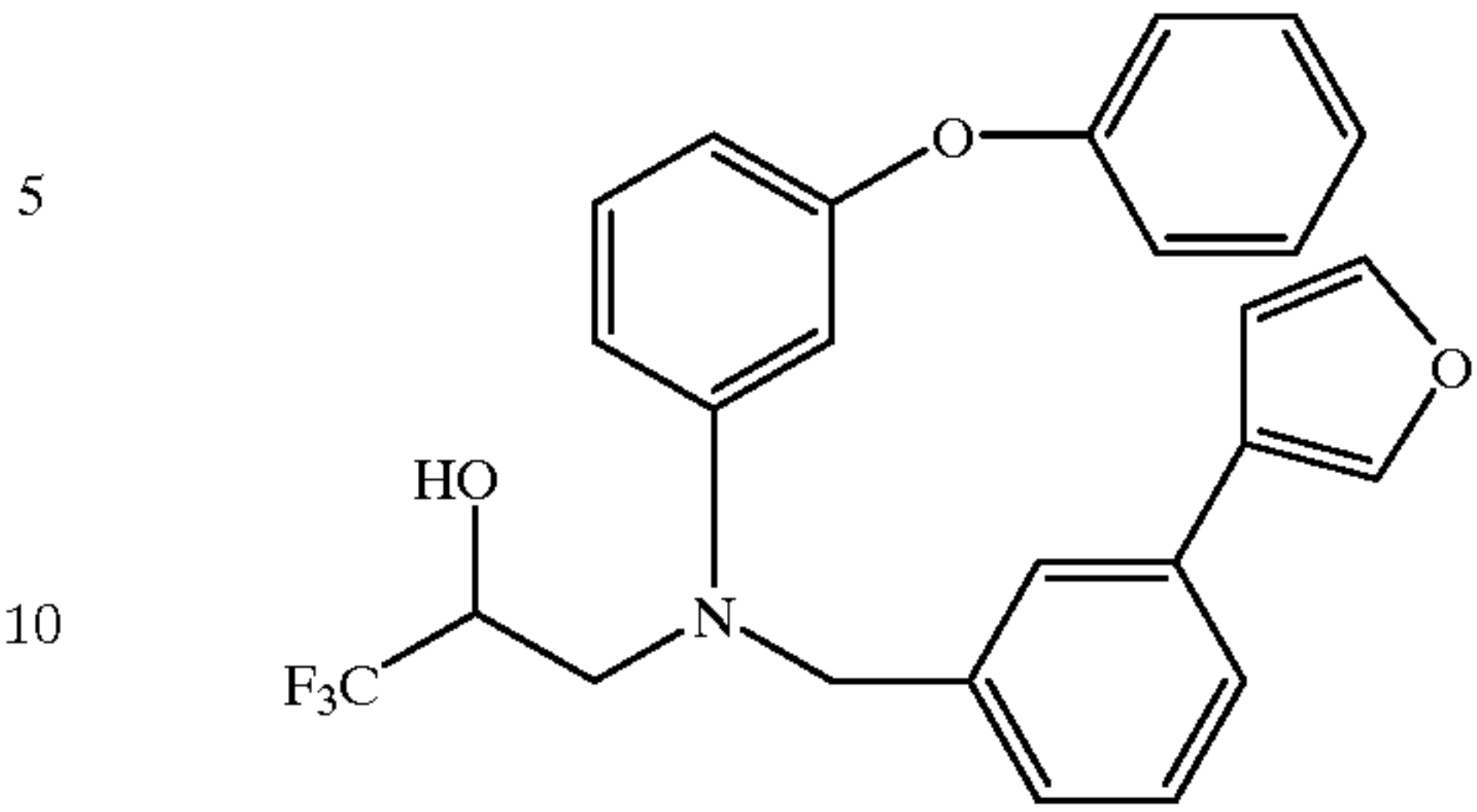
Example Table 35. 3-[(3-phenoxyphenyl)[[3-(alkyl- or cycloalkyl-)phenyl]methyl]amino]-1,1,1-trifluoro-2-propanols.
