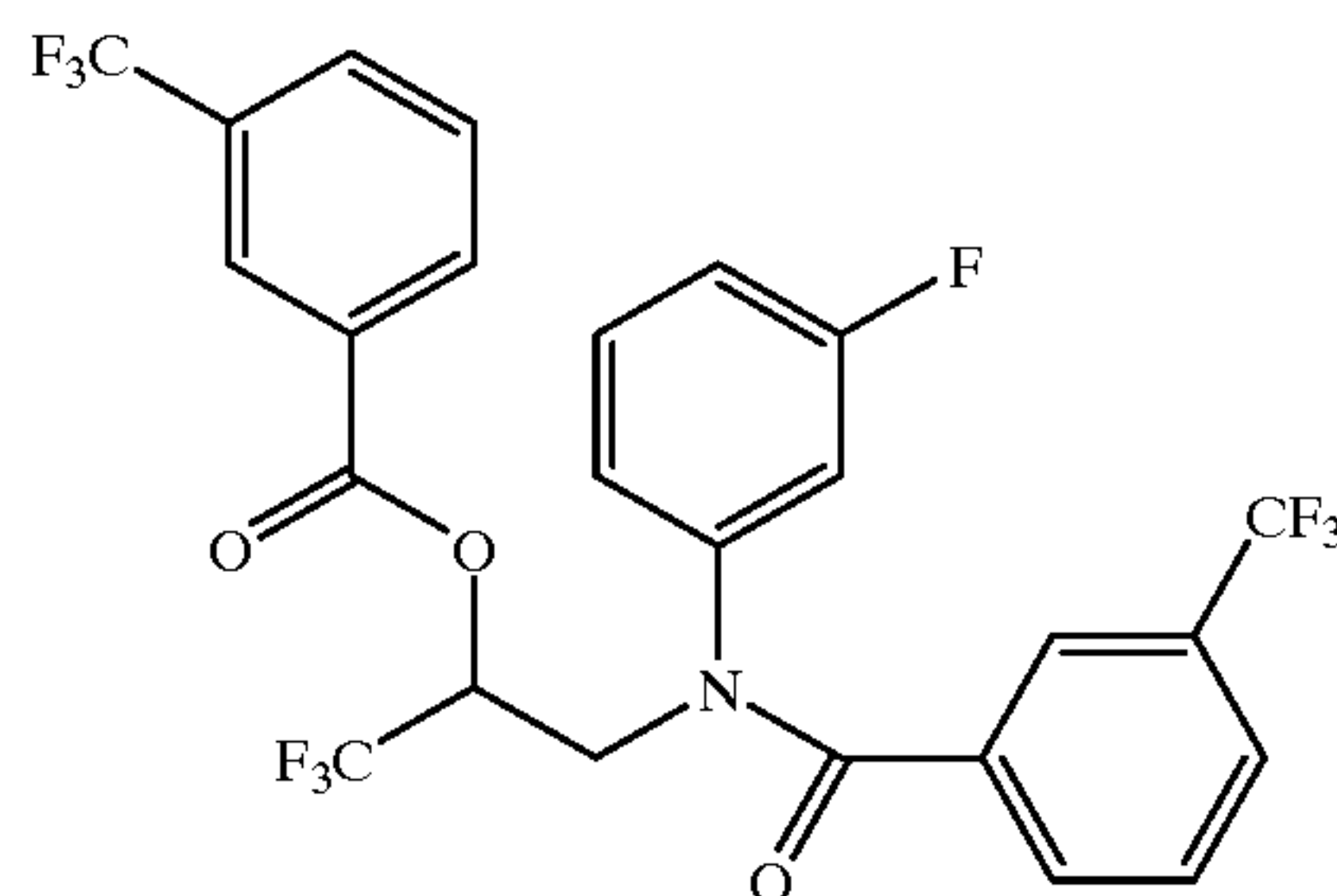
2,2,2-trifluoro-1-[[3-(3-fluorophenyl)[3-(trifluoromethyl)benzoyl]amino]-methyl]ethyl 3-trifluoromethylbenzoate
