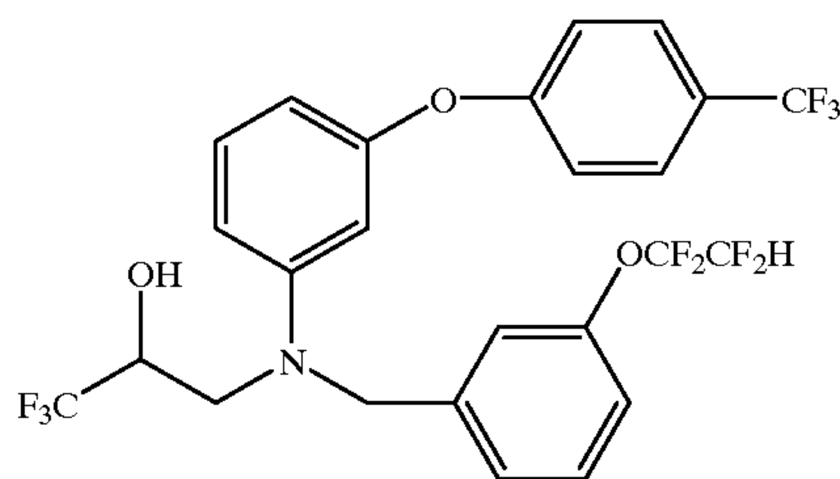
3-[[[3-(4-trifluoromethylphenoxy)phenyl][[3-(1,1,2,2-tetrafluoroethoxy)-phenyl]methyl]amino]-1,1,1-trifluoro-2-propanol
