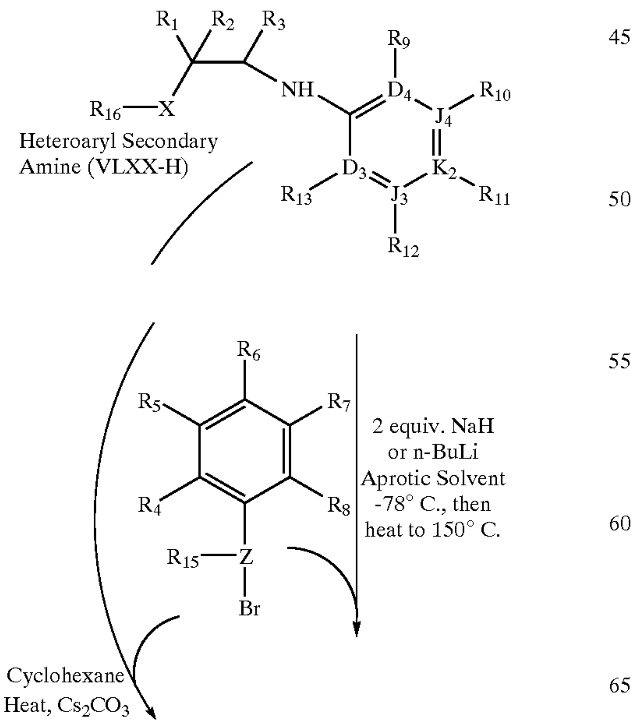
Scheme 52
