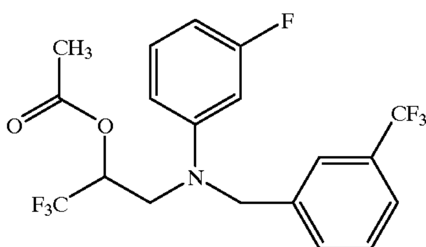
2,2,2-trifluoro-1-[[[3-(3-fluorophenyl)[3-(trifluoromethyl)phenyl]-methyl]amino]methyl]ethyl acetate
