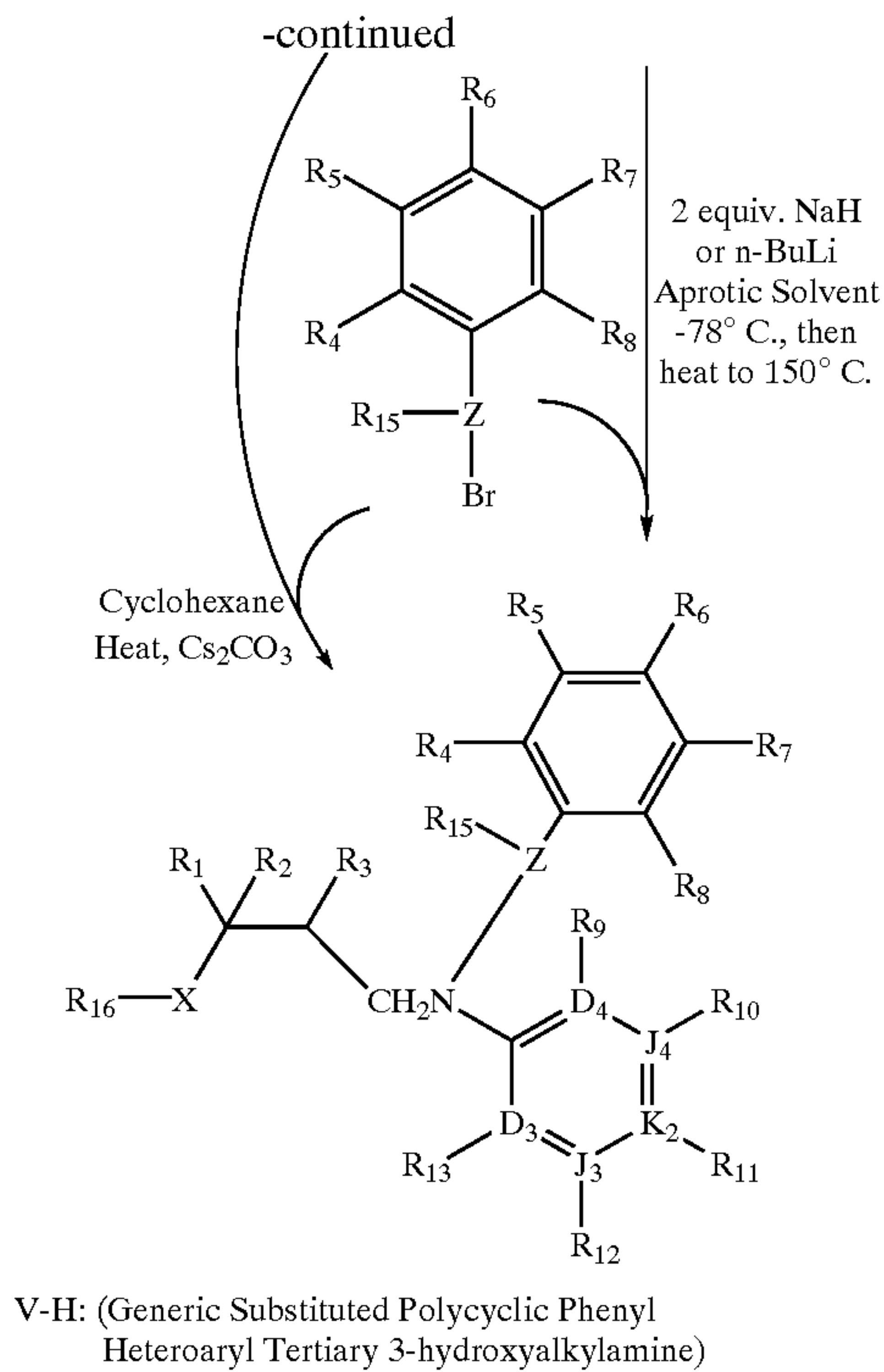
Scheme 55
