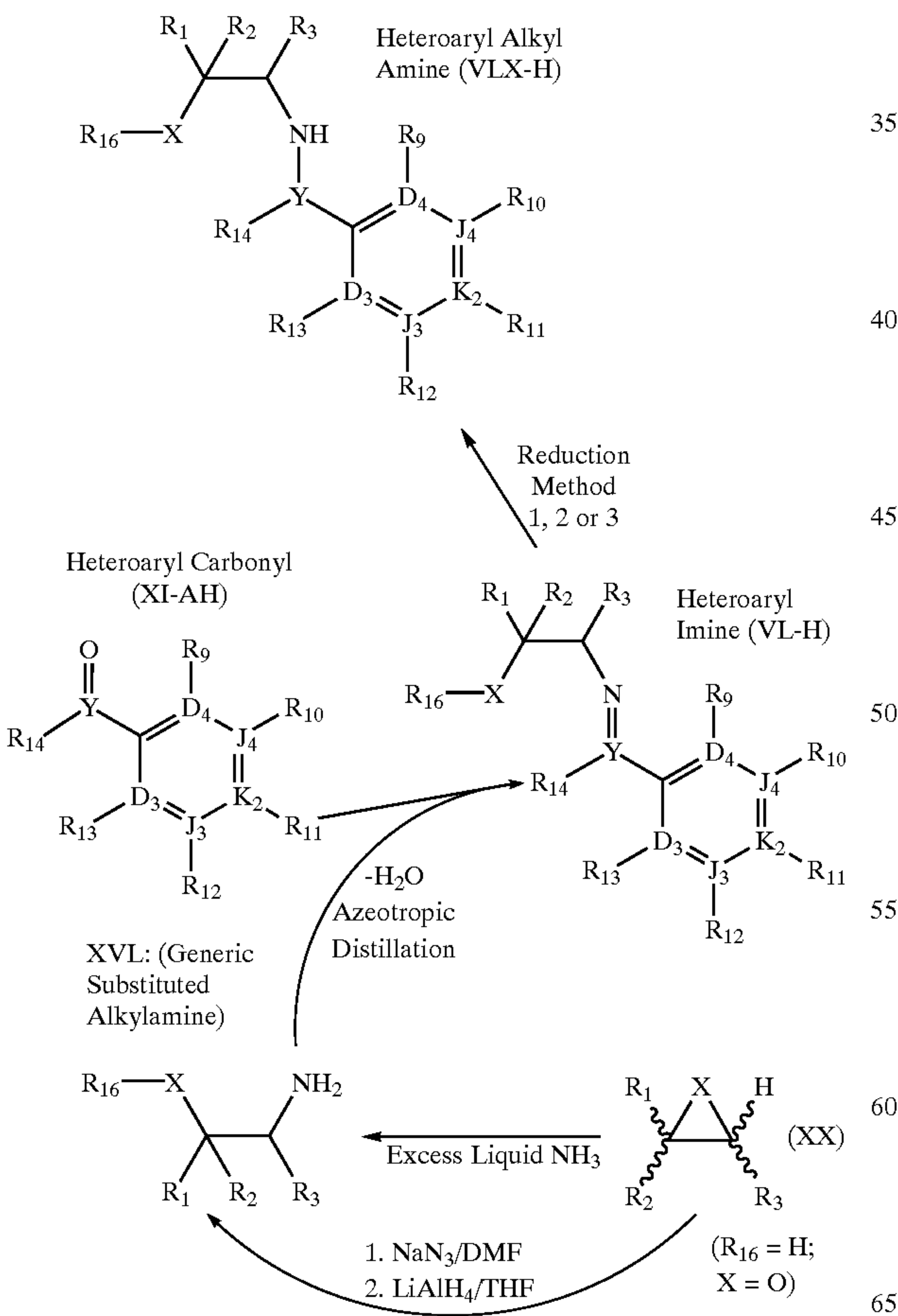
Scheme 45
