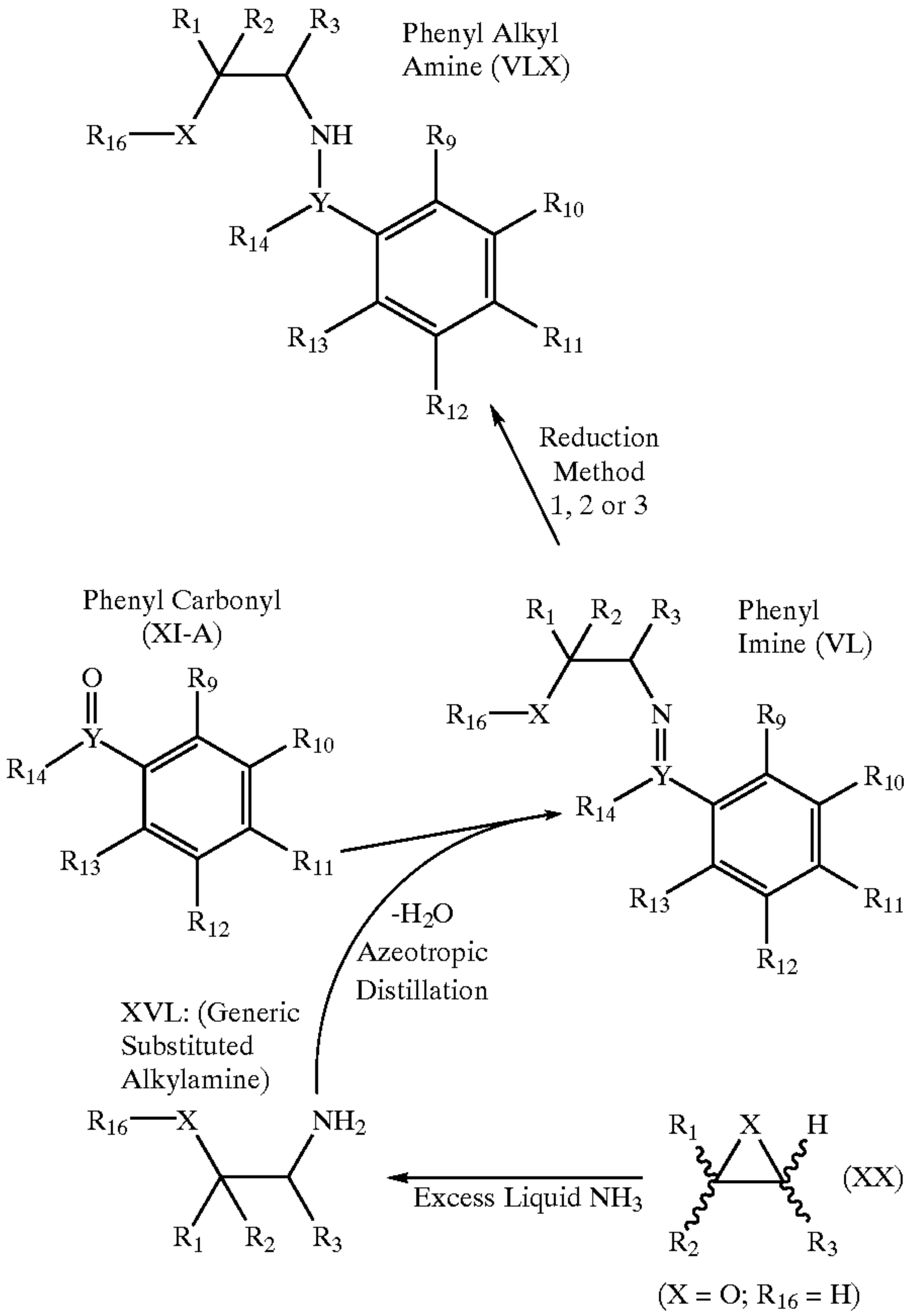
Scheme 48
