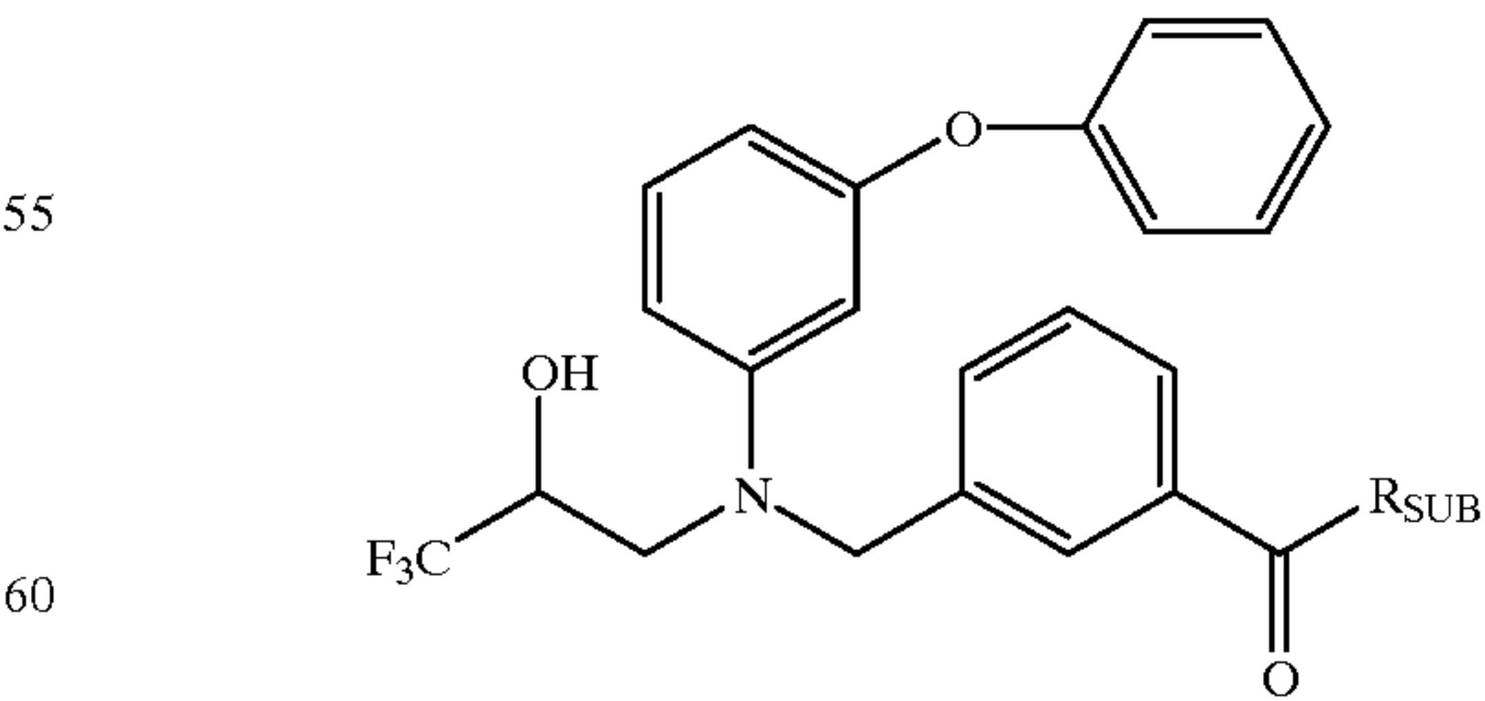
Example Table 37. 1-[3-[[[(3-phenoxyphenyl)(3,3,3-trifluoro-2-hydroxy-propyl)amino]methyl]-phenyl]-1-alkanones.
