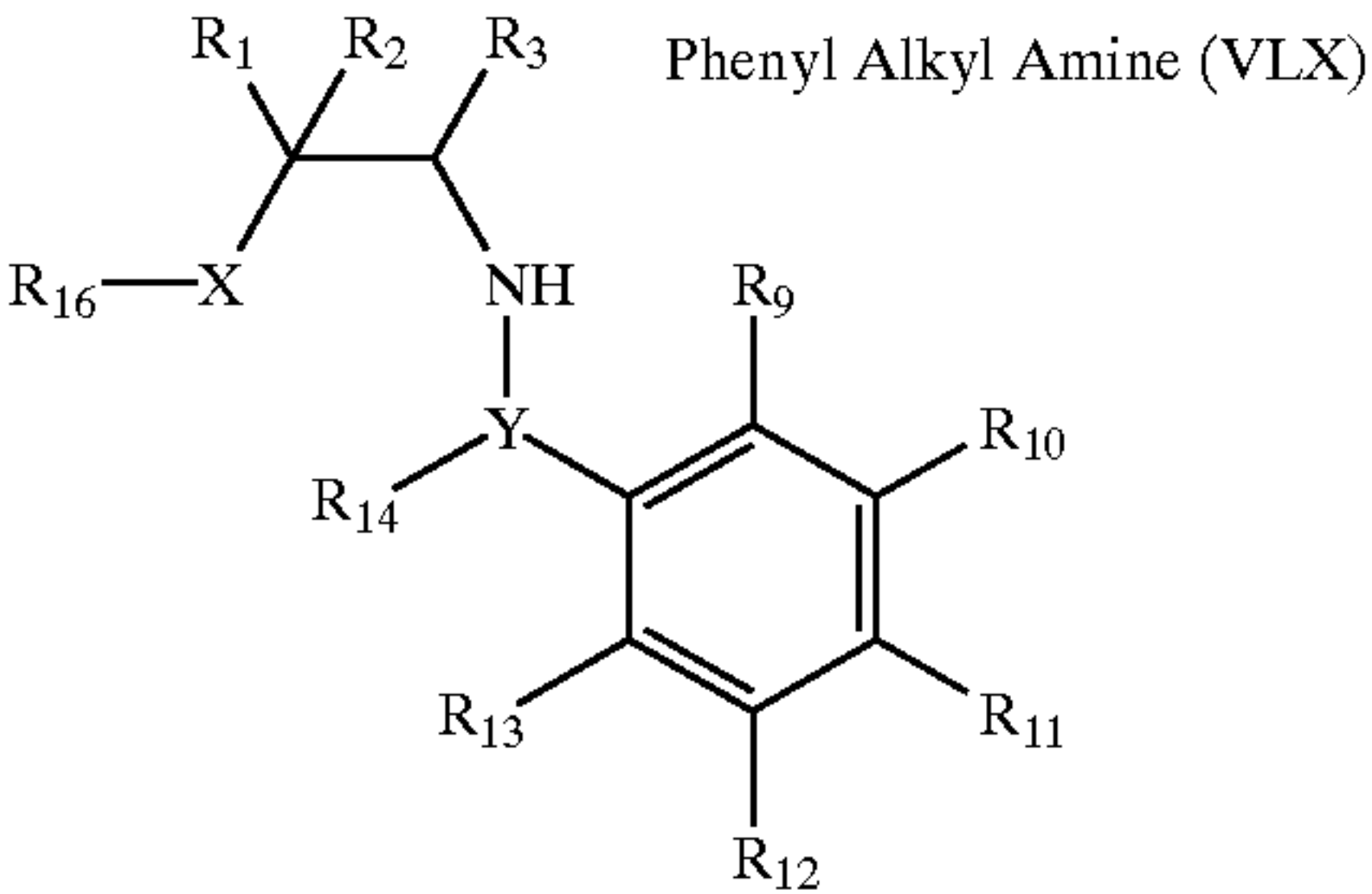
Scheme 49
