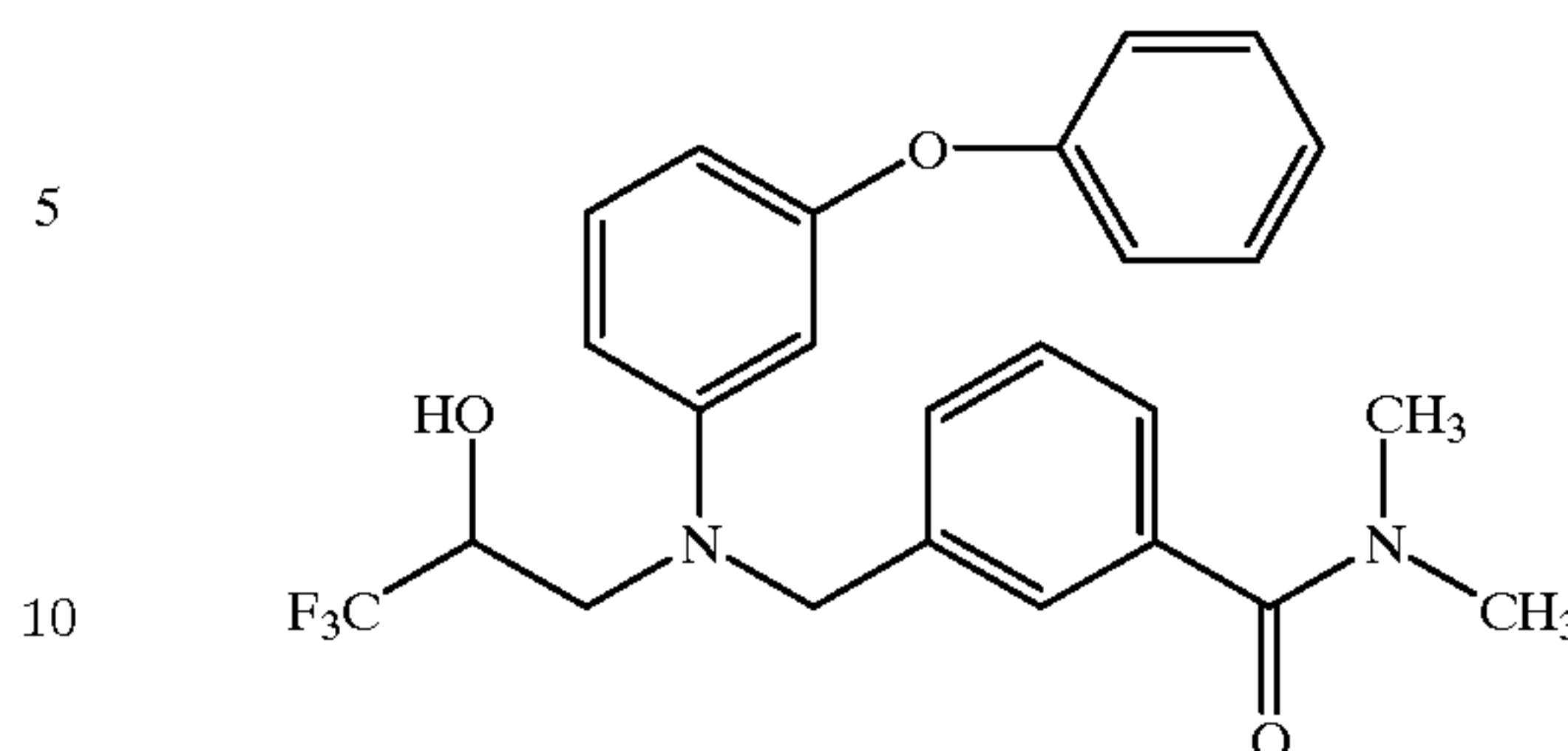
N,N-dimethyl-3-[[[(3-phenoxyphenyl)(3,3,3-trifluoro-2-hydroxypropyl)amino]methyl]benzamide
