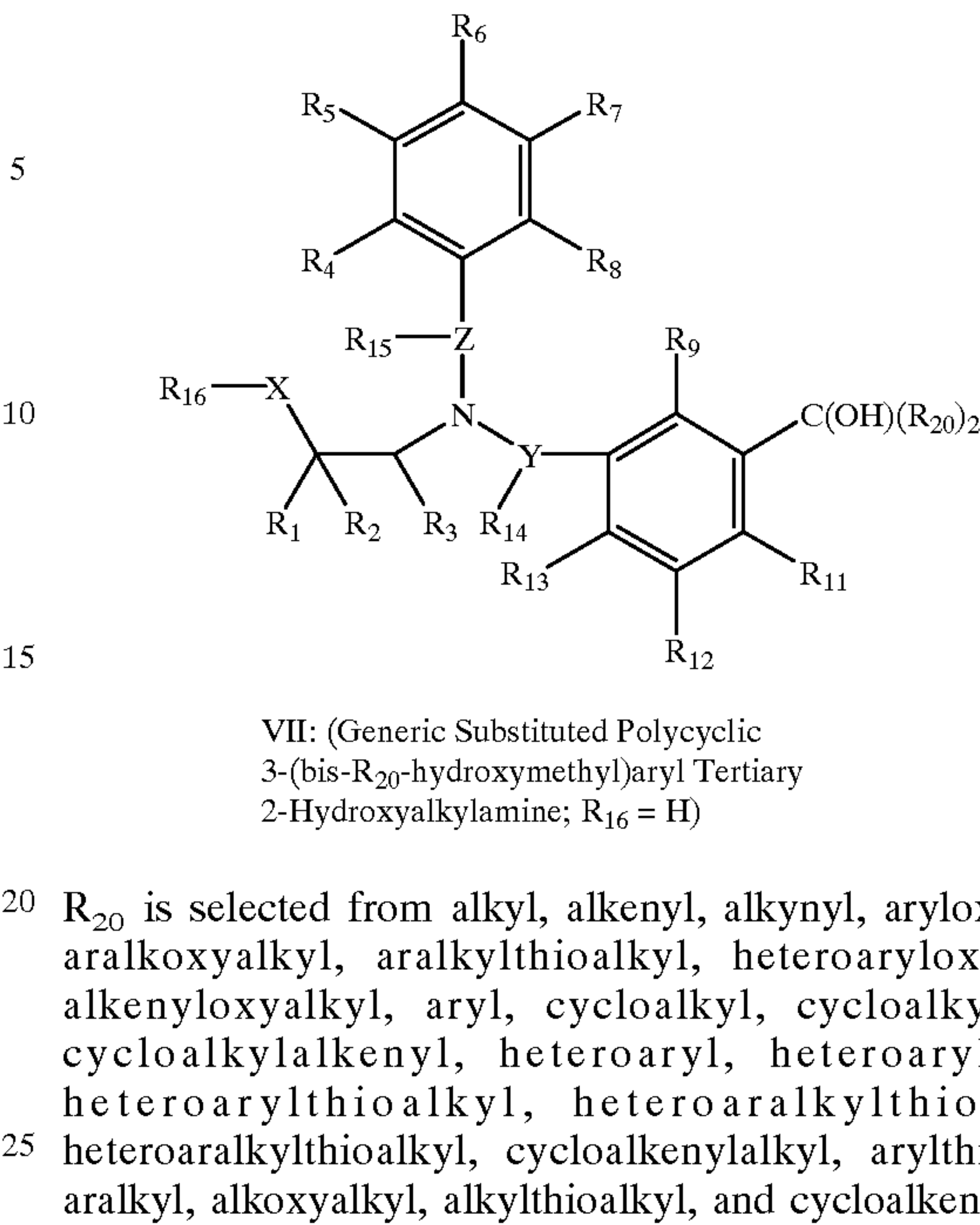
Scheme 38
