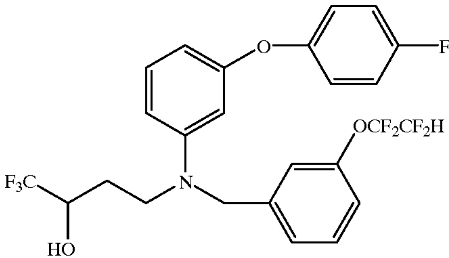
4-[[[3-(1,1,2,2-tetrafluoroethoxy)phenyl]methyl]amino]-1,1,1-trifluoro-2-butanol
