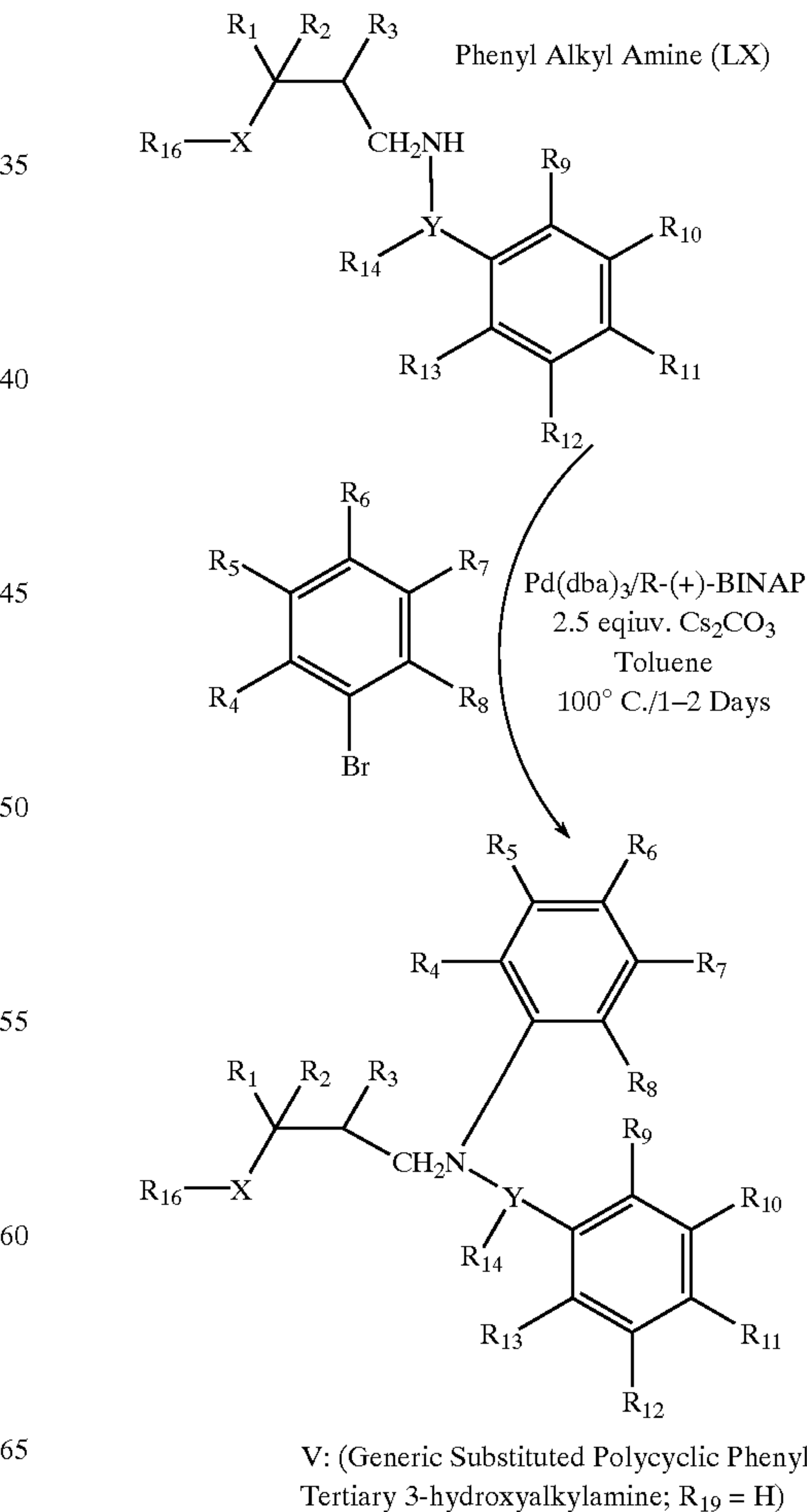
Scheme 35
