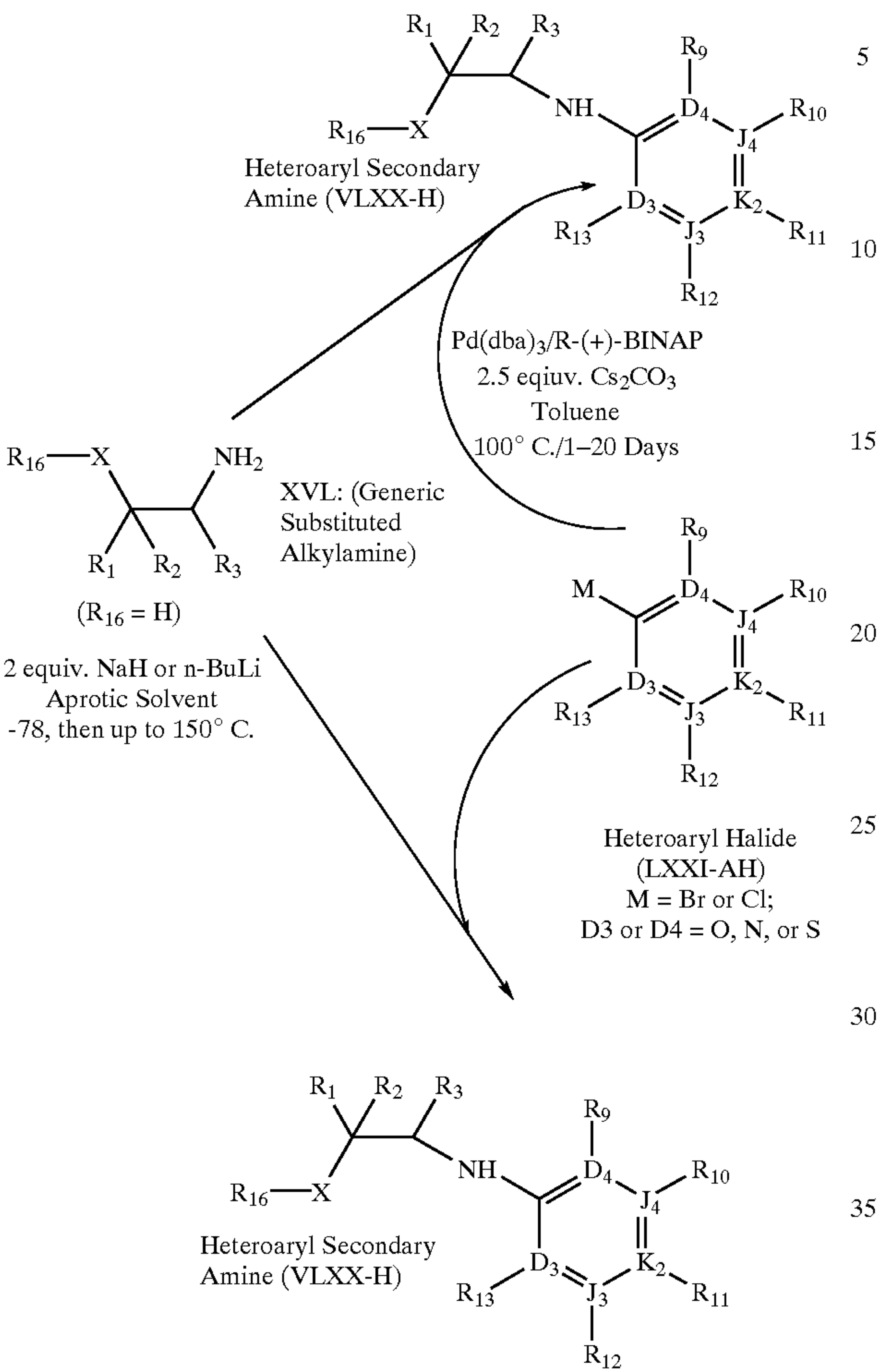
Scheme 51
