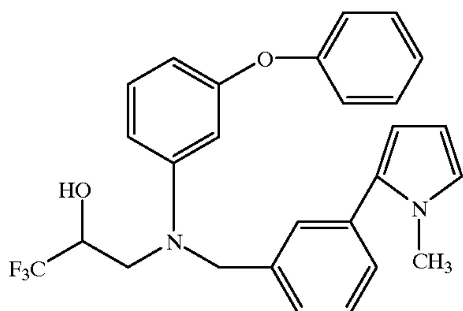
3-[(3-phenoxyphenyl)[[3-(1-methyl-1H-pyrrol-2-yl)phenyl]methyl]amino]-1,1,1-trifluoro-2-propanol
