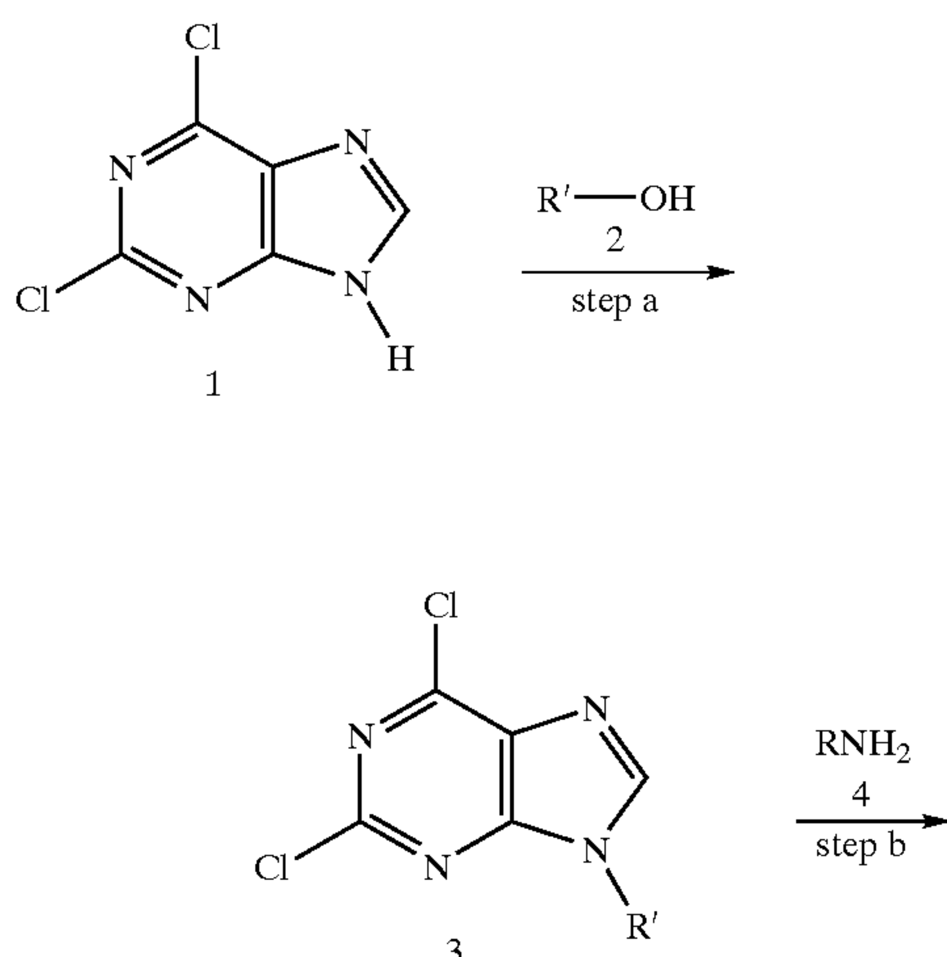
Scheme A
