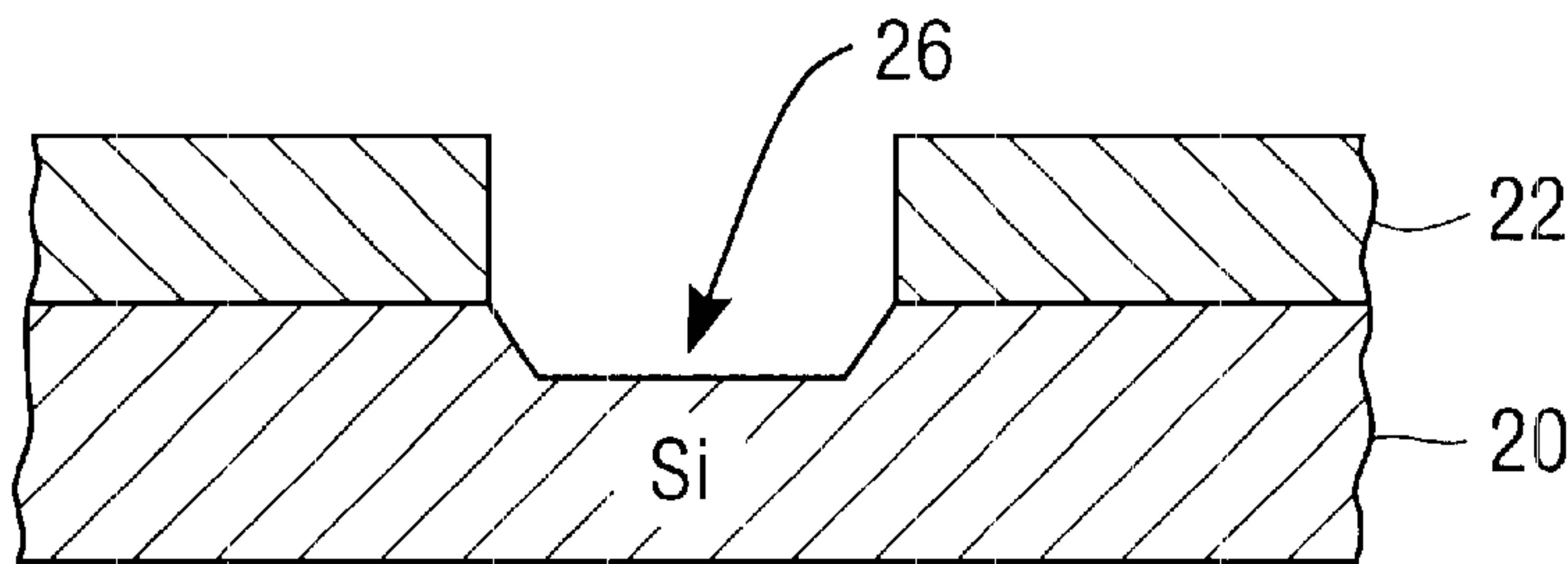
FIG. 2C (Prior Art)
