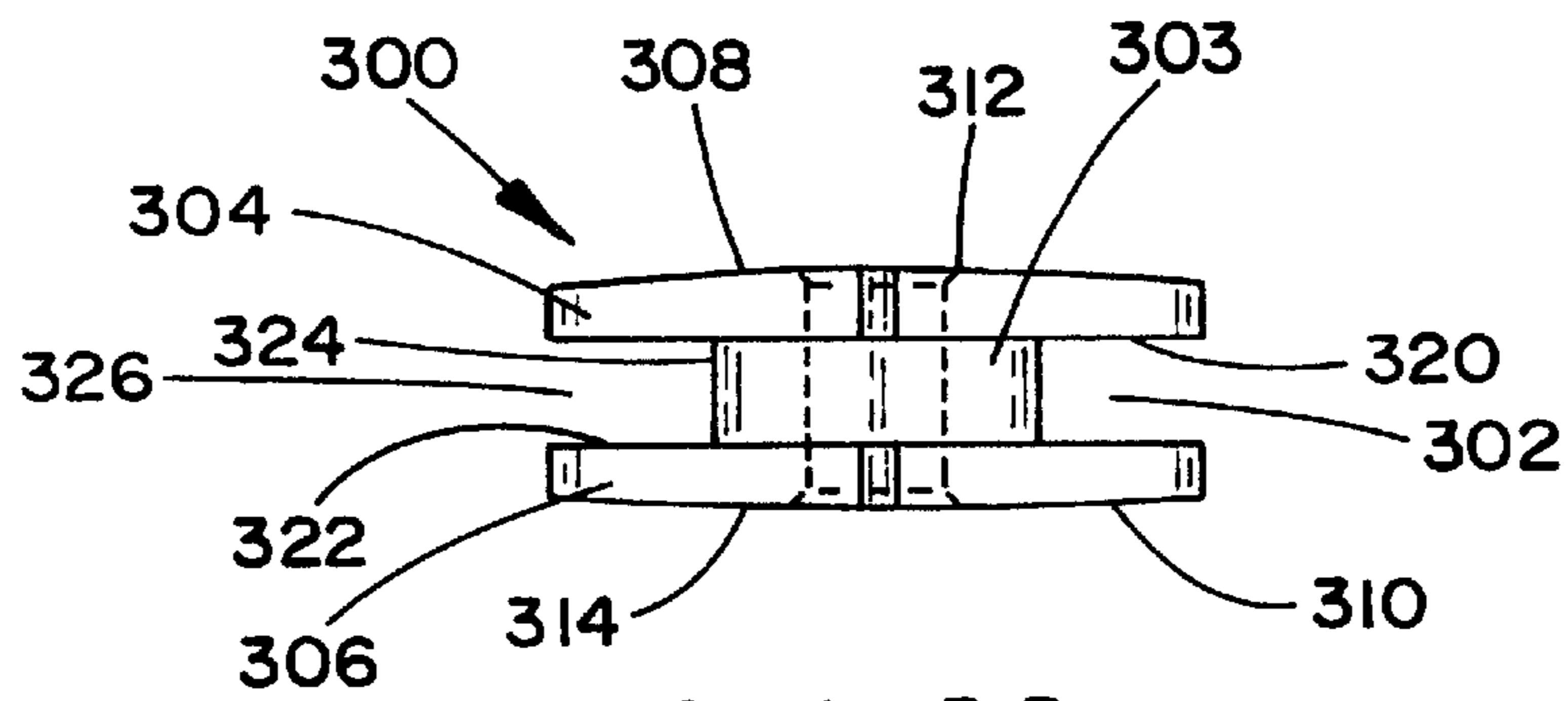
Section B-B
