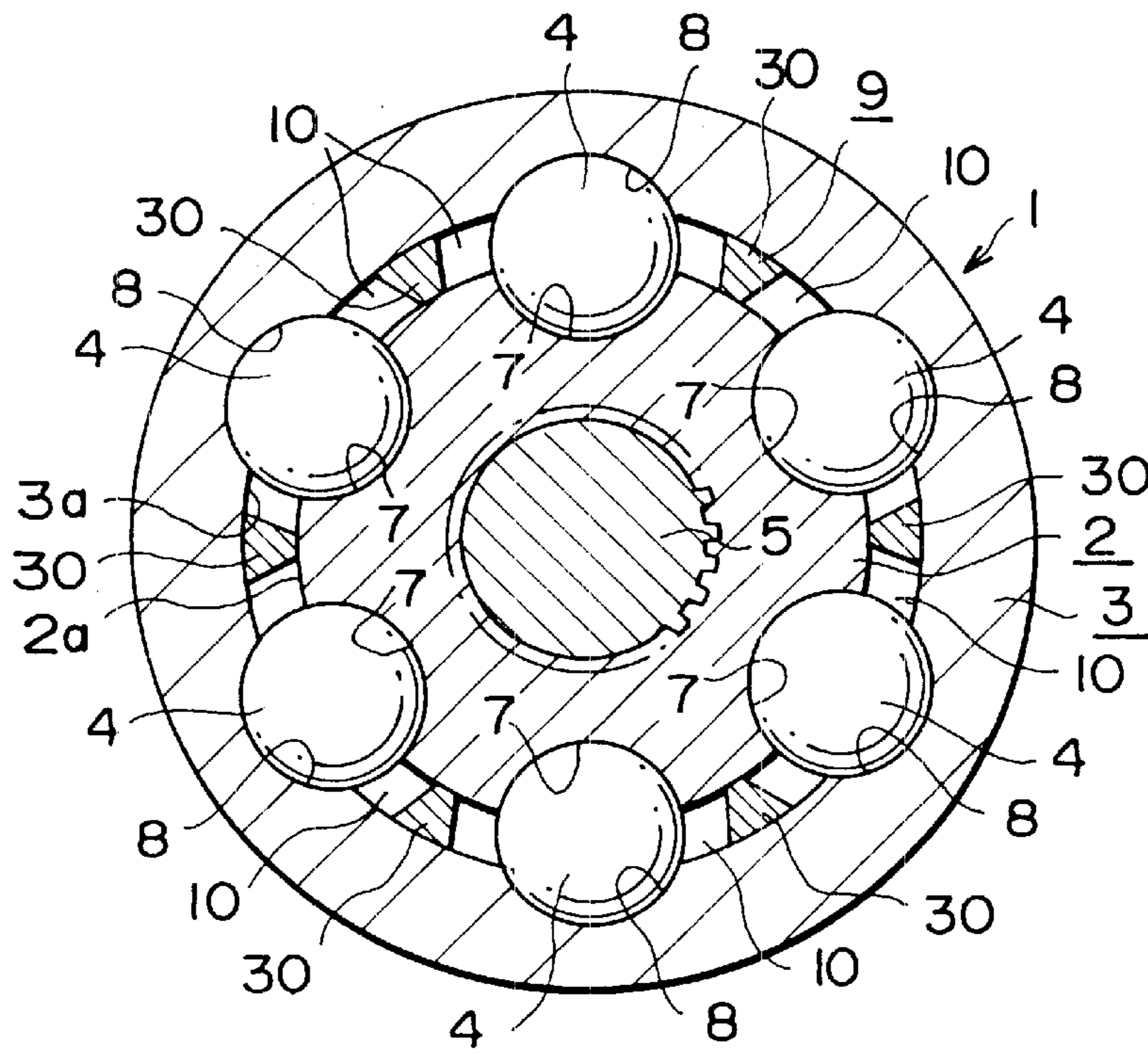
FIG. 22 PRIOR ART
