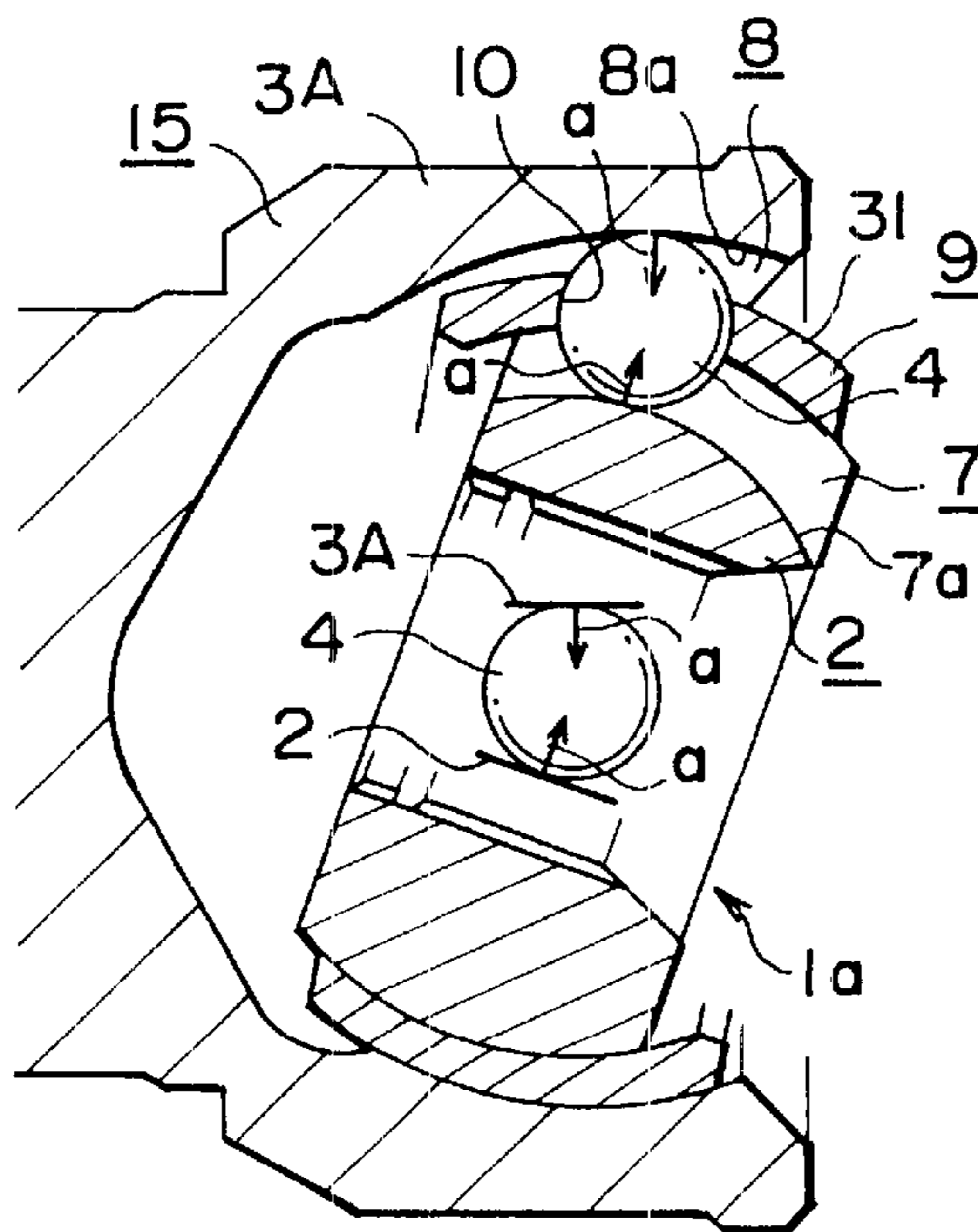
FIG. 26 PRIOR ART
