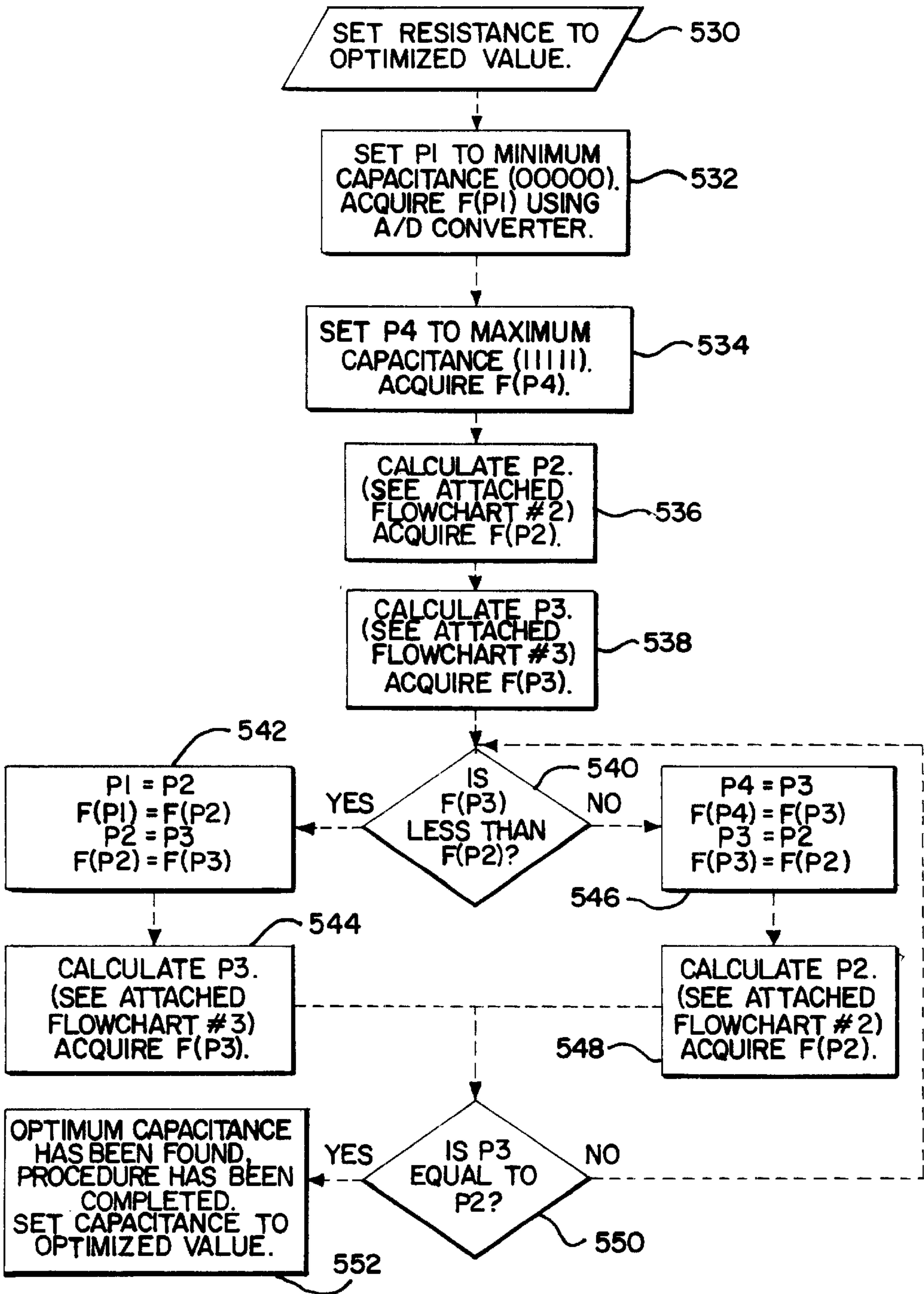
CAPACITANCE OPTIMIZATION FLOWCHART #4
