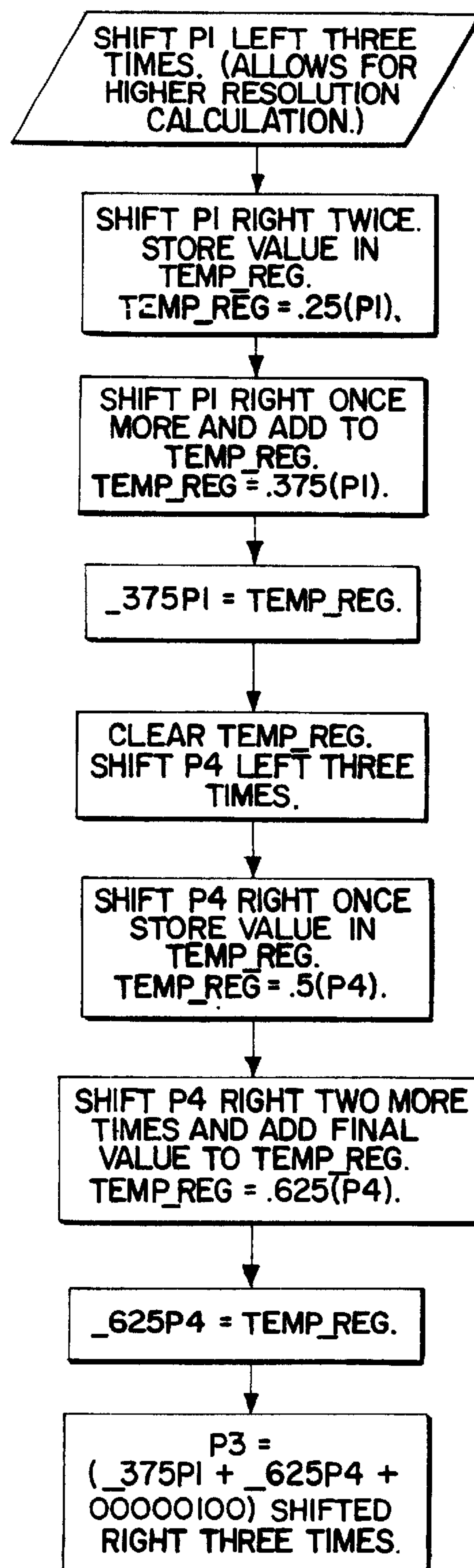
CALCULATION OF P3 FLOWCHART # 3
