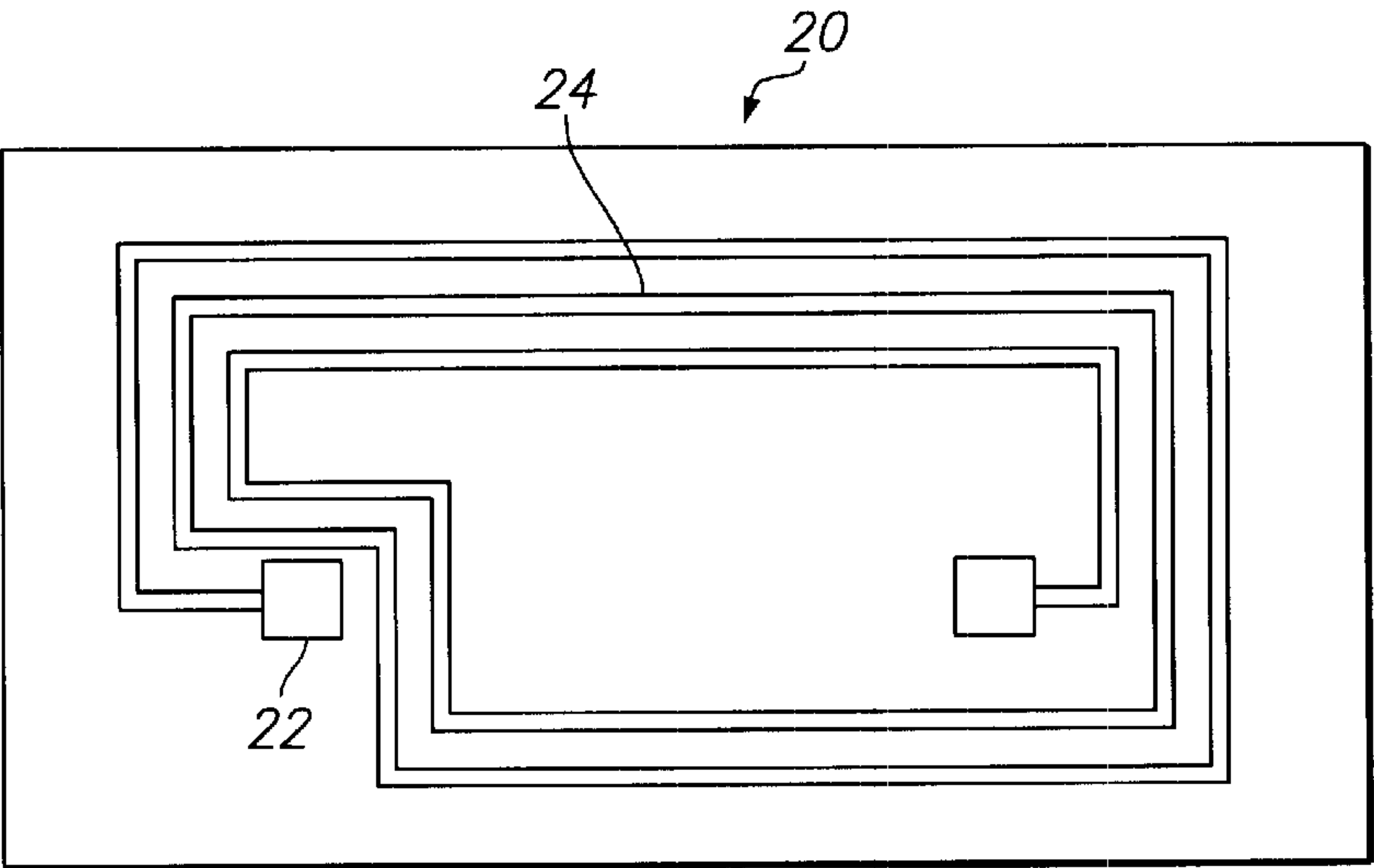
FIG. 1 (PRIOR ART)
