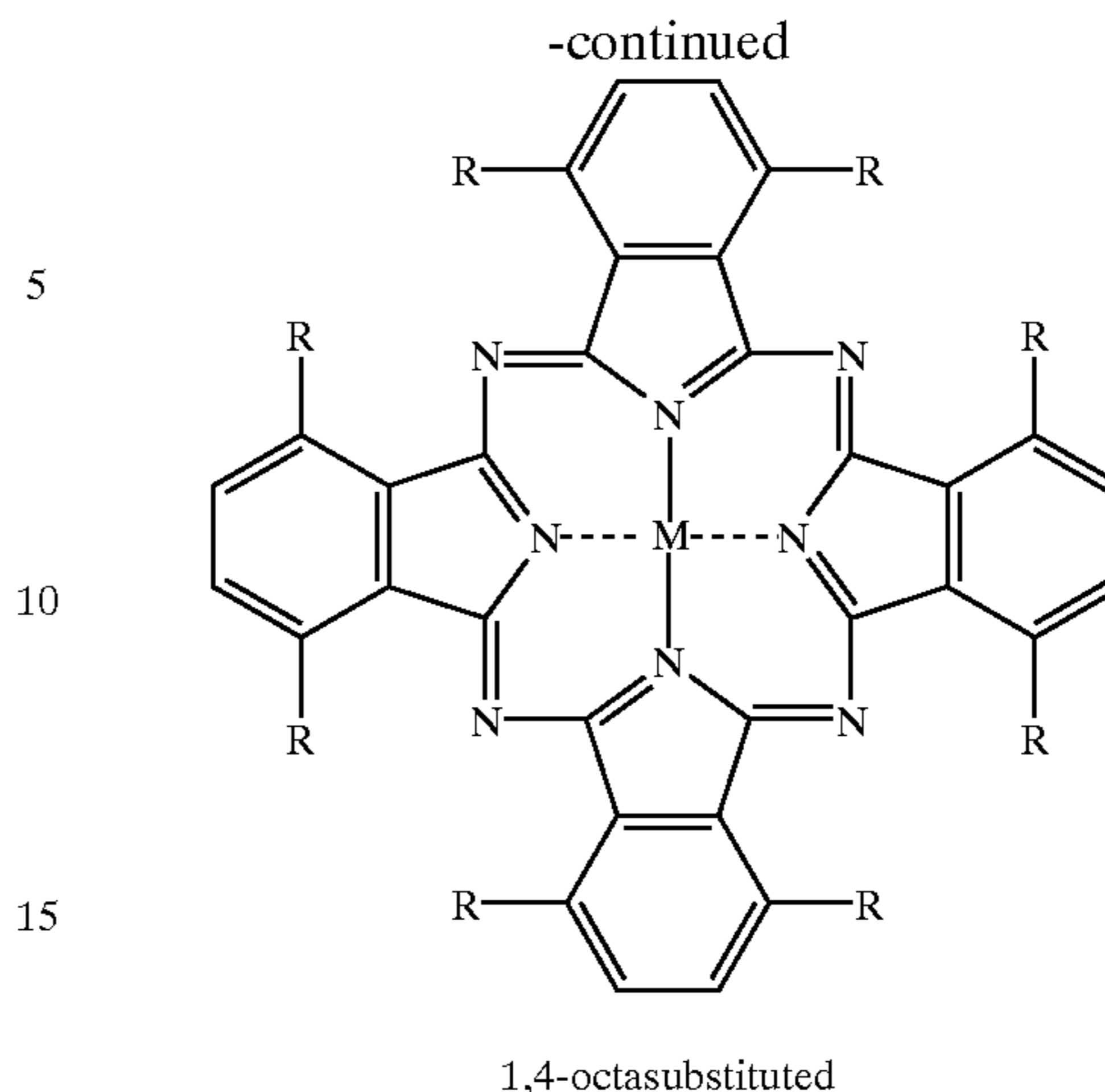
1,4-octasubstituted
