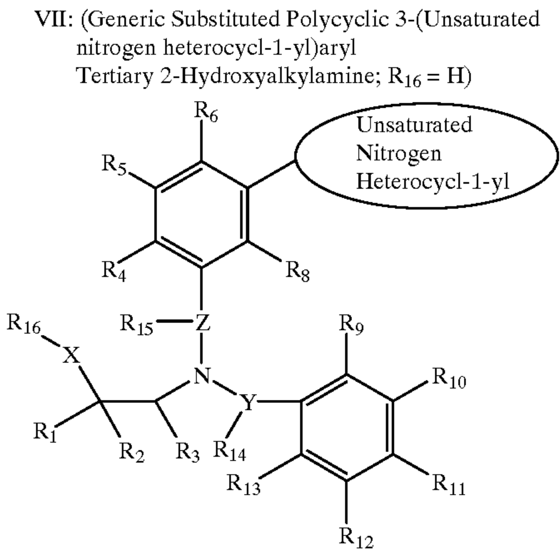
Scheme 26
