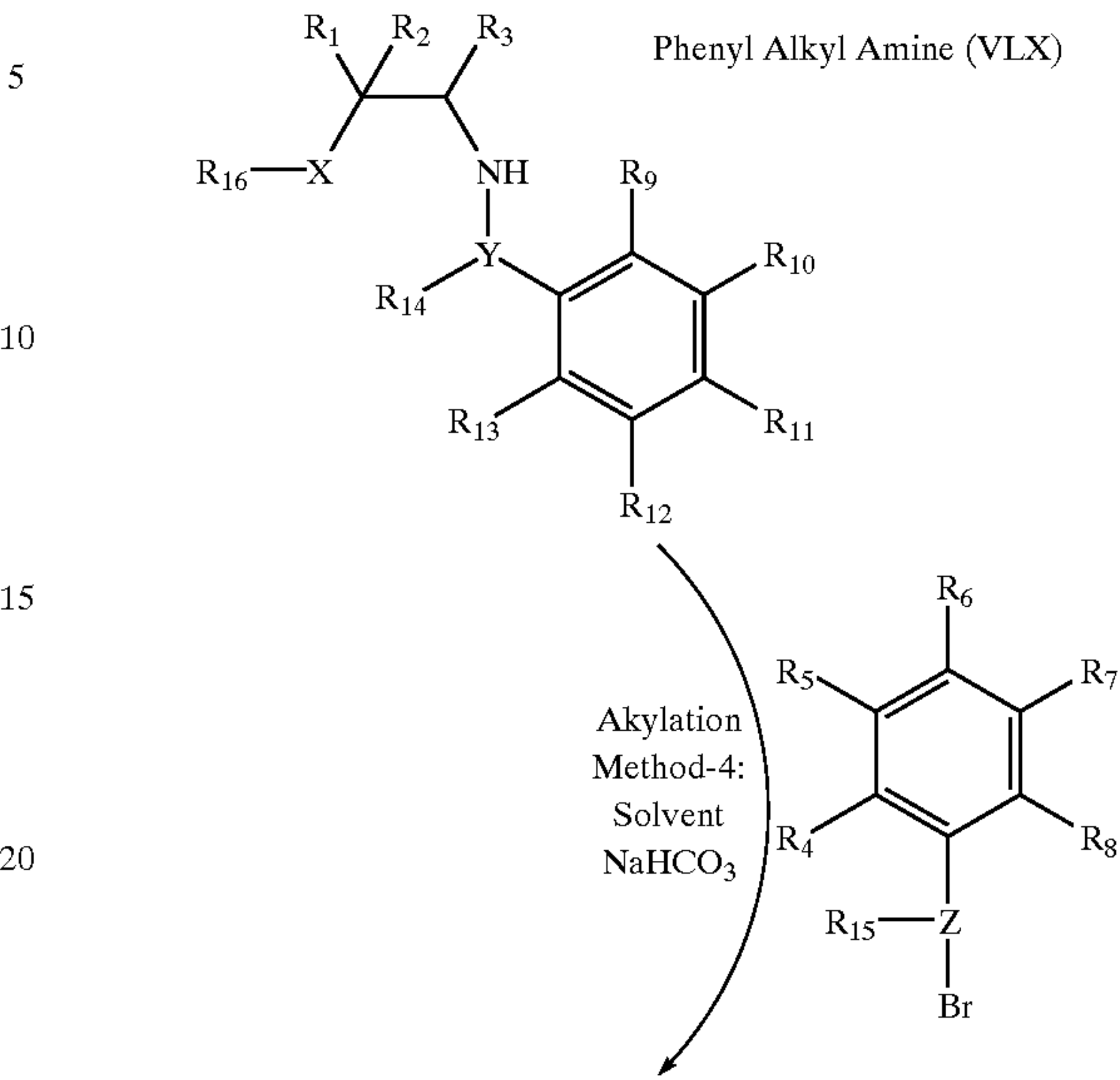
Scheme 49
