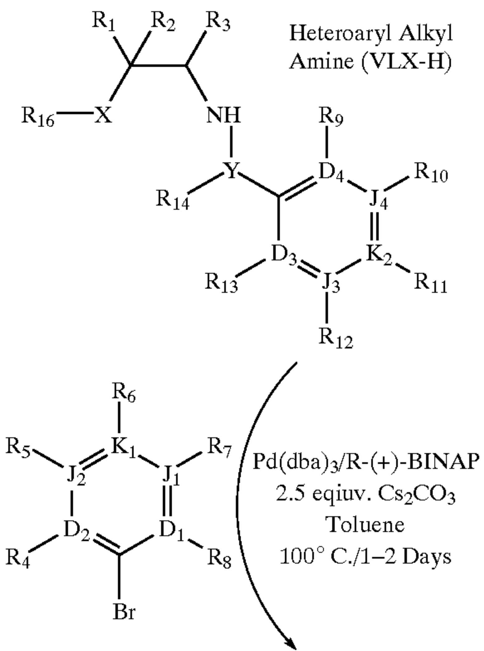
Scheme 47
