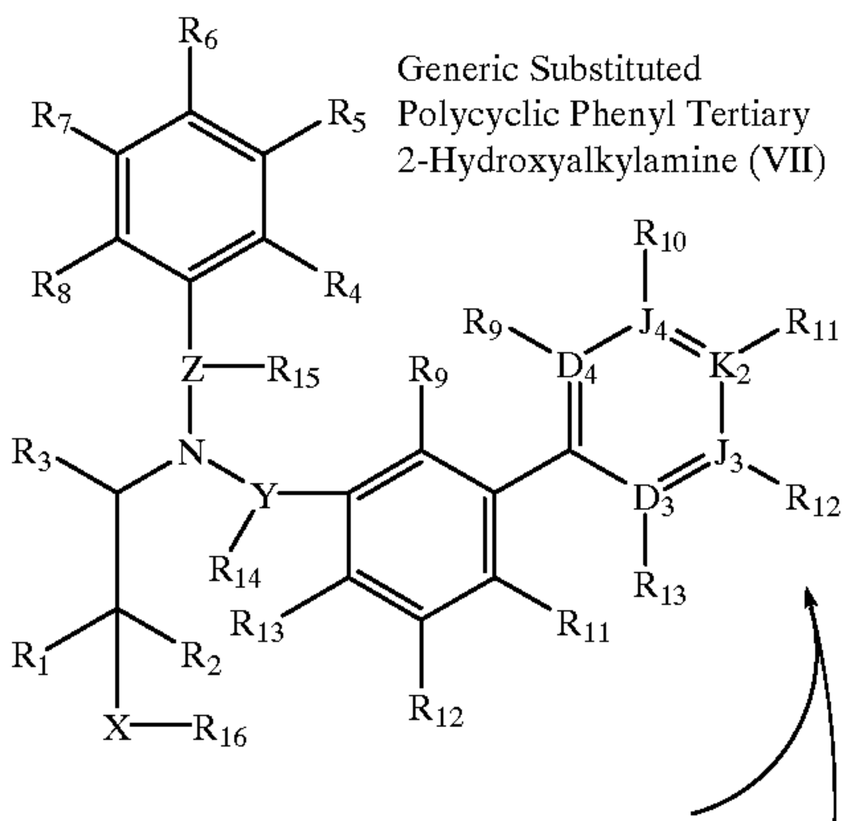
Scheme 56
