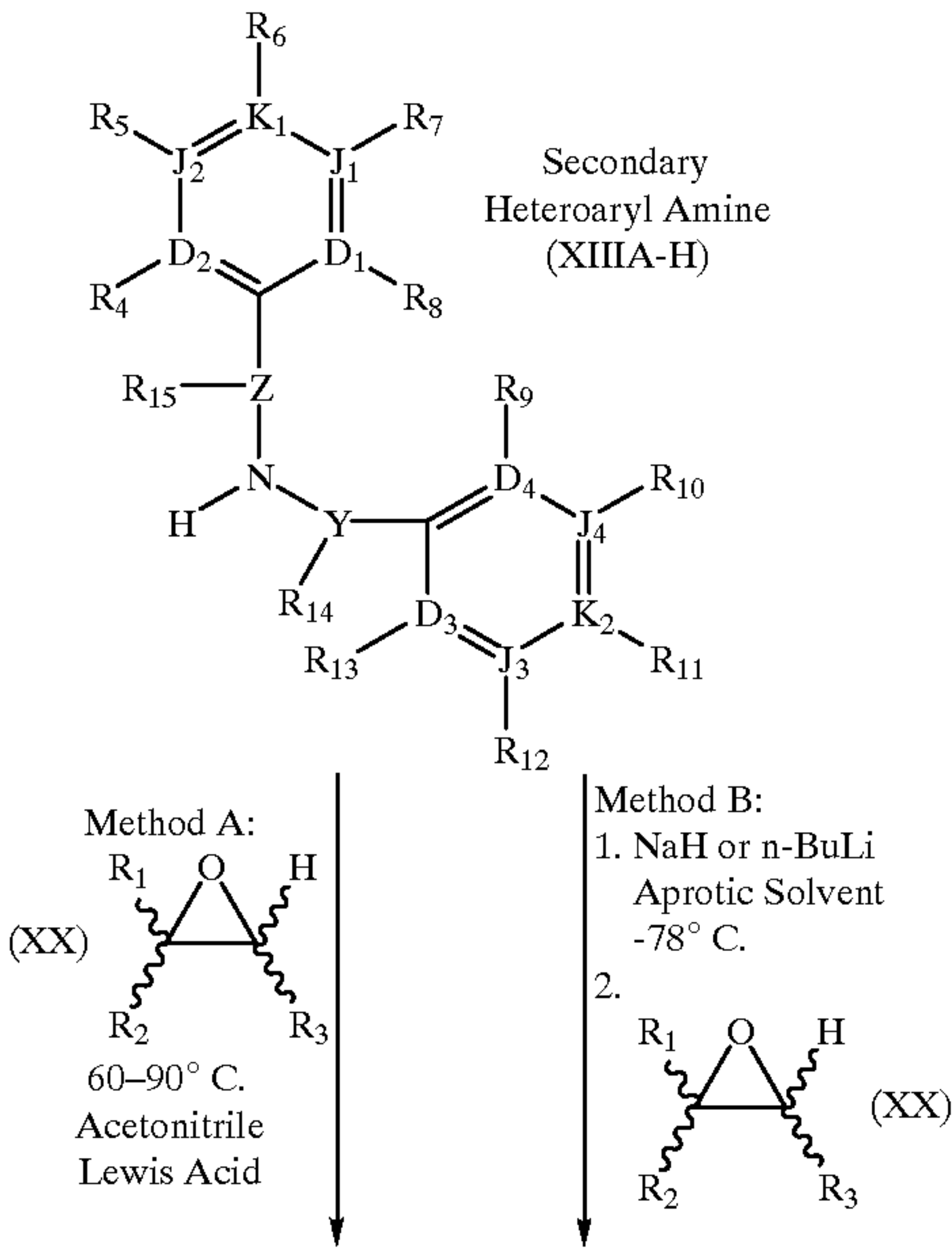
Scheme 7
