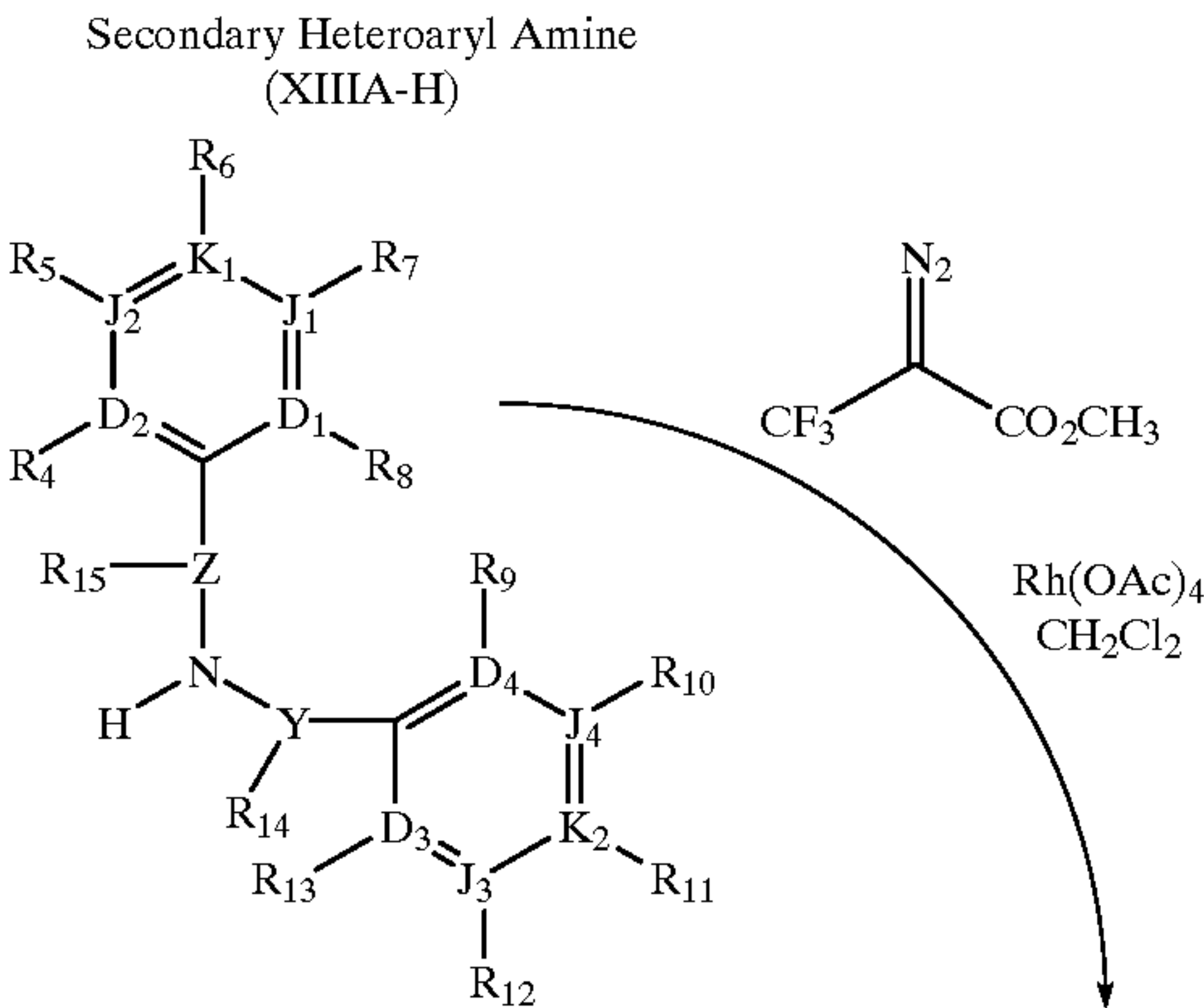
Scheme 57
