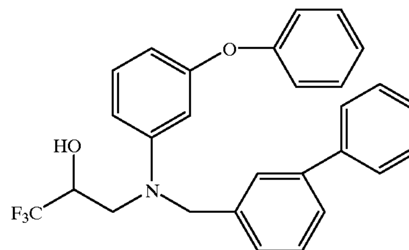
3-[(3-phenoxyphenyl)[[1,1'-biphenyl]-3-ylmethyl]amino]-1,1,1-trifluoro-2-propanol
