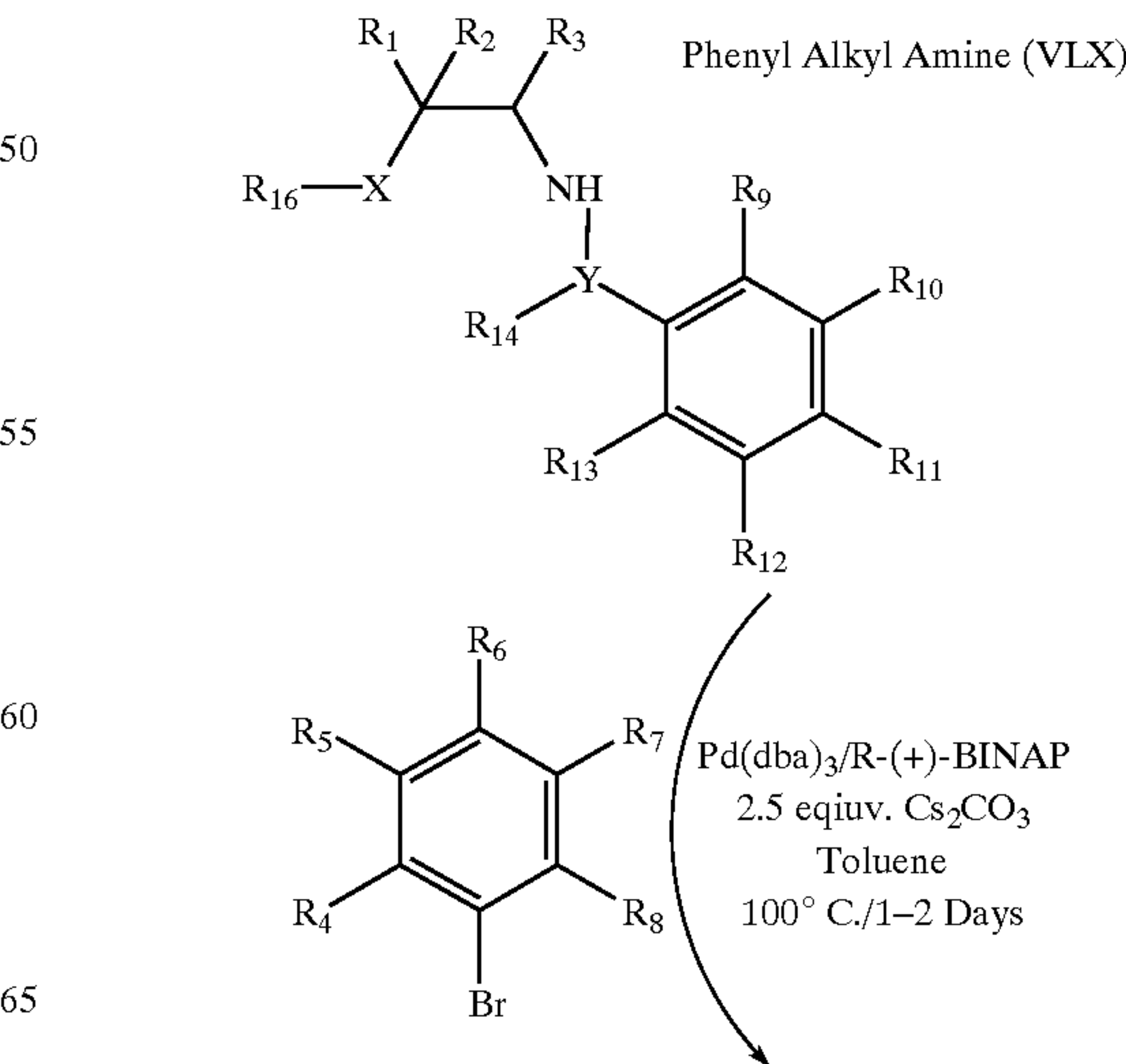
Scheme 50
