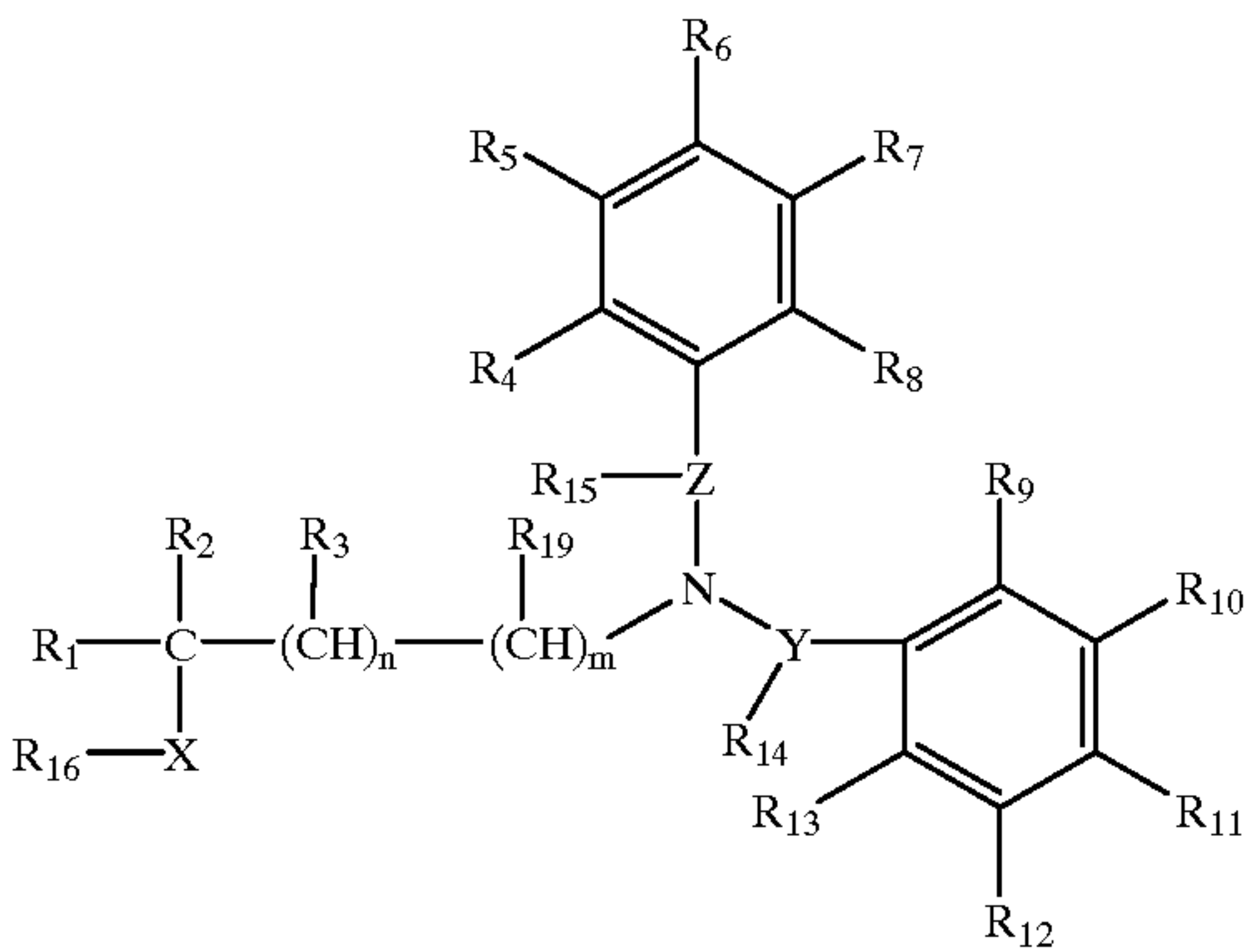
Scheme 5
