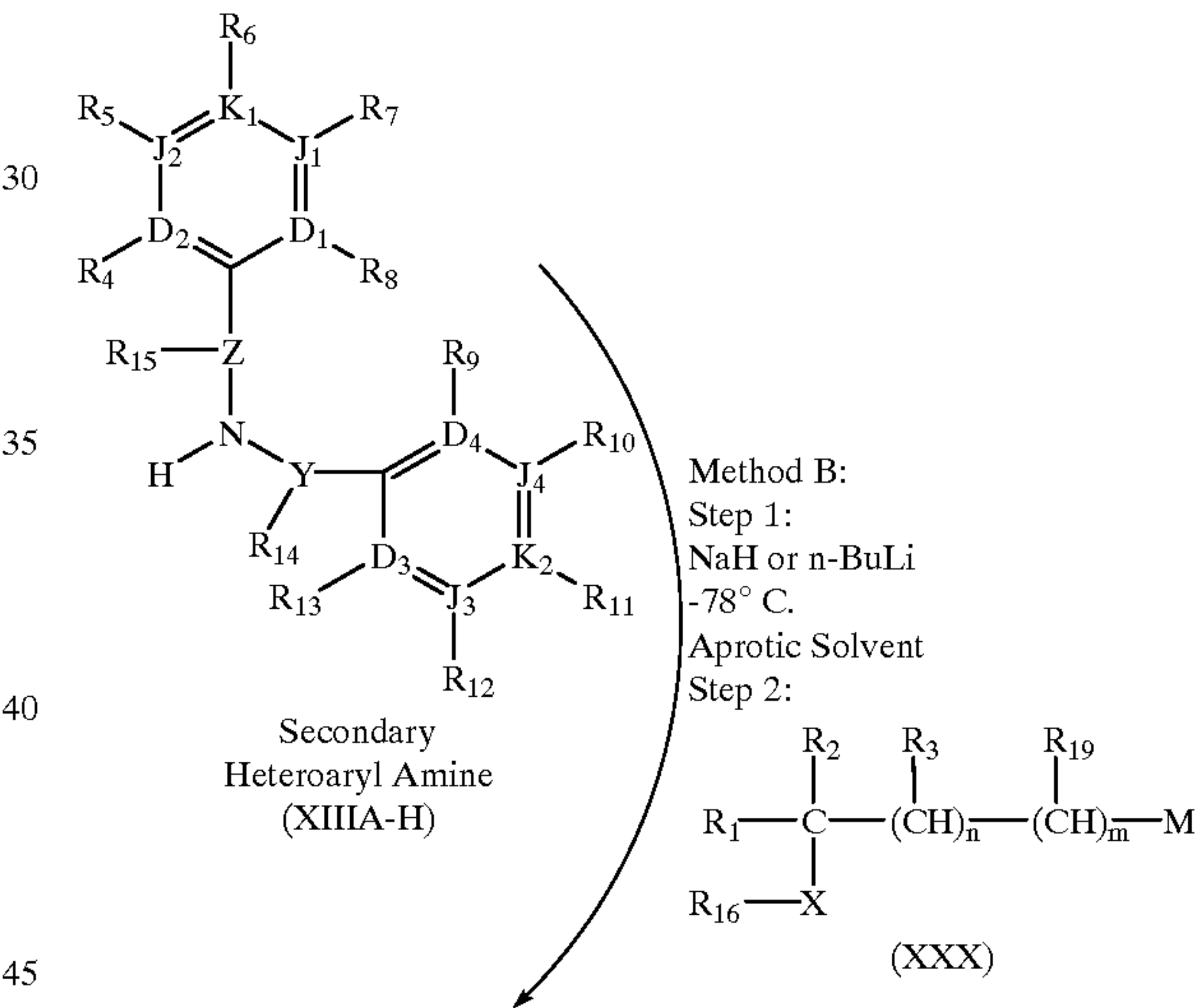
Scheme 6
