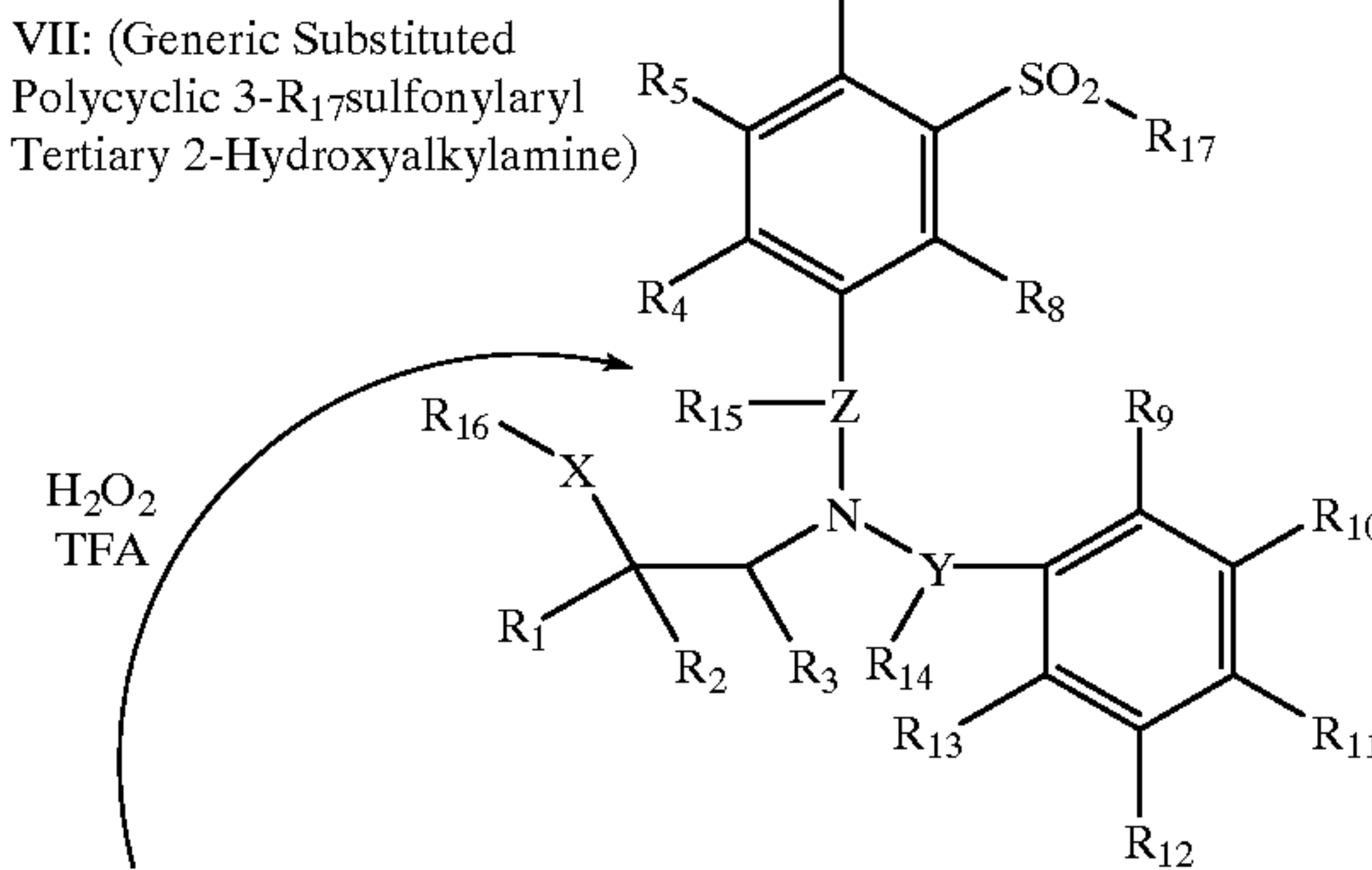
Scheme 19
