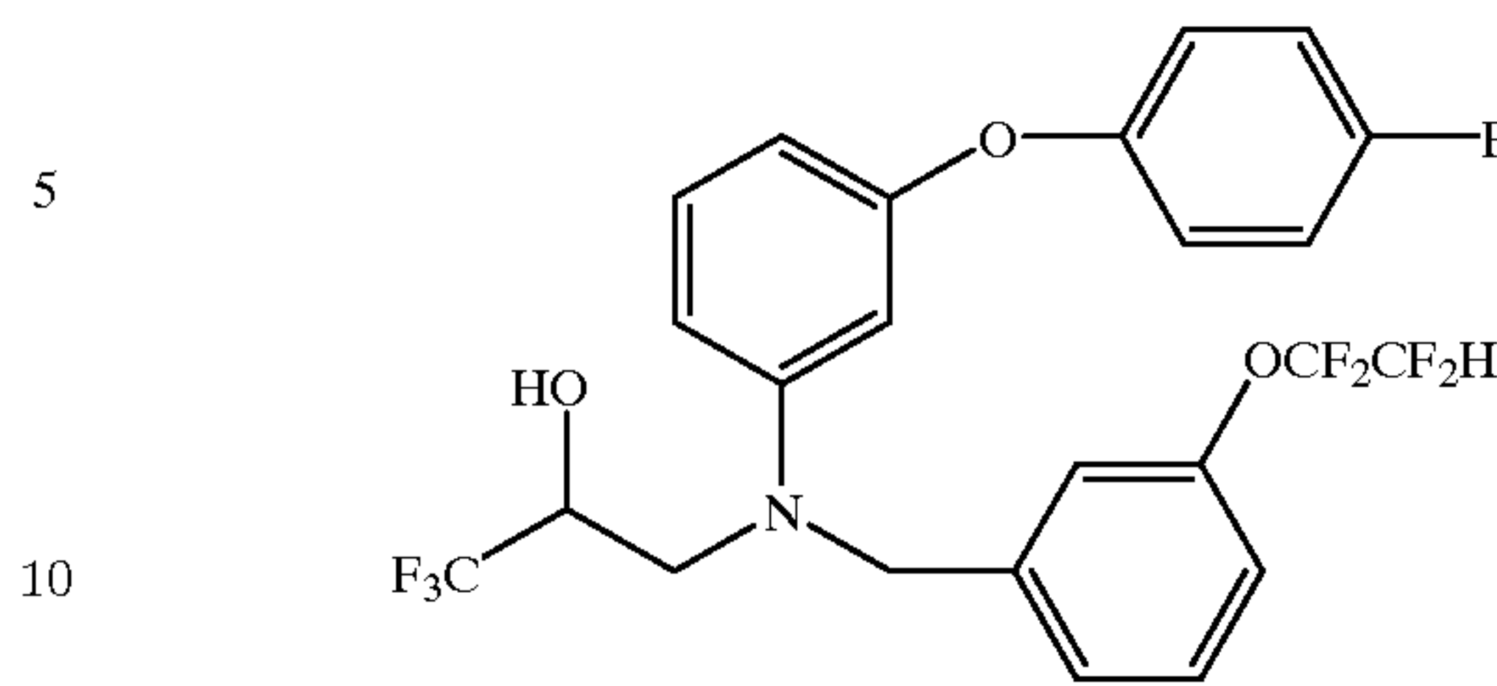
3-[[3-(4-fluorophenoxy)phenyl][[3-(1,1,2,2-tetrafluoroethoxy)phenyl]methyl]amino]-1,1,1-trifluoro-2-propanol
