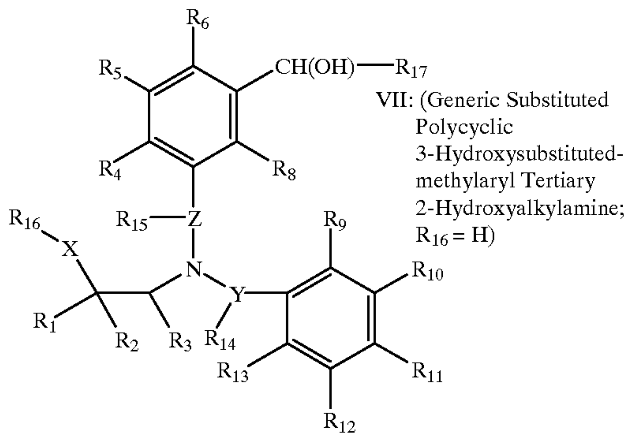
Scheme 29
