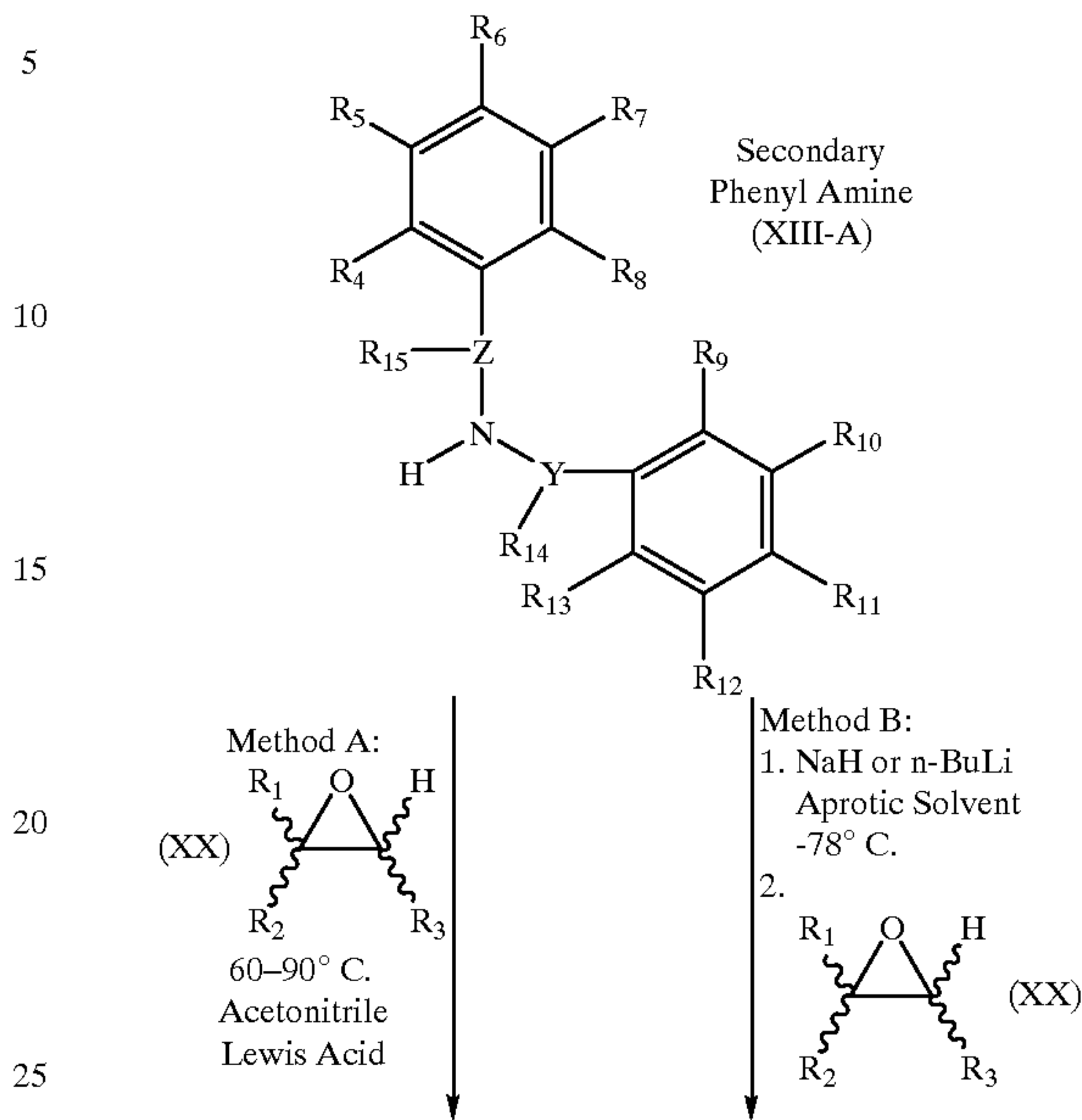
Scheme 11
