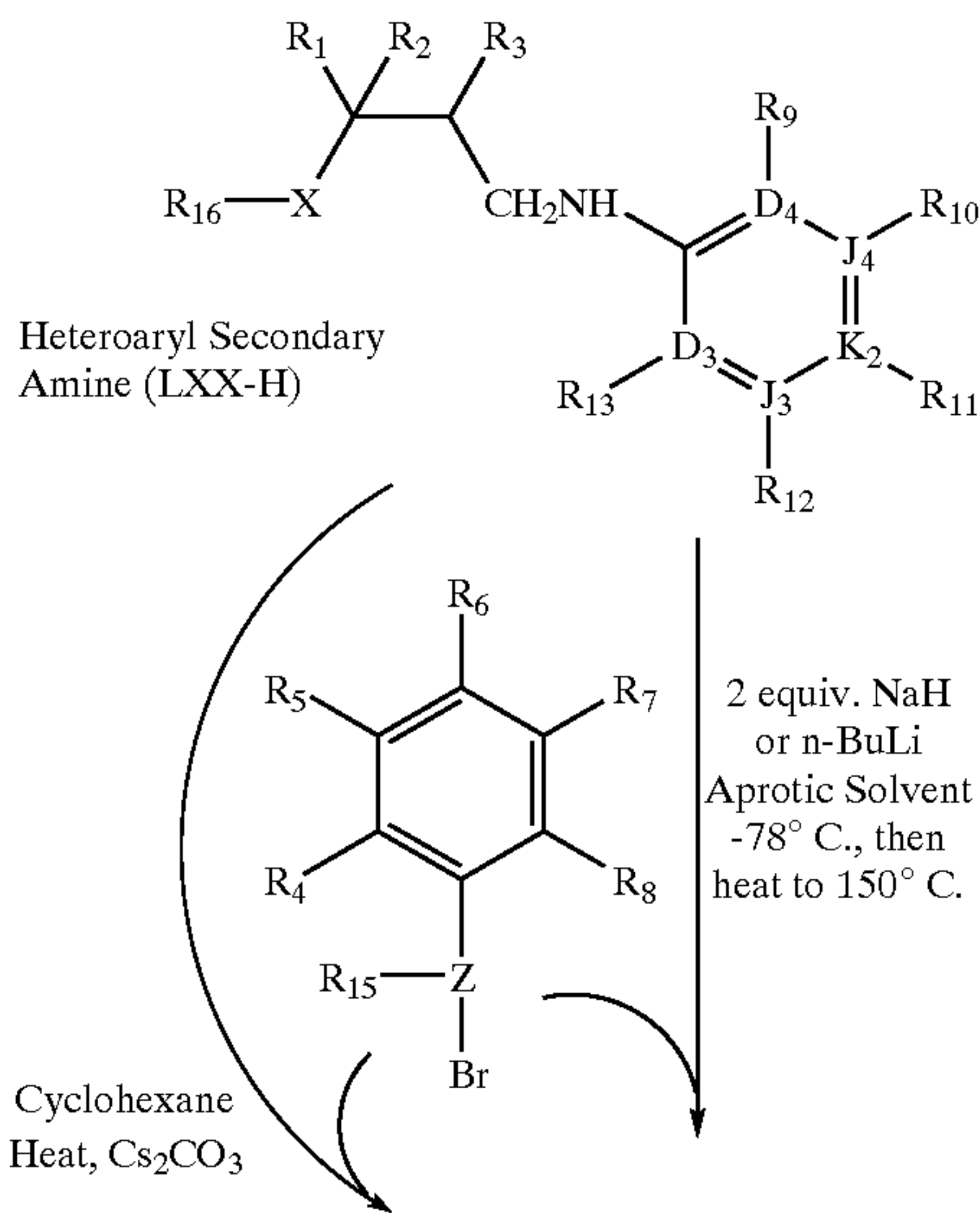
Scheme 54
