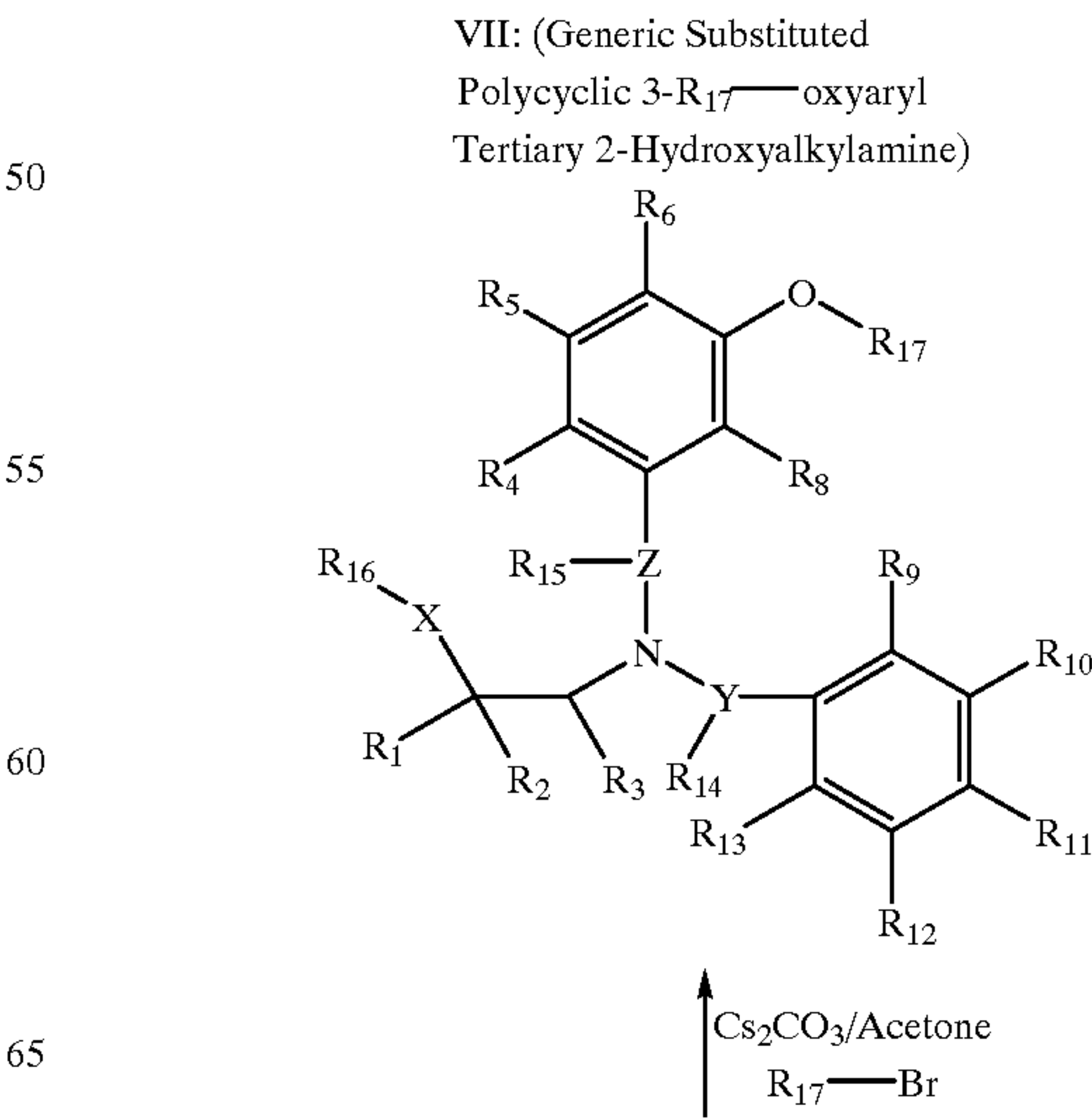
Scheme 20
