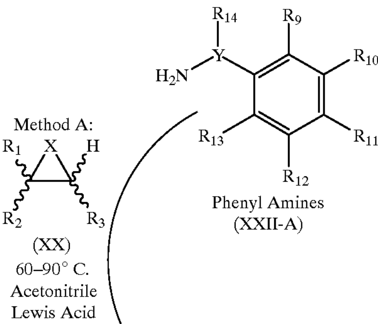
Scheme 58
