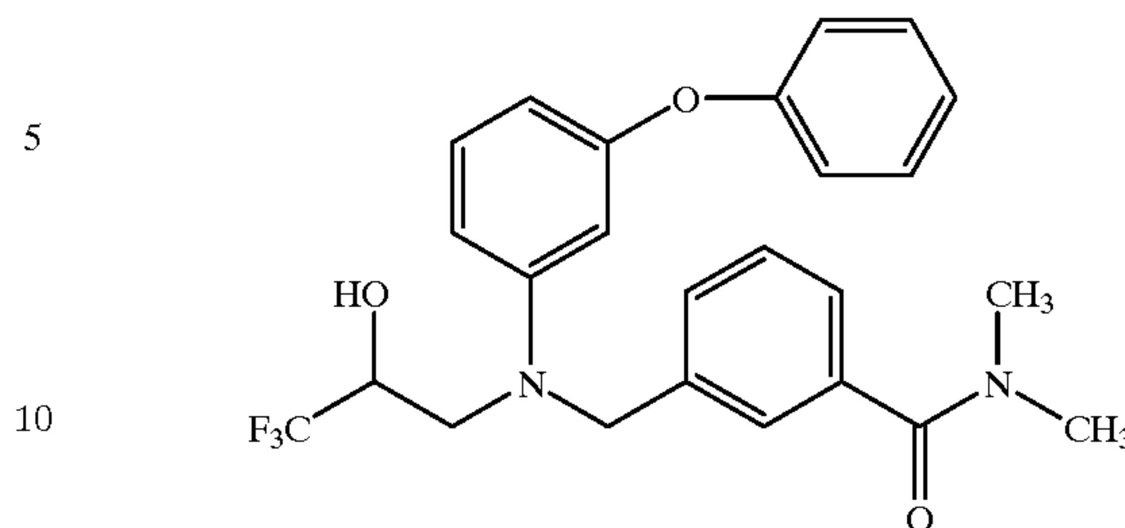
N,N-dimethyl-3-[[[(3-phenoxyphenyl)(3,3,3-trifluoro-2-hydroxypropyl)amino]methyl]benzamide
