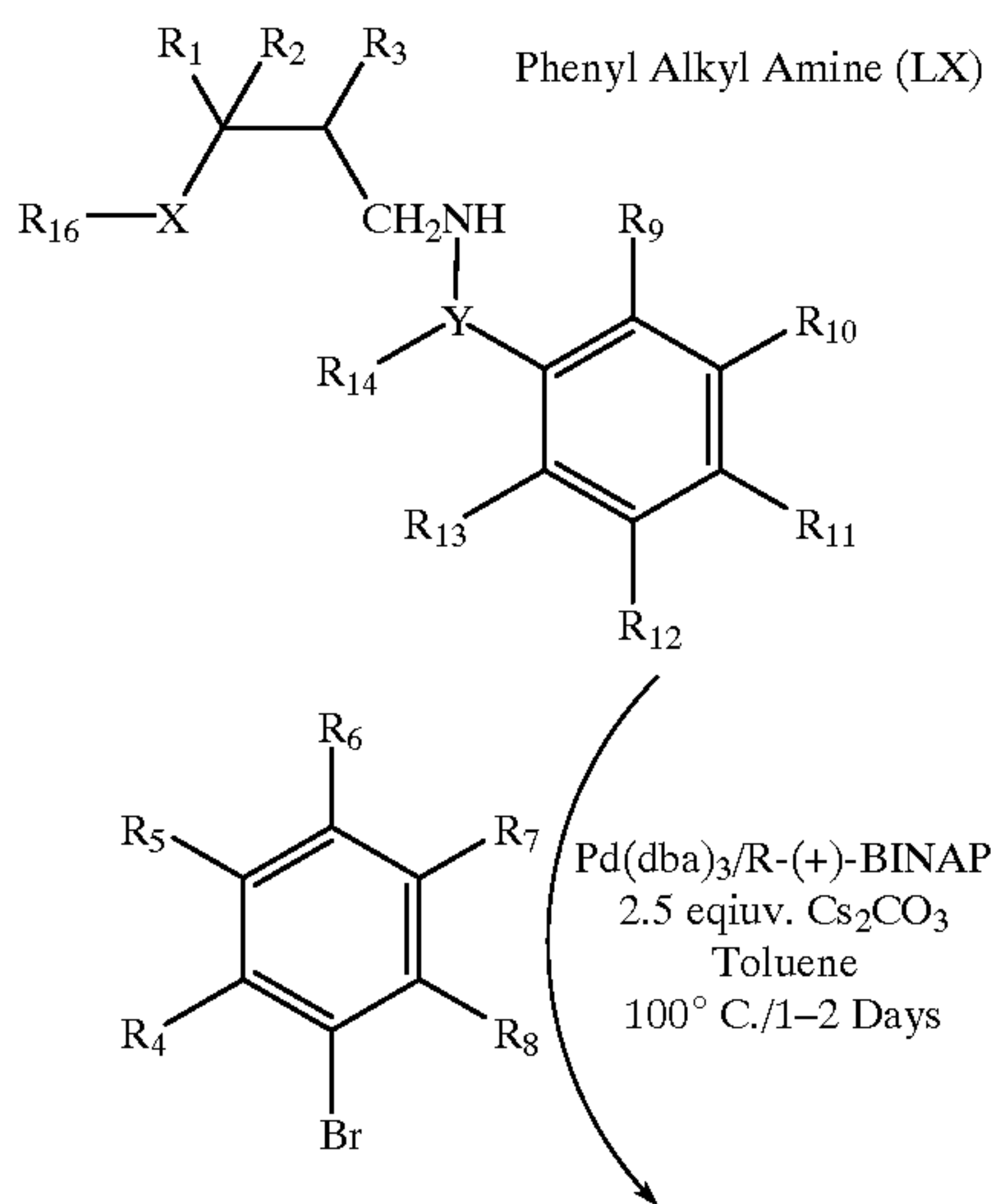
Scheme 35
