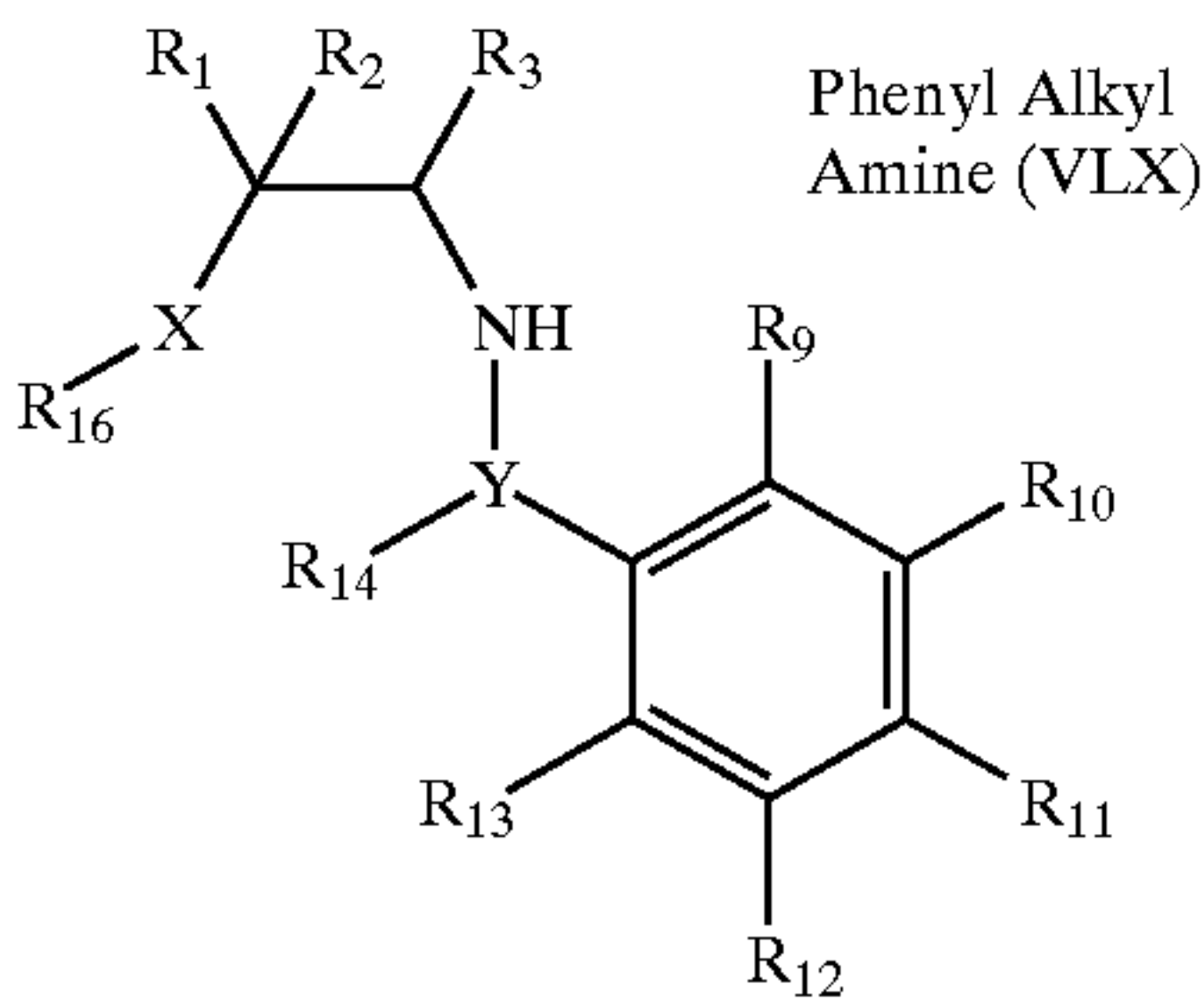
Scheme 48
