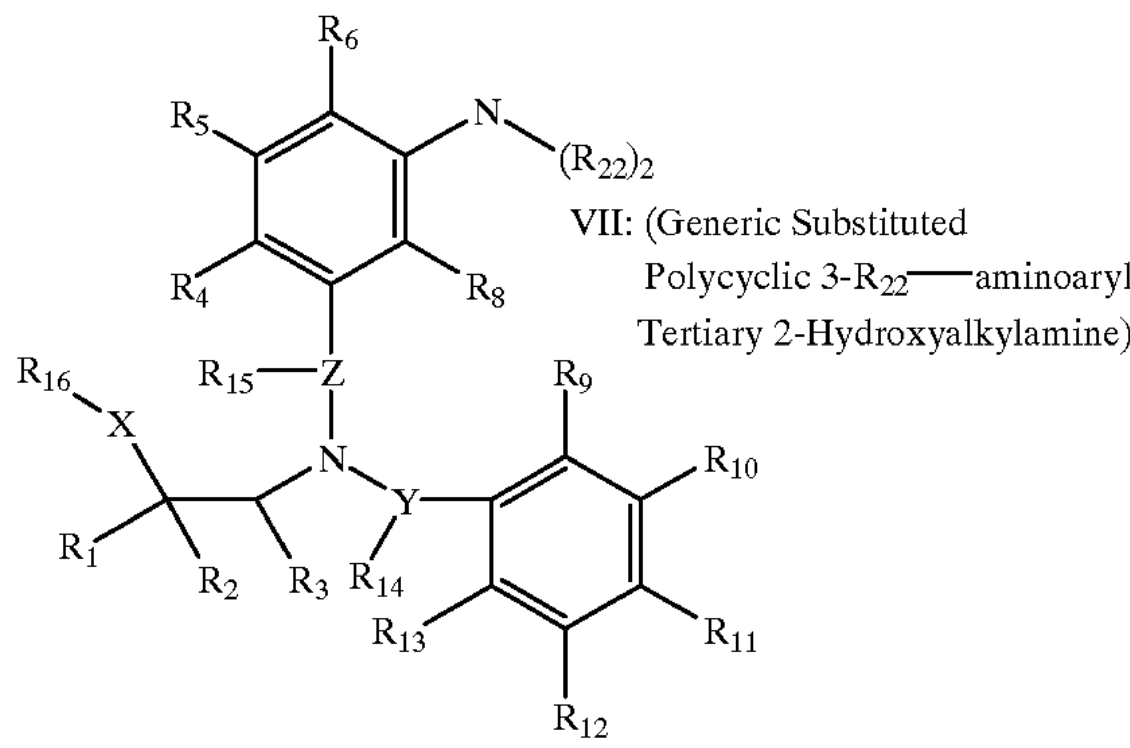
Scheme 23
