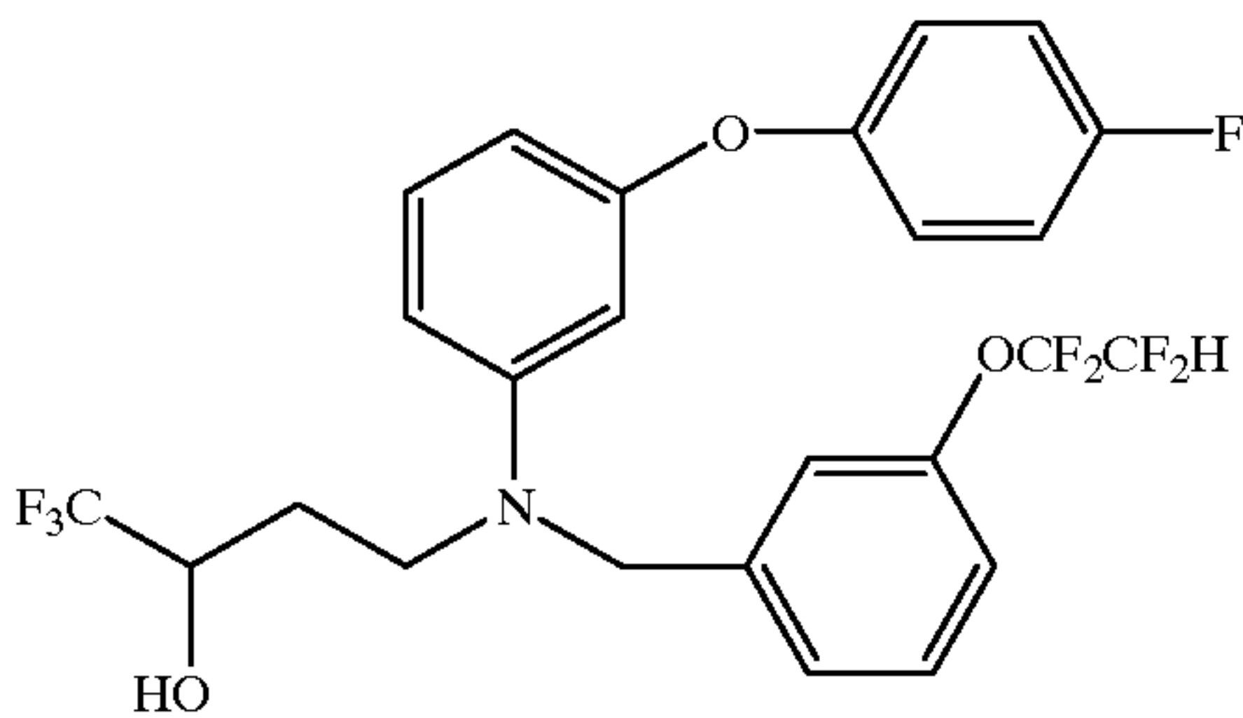
4-[[[3-(1,1,2,2-tetrafluoroethoxy)phenyl]methyl]amino]-1,1,1-trifluoro-2-butanol
