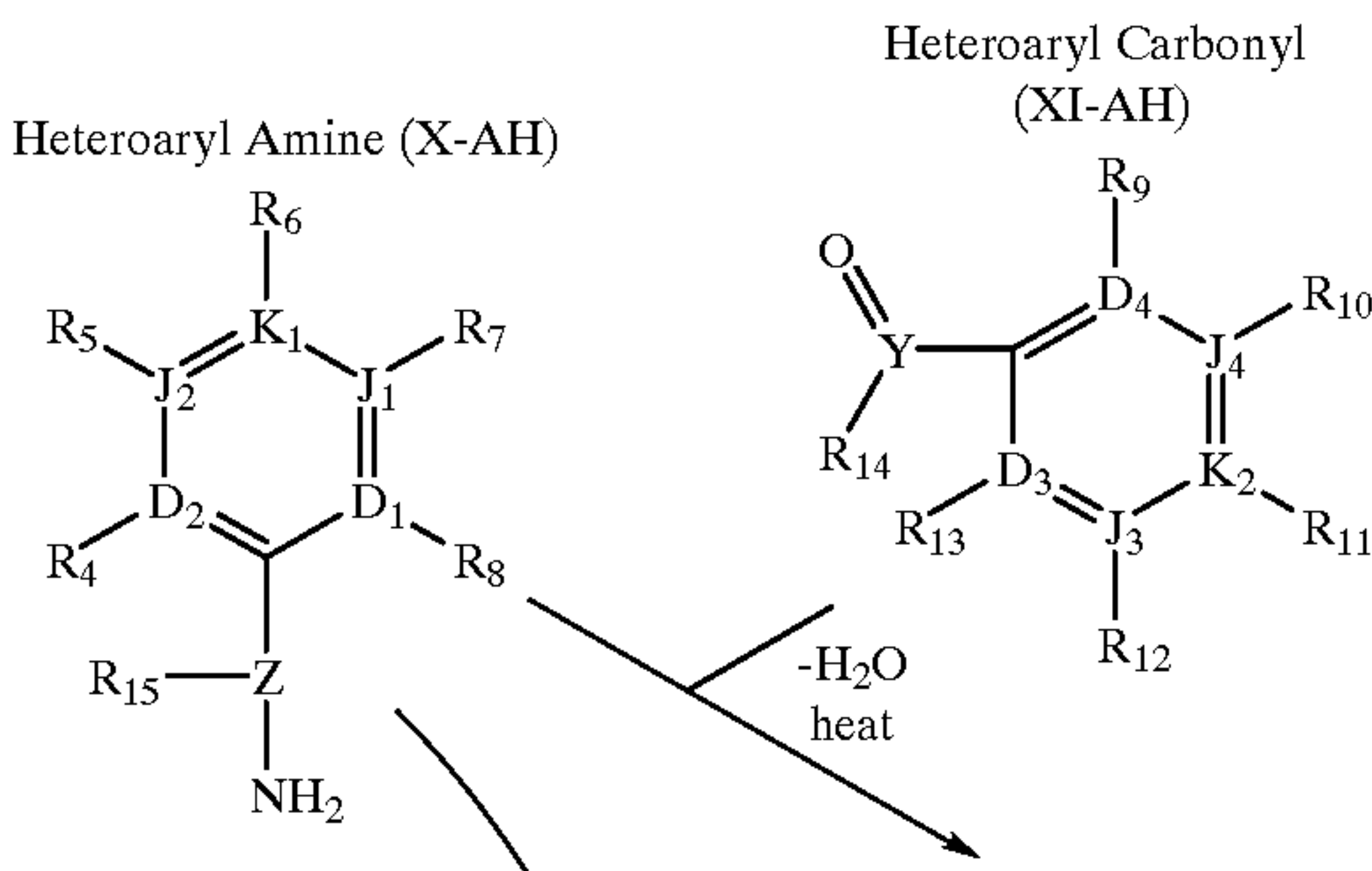
Scheme 3
