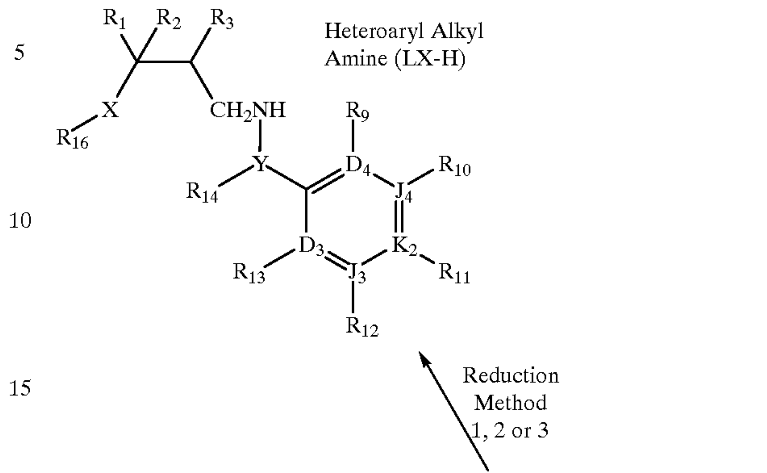
Scheme 30
