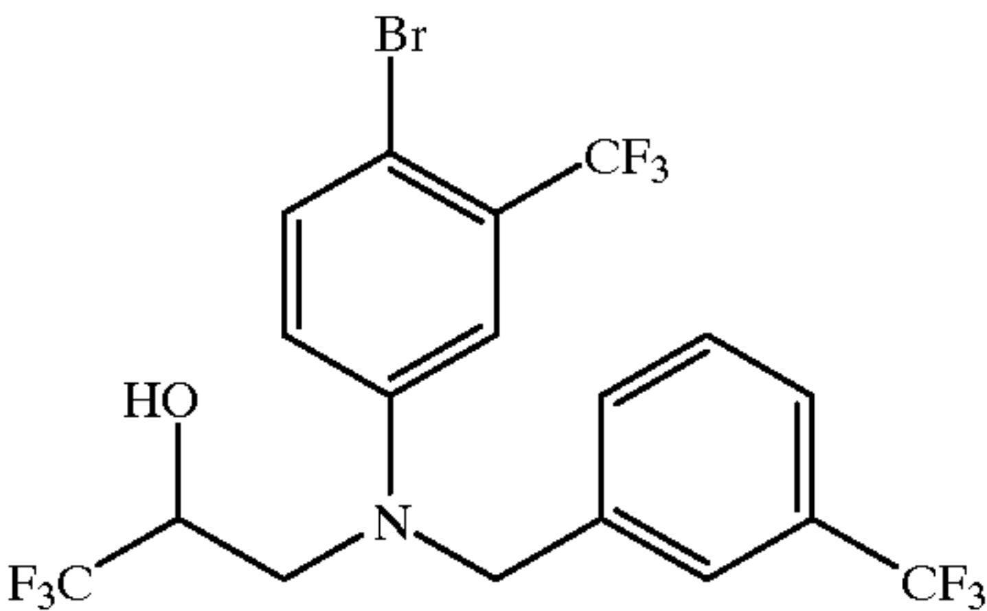
3-[4-bromo-3-(trifluoromethyl)phenyl][[3-(trifluoromethyl)phenyl]methyl]amino]-1,1,1-trifluoro-2-propanol
