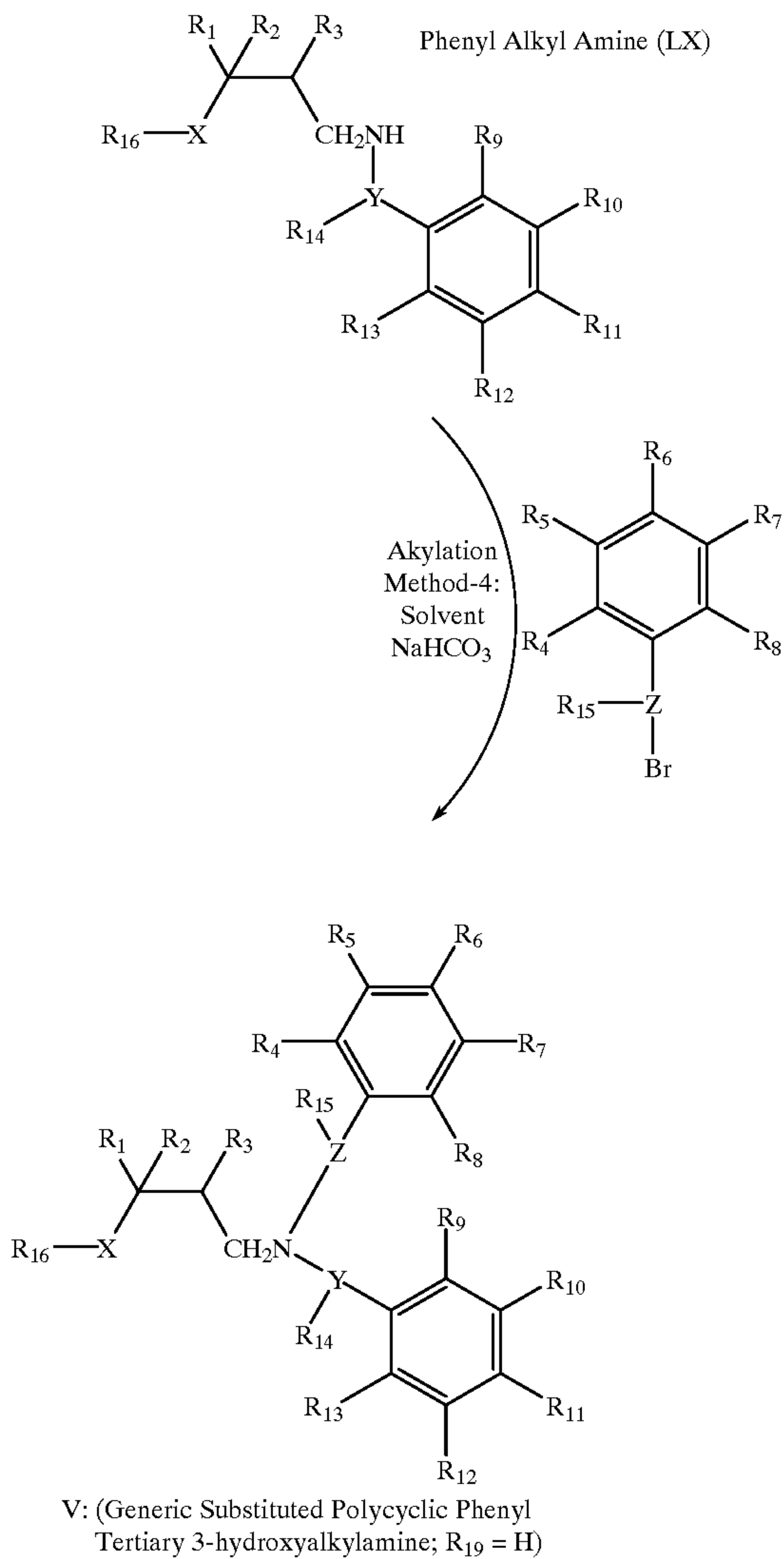
Scheme 34
