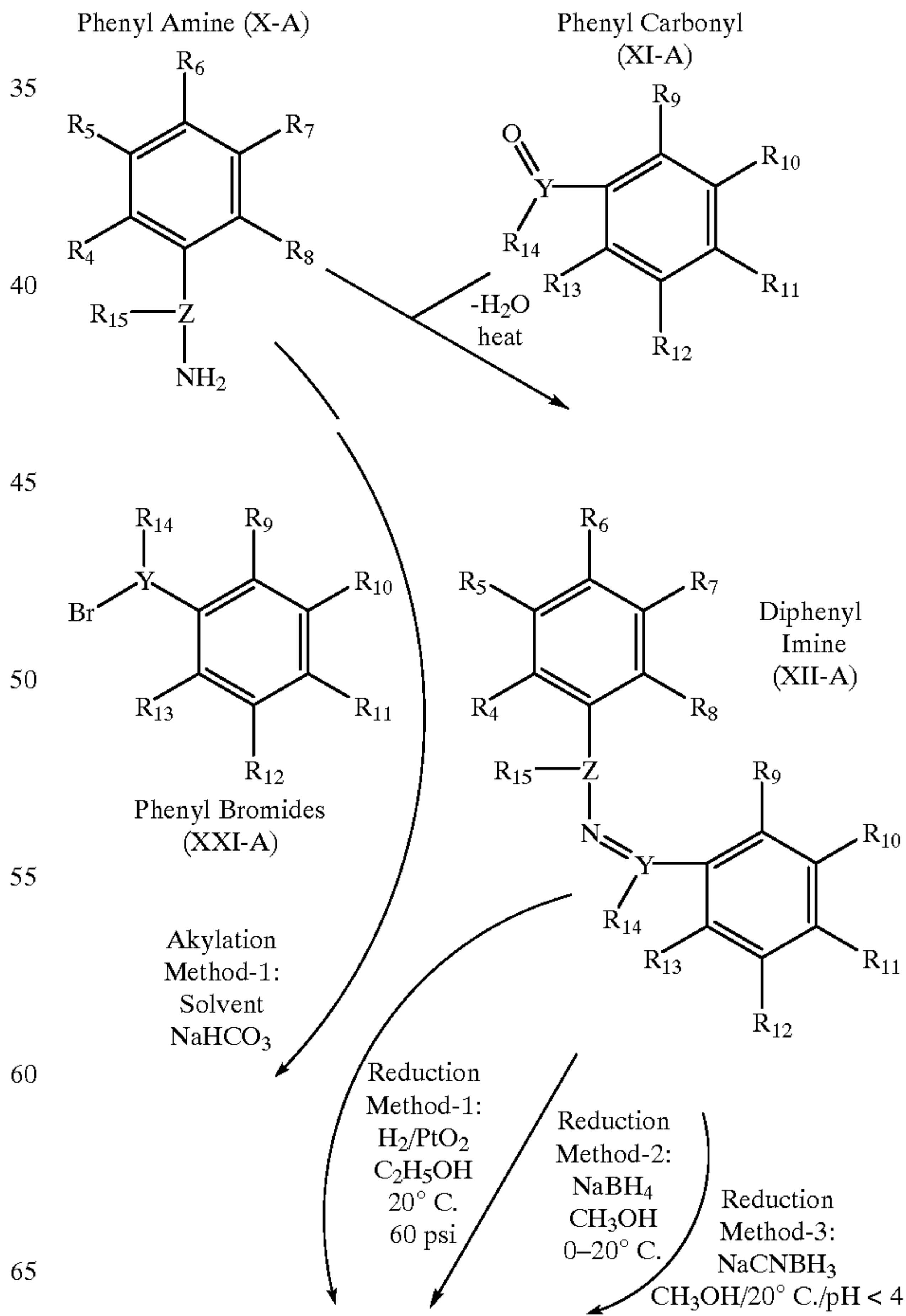
Scheme 9
