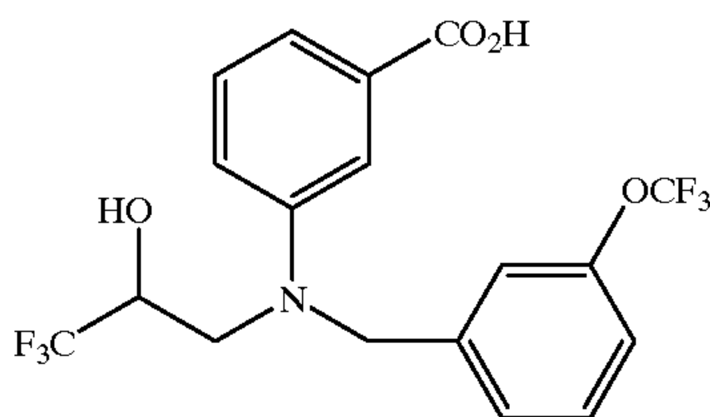
3-[(3,3,3-trifluoro-2-hydroxypropyl)[[(3-trifluoromethyl)phenyl]methyl]amino]benzoic Acid
