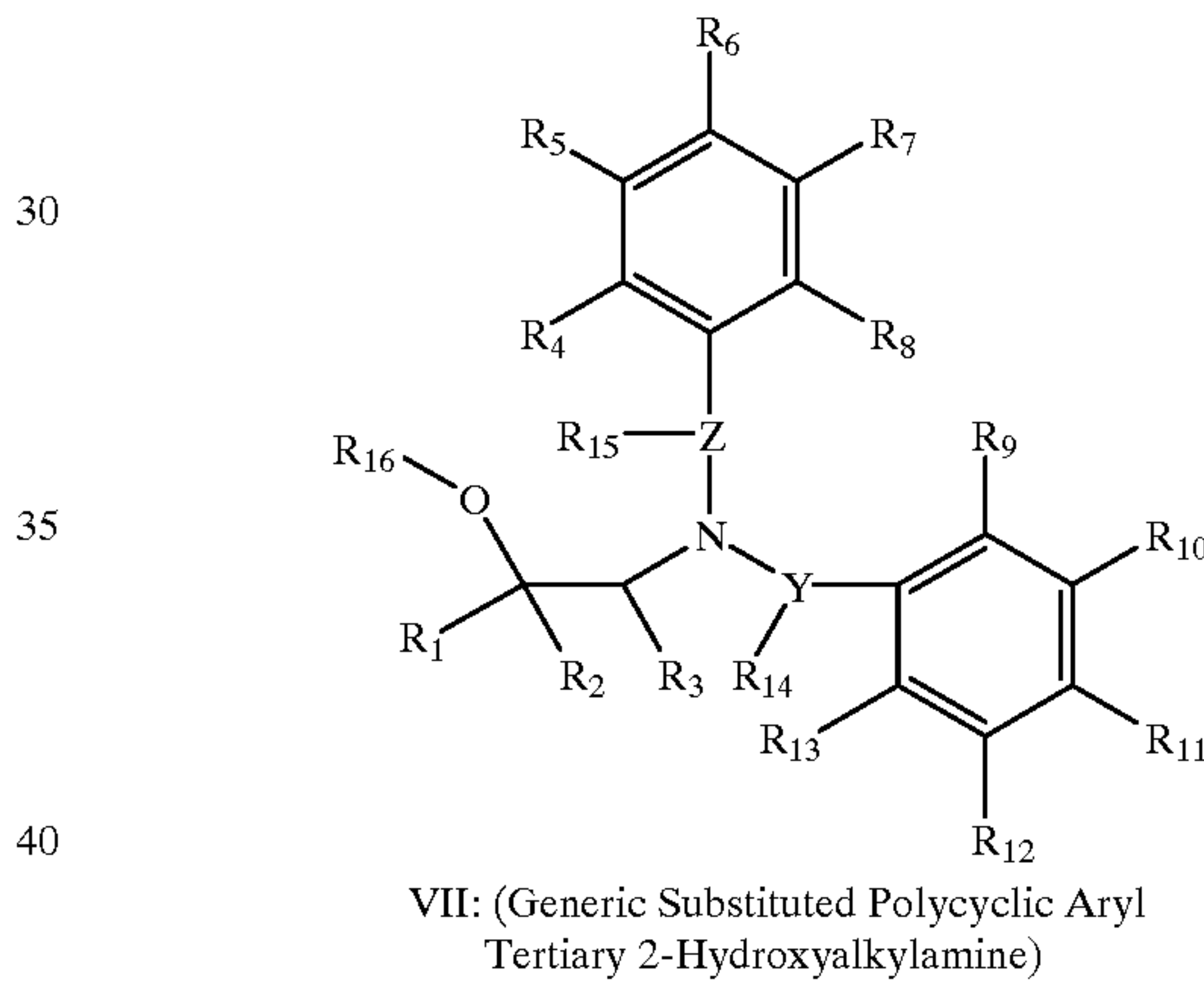
Scheme 12
