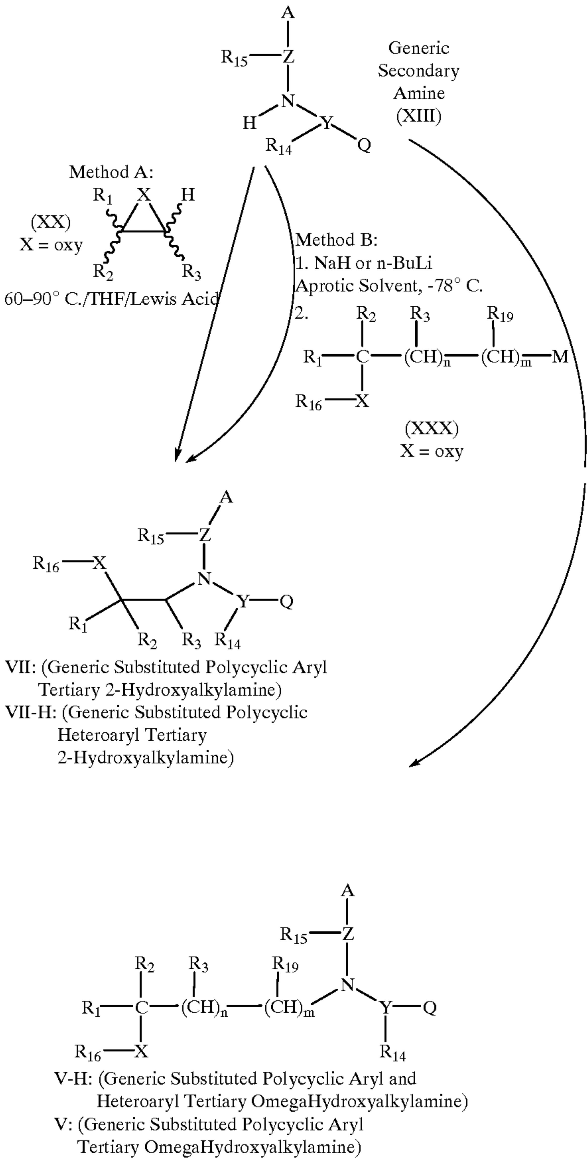
Scheme 2
