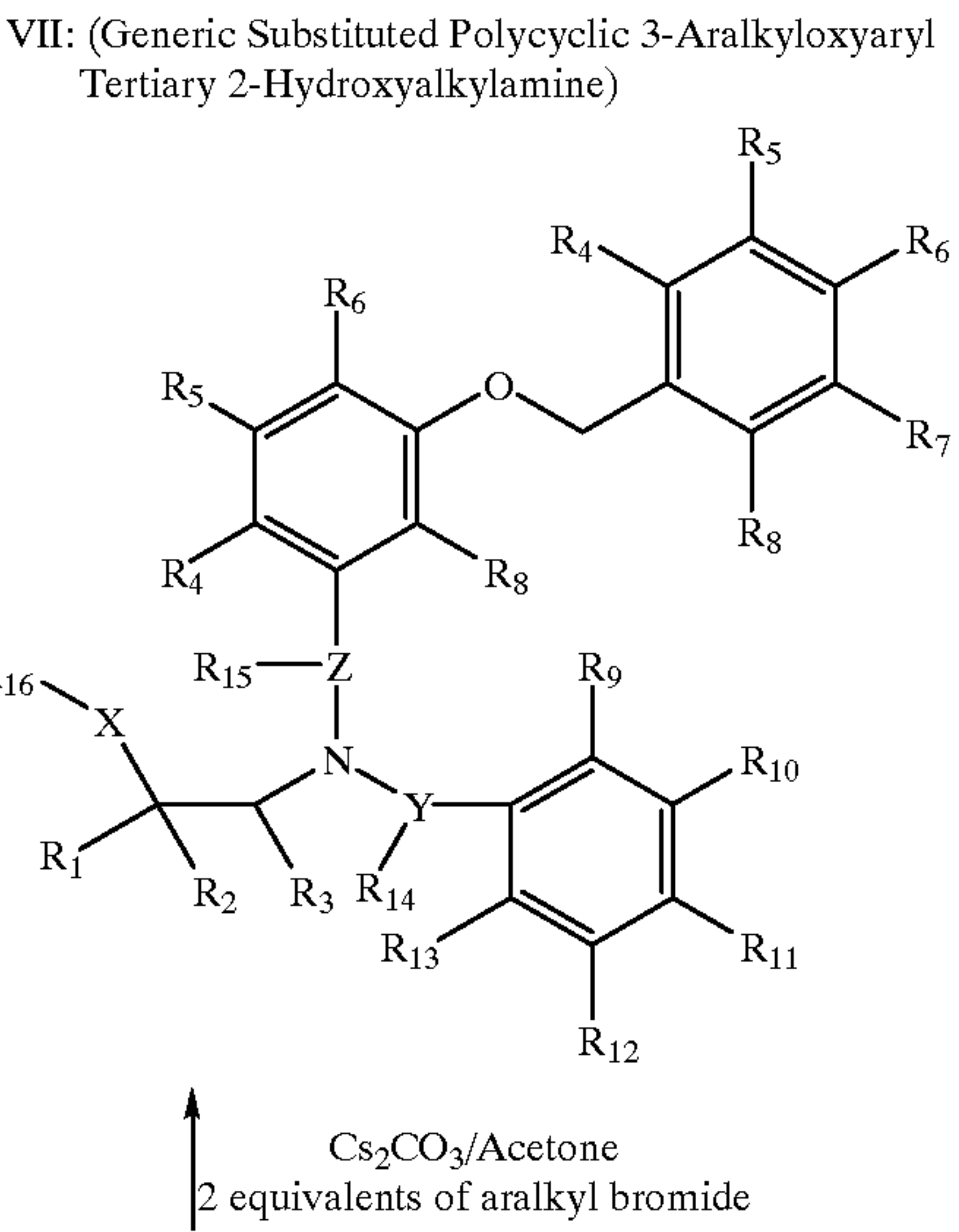
Scheme 16
