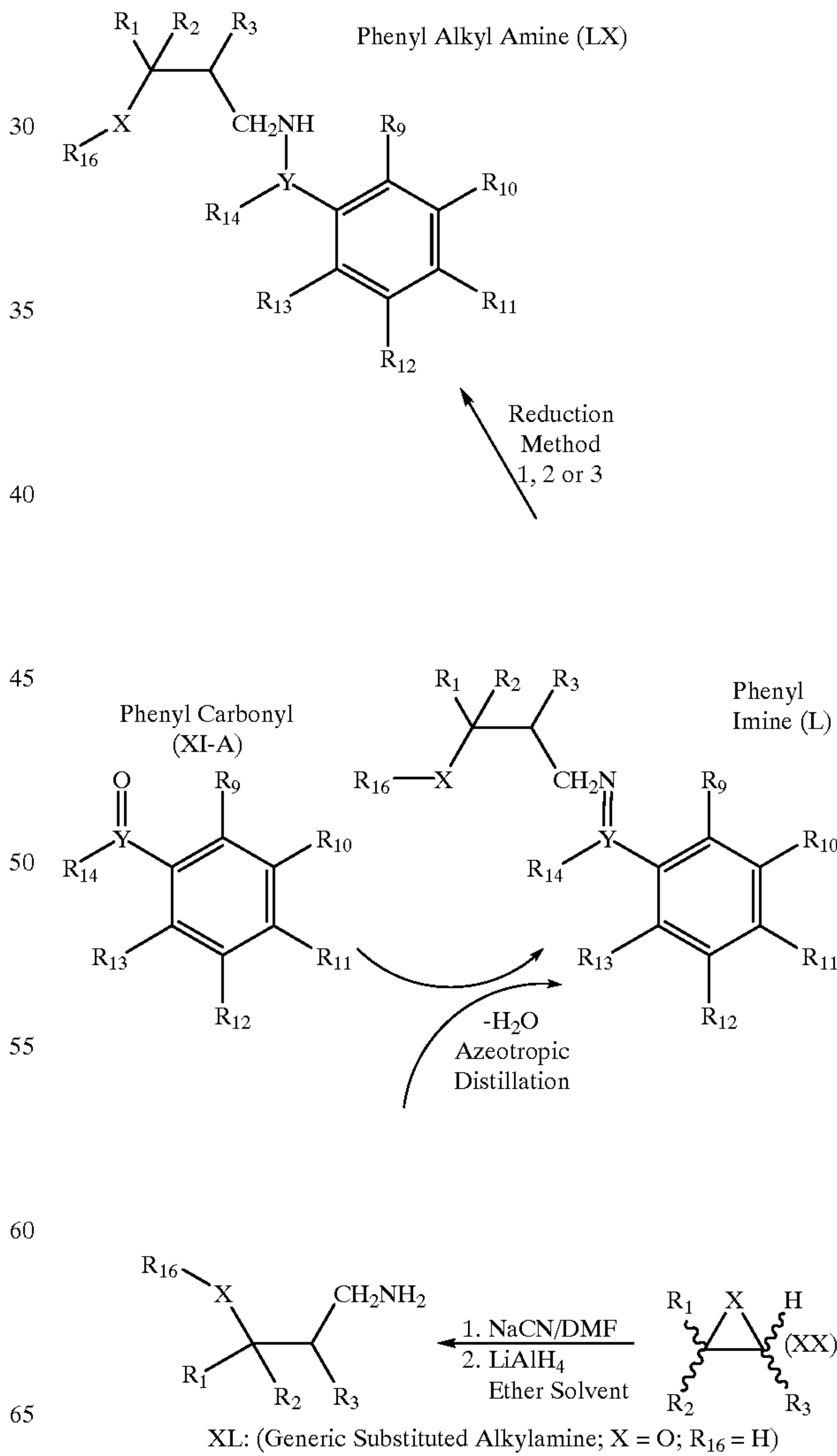
Scheme 33
