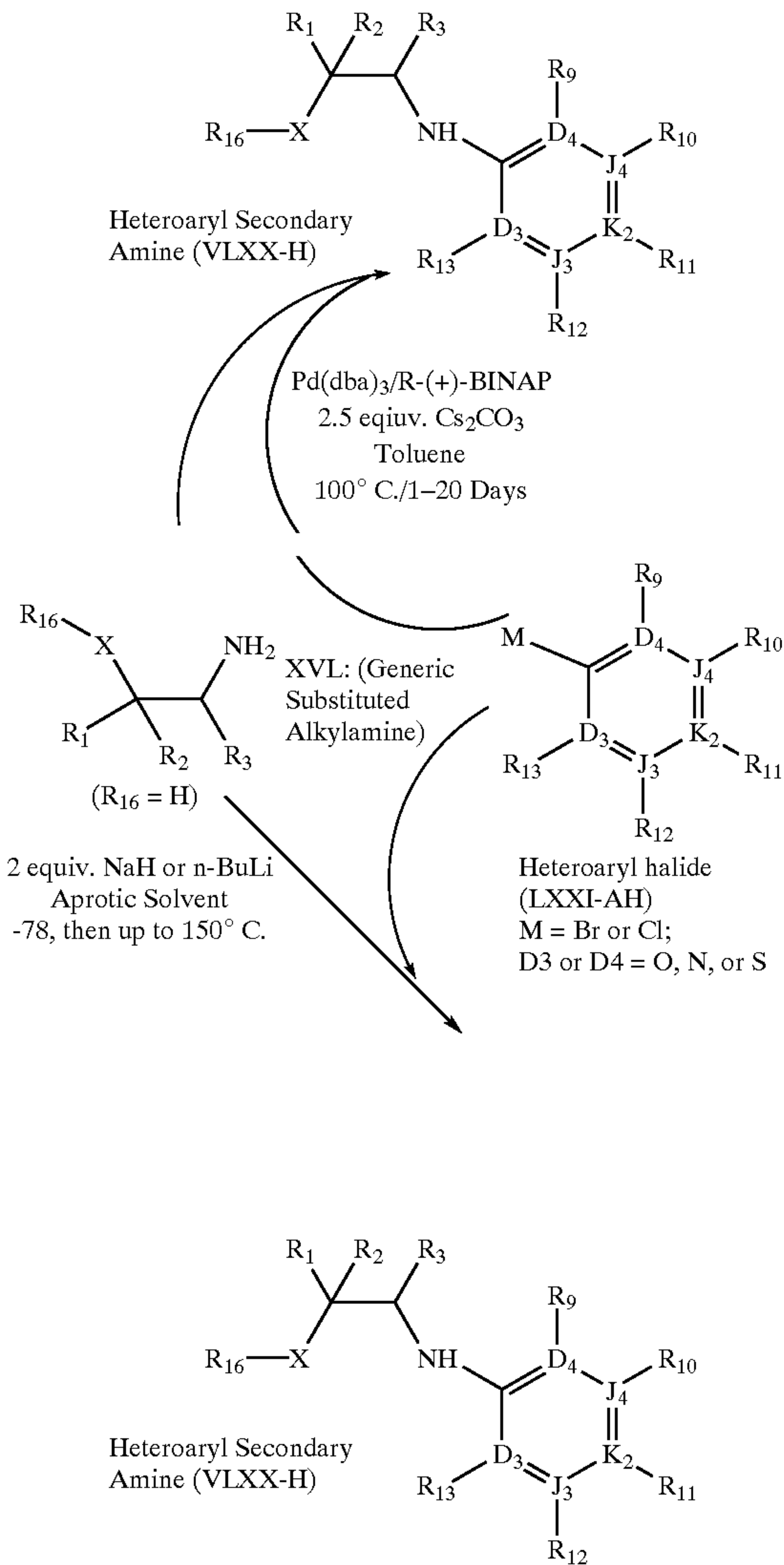
Scheme 51
