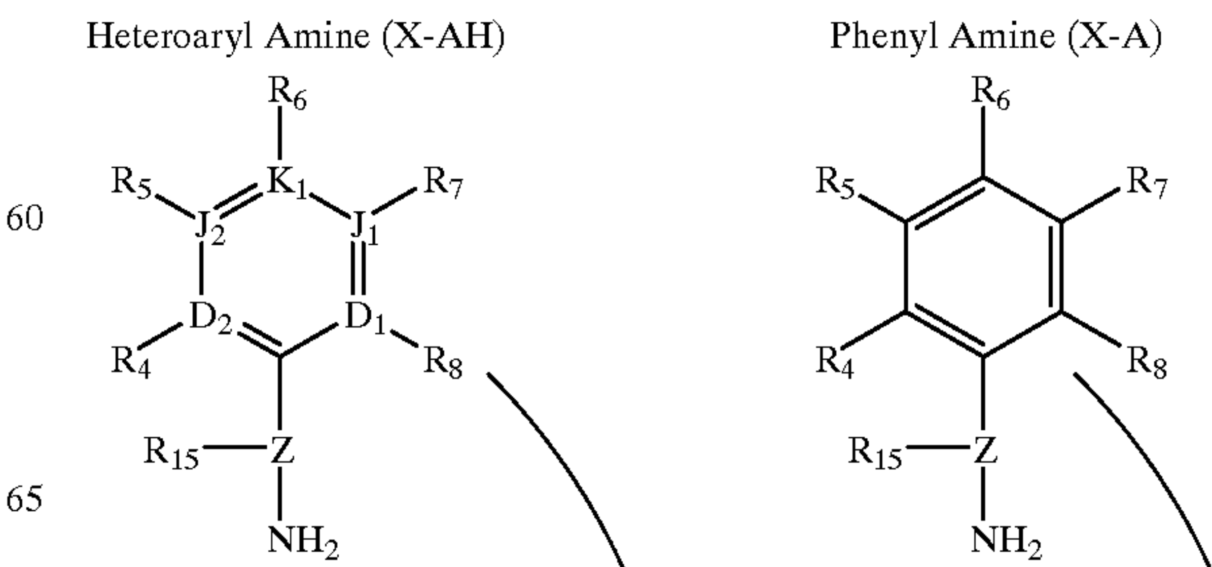
Scheme 4
