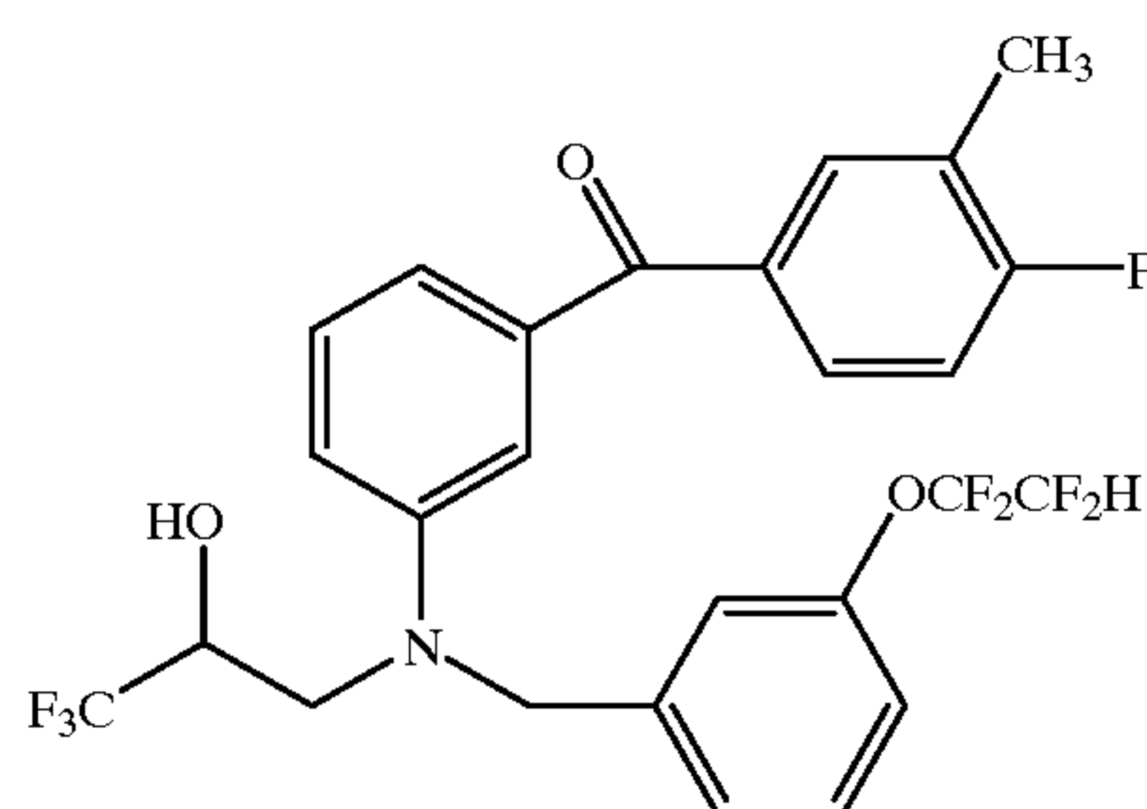
(4-Fluoro-3-methylphenyl)[3-[[[(1,1,2,2-tetrafluoroethoxy)phenyl]methyl](3,3,3-trifluoro-2-hydroxypropyl)amino]phenyl]methanone
