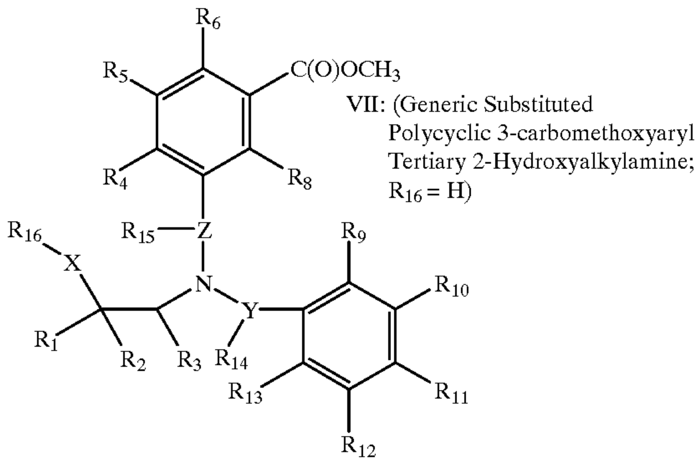
Scheme 27
