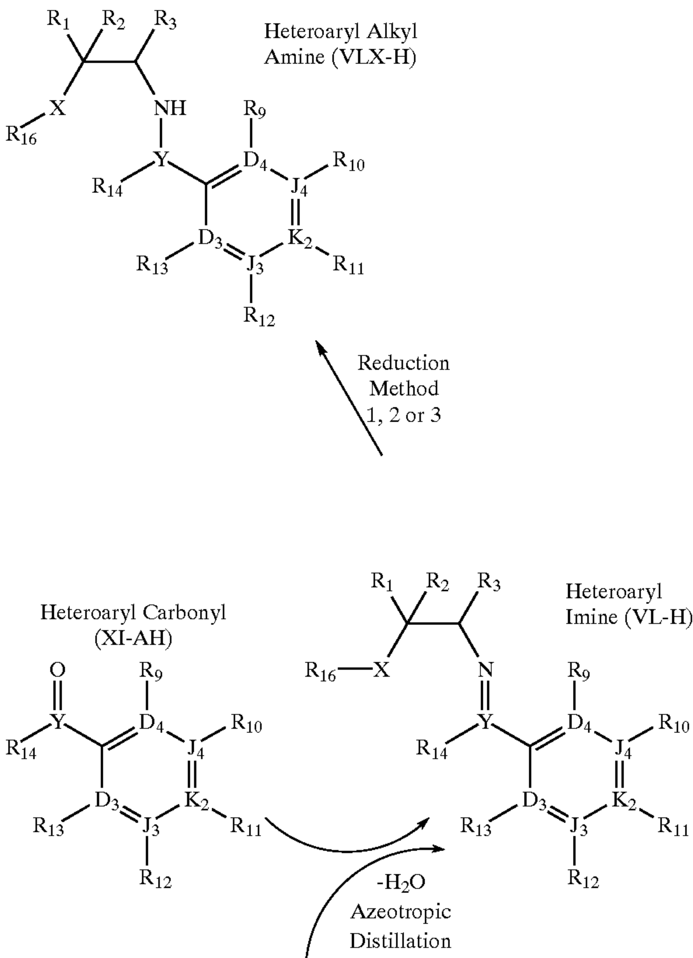
Scheme 45
