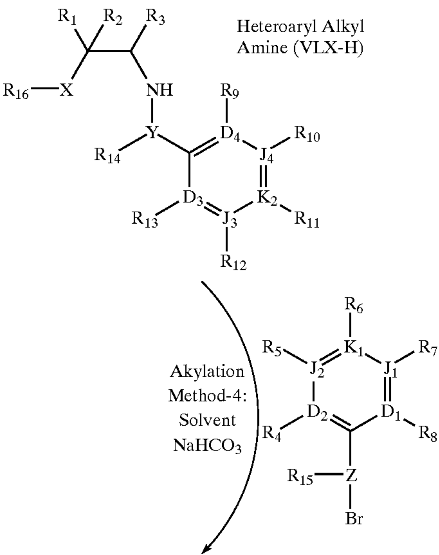
Scheme 46
