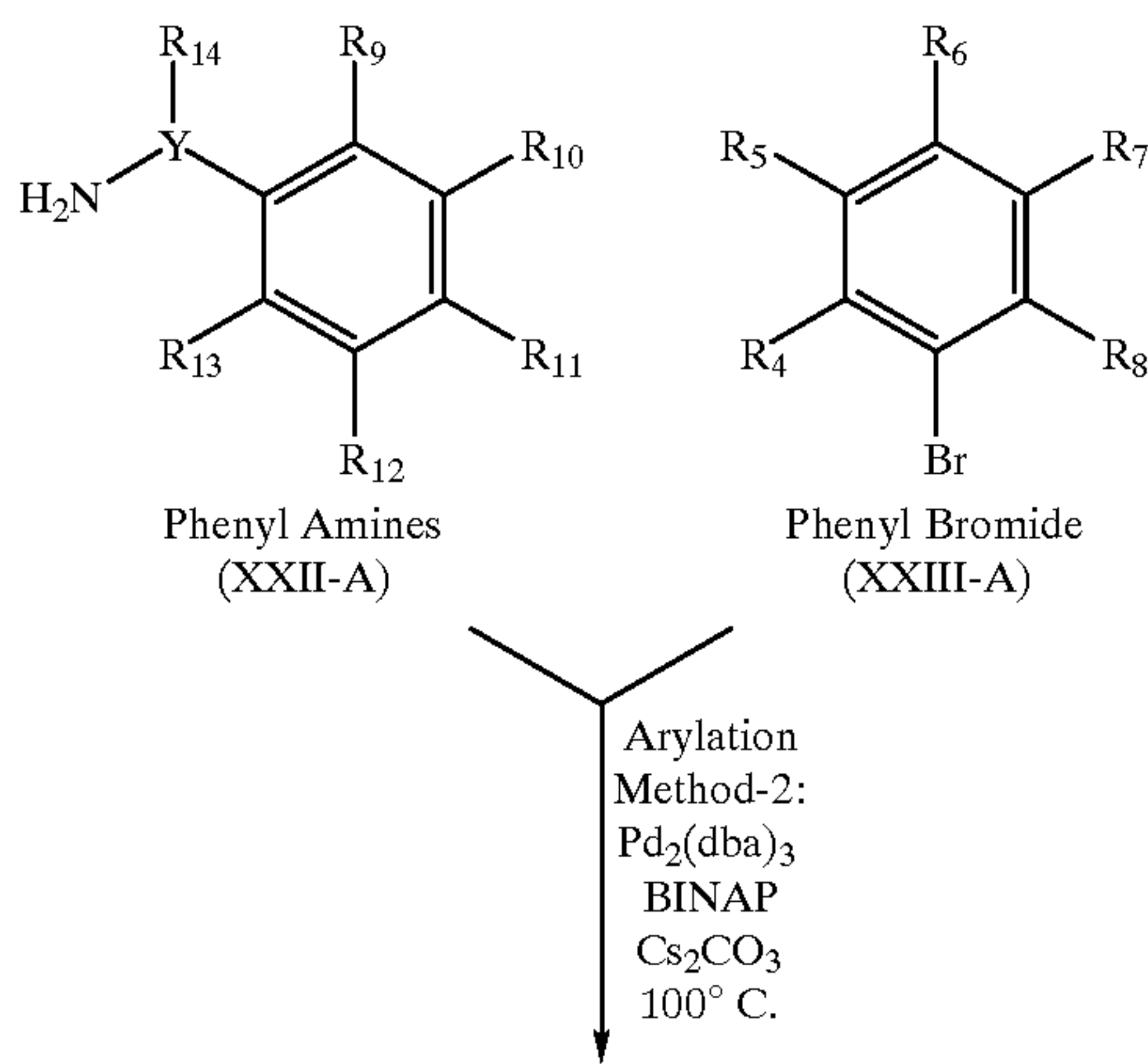
Scheme 10
