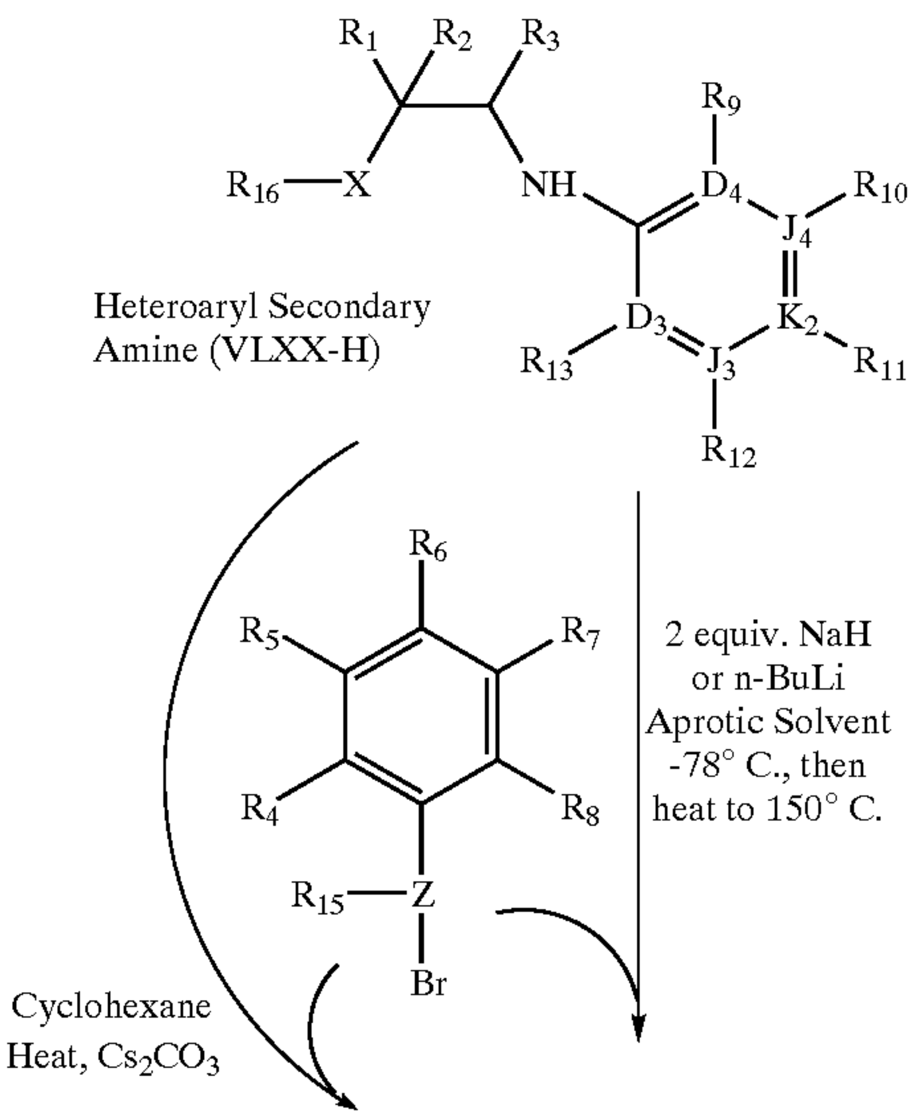
Scheme 52
