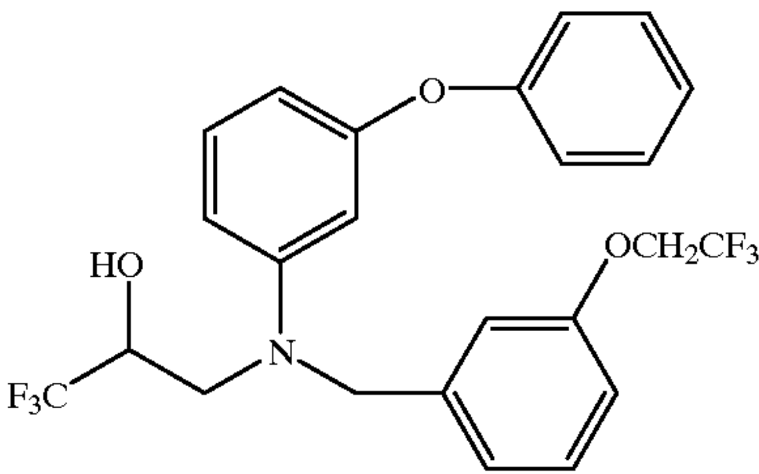
3-[(3-phenoxyphenyl)[[3-(2,2,2-trifluoroethoxy)phenyl]methyl]amino]-1,1,1-trifluoro-2-propanol
