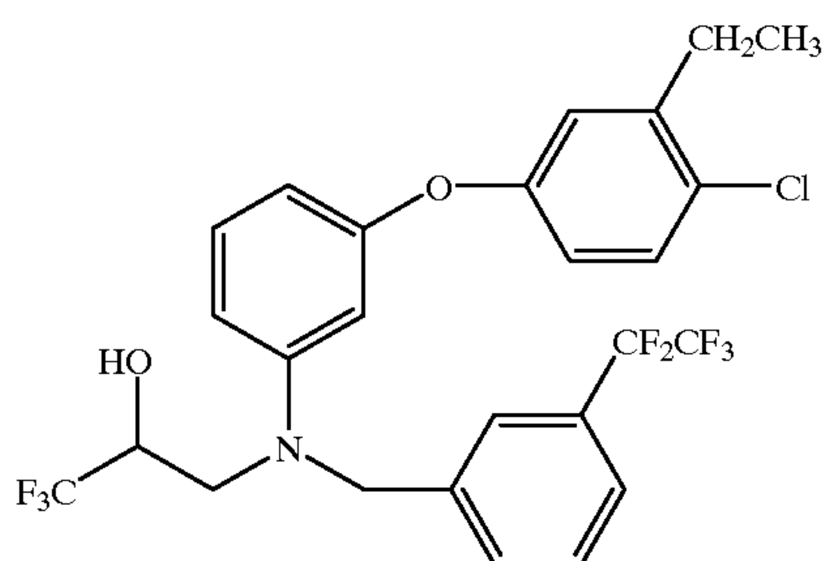
3-[(4-chloro-3-ethylphenoxy)phenyl][[3-(pentafluoroethyl)phenyl]methyl]-amino]-1,1,1-trifluoro-2-propanol
