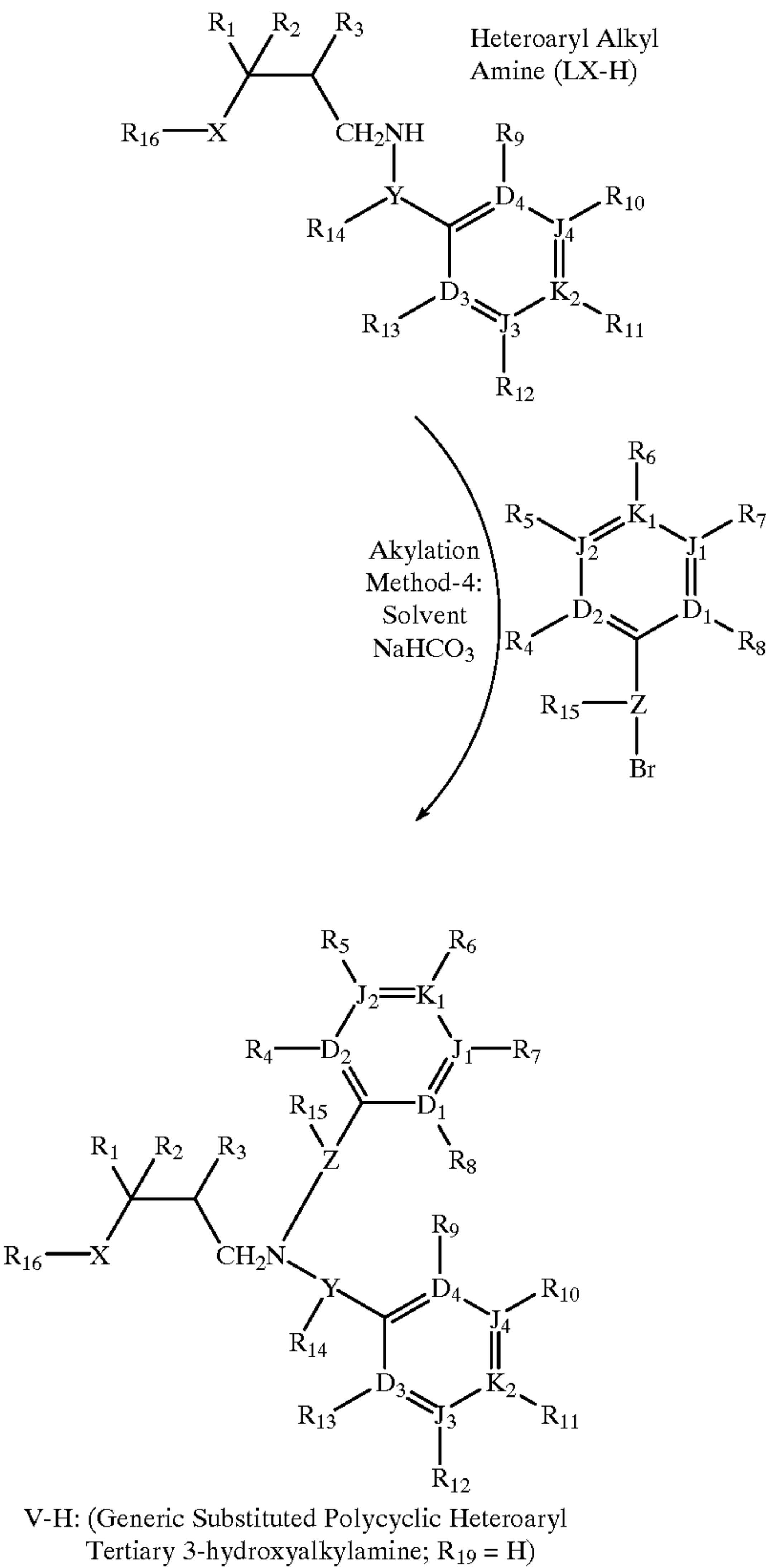
Scheme 31
