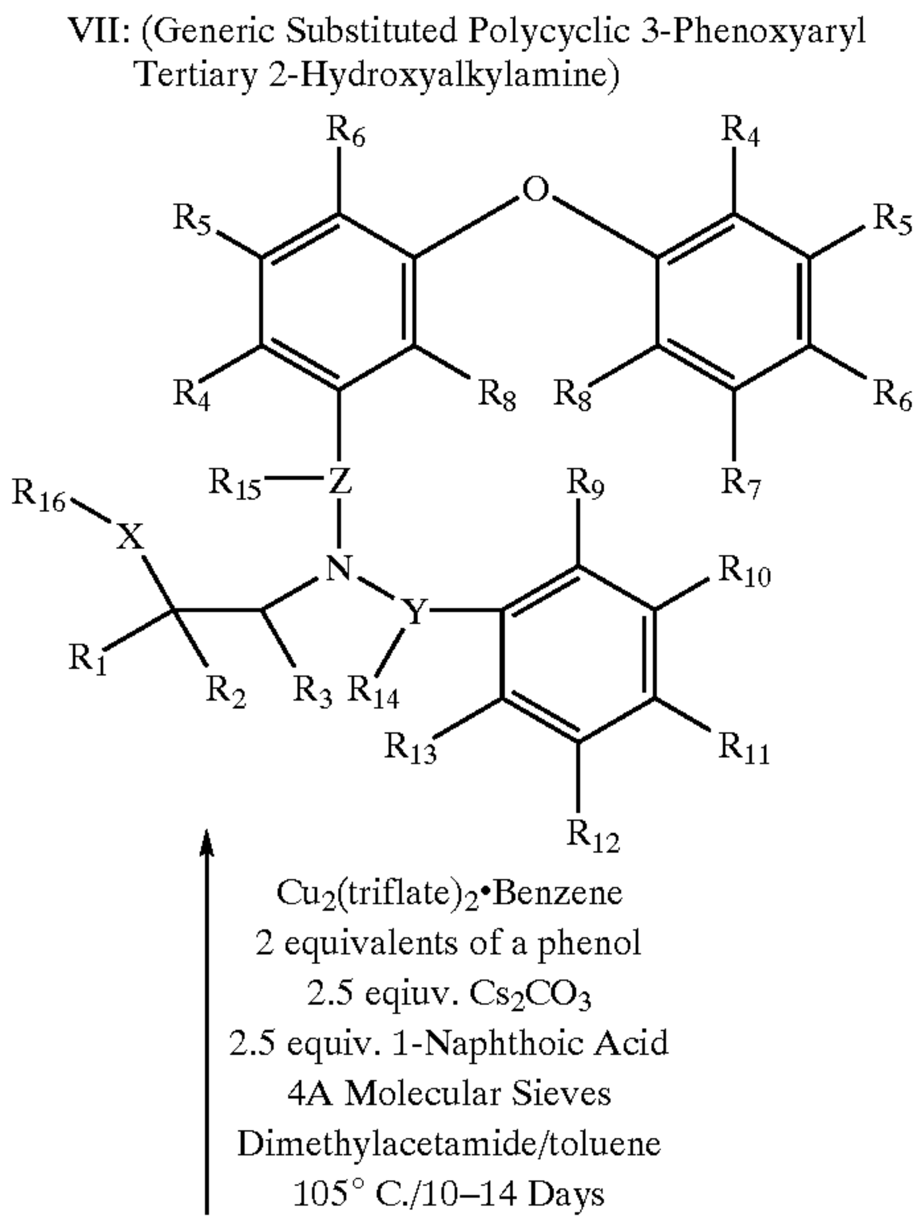
Scheme 8
