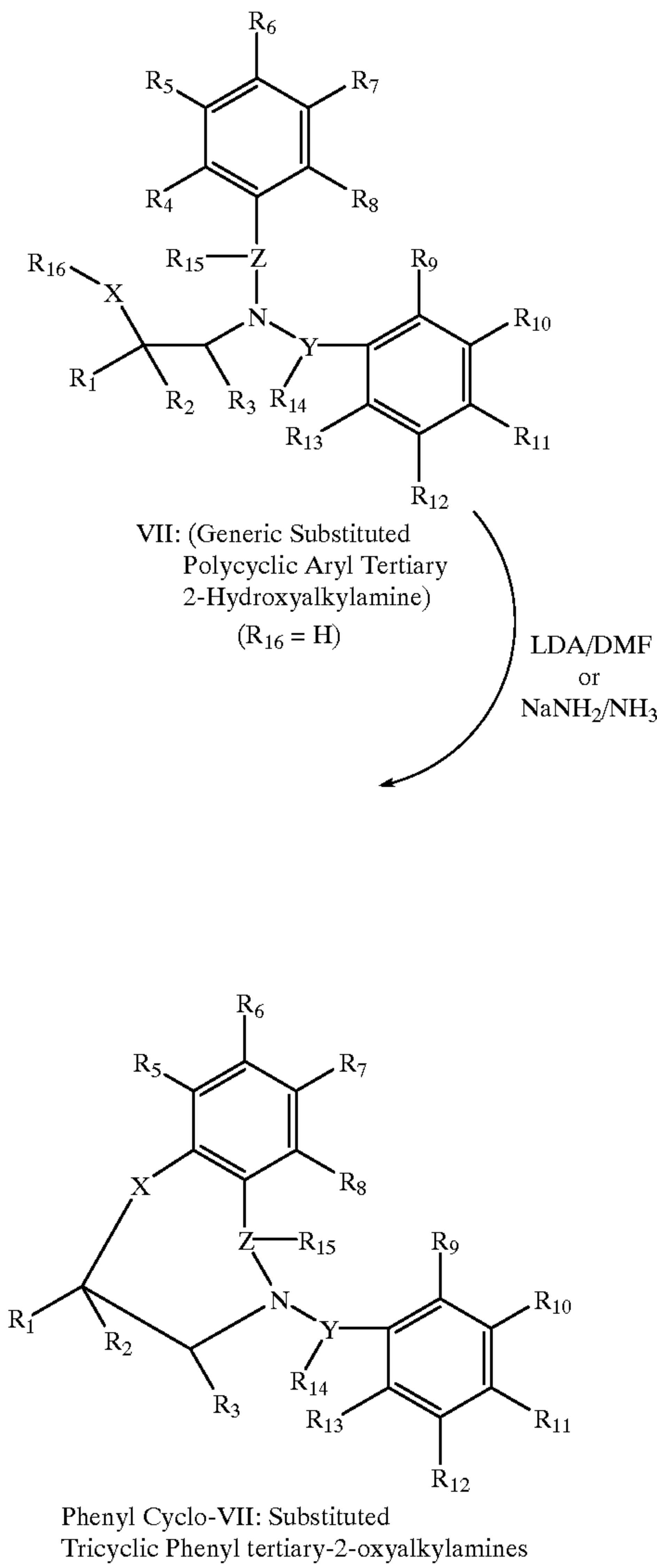
Scheme 18
