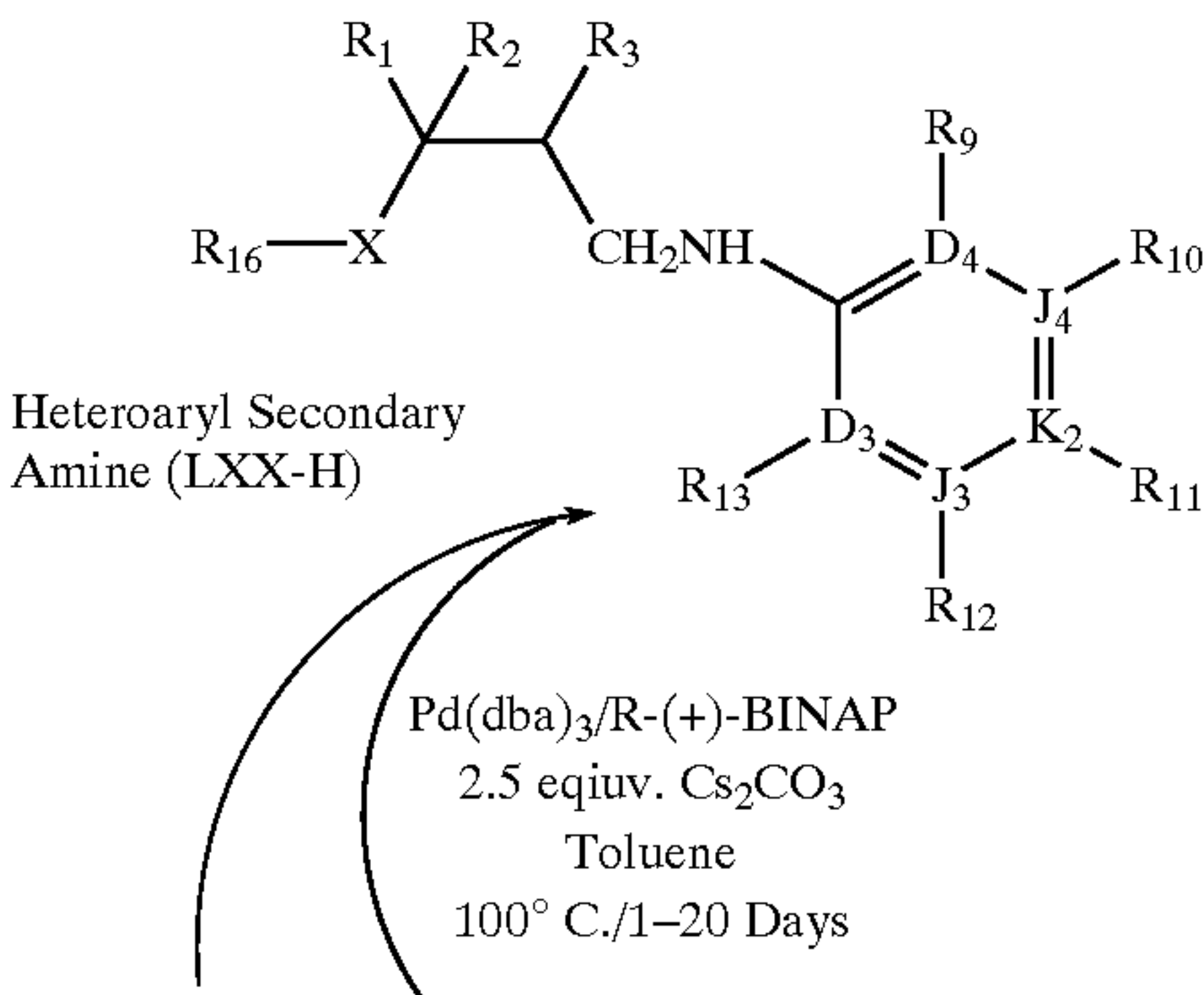
Scheme 53
