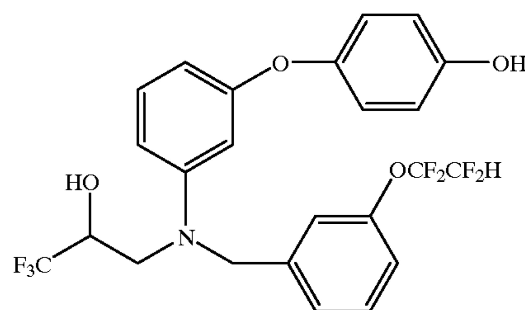
4-[3-[[[3-(1,1,2,2-tetrafluoroethoxy)phenyl]methyl](3,3,3-trifluoro-2-hydroxypropyl)amino]phenoxy]phenol
