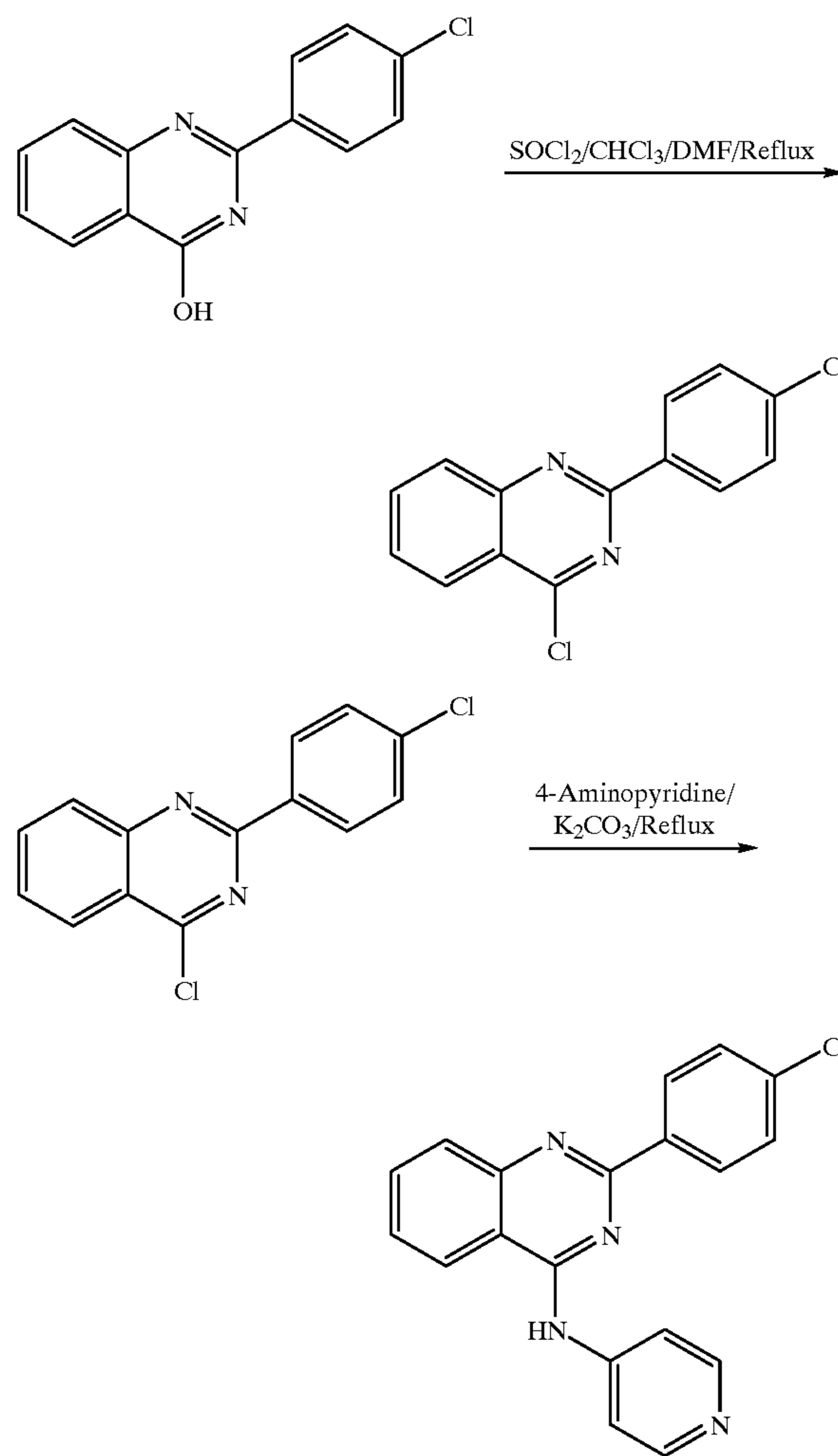
Reaction Scheme 2
