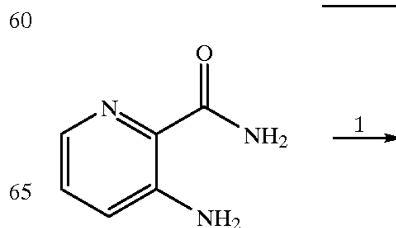
Reaction Scheme 5
