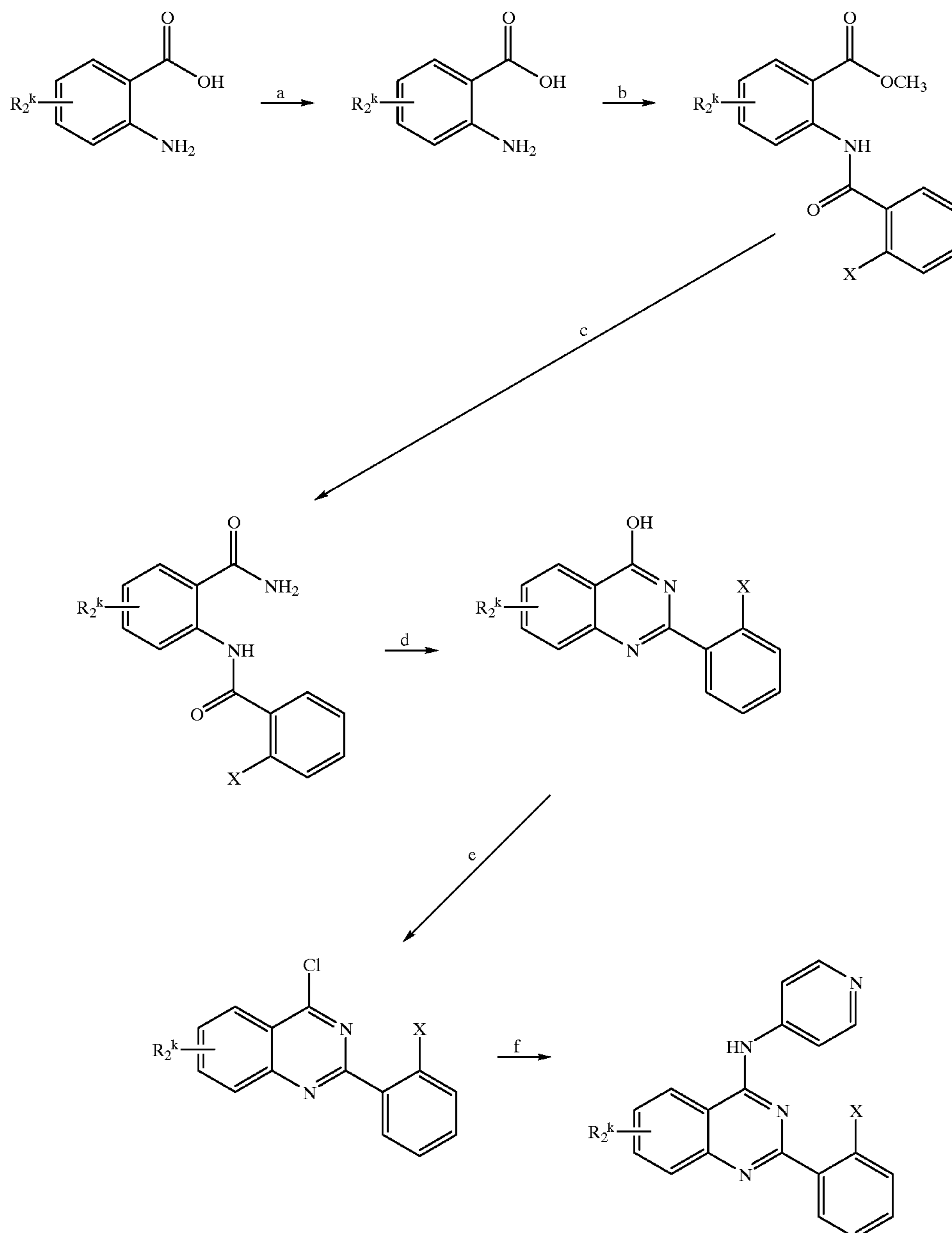
Reaction Scheme 8
