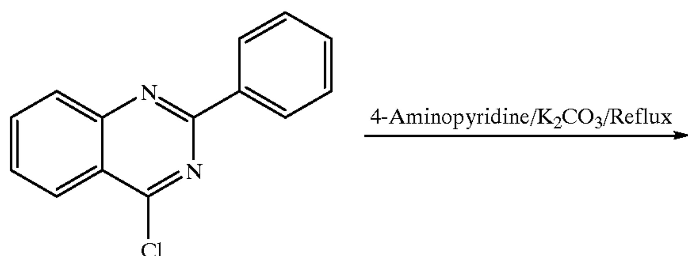
Reaction Scheme 1
