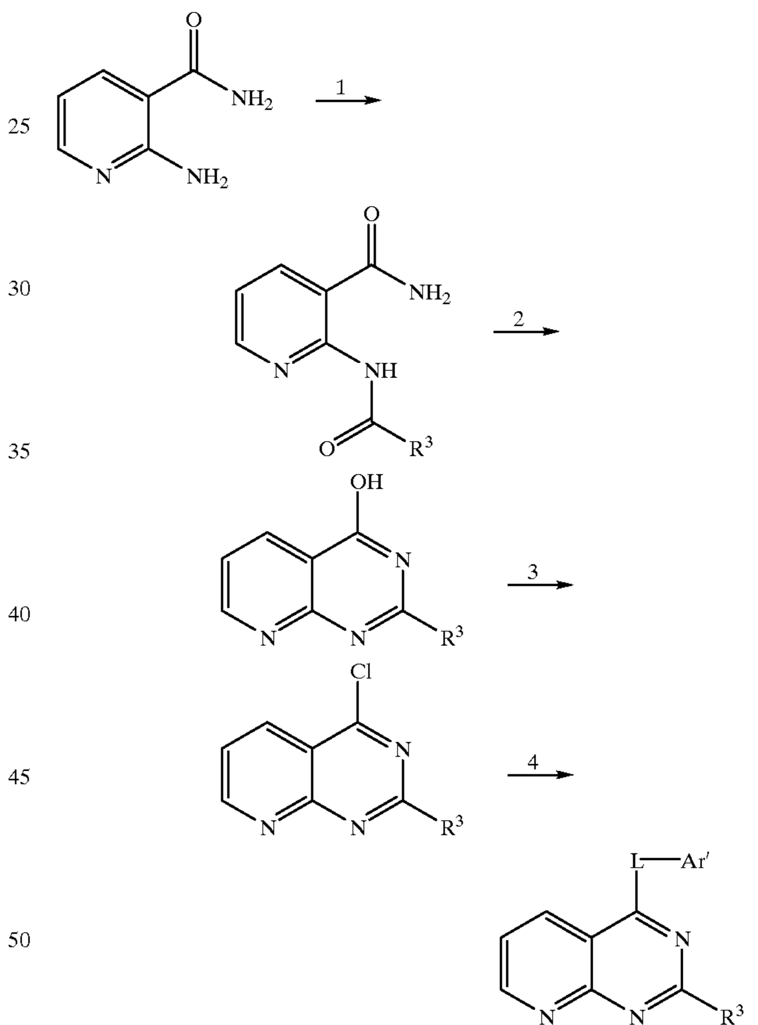
Reaction Scheme 4
