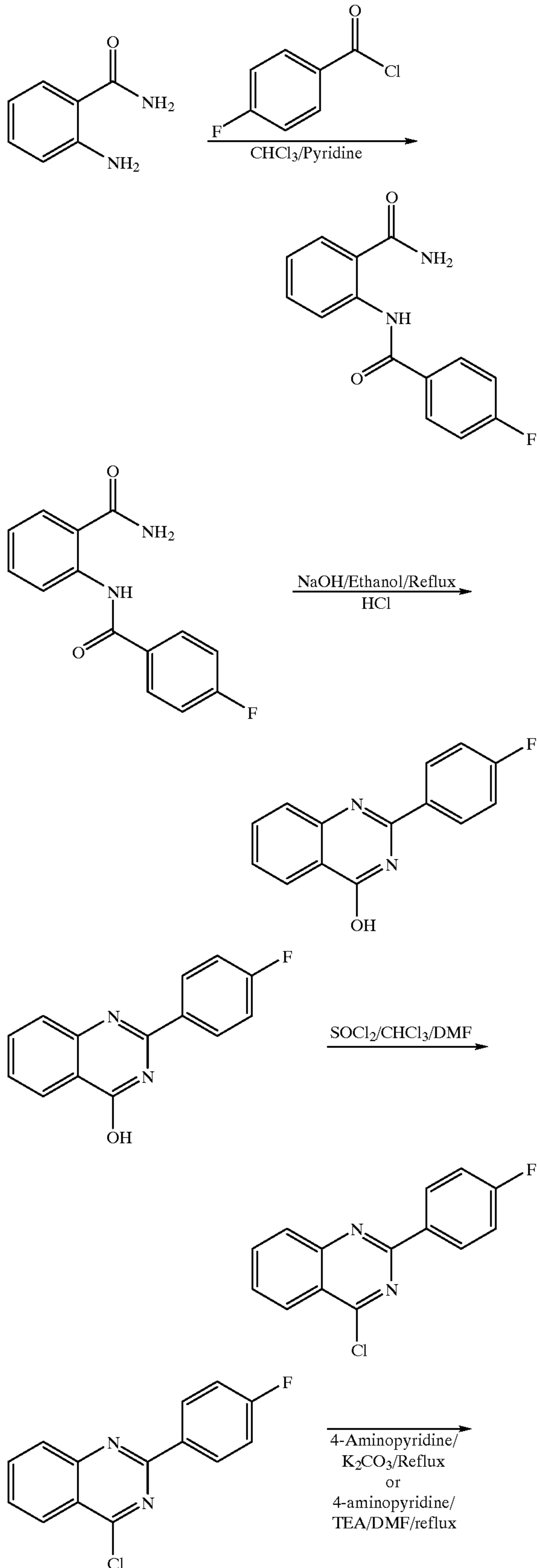
Reaction Scheme 3
