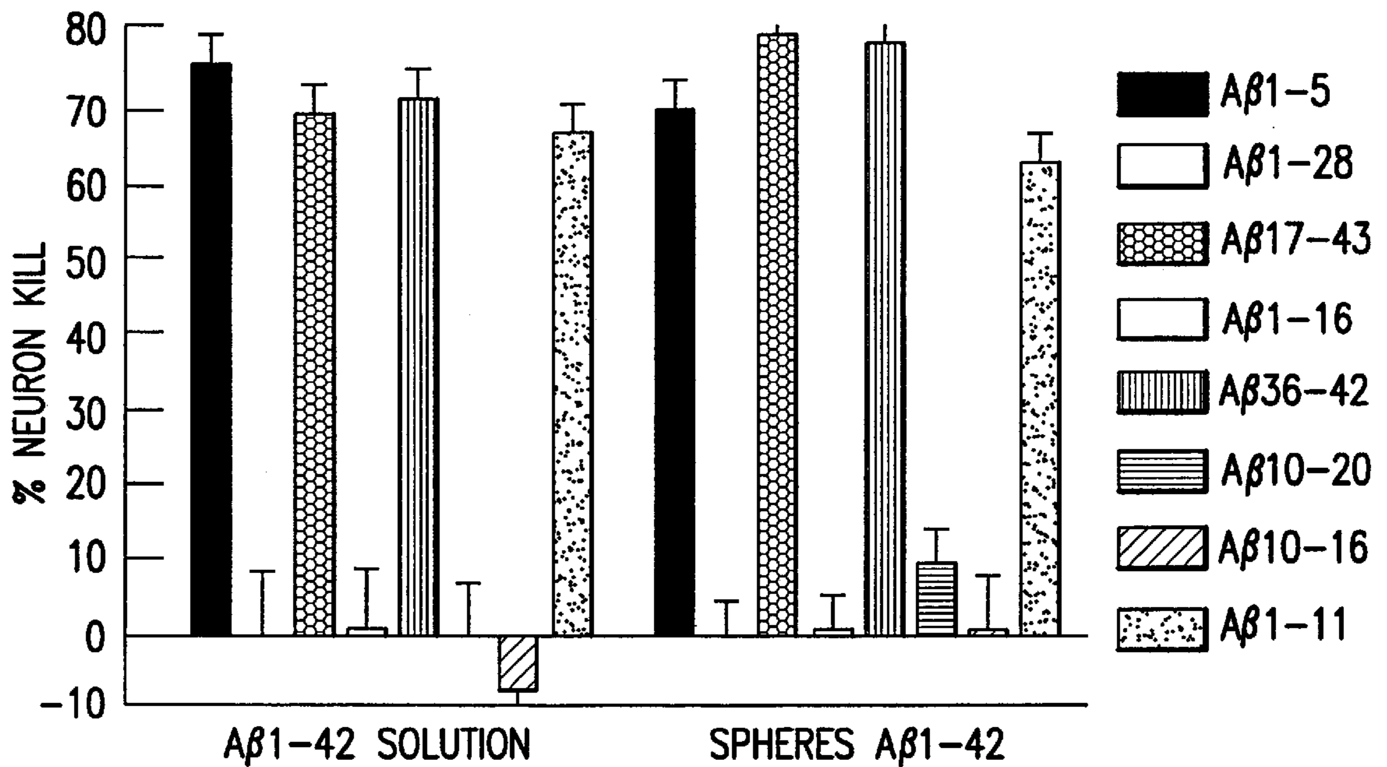
FORMS OF Aβ
