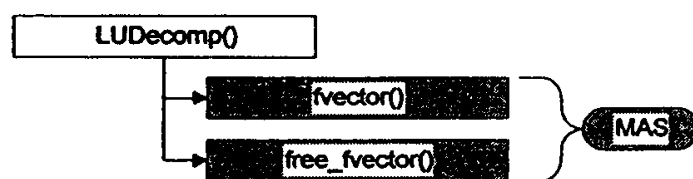
Figure 19 LUDecomp() Subordinates
