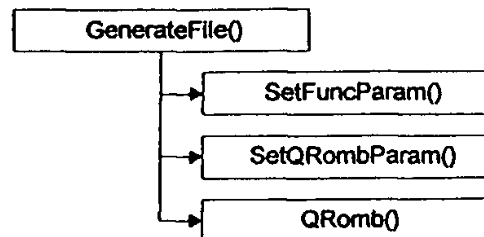
Figure 39 GenerateFile() Subordinates
