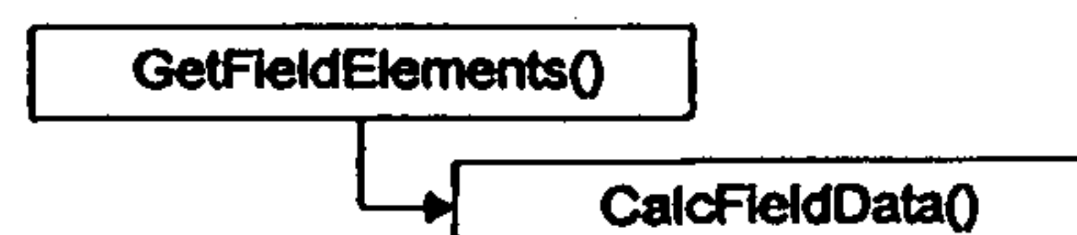
Figure 33 GetFieldElements() Subordinates
