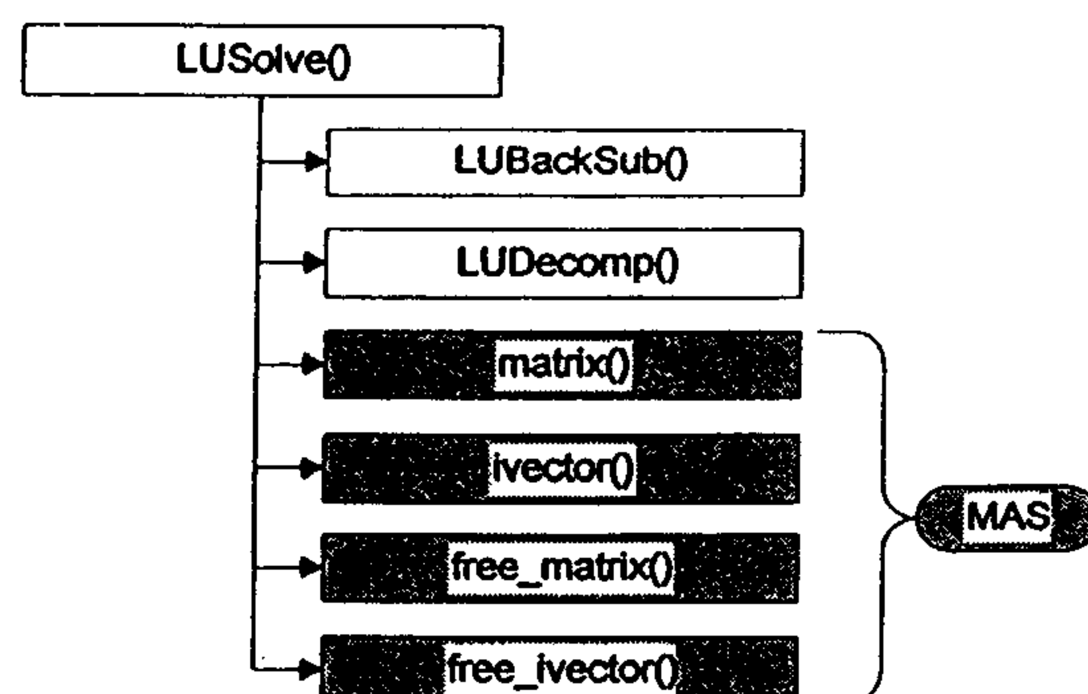
Figure 20 LUSolve() Subordinates
