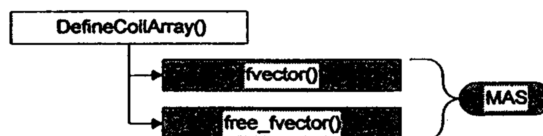
Figure 37 DefineCoilArray() Subordinates
