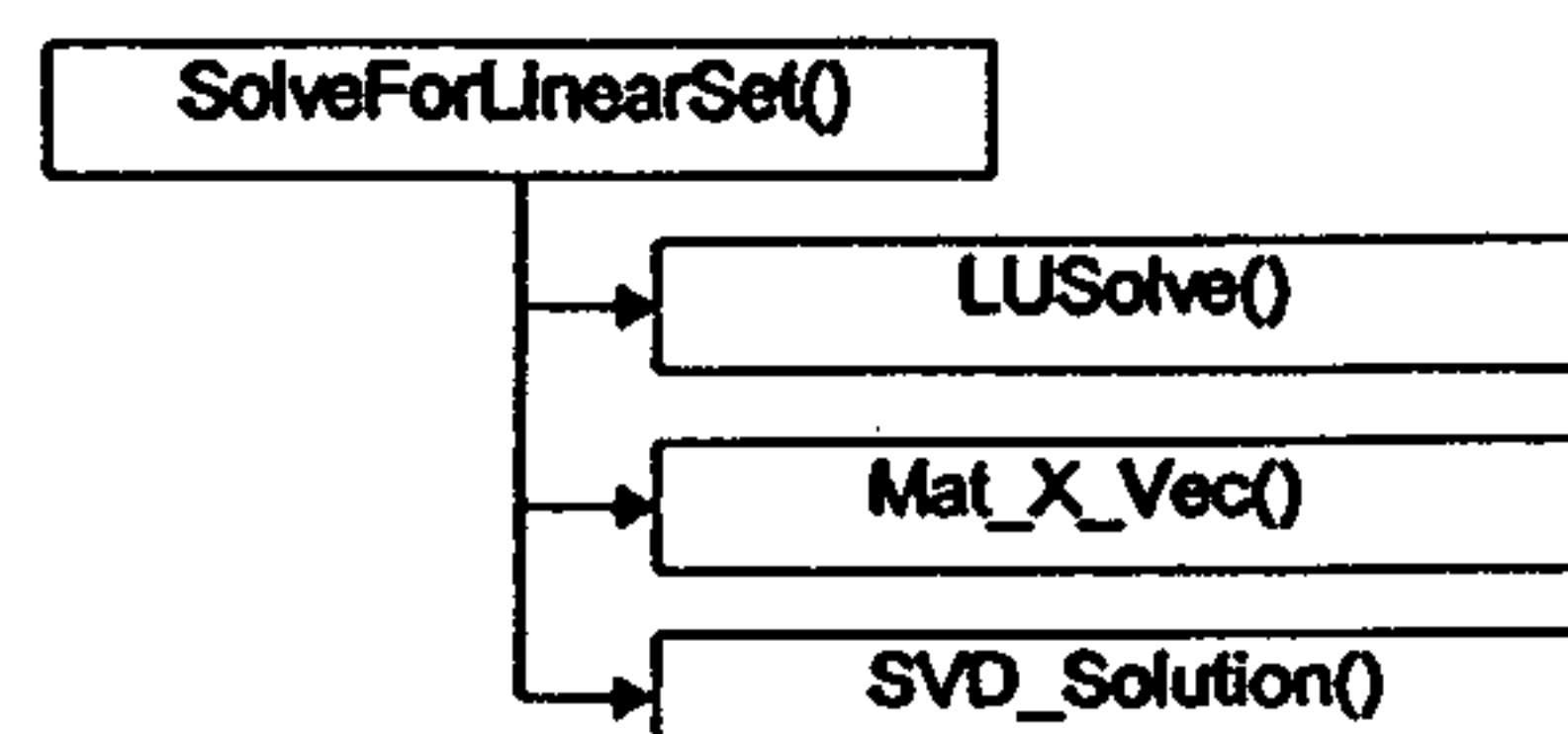
Figure 22 SolveForLinearSet() Subordinates
