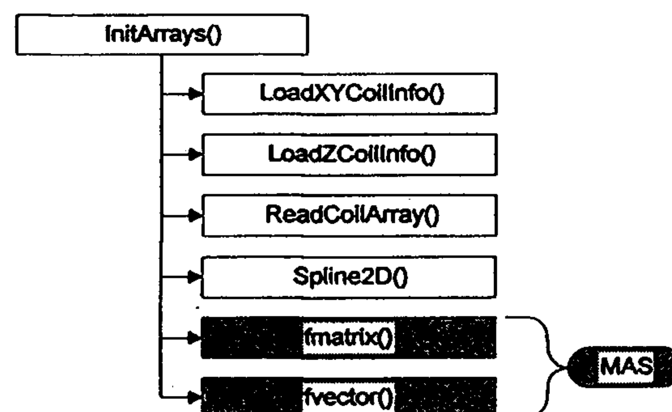
Figure 36 InitArrays() Subordinates
