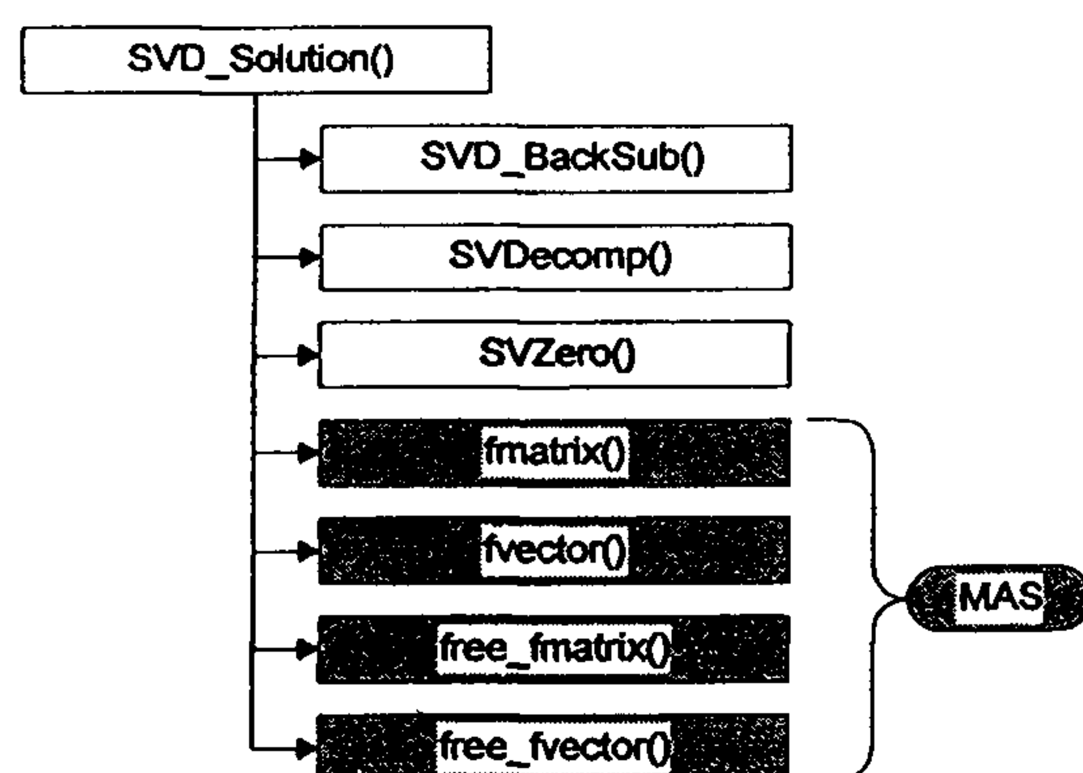
Figure 23 SVD_Solution() Subordinates
