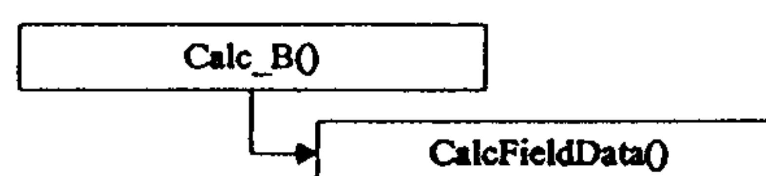
Figure 25 Calc_B() Subordinates
