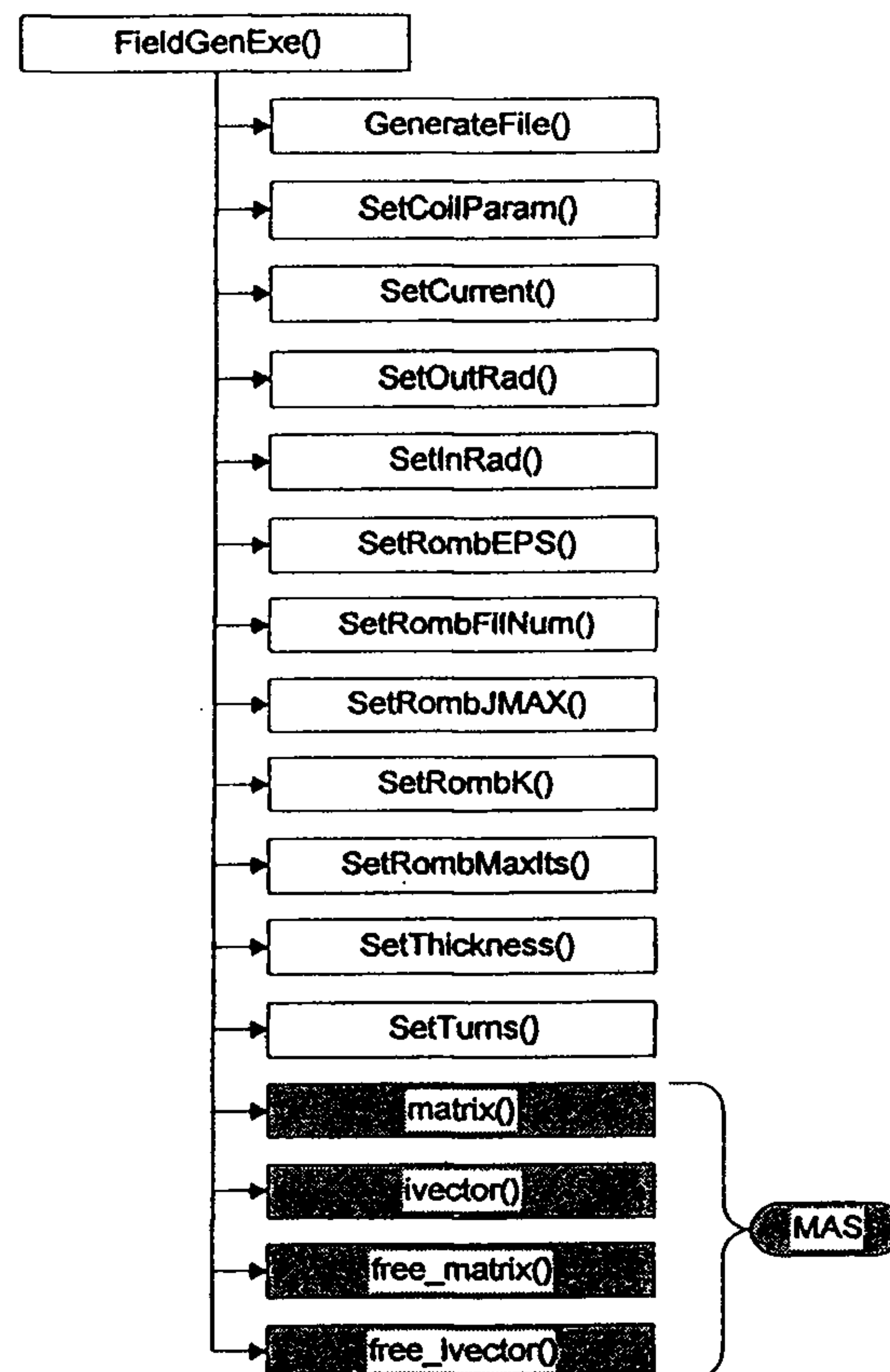
Figure 38 FieldGenExe() Subordinates
