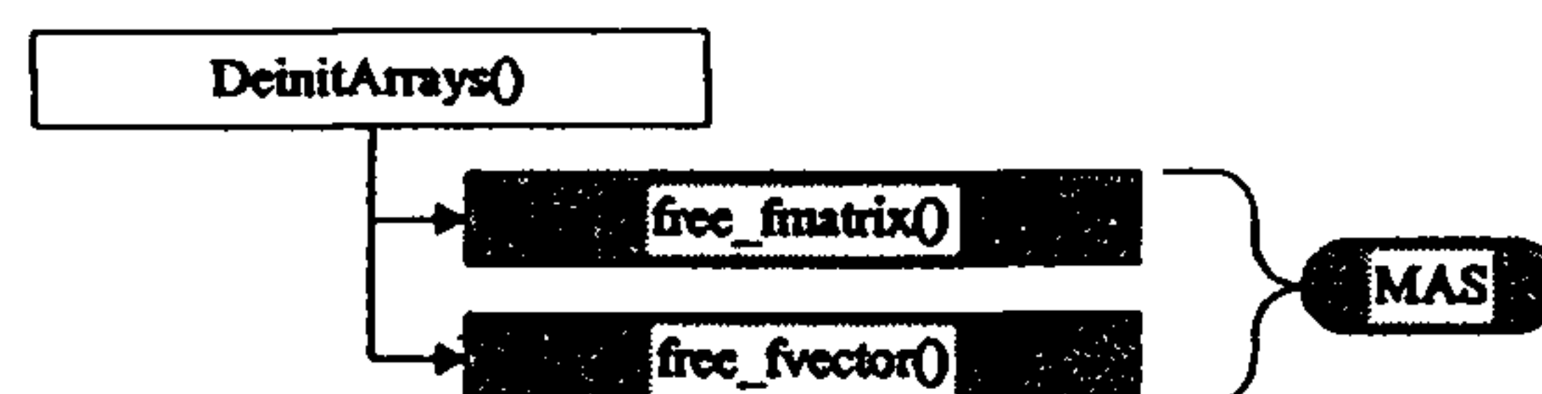
Figure 32 DeinitArrays() Subordinates
