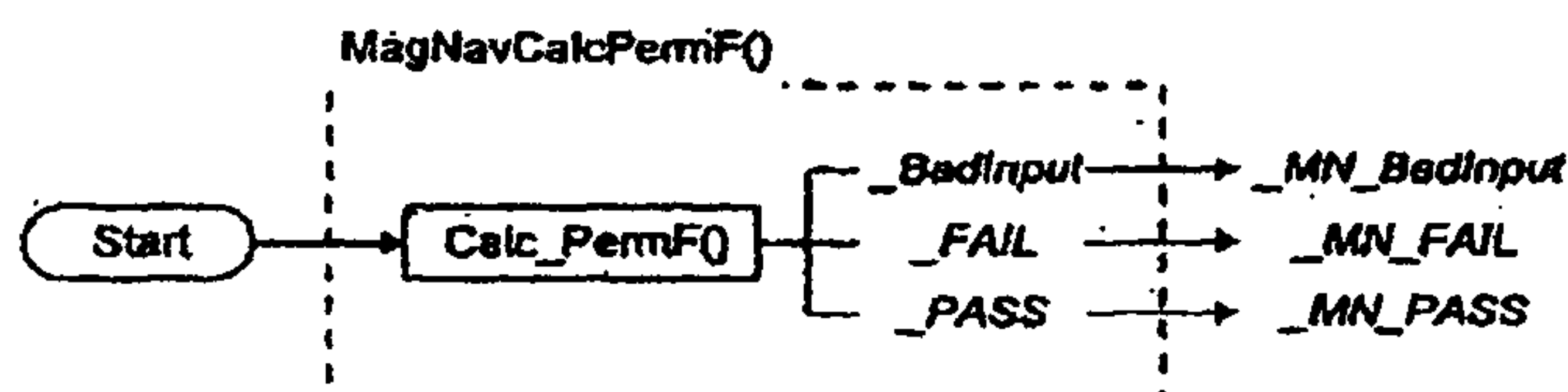
Figure 7 Error Decomposition of MagNavCalcPermF()
