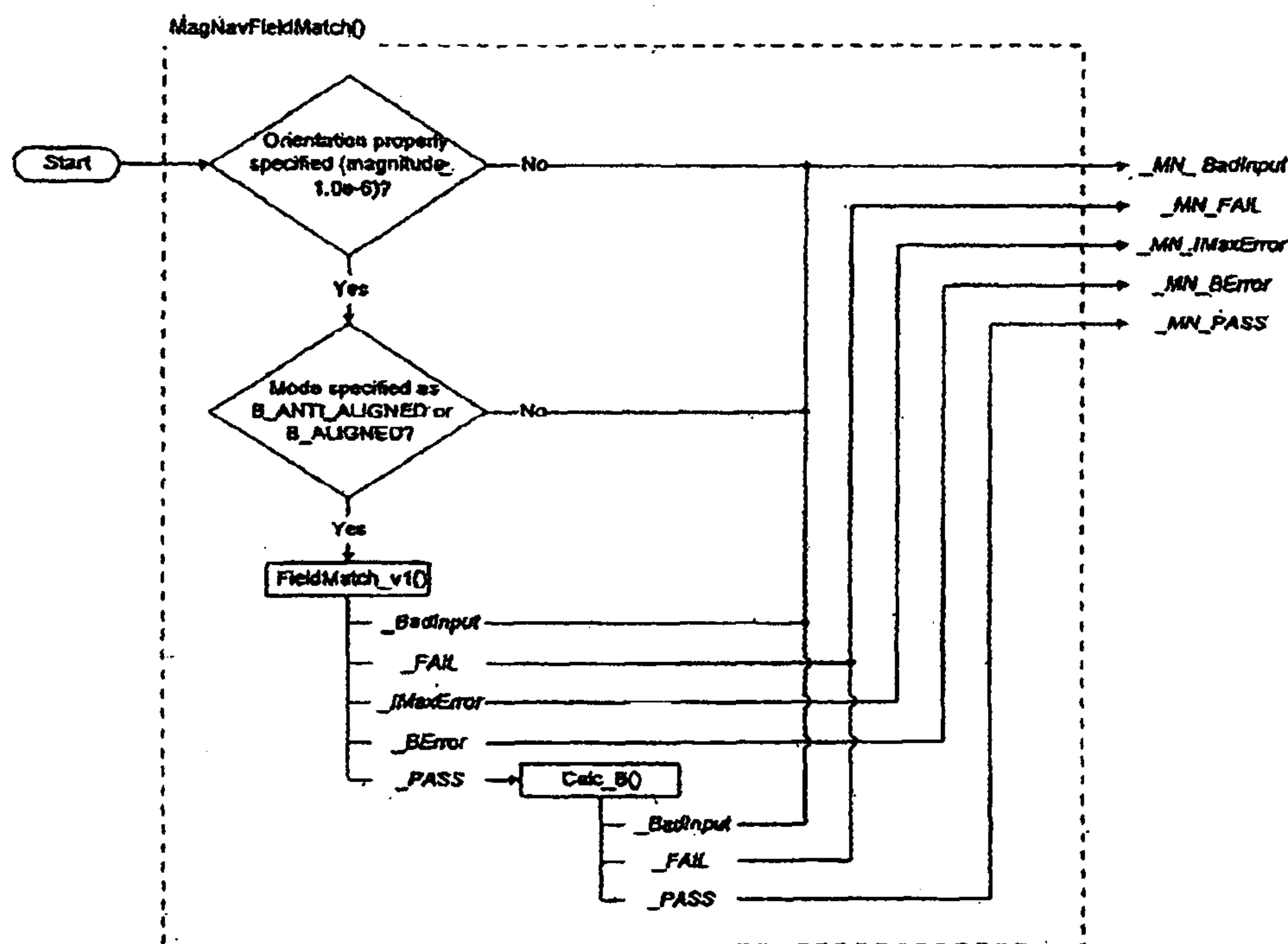
Figure 10 Error Decomposition of MagNavFieldMatch()
