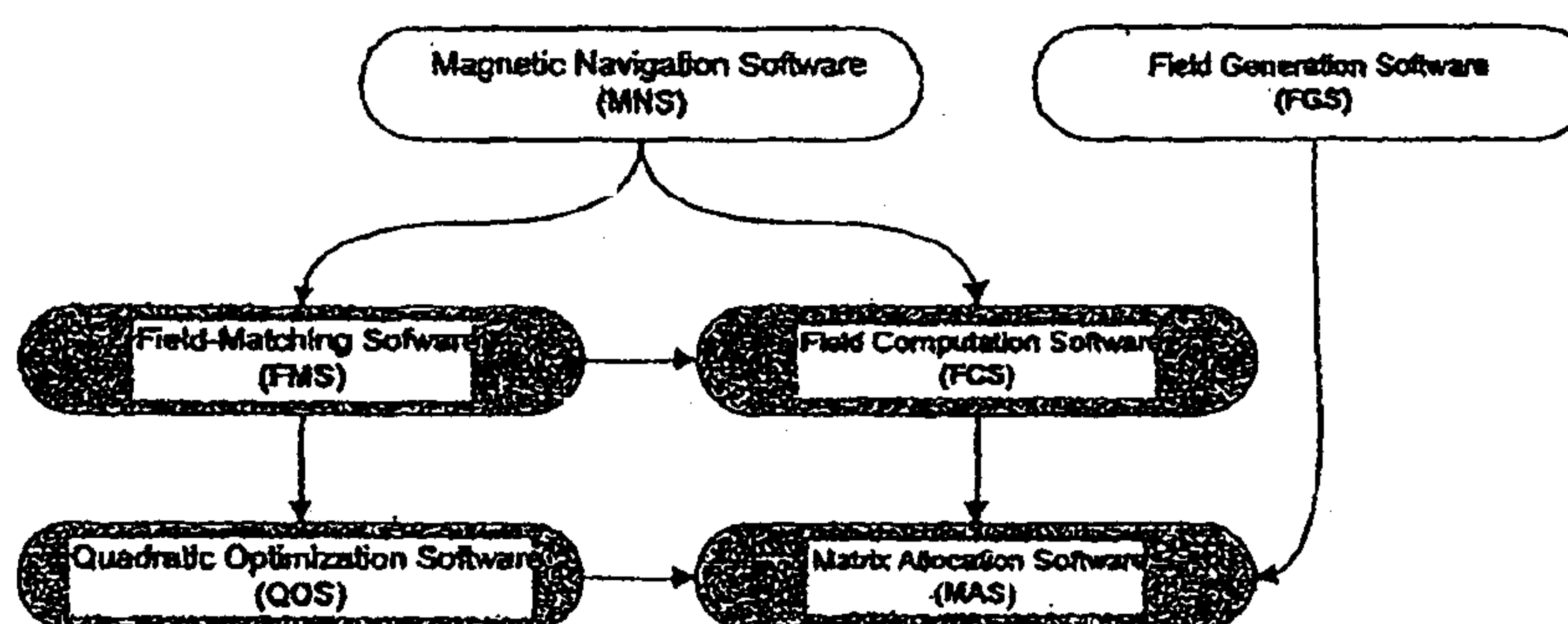
Figure 1. Magnetic Navigation Software Dependency
