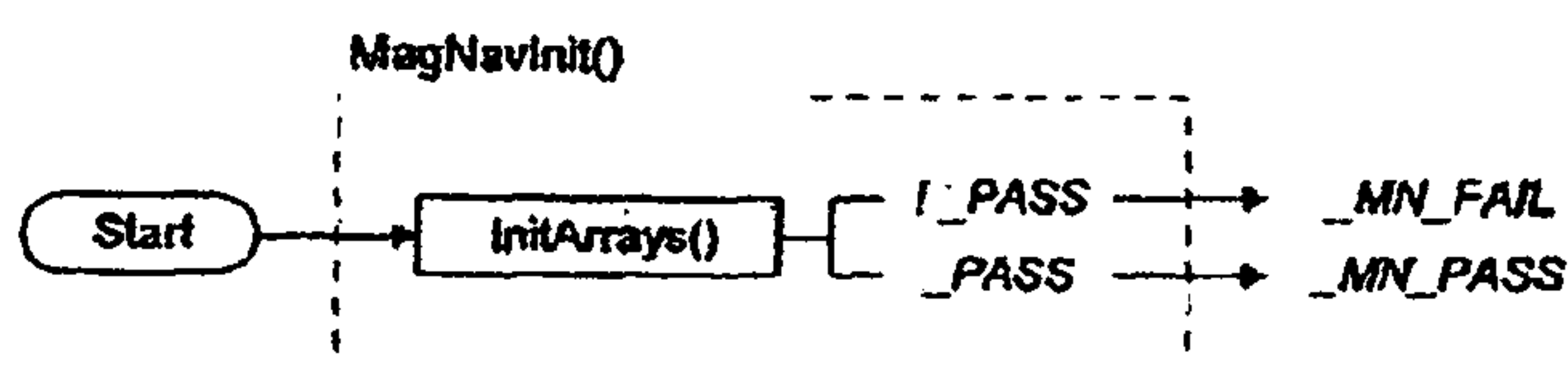
Figure 12 Error Decomposition of MagNavInit()
