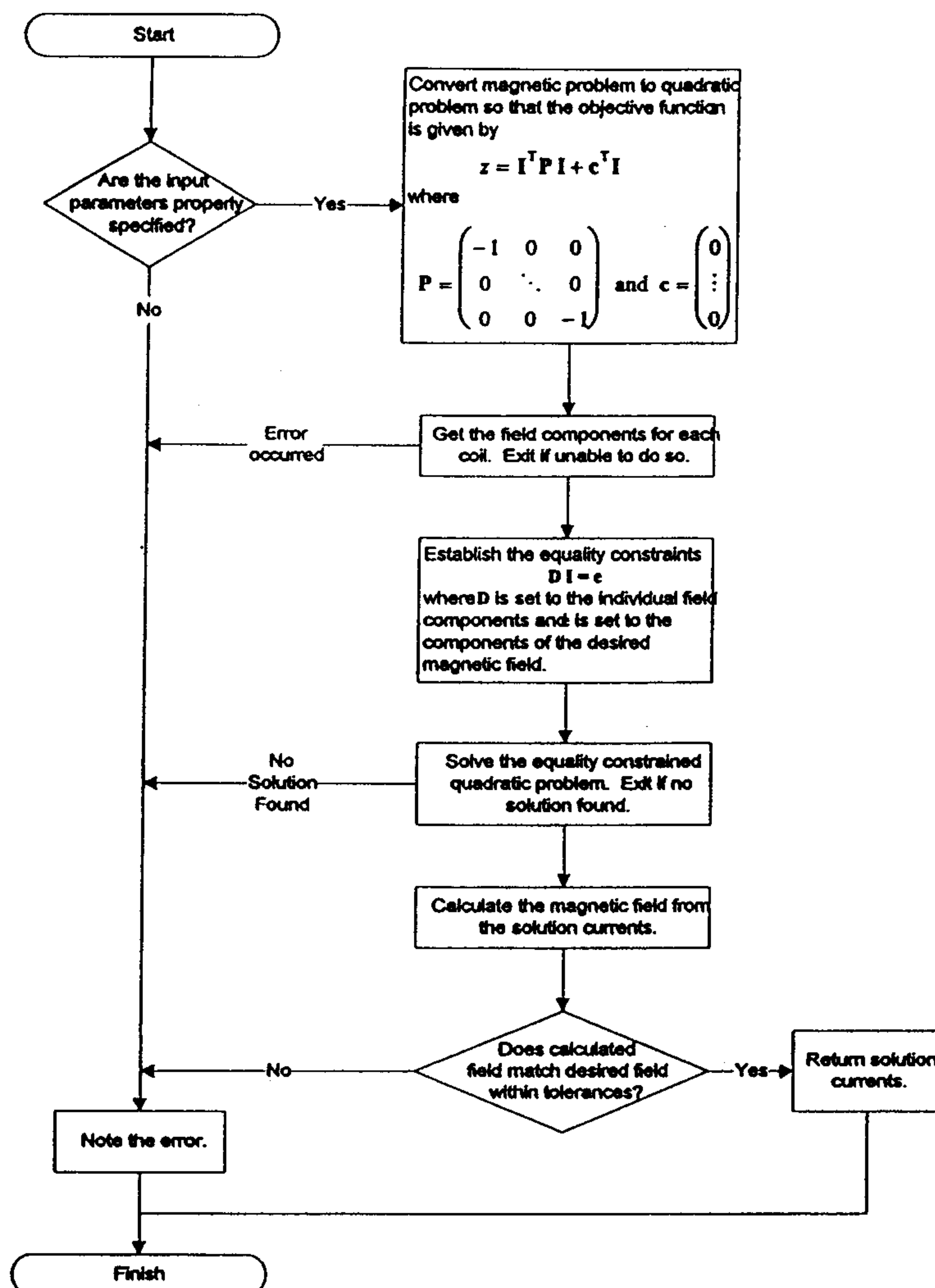
Figure 17 Flowchart of FieldMatch_v10
