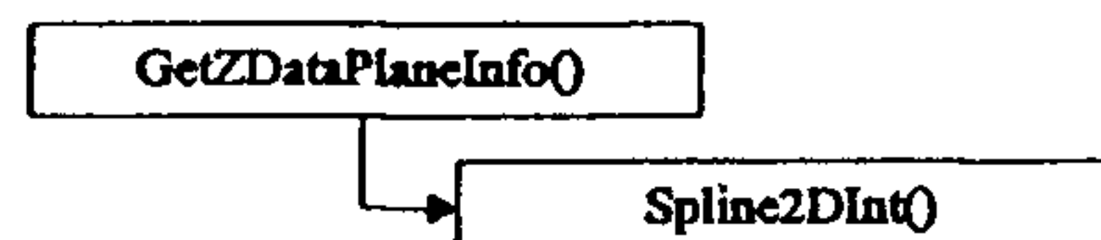
Figure 35 GetZDataPlaneInfo() Subordinates
