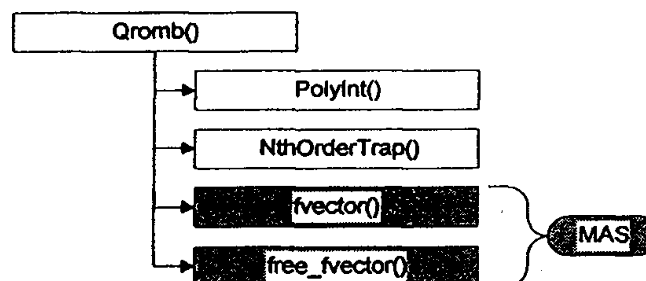
Figure 40 QRomb() Subordinates
