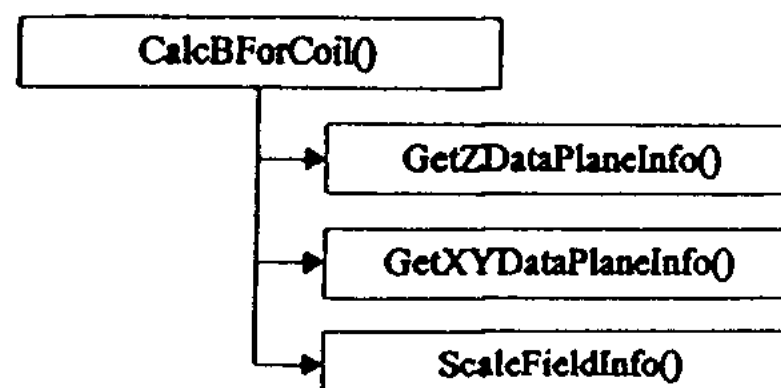
Figure 30 CalcBForCoil() Subordinates
