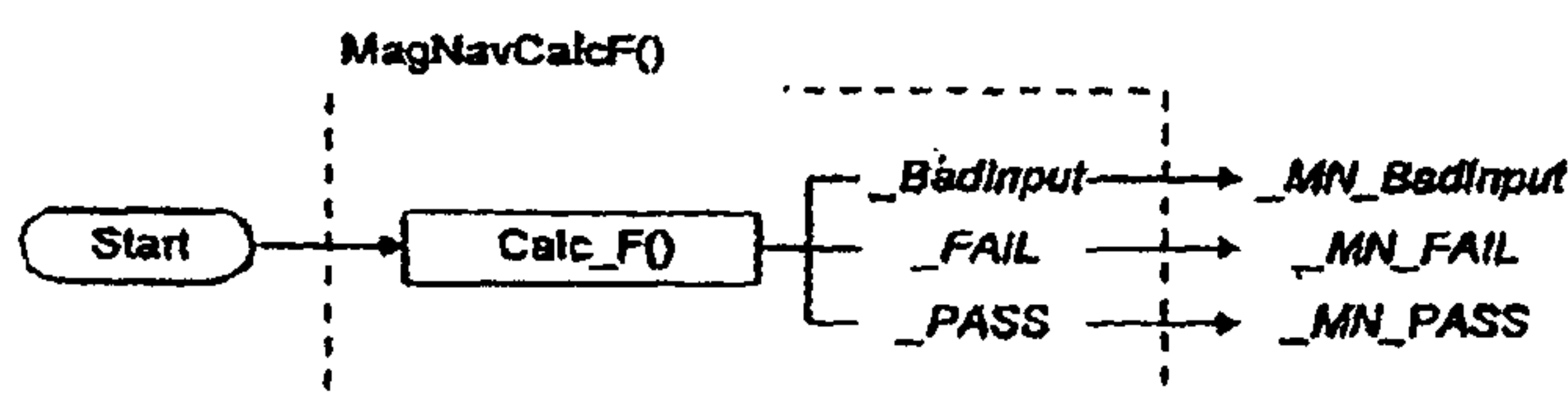
Figure 5 Error Decomposition of MagNavCalcF()
