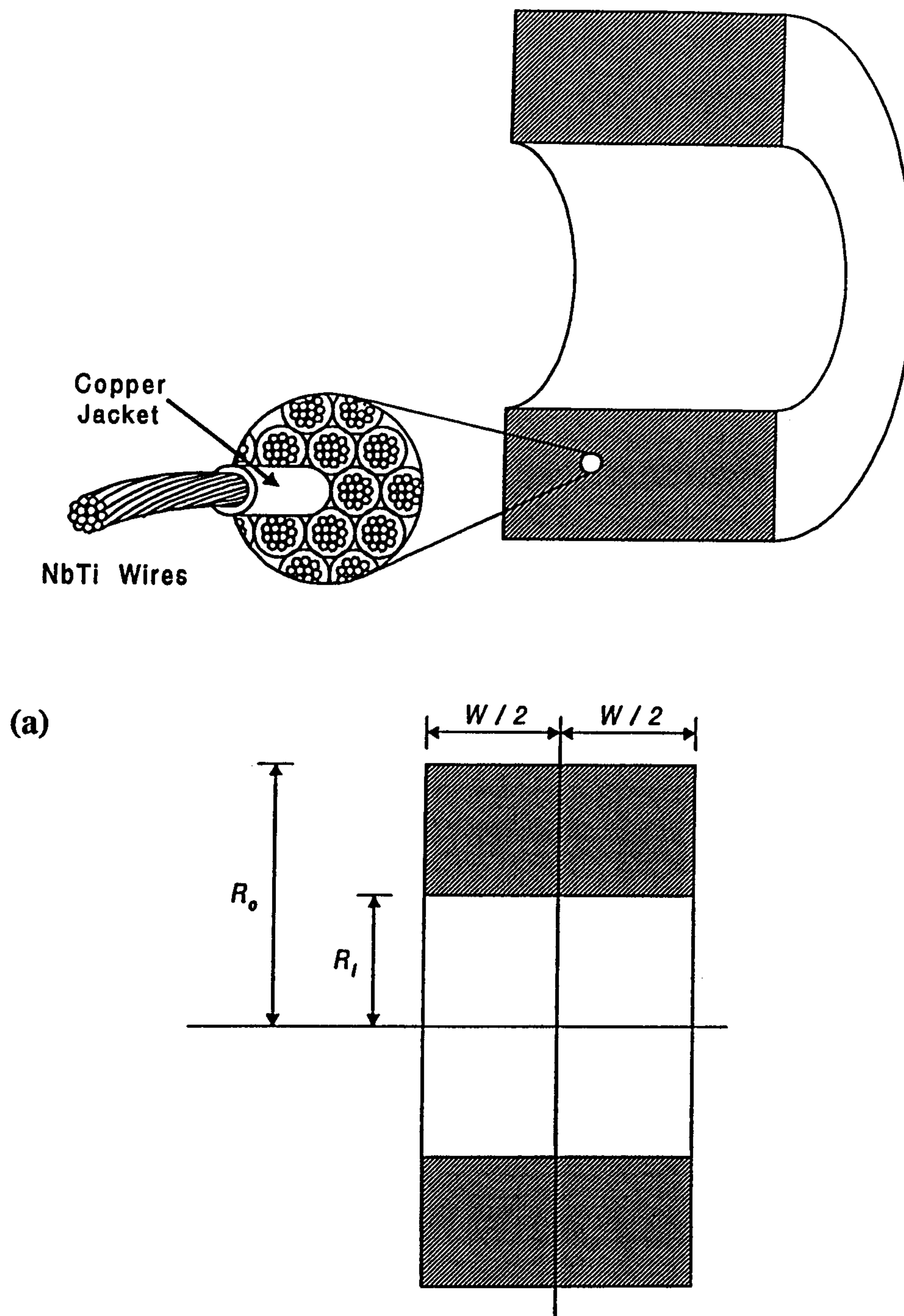
(b) FIG. 3-3. Depiction of (a) the cross section (shaded) and (b) the width, W , and inner and outer radii, R_i and R_o , respectively, of a circular coil. Figure (a) also depicts a cross-sectional element consisting of the copper encased (i.e., thermally-lagged) NbTi windings that carry the current. The relatively high number of windings allows the current density to be approximated as being uniform.
