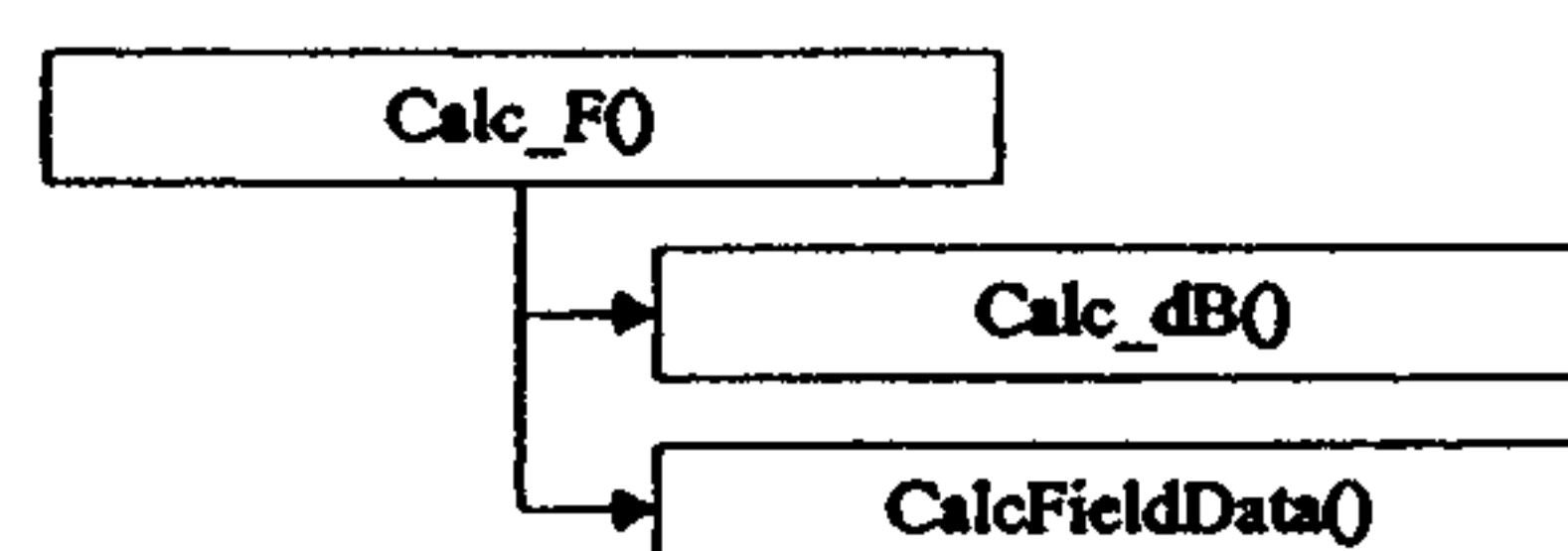
Figure 29 Calc_F() Subordinates
