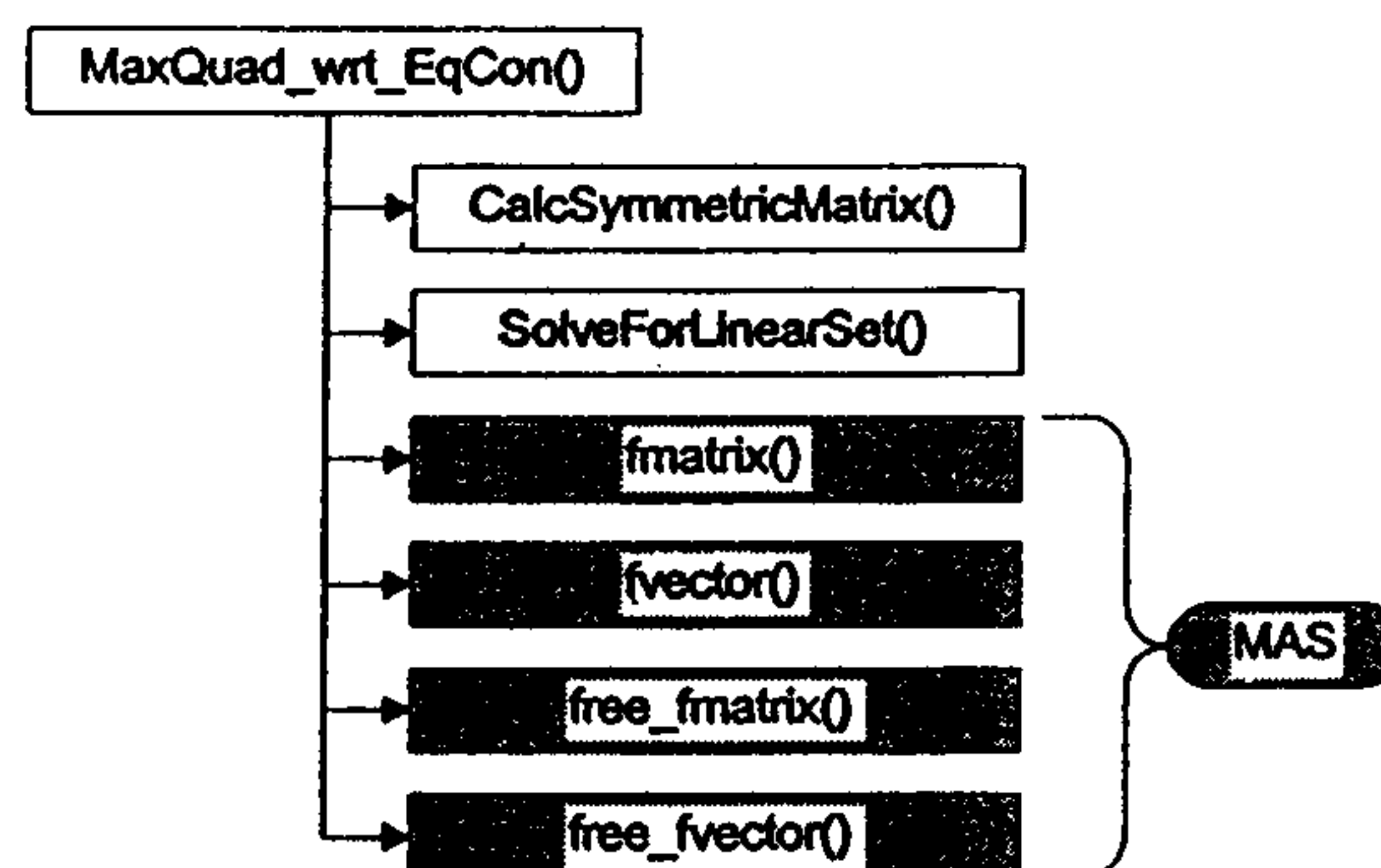
Figure 21 MaxQuad_wrt_EqCon() Subordinates
