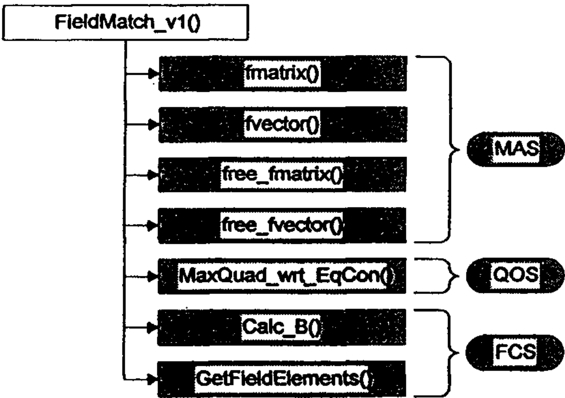
Figure 16 FieldMatch_v1() Subordinates
