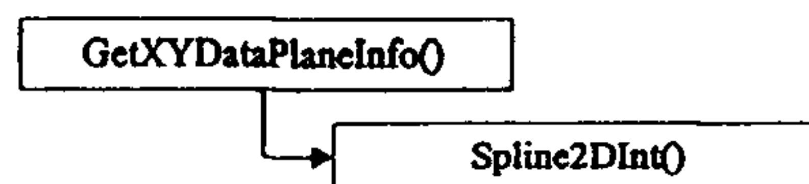
Figure 34 GetXYDataPlaneInfo() Subordinates
