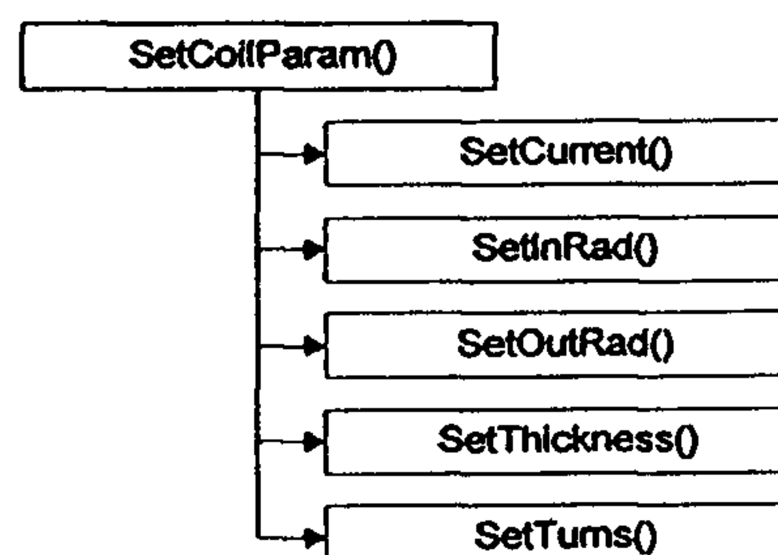
Figure 41 SetCoilParam() Subordinates
