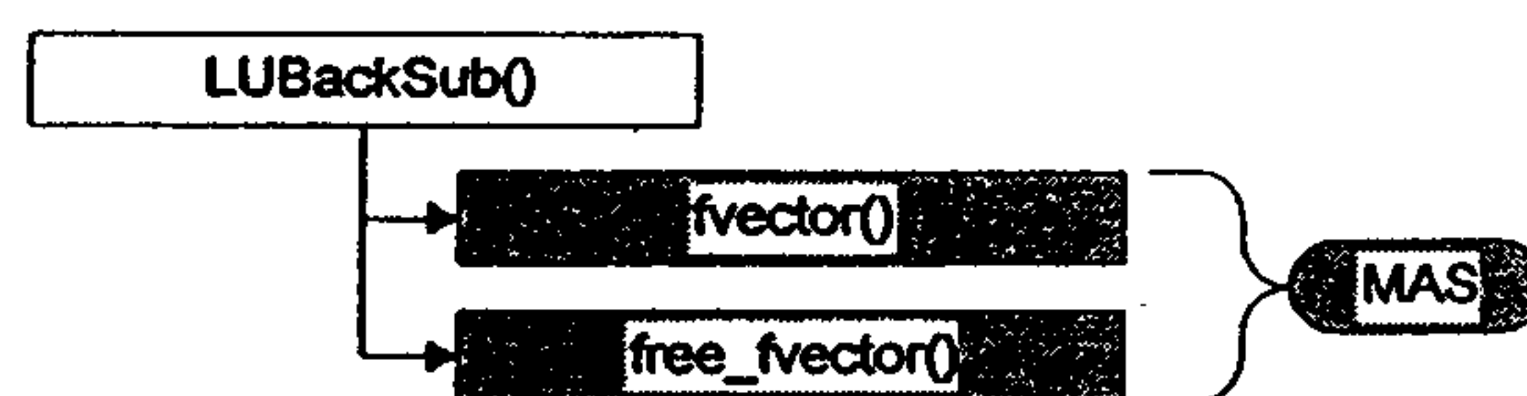
Figure 18 LUBackSub() Subordinates
