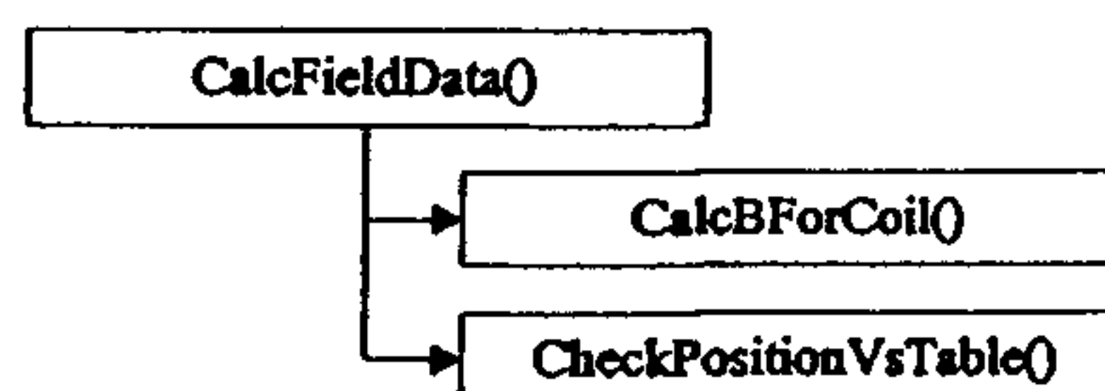
Figure 31 CalcFieldData() Subordinates
