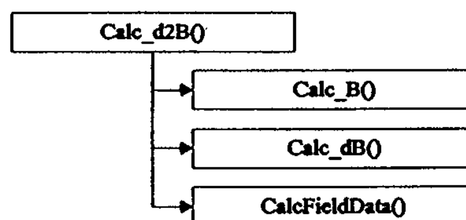
Figure 26 Calc_d2B() Subordinates
