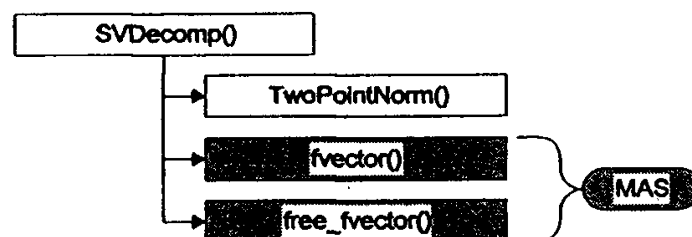
Figure 24 SVDDecomp() Subordinates
