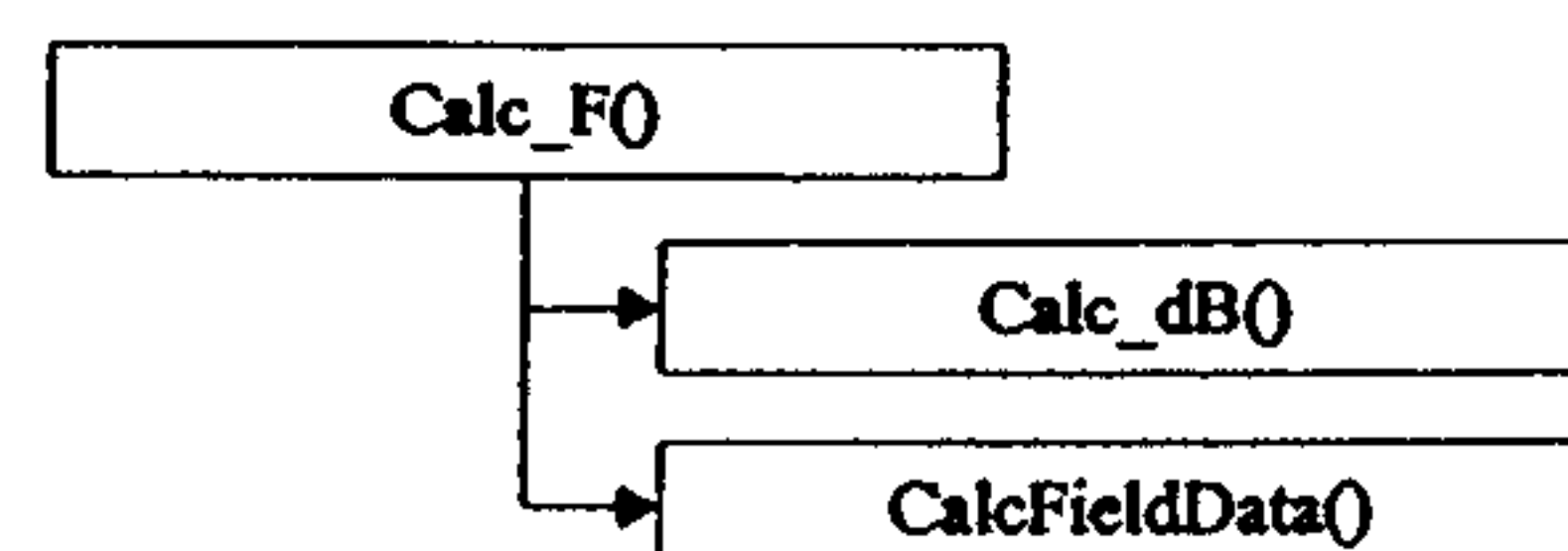
Figure 28 Calc_F() Subordinates
