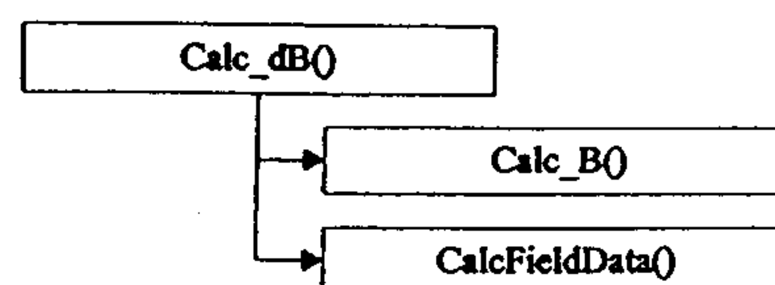
Figure 27 Calc_dB() Subordinates
