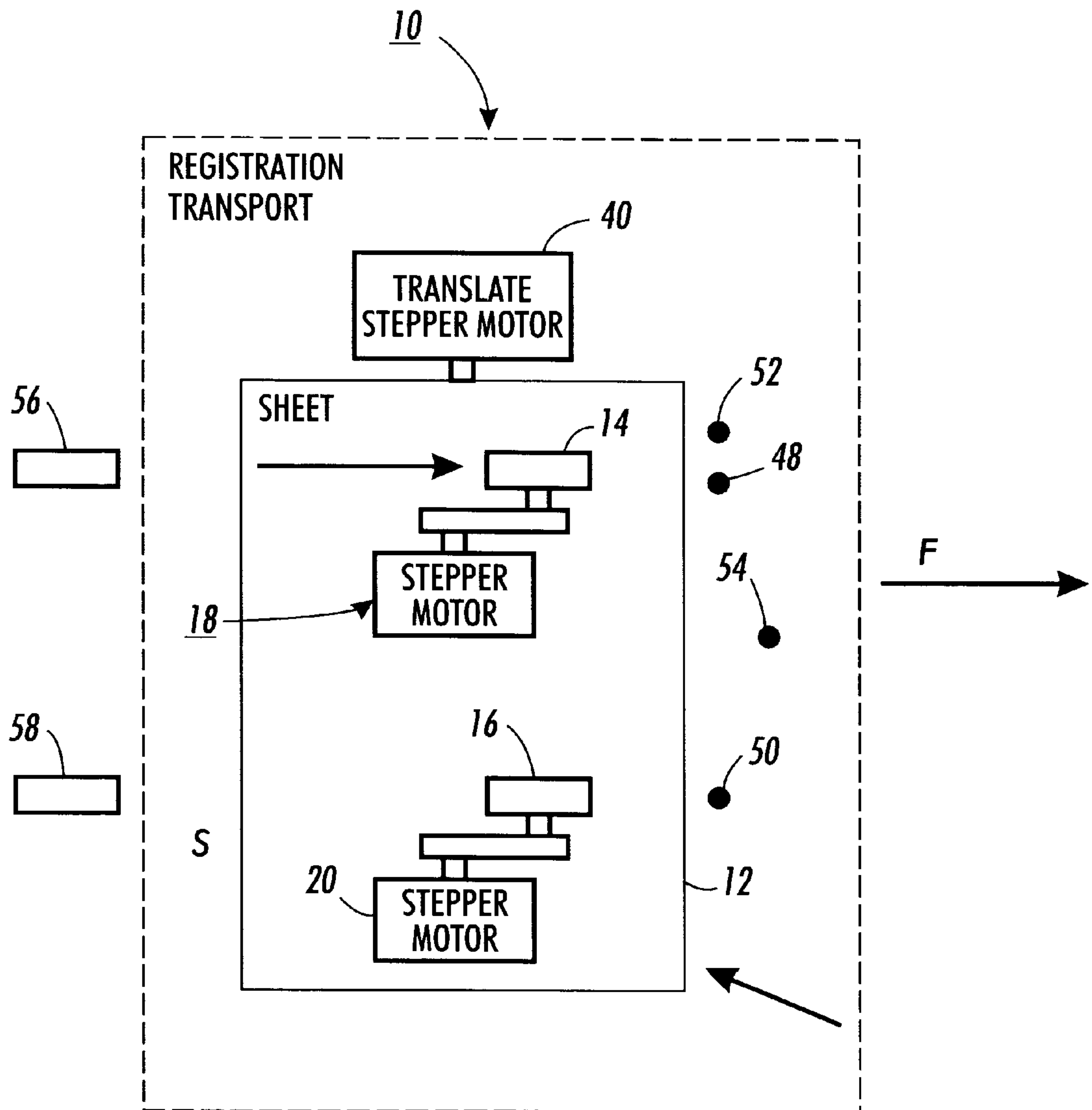
FIG. 3 (Prior Art)
