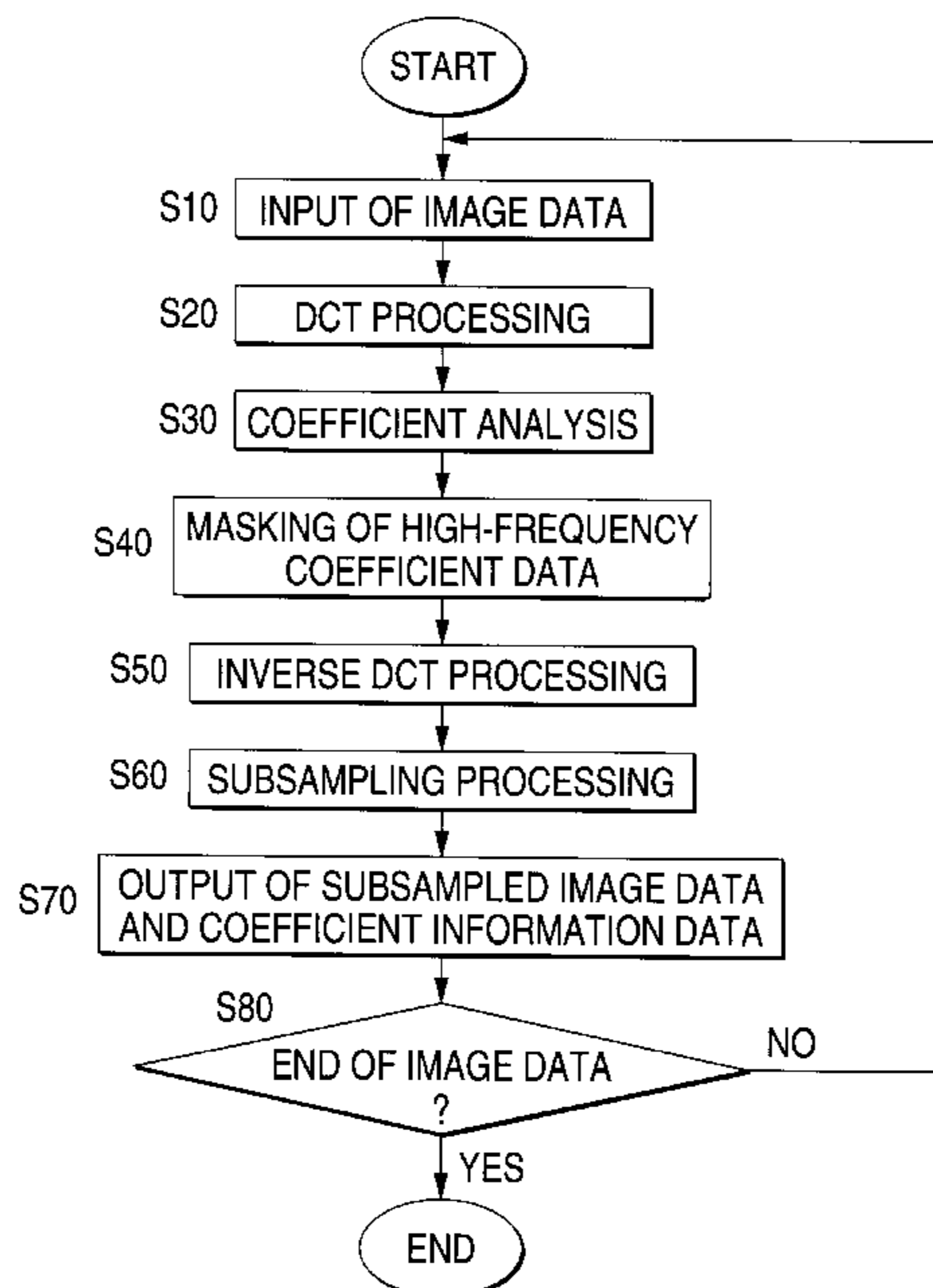
1ST EMBODIMENT / ENCODING PROCEDURE
