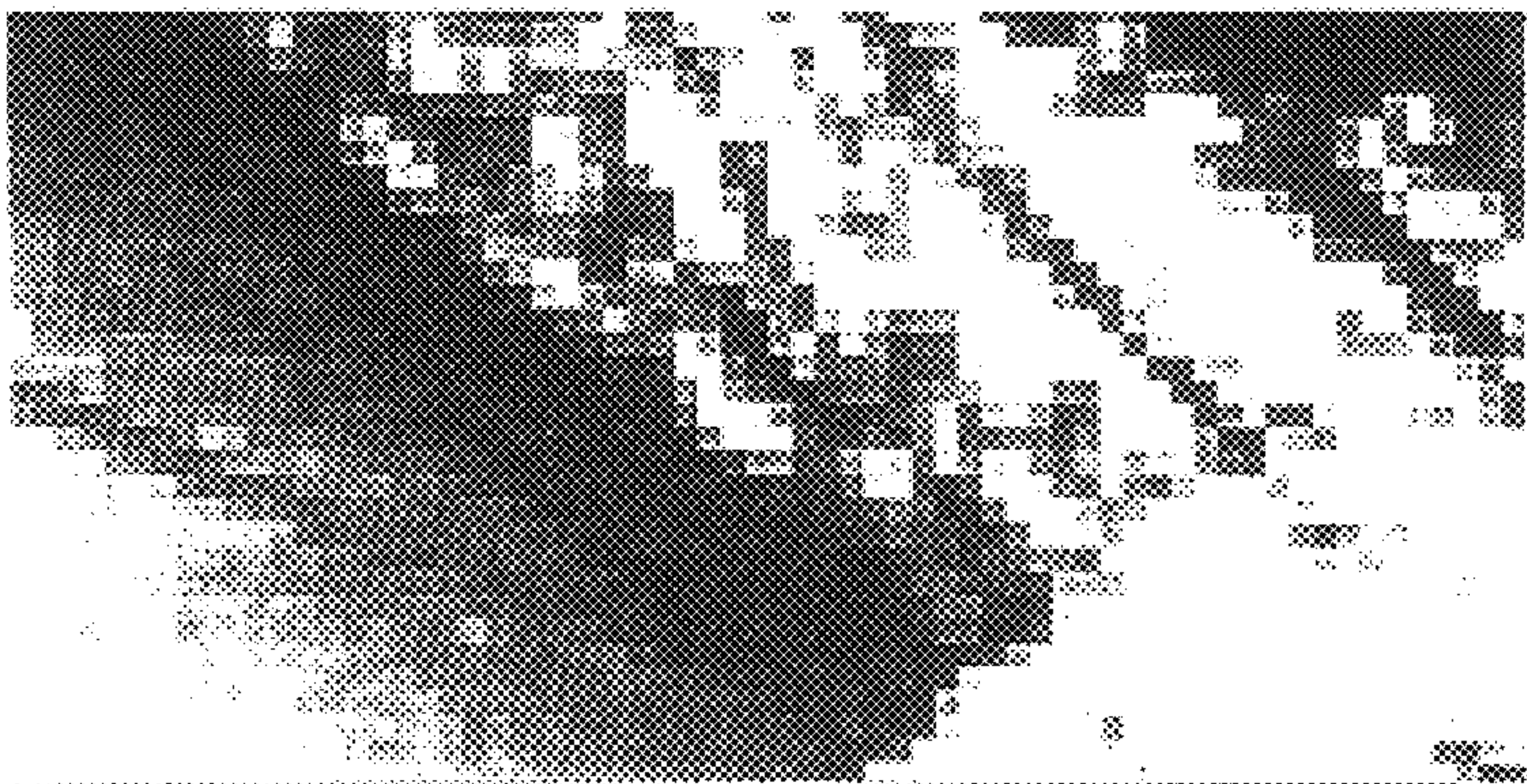
INPUT IMAGE
