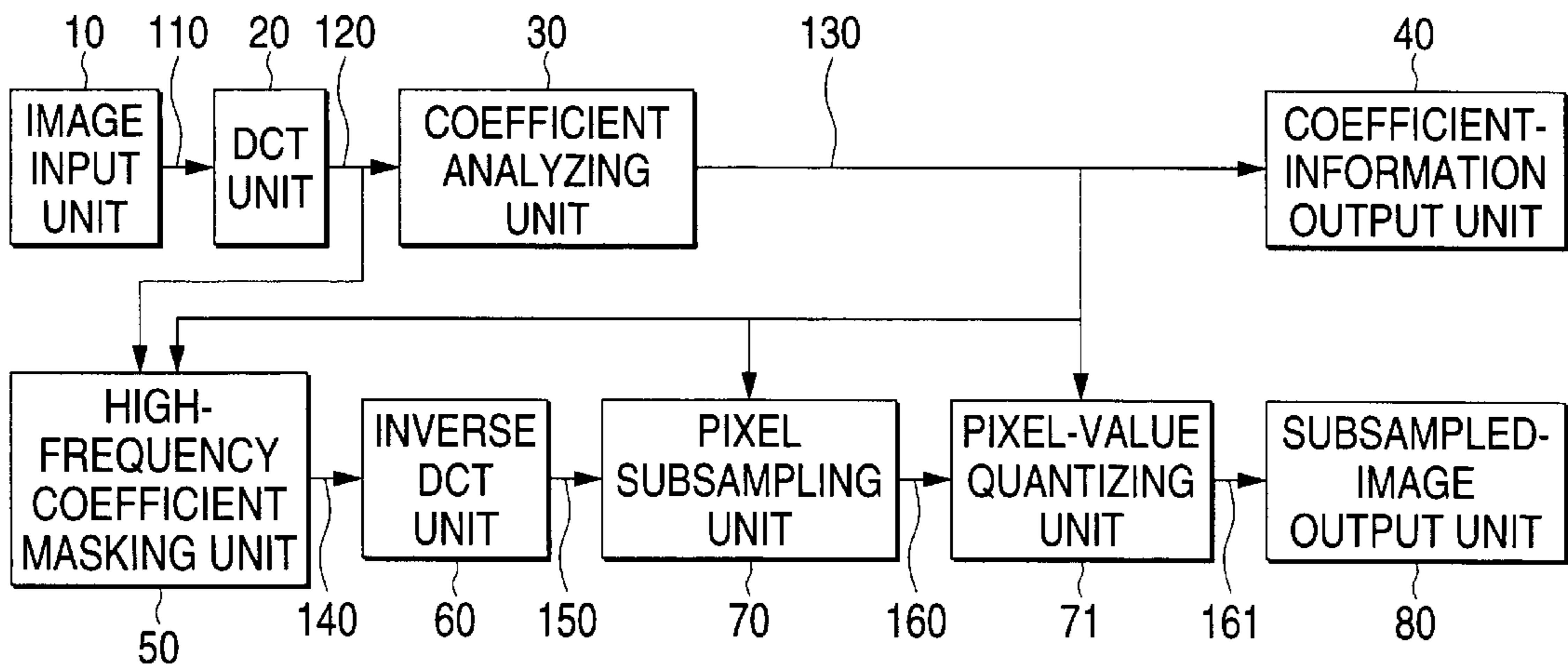
ENCODING APPARATUS FOR QUANTIZING PIXEL VALUES
