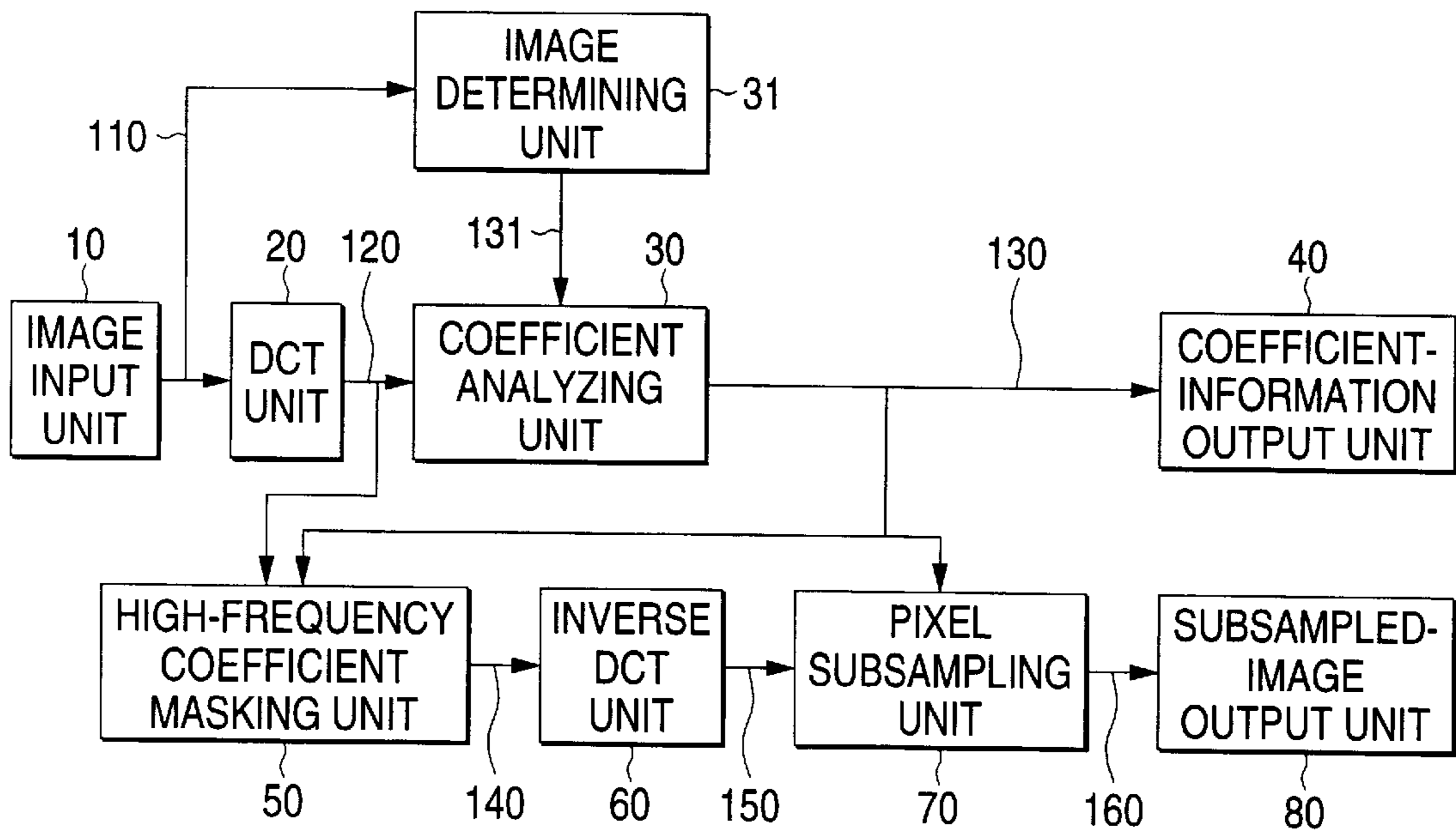
ENCODING APPARATUS FOR DYNAMICALLY CHANGING THRESHOLDS
