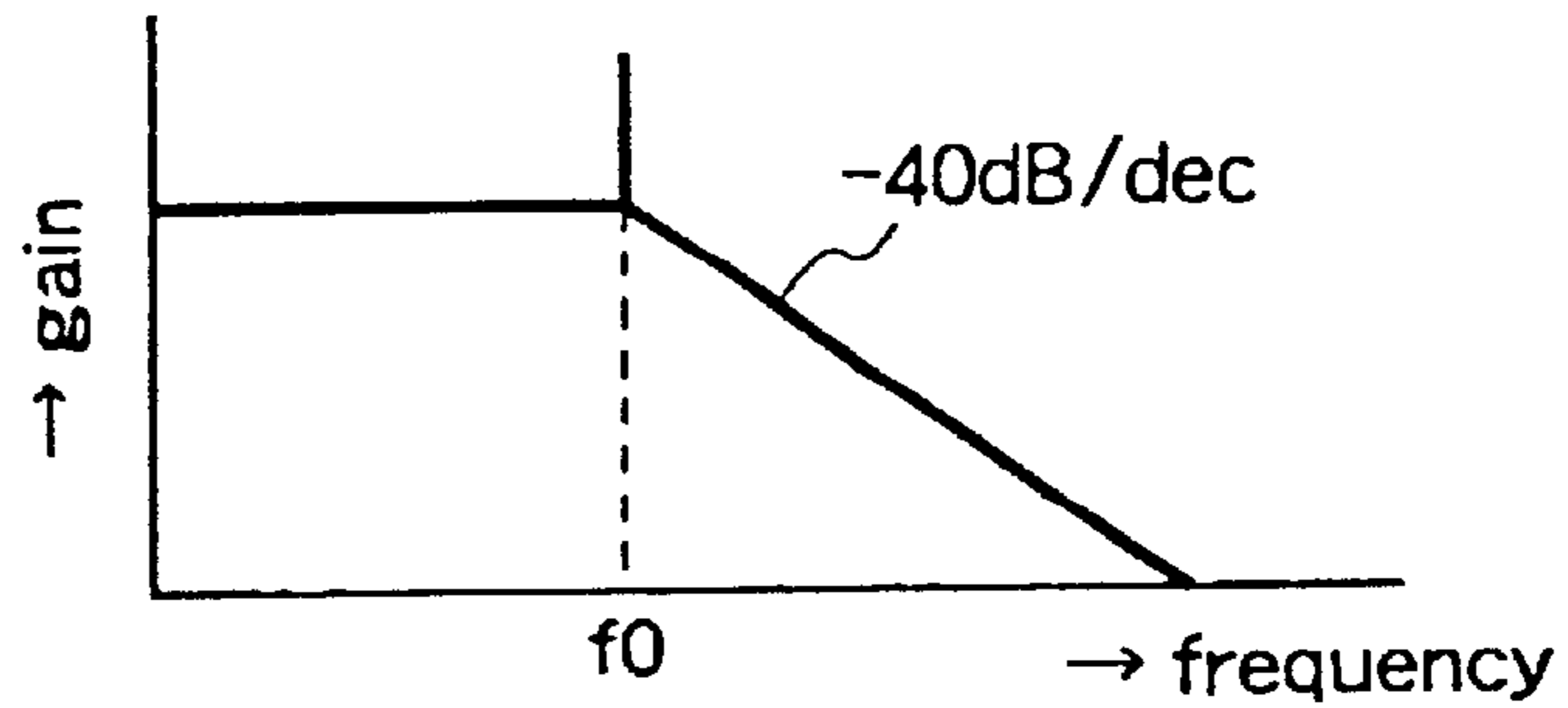
Fig.19 (a) open-loop gain characteristics without spot position loop filter 111
