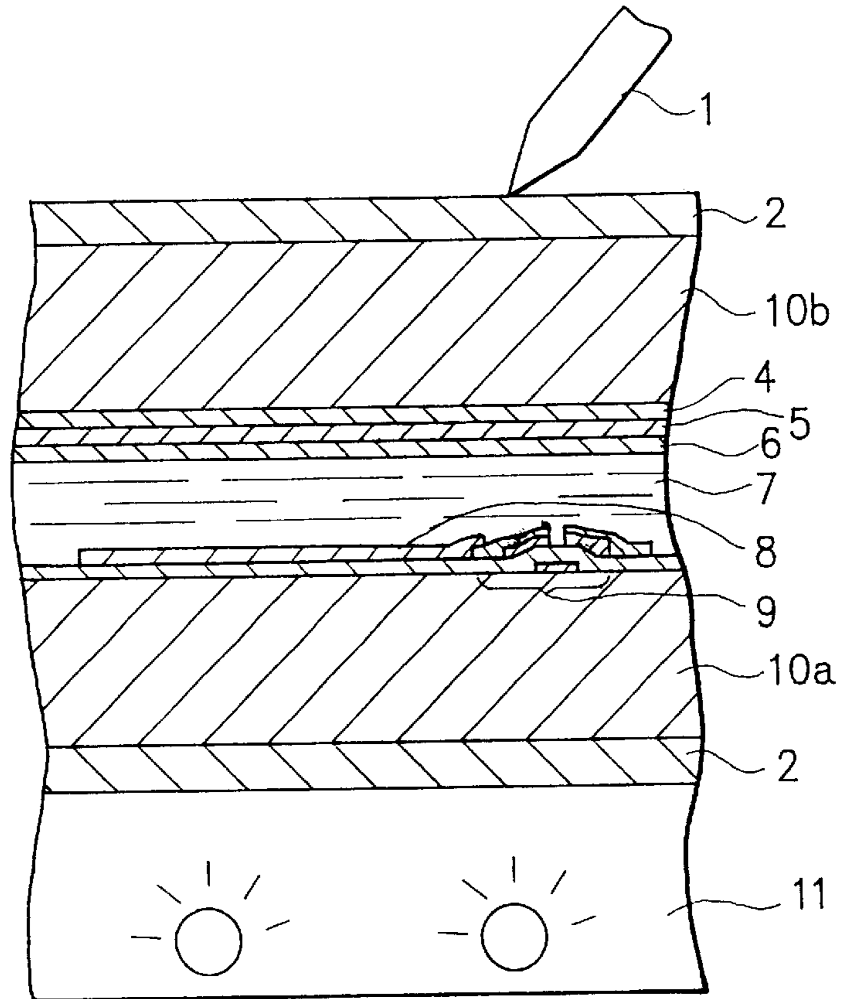
FIG. 1 PRIOR ART
