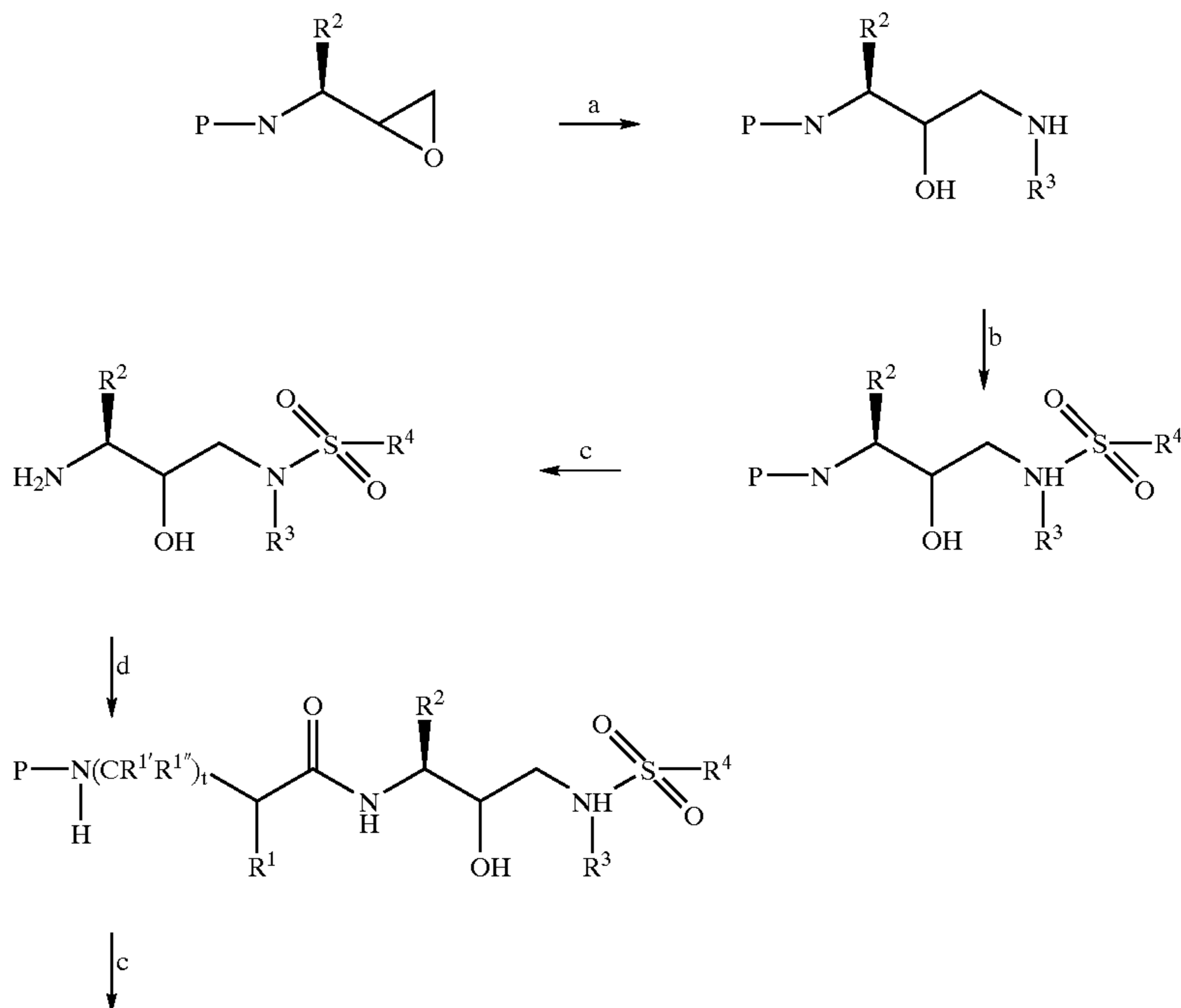
SCHEME I
