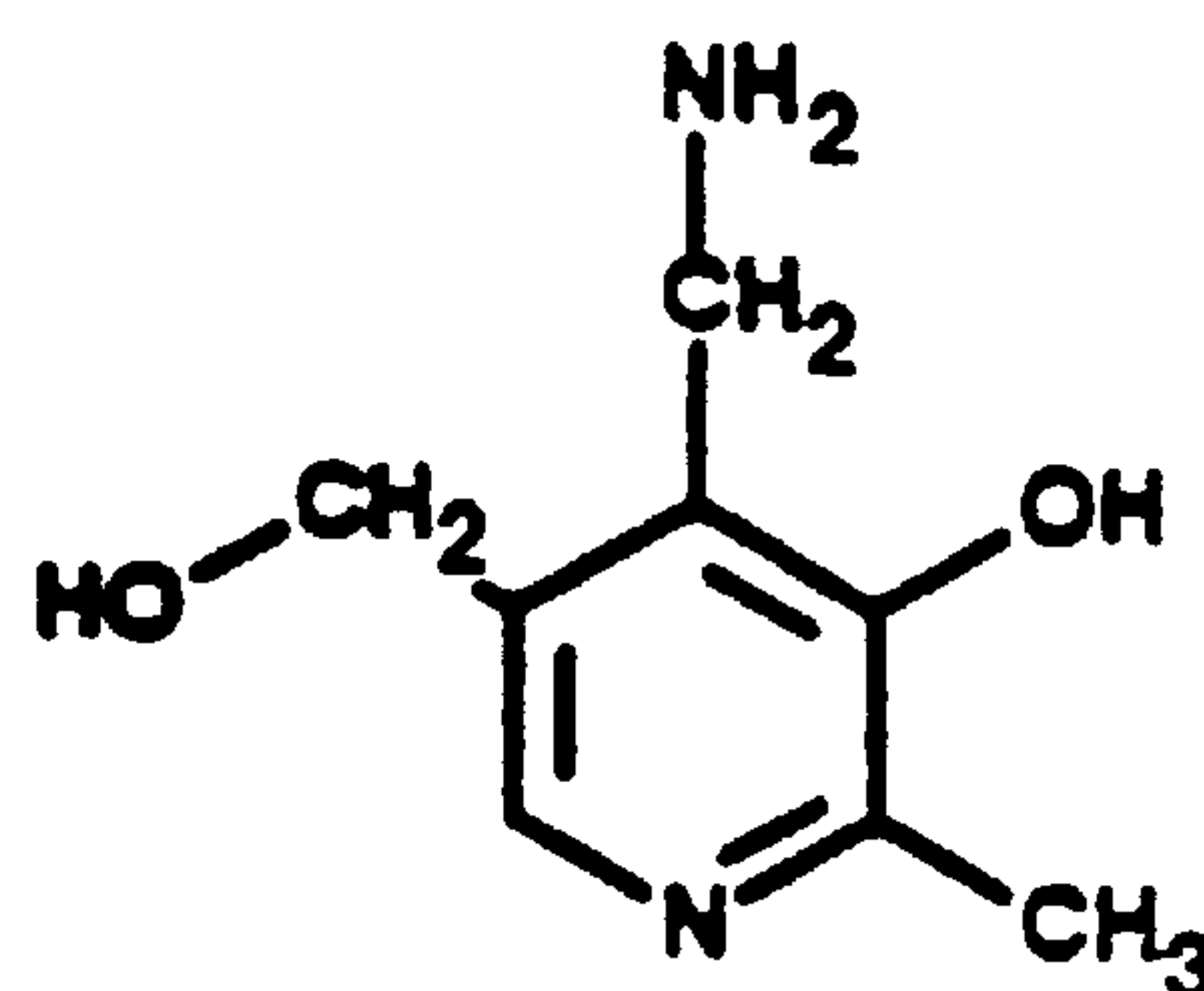
Pyridoxamine
