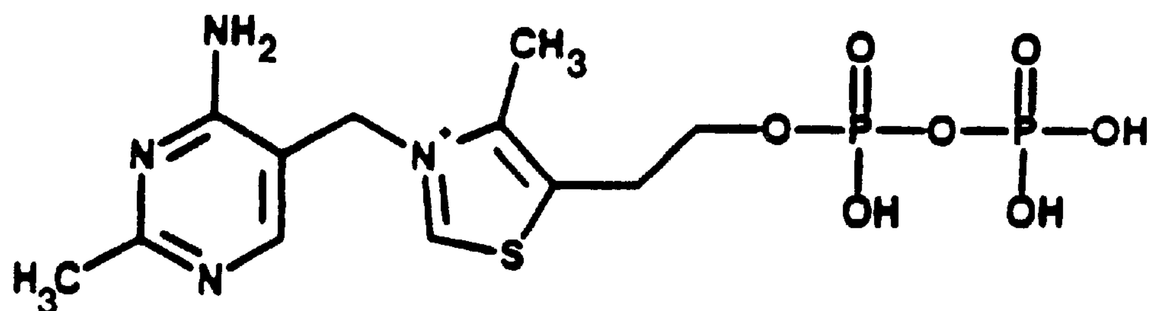
Thiamine Pyrophosphate
