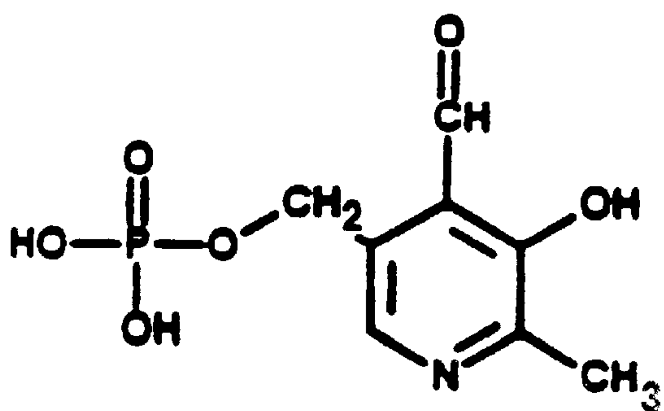
Pyridoxal-5'-Phosphate
