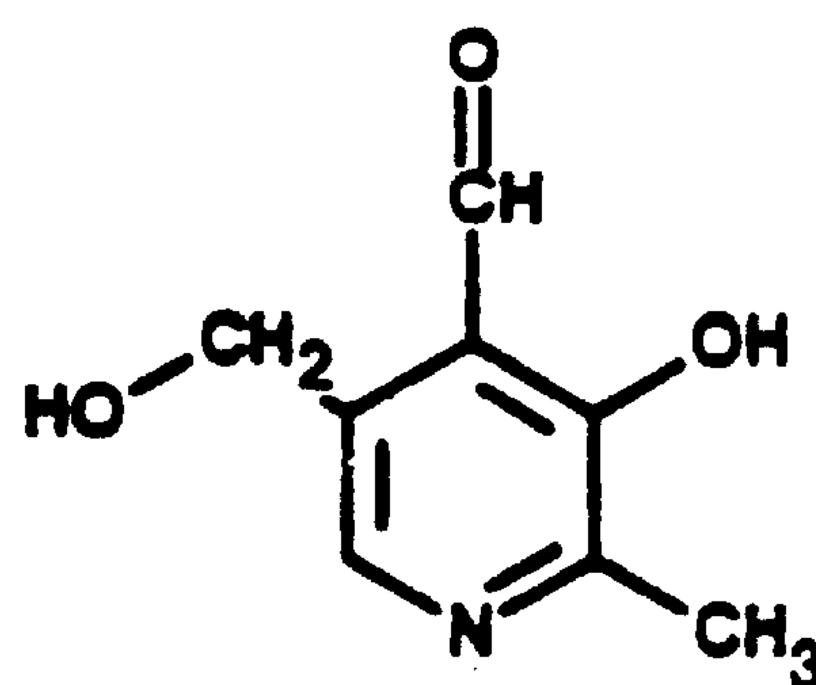
Pyridoxal
