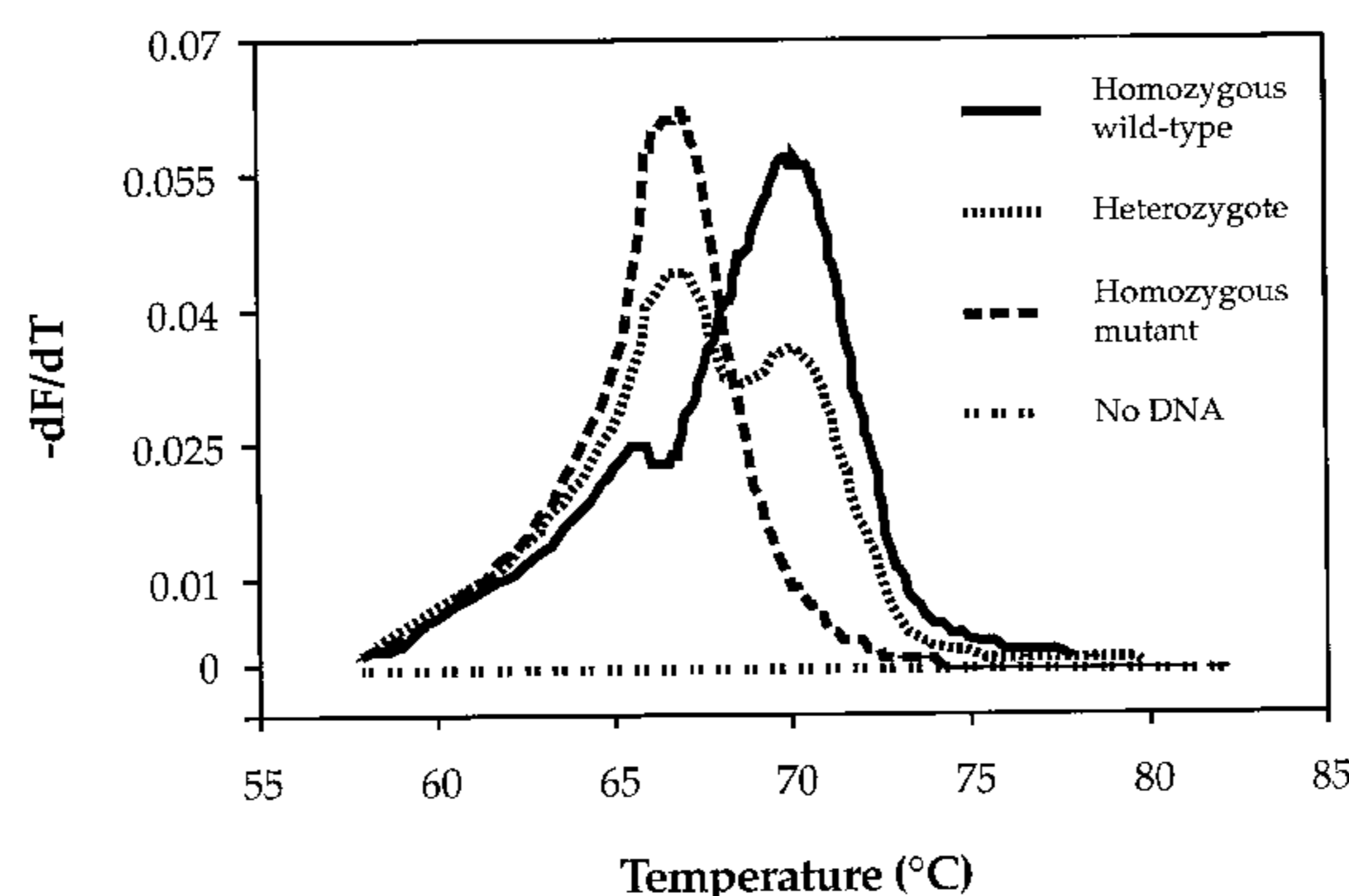
Melting Curves for Genotyping the Most Stable Mismatch
