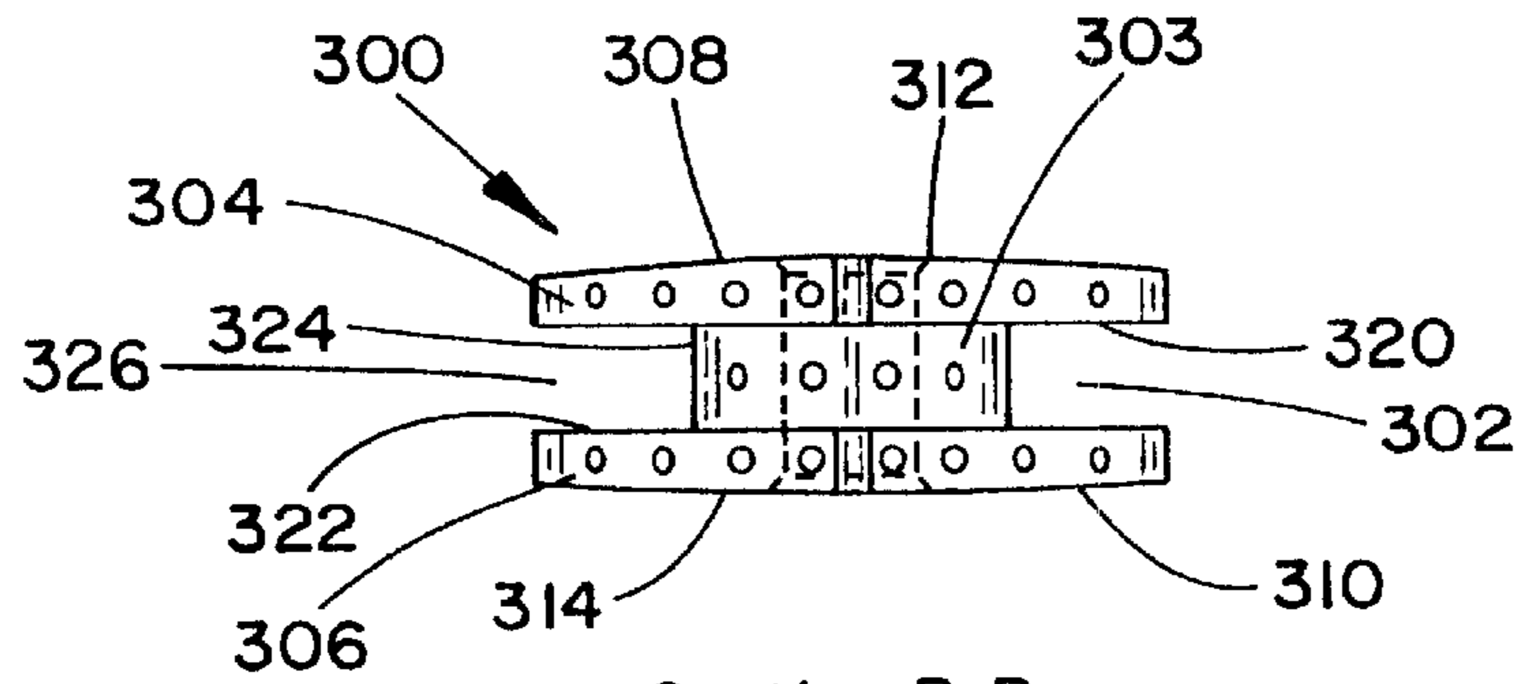
Section B-B
