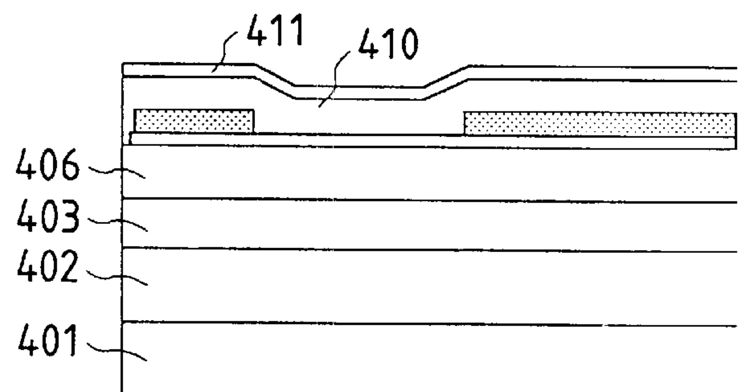
FIG. 5D SIMULTANEOUS FORMATION OF Ta AND SiN FILMS
