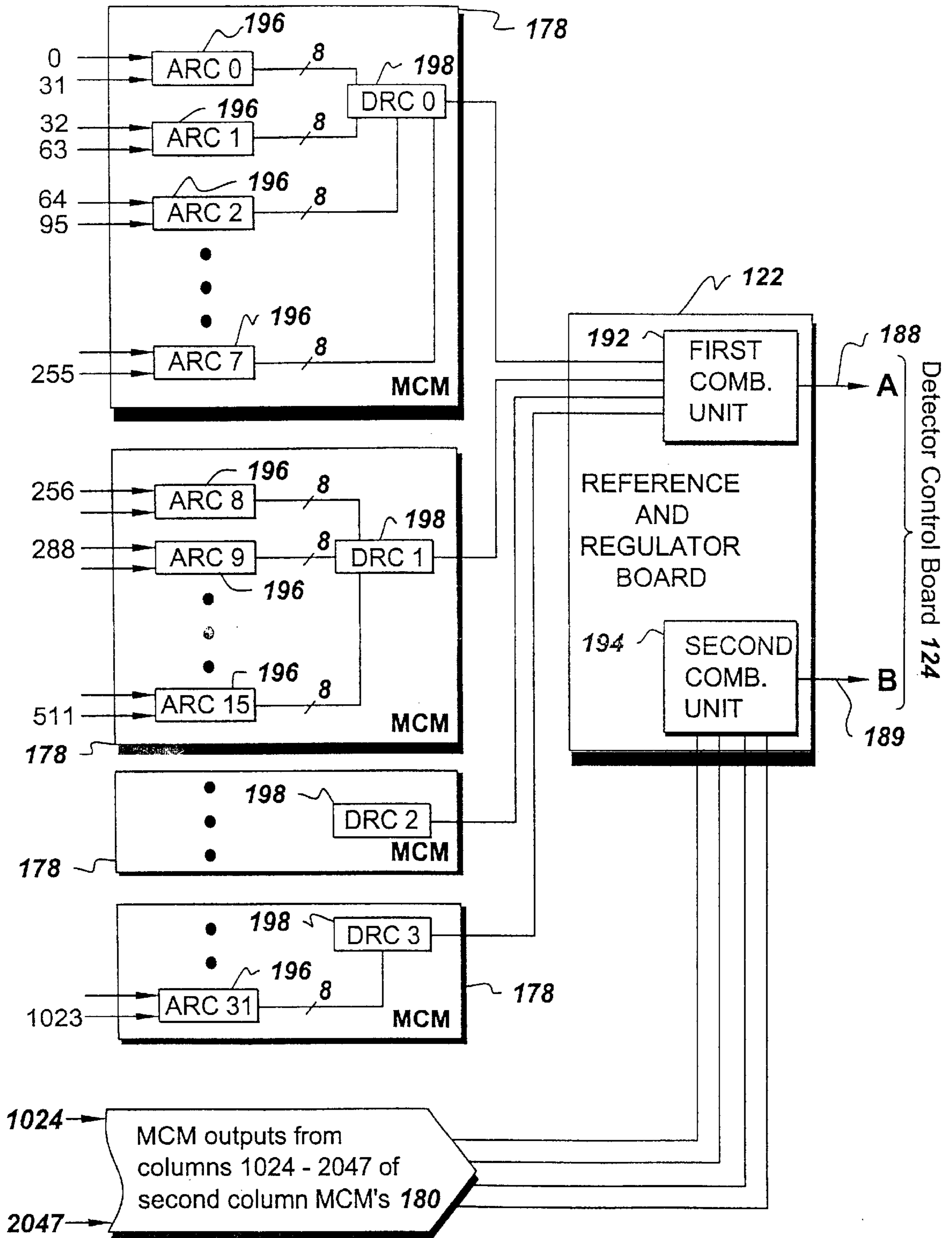
fig. 9 (PRIOR ART)
