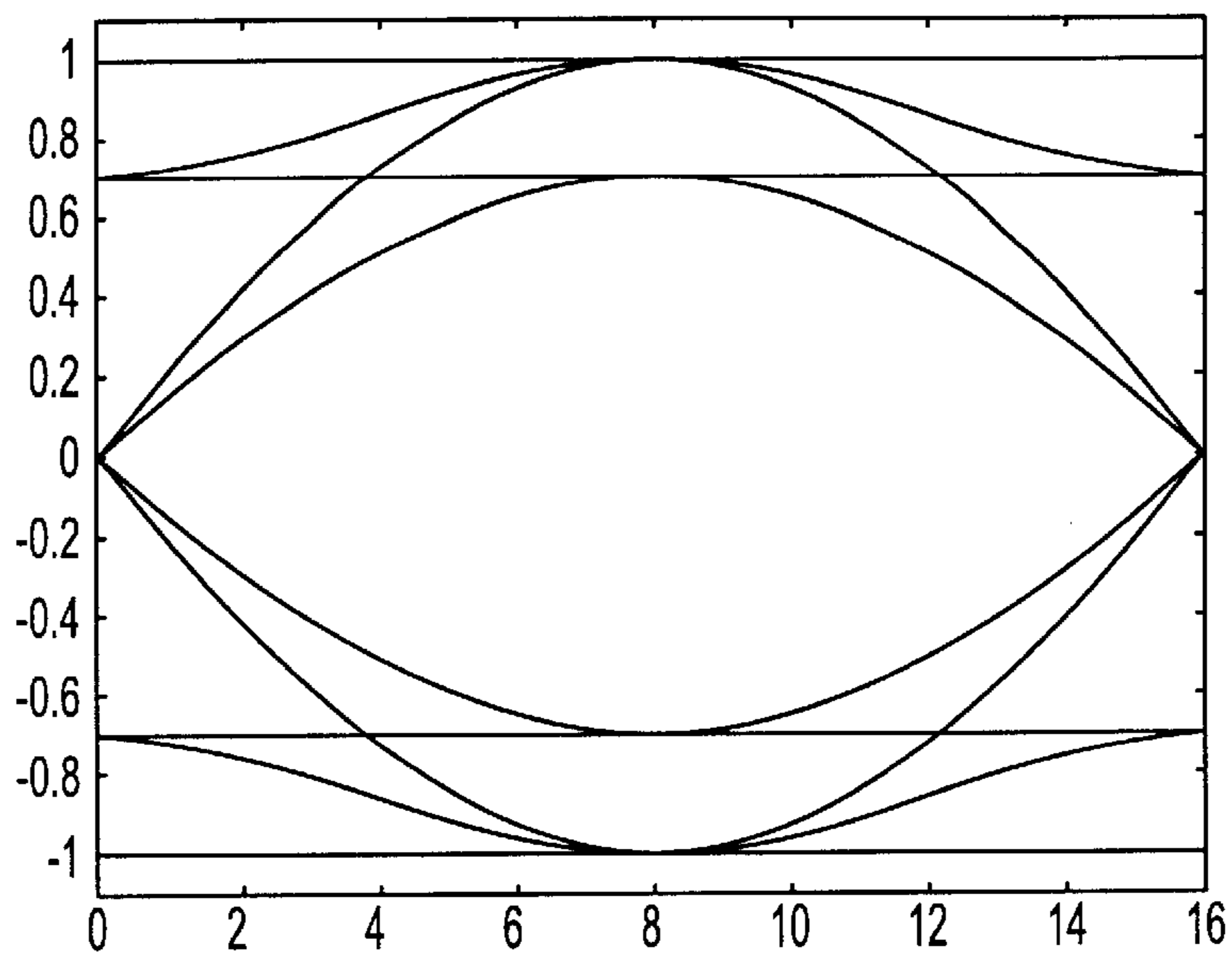
FQPSK COMPUTER. GENER. A=0.7, NO POST TCS FILTERING
