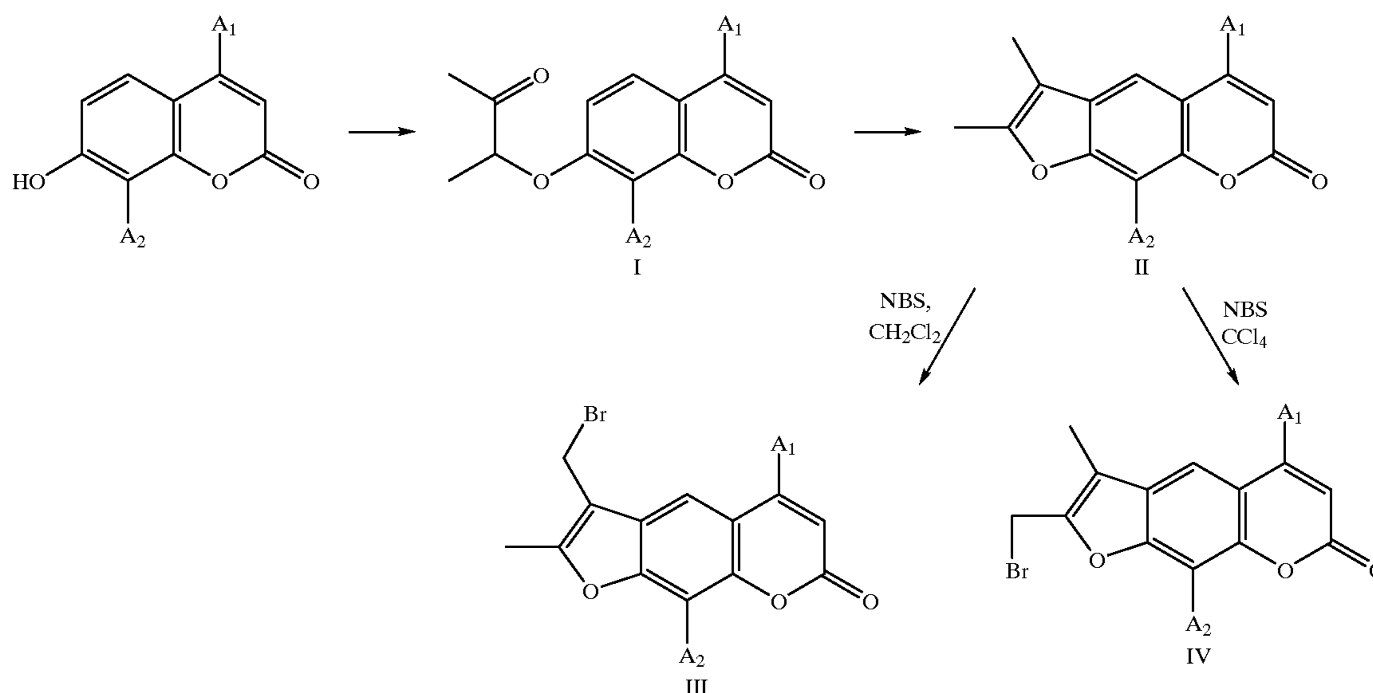
SCHEMATIC 1
