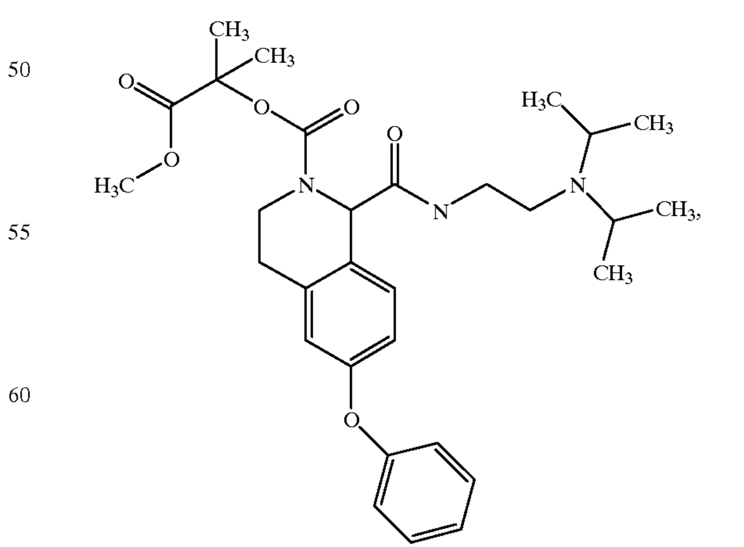
65 Isomer A
