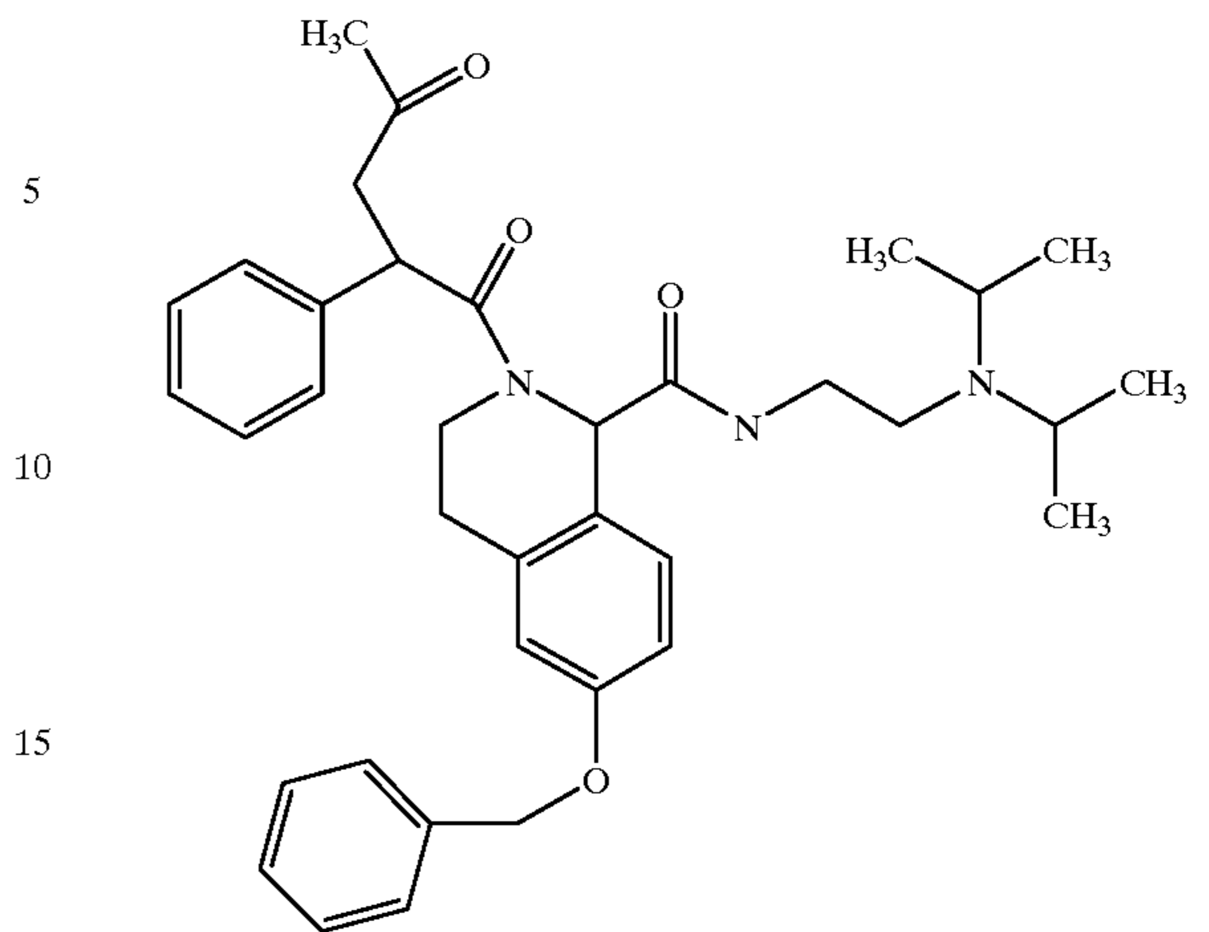
Isomer A
