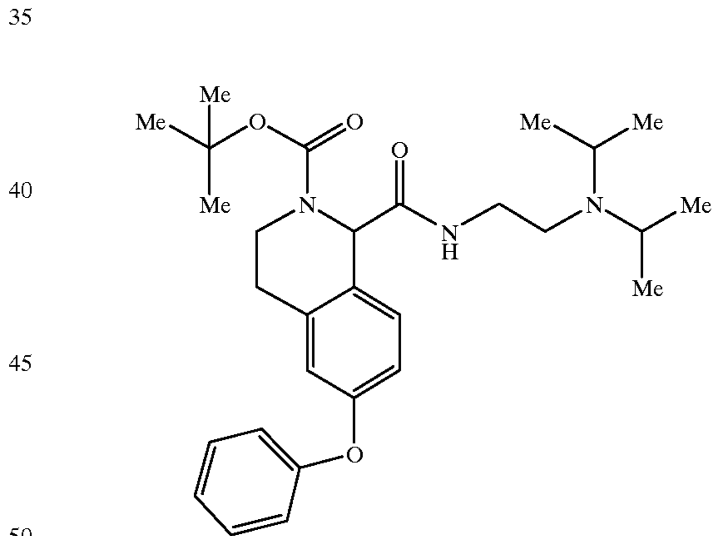
Isomer B
