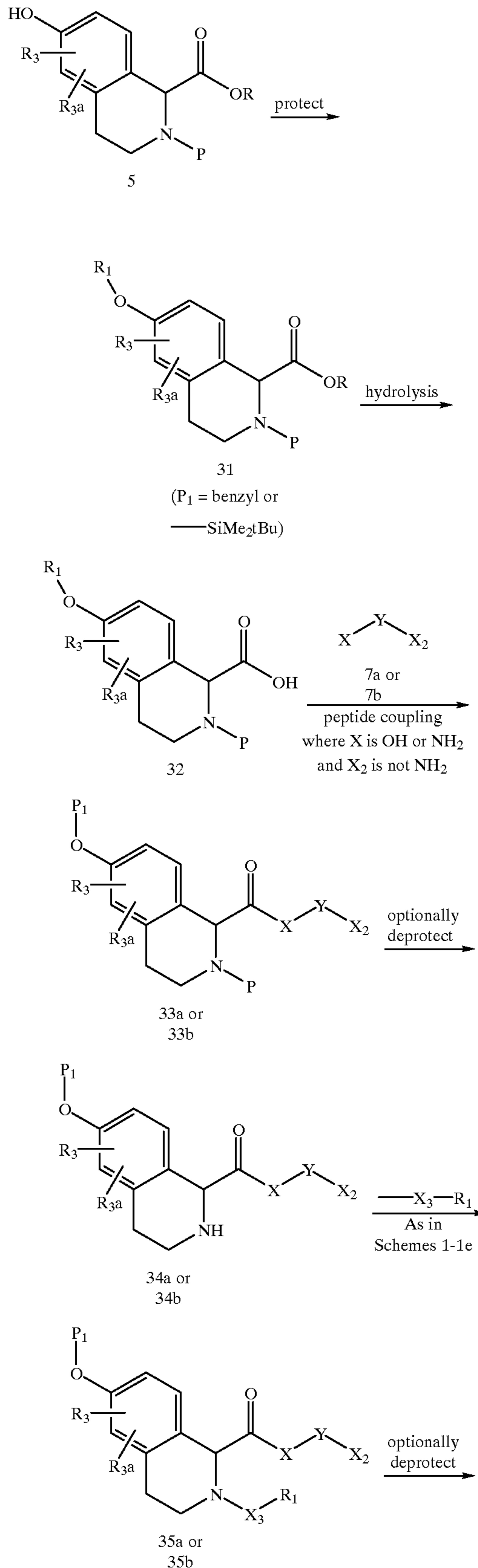
General Scheme 3
