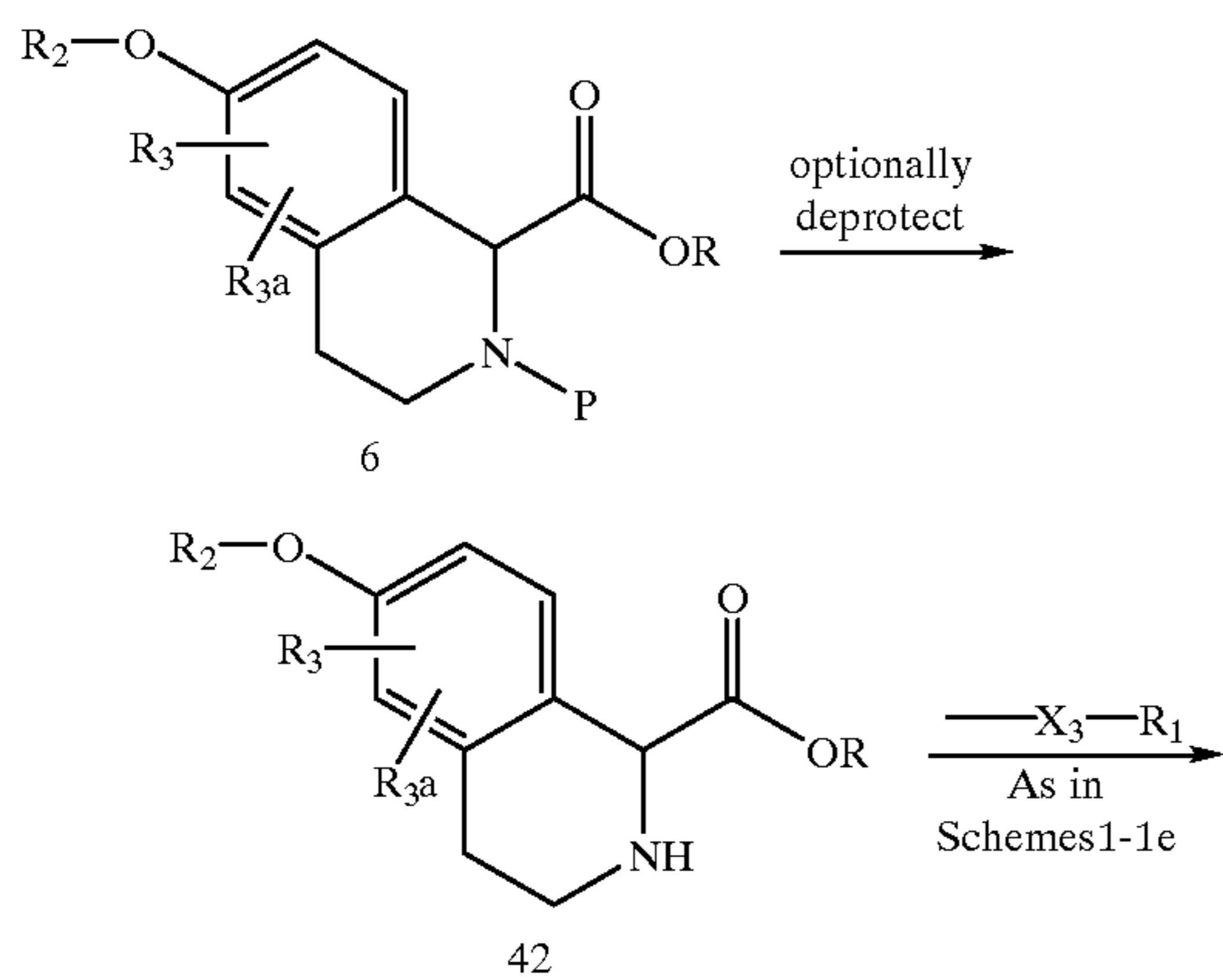
General Scheme 5
