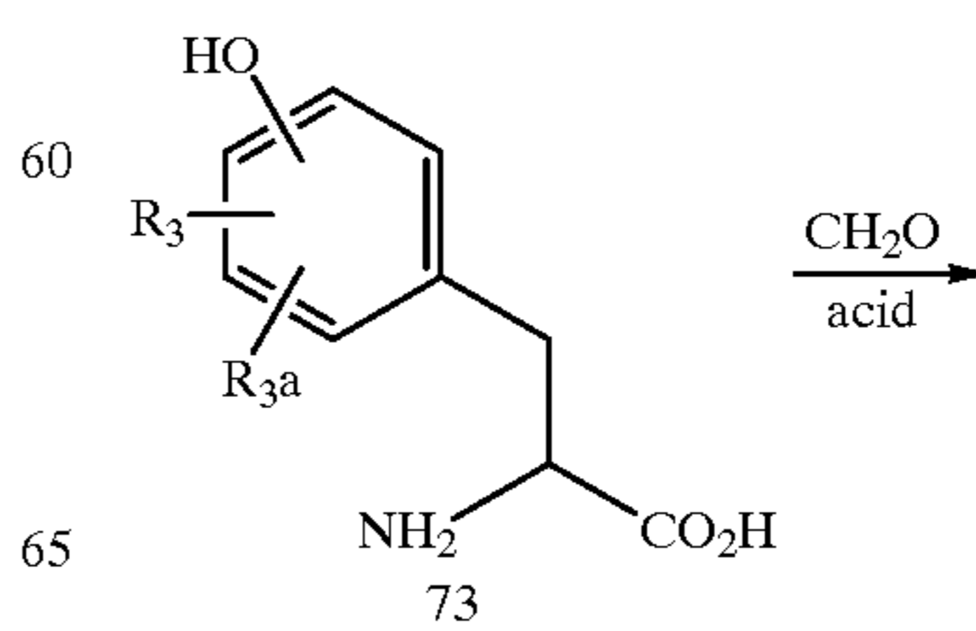
Scheme 11: Alternate Core
