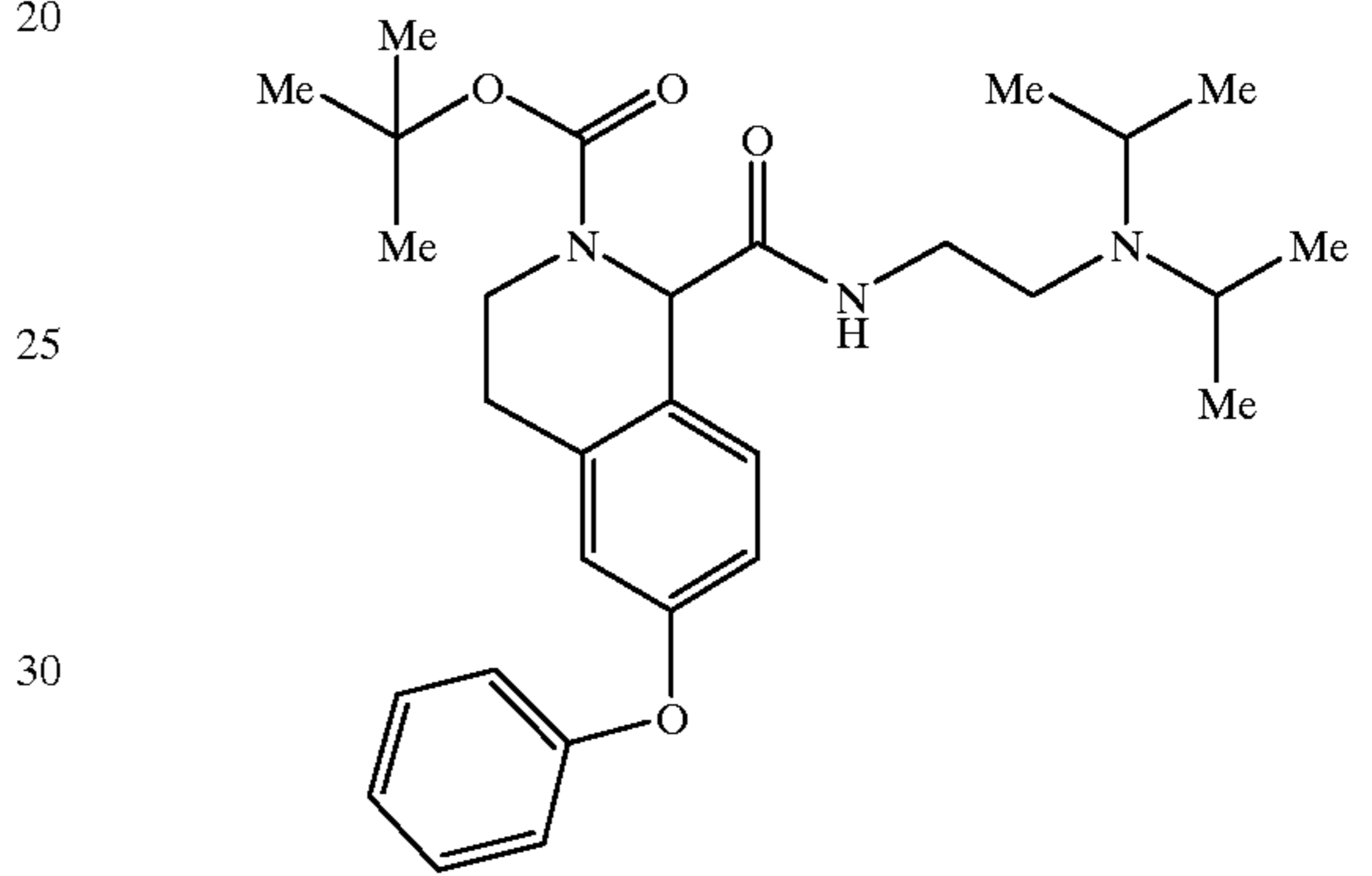
Isomer A
