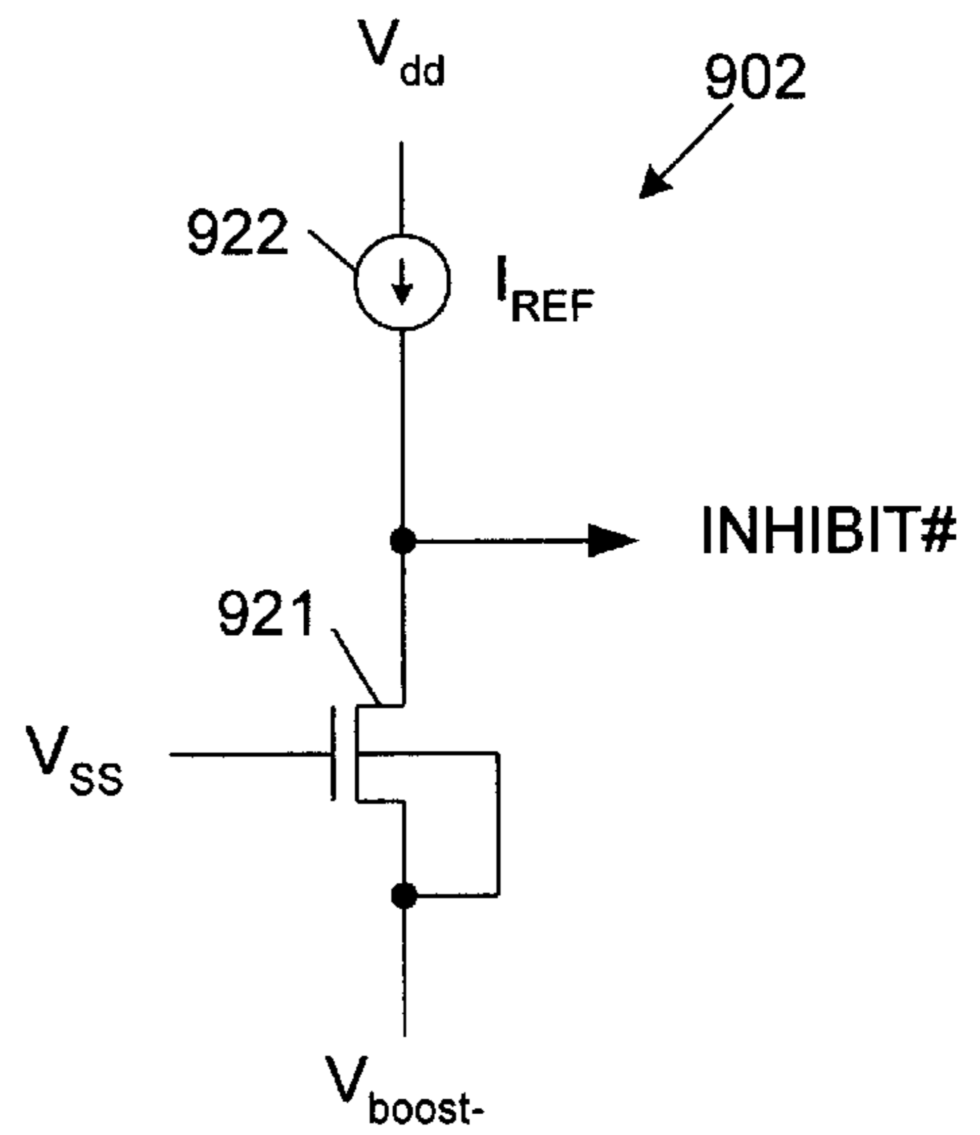
FIG. 9C (PRIOR ART)
