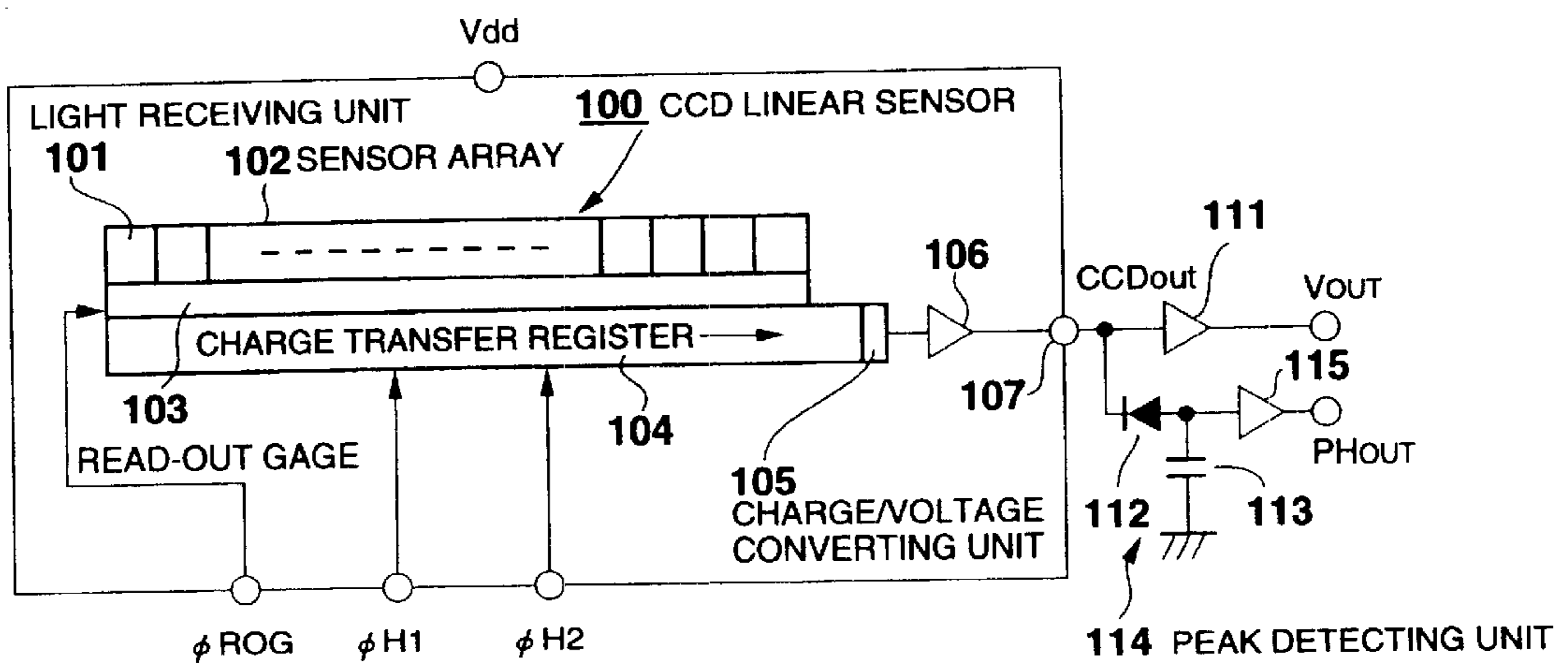
FIG. 11 (Related Art)
