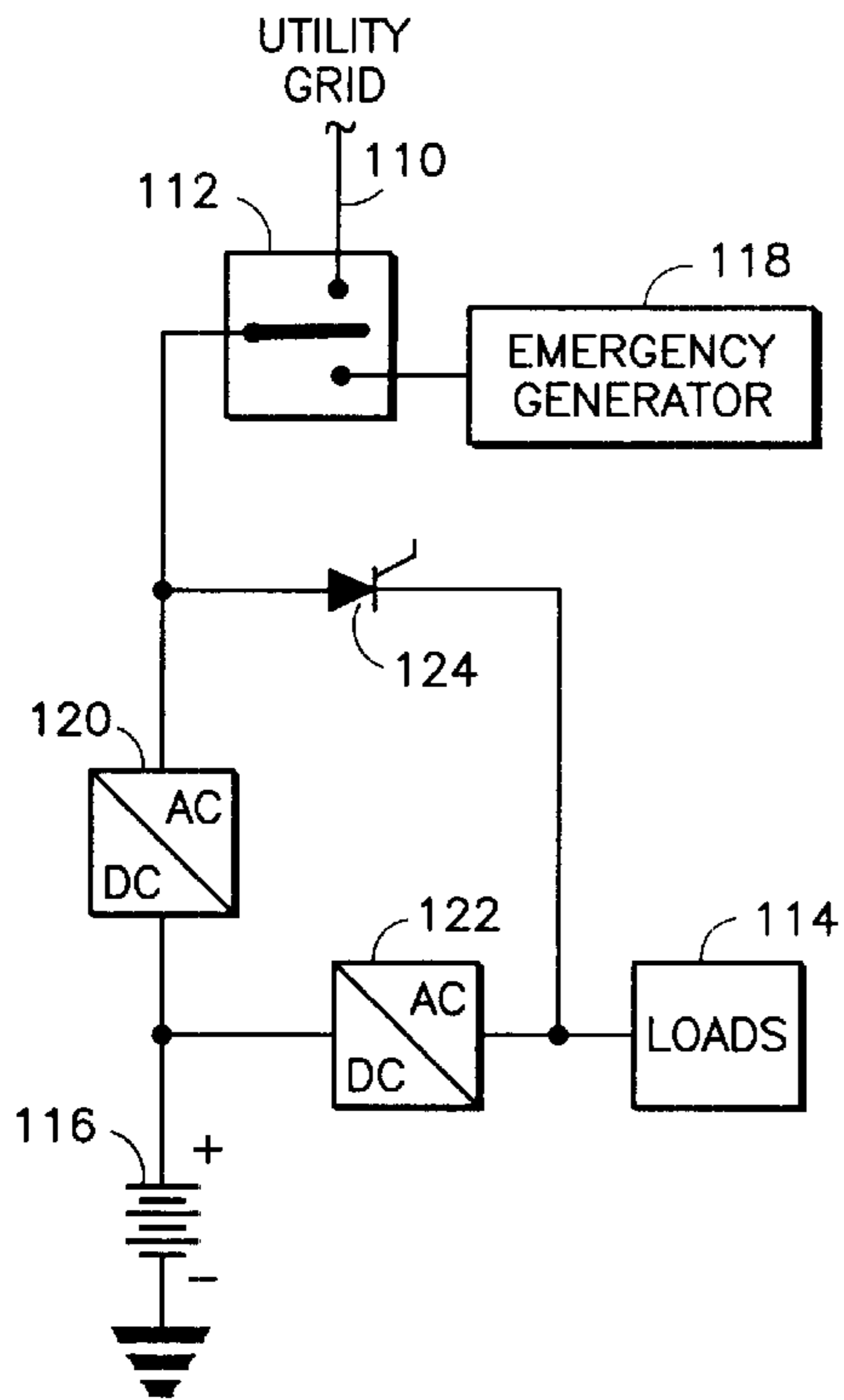
FIG. 1 Prior Art
