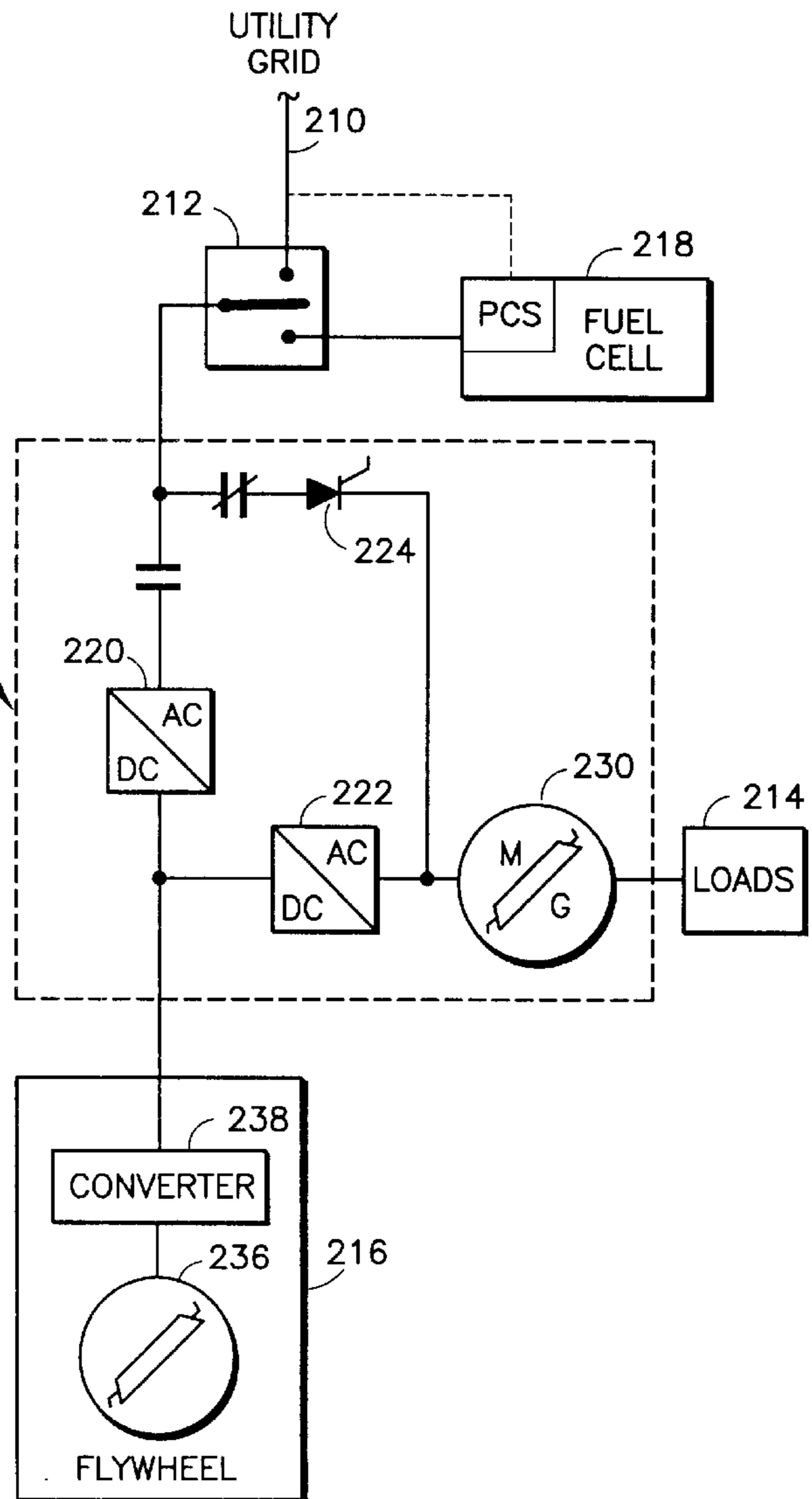
FIG. 2 Prior Art
