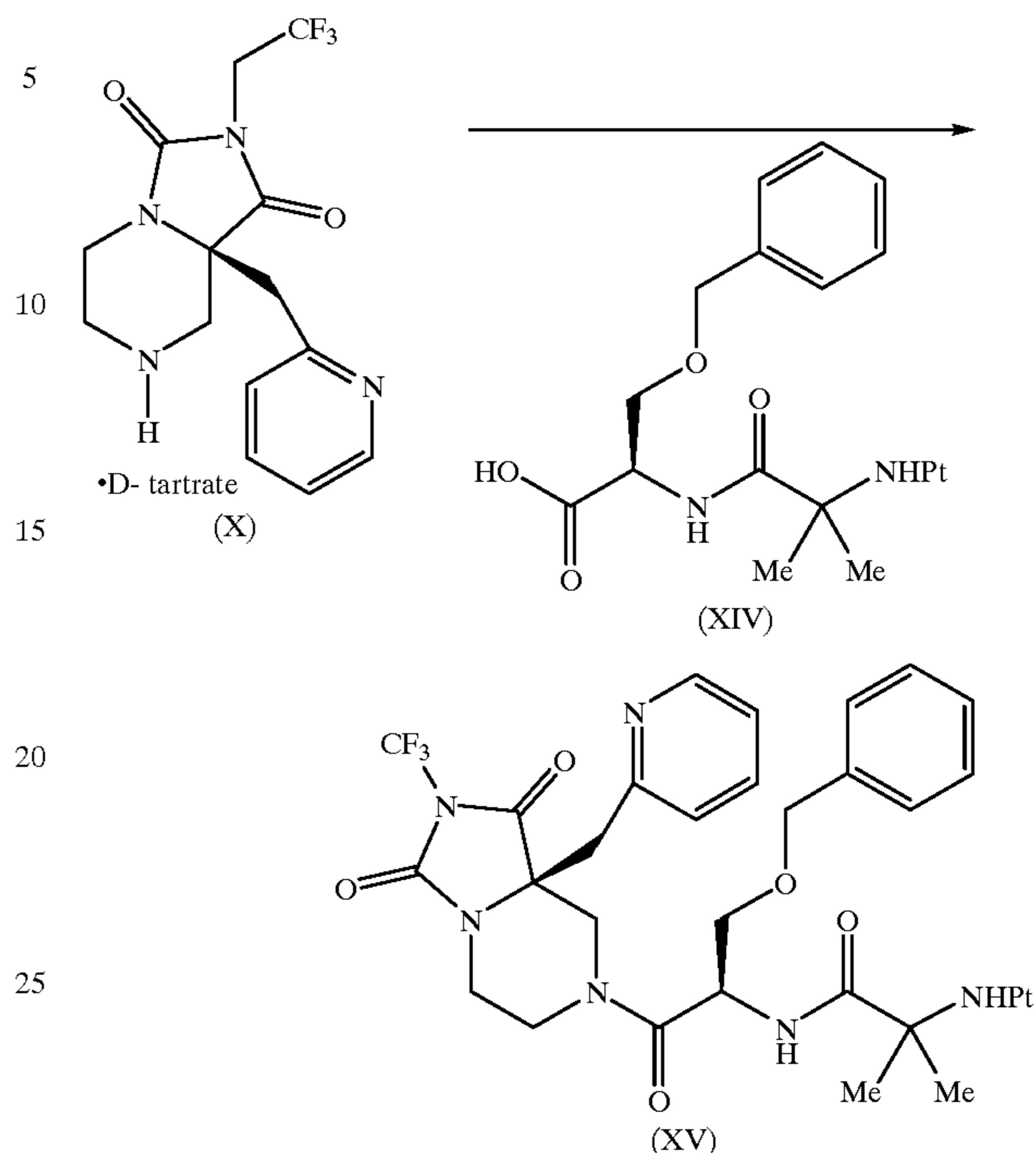
Scheme 4
