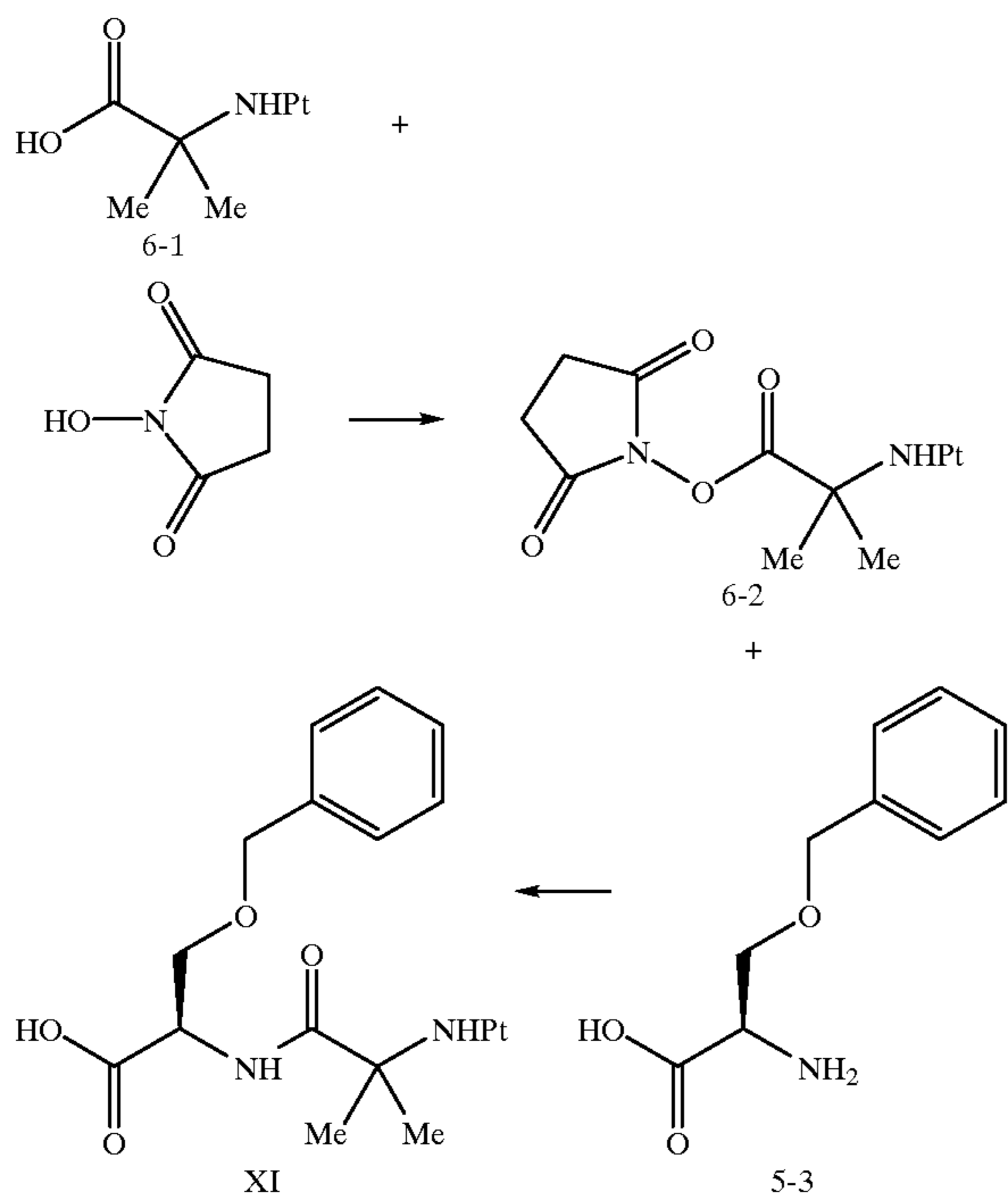
Scheme 6
