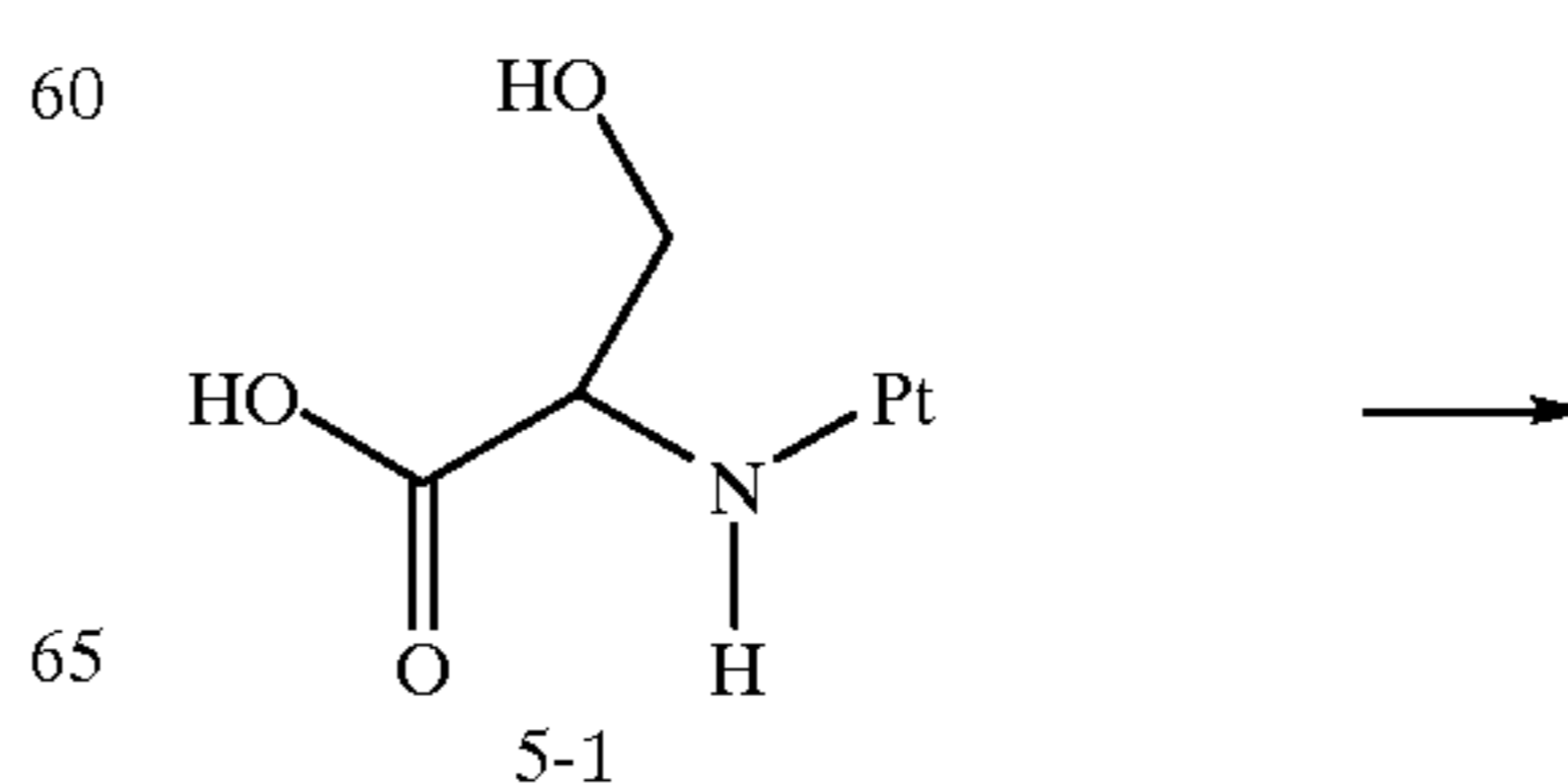
Scheme 5
