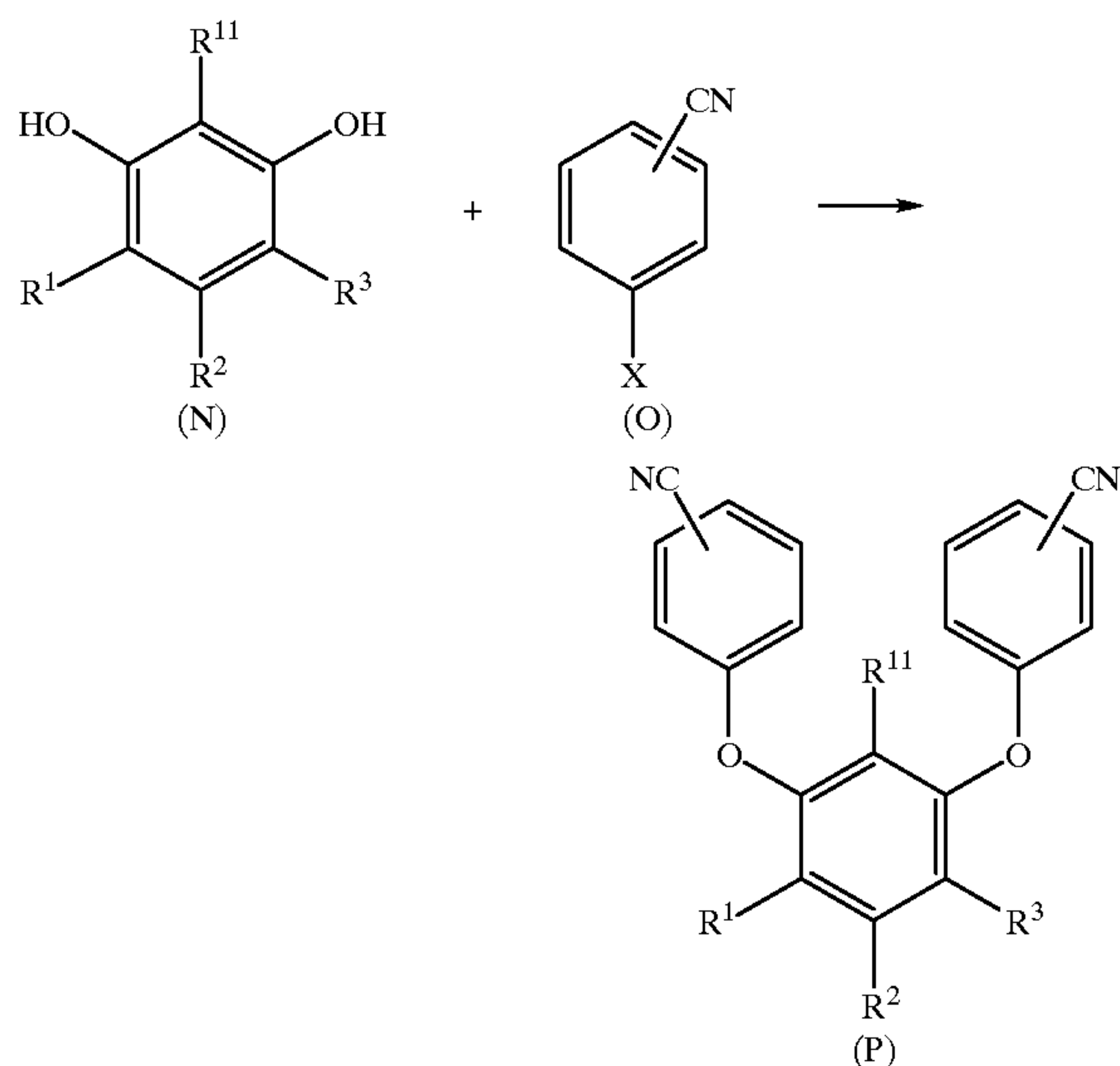
REACTION SCHEME 5
