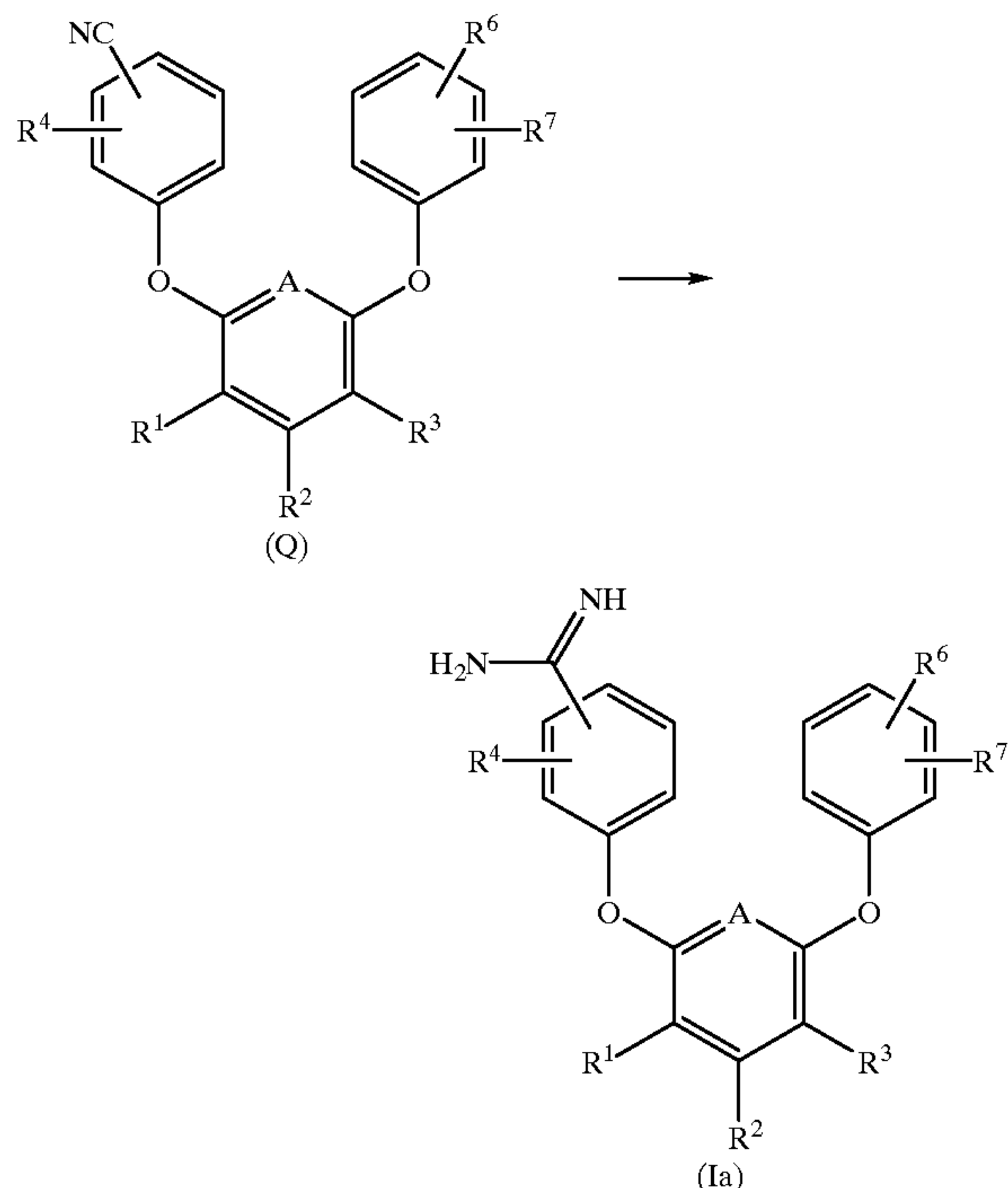
REACTION SCHEME 6
