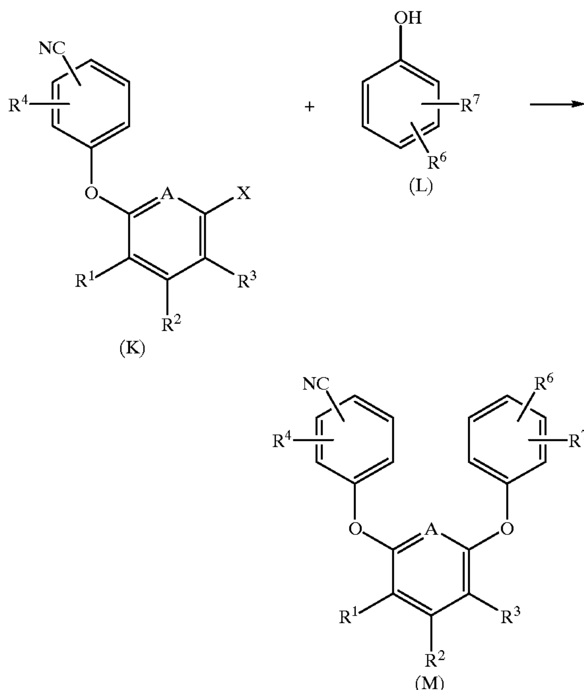
REACTION SCHEME 4
