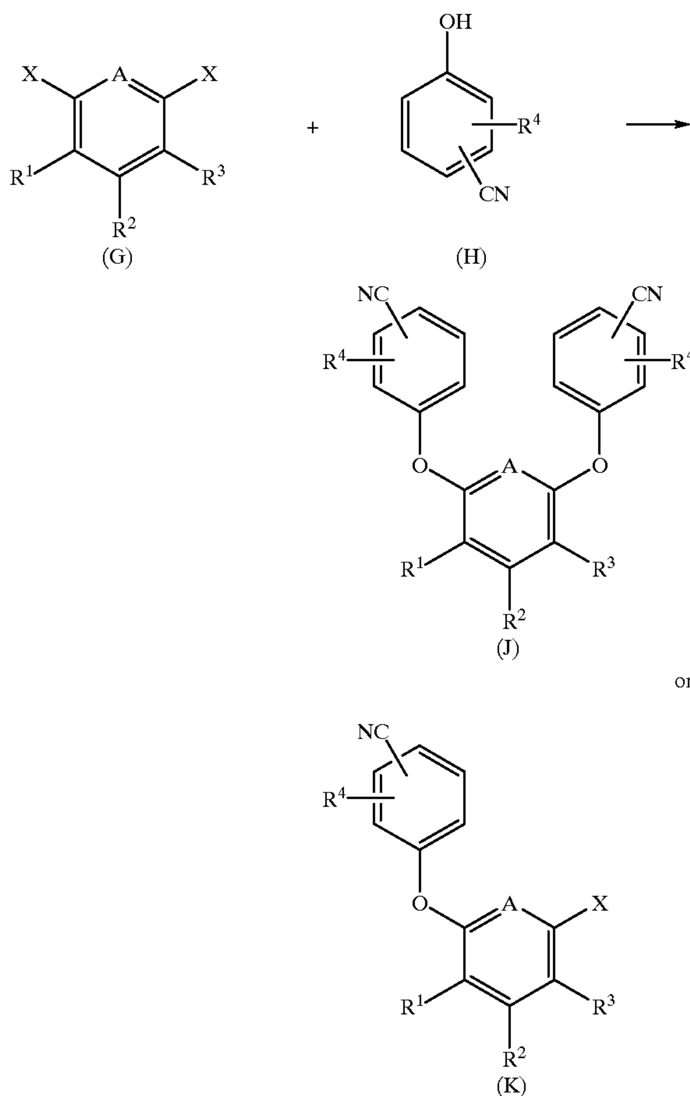
REACTION SCHEME 3
